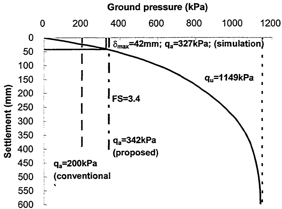
Figure 6-8 Load settlement curve for Fort Nelson case
