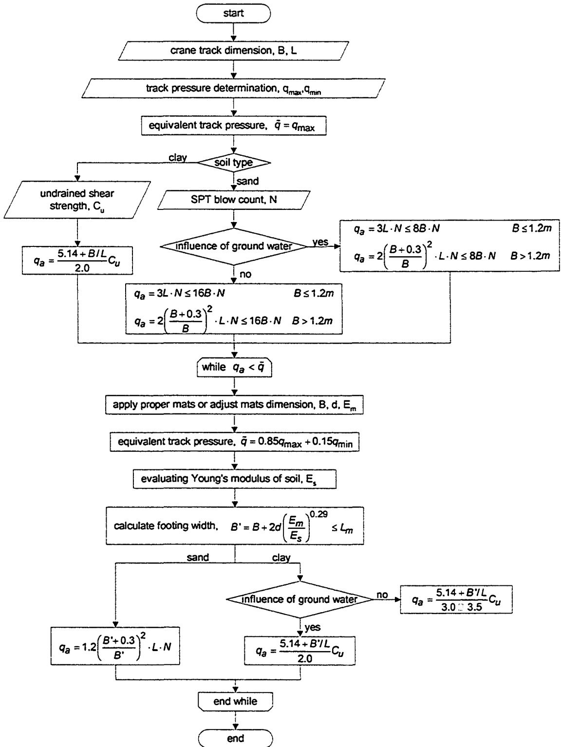
Figure 7-1 Procedures to determine the bearing capacity for crawler crane
