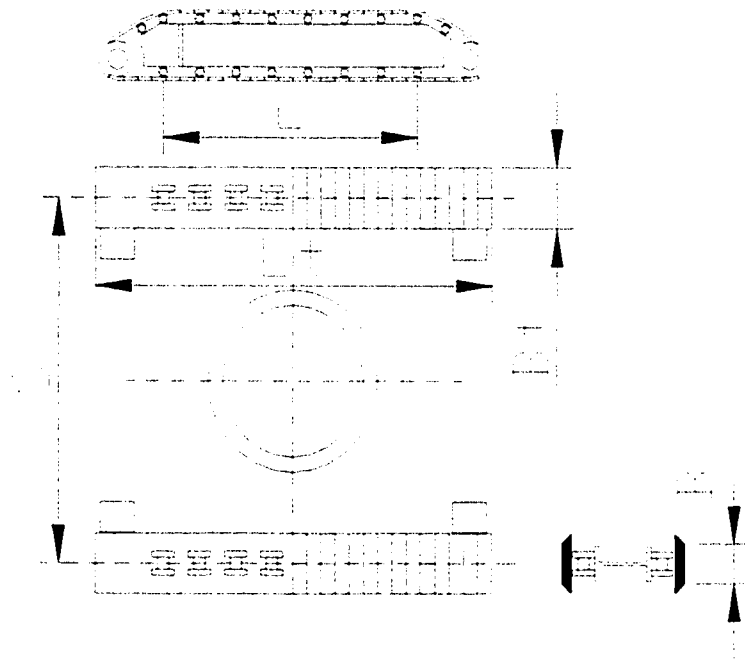
Figure 3-1 Dimensions of supporting area of crane tracks (Modified from Becker 2001)
