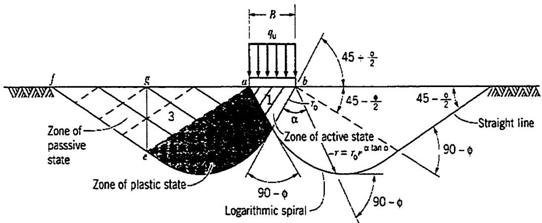
Figure 2-3 Prandtl's plastic equilibrium model
