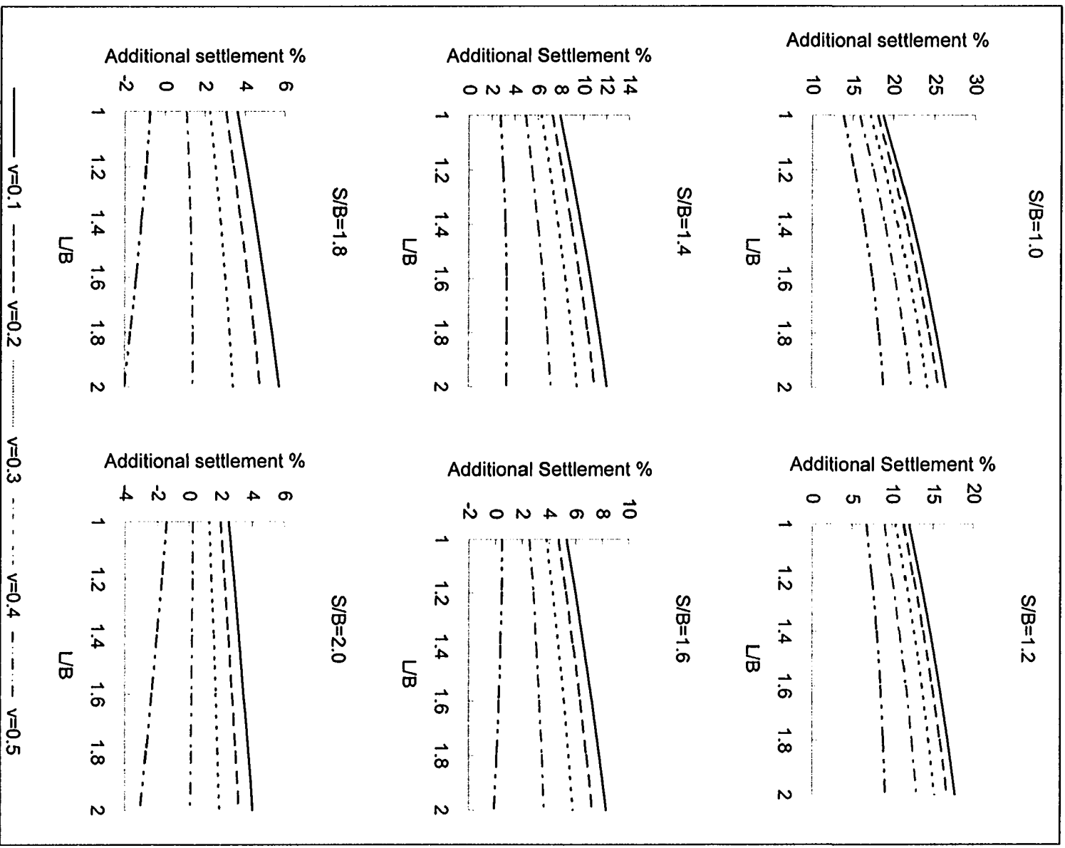
Figure 4-1 Additional settlement caused by adjacent footing
