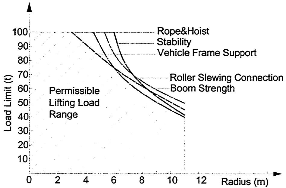
Figure 3-2 Load limits of crane with short boom (Modified from Becker 2001)
