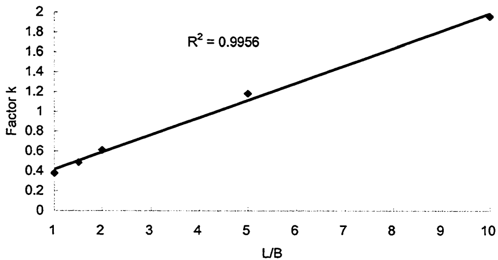
Figure 4-9 Correlation of factor k with L/B ratio
