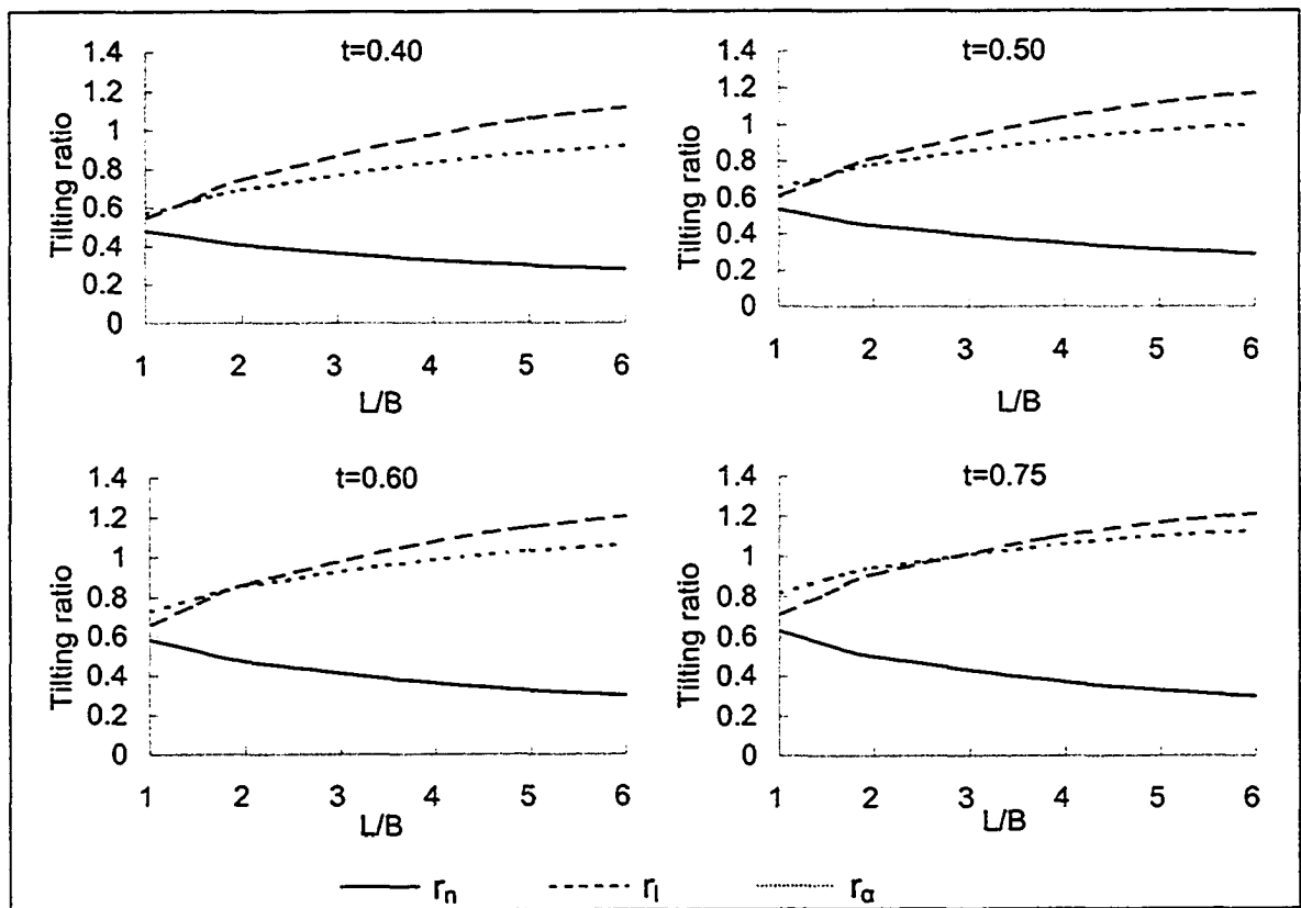
Figure 4-7 Variation of tilting ratios
