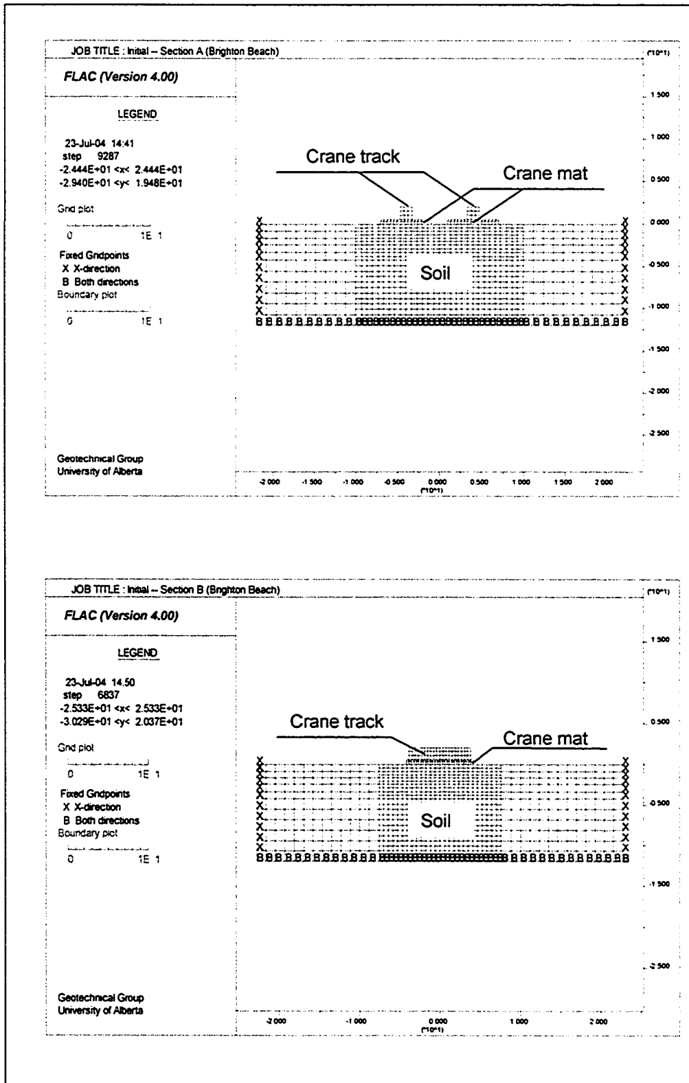
Figure 6-3 Model configuration for Brighton Beach case
