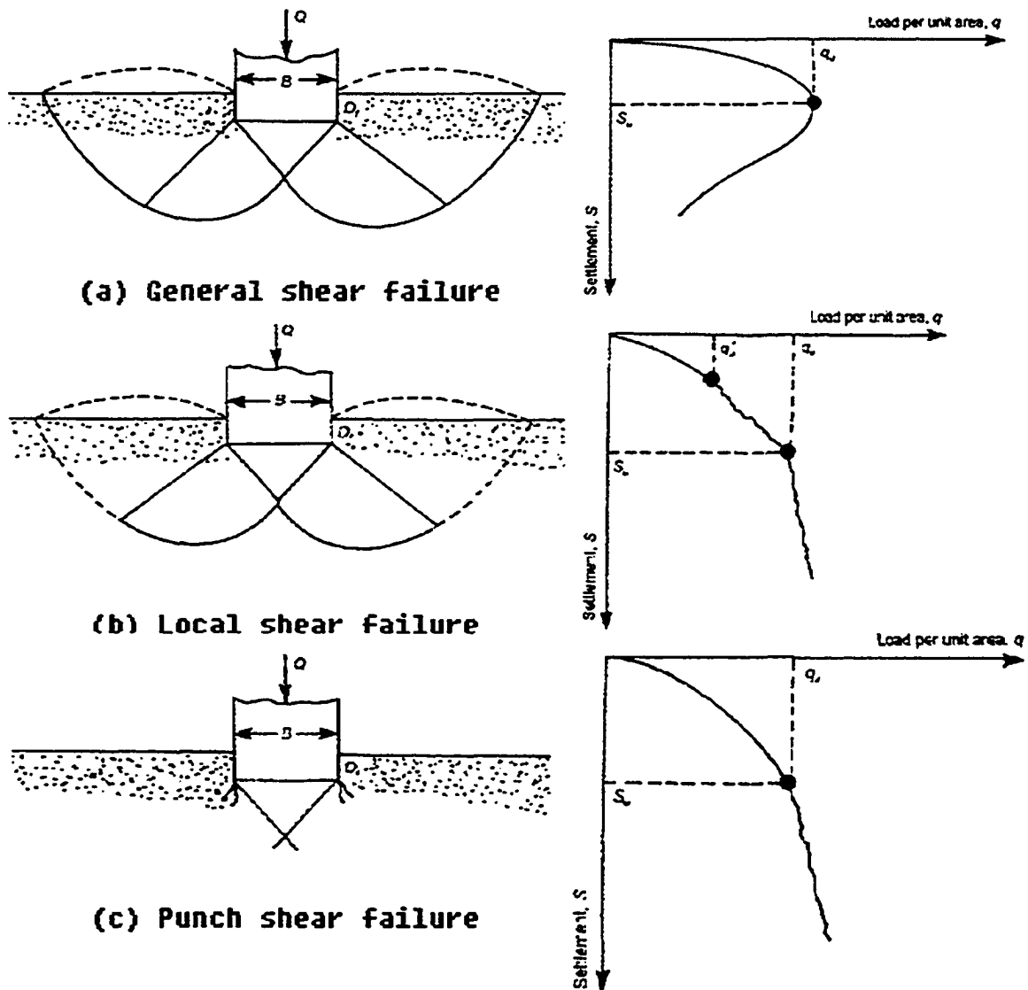
Figure 2-1 Modes of bearing capacity failure (from Vesic, 1963)
