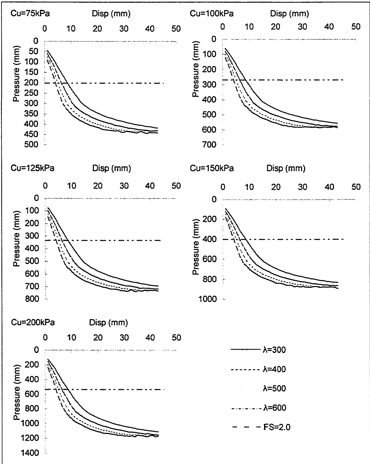
Figure 5-10 Load immediate settlement curve of stiff clay for crane without mat
