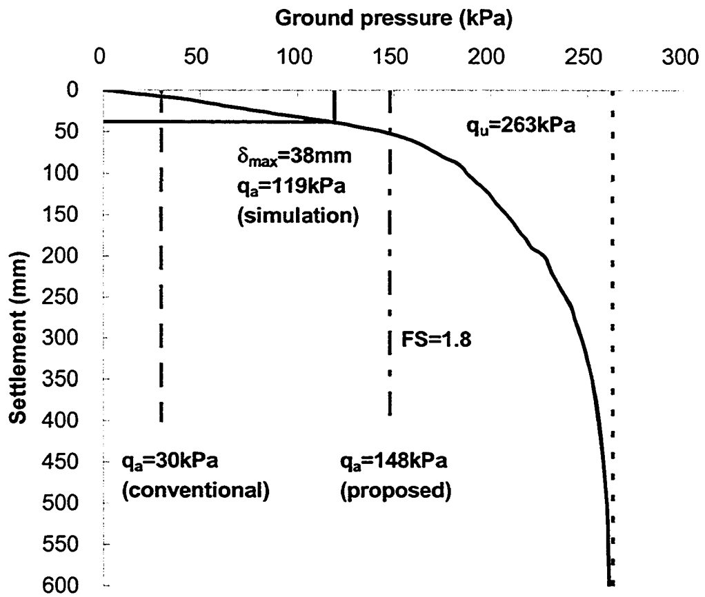
Figure 6-4 Load settlement curve for Brighton Beach case
