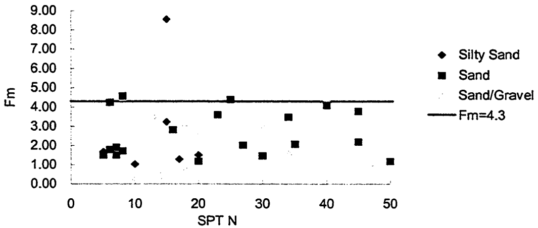
Figure 5-4 Factor F for crane with mats
