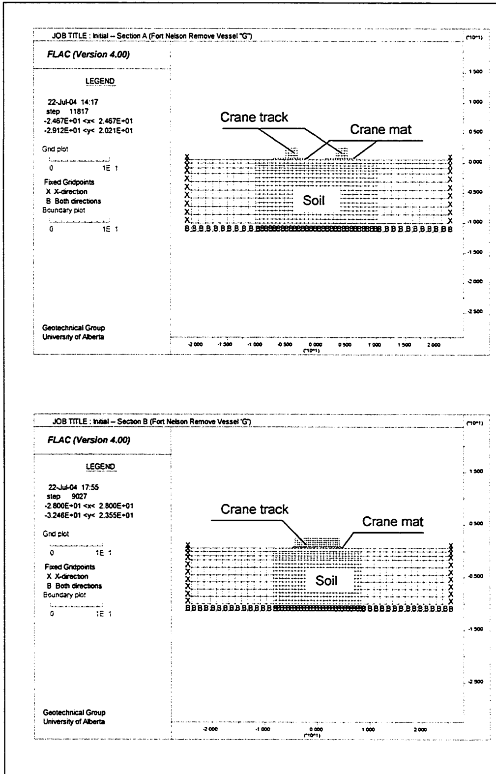
Figure 6-5 Model configuration for Fort Nelson case
