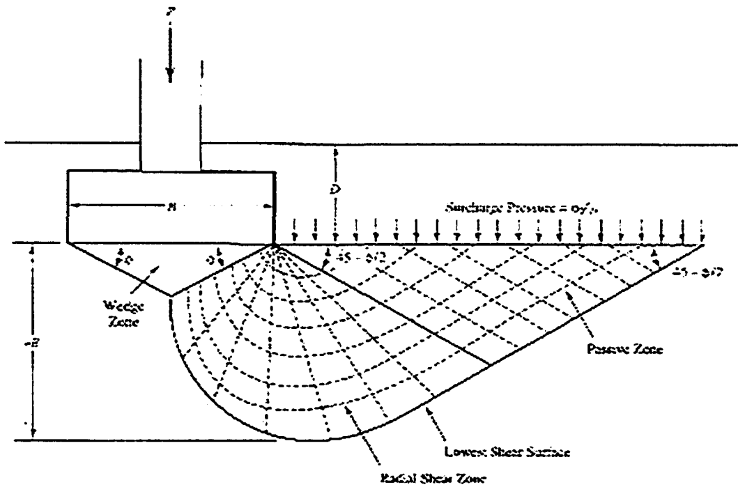
Figure 2-4 Geometry of Terzaghi's bearing capacity model
