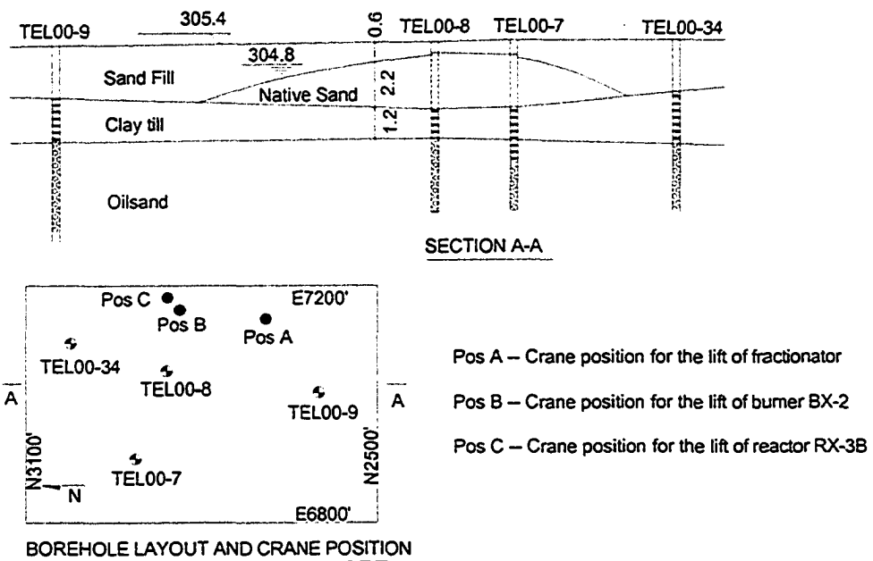
Figure 6-9 Crane layout and soil stratification of Fort McMurray case
