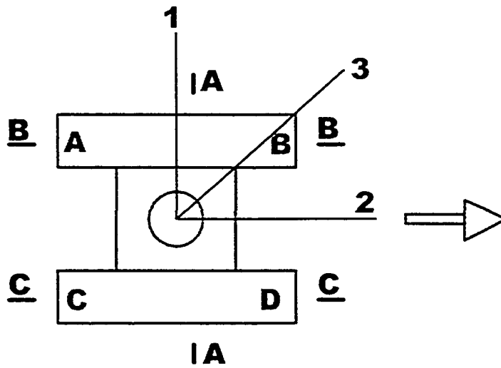
Figure 4-2 Sections to be modeled and critical boom orientations
