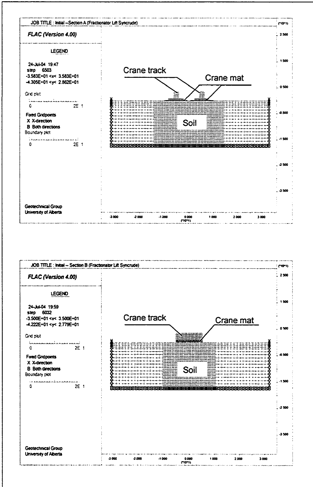
Figure 6-10 Model configuration for the Fractionator lift at Fort McMurray
