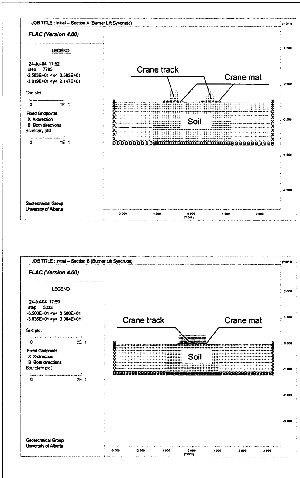
Figure 6-11 Model configuration for the lift of burner and reactor at Fort McMurray
