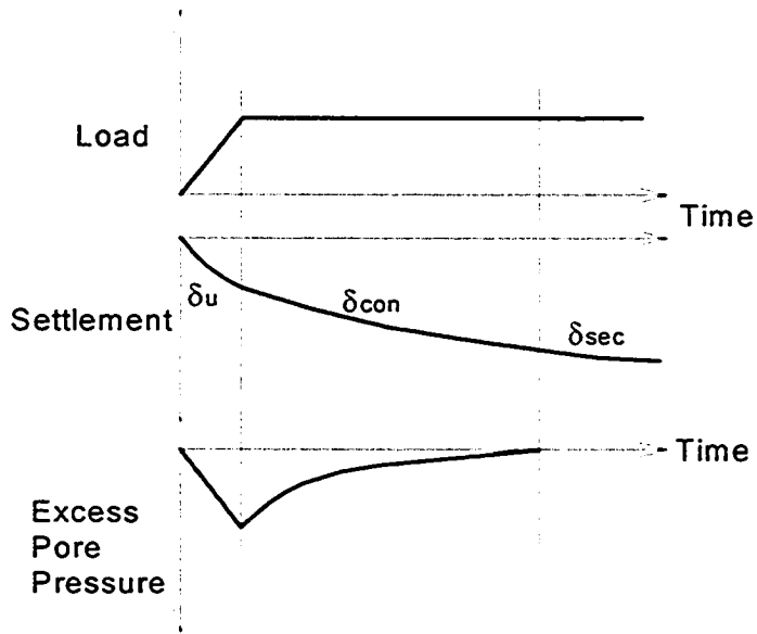
Figure 2-8 Development of settlement with time
