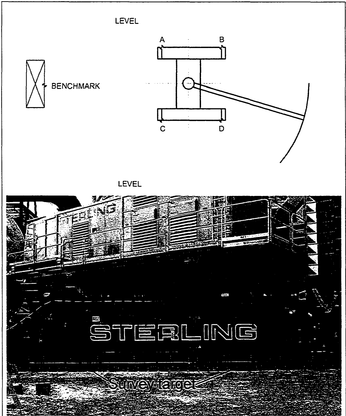
Figure 6-1 Typical level and targets layout for settlement observation
