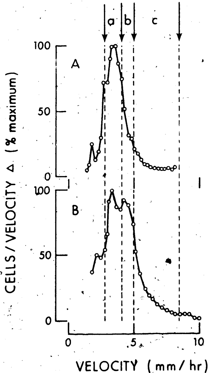
Figure 21. A typical velocity sedimentation distribution profile of:
