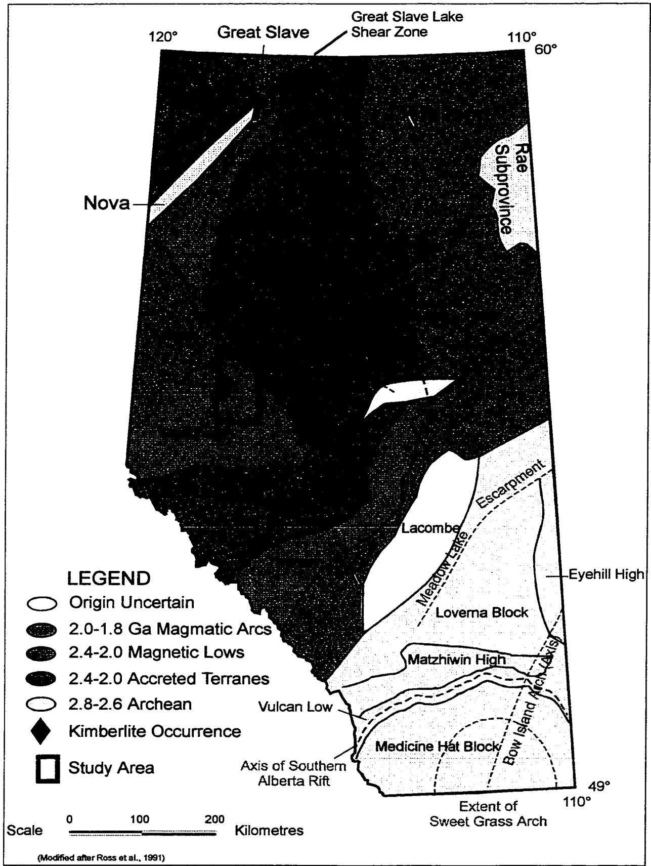
FIGURE 2.1 Basement Geology of Alberta
