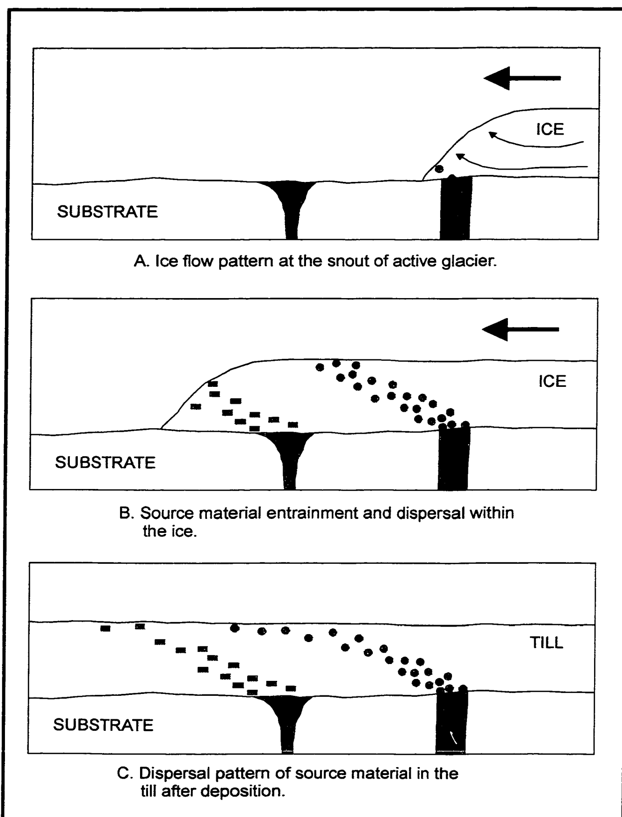
FIGURE 7.1 - Entrainment and dispersal patterns of material from source points.
