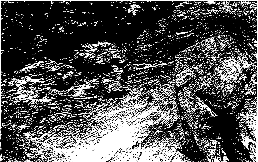
PLATE 5.5 - Dewatering structures, convulsion and slumping near Watino.
