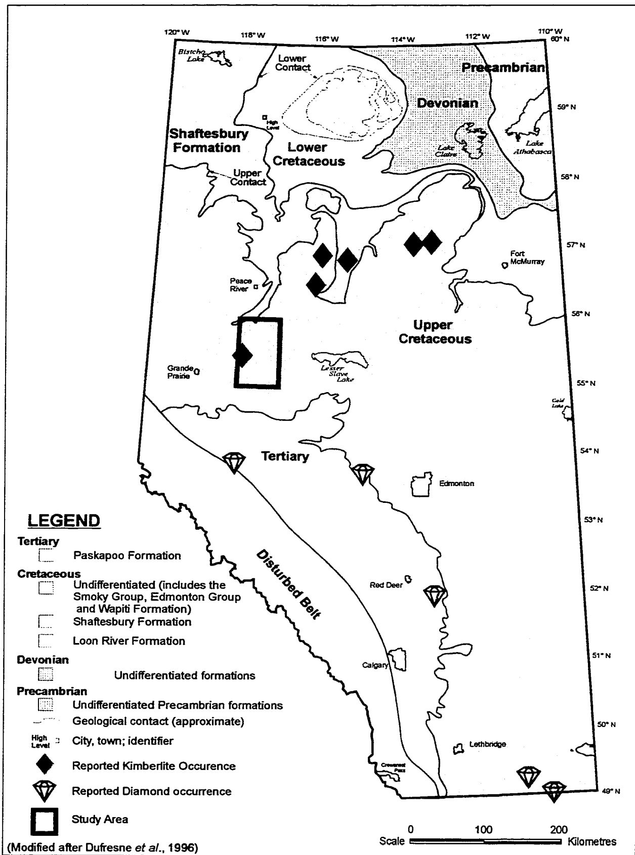
FIGURE 2.2 Generalised Geology of Alberta
