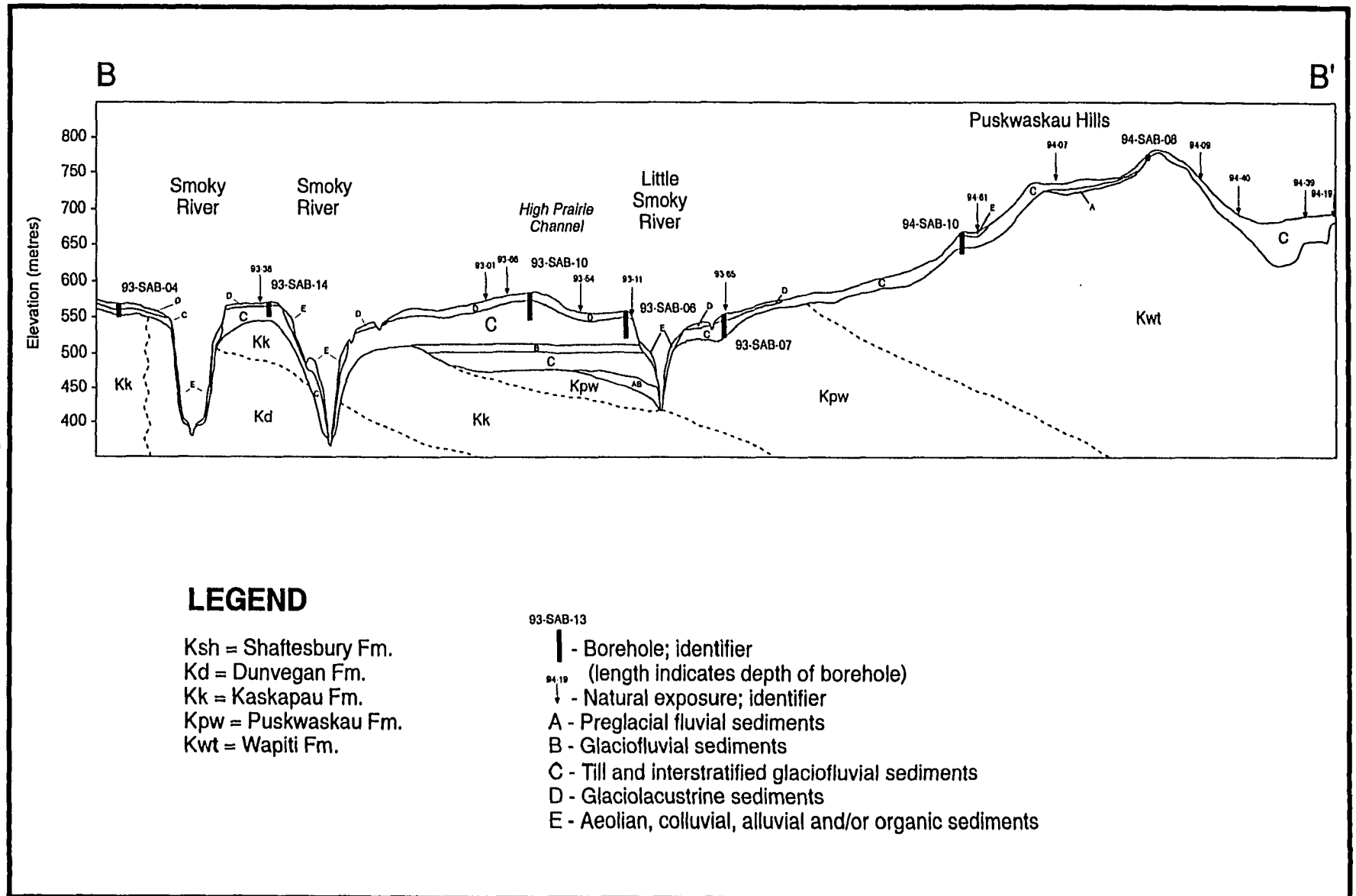
FIGURE 6.4 Cross-section B-B'.
