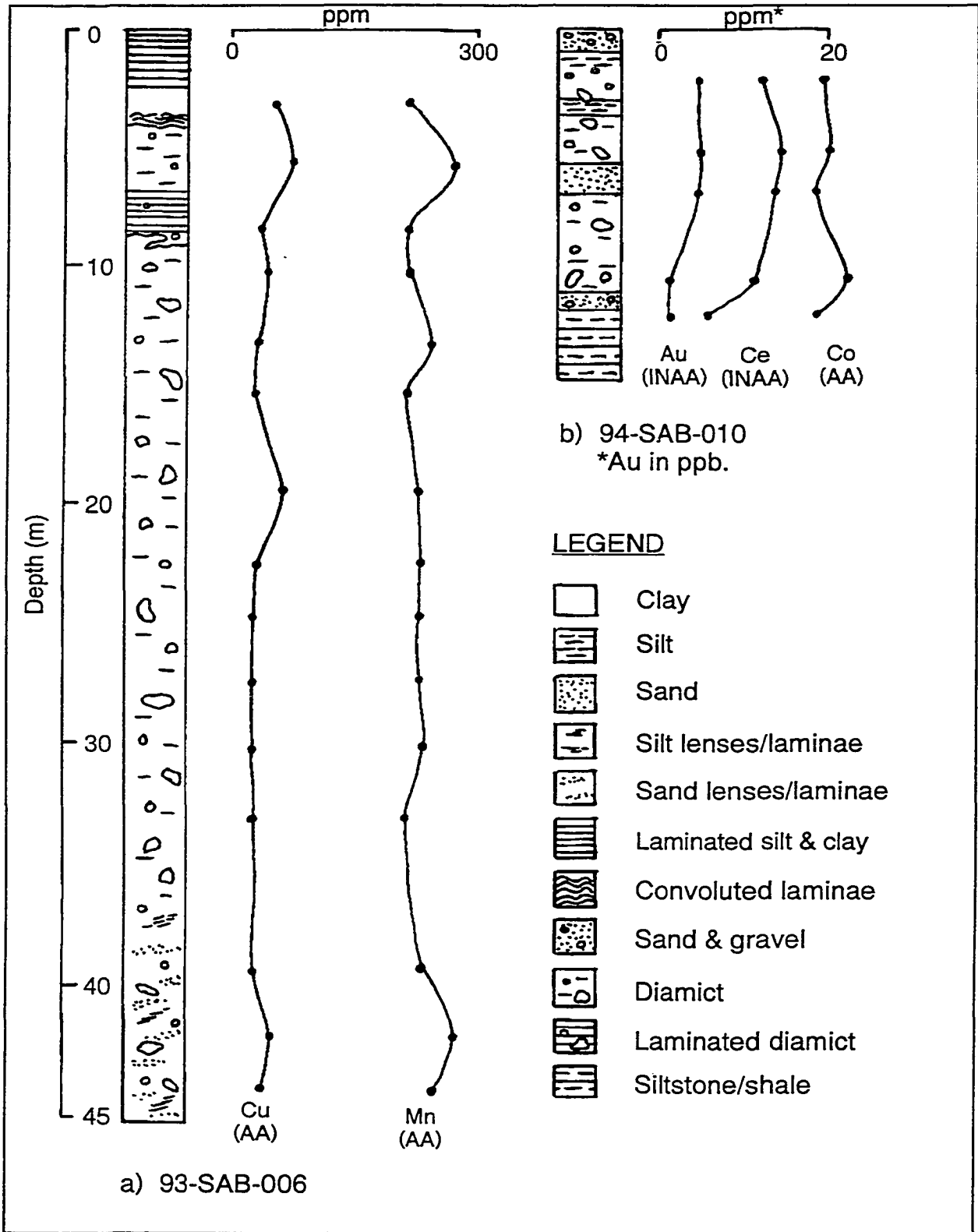
FIGURE 4.1 Vertical profiles of selected borehole geochemistry.
