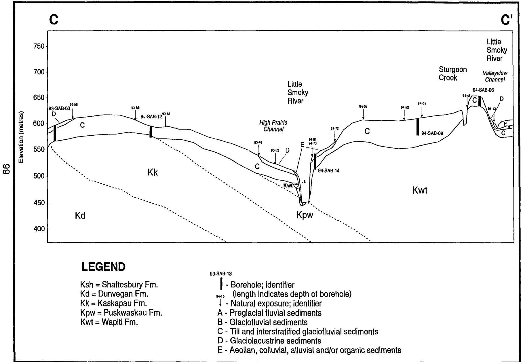
FIGURE 6.5 Cross-section C-C'.
