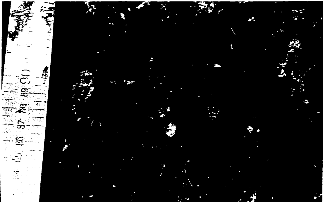
PLATE 5.14 - Weathered diamict with gypsum mineralisation.
