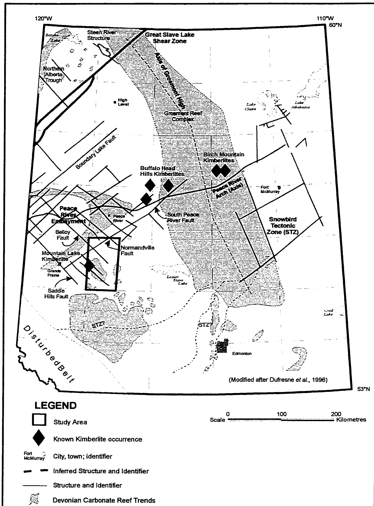
FIGURE 2.3 Structural Geology of Northern Alberta
