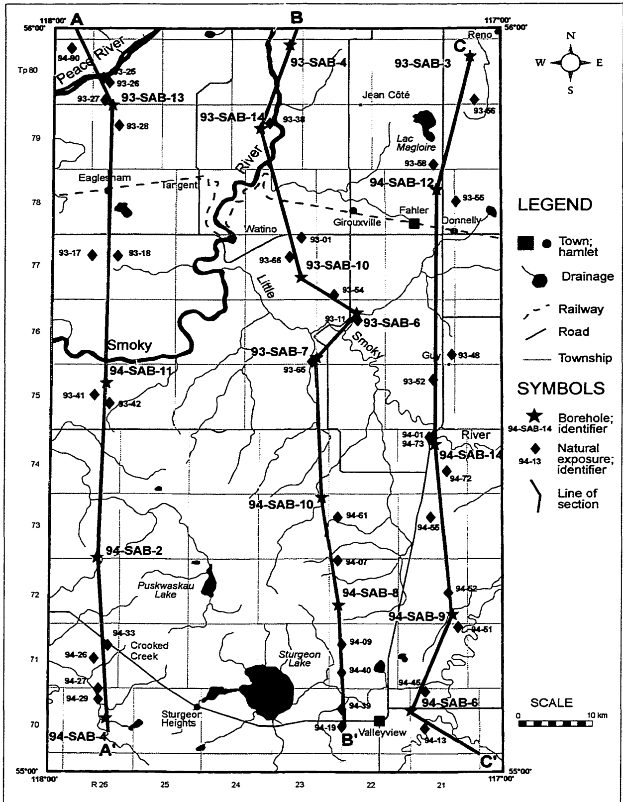
FIGURE 6.2 Location of Cross-sections.
