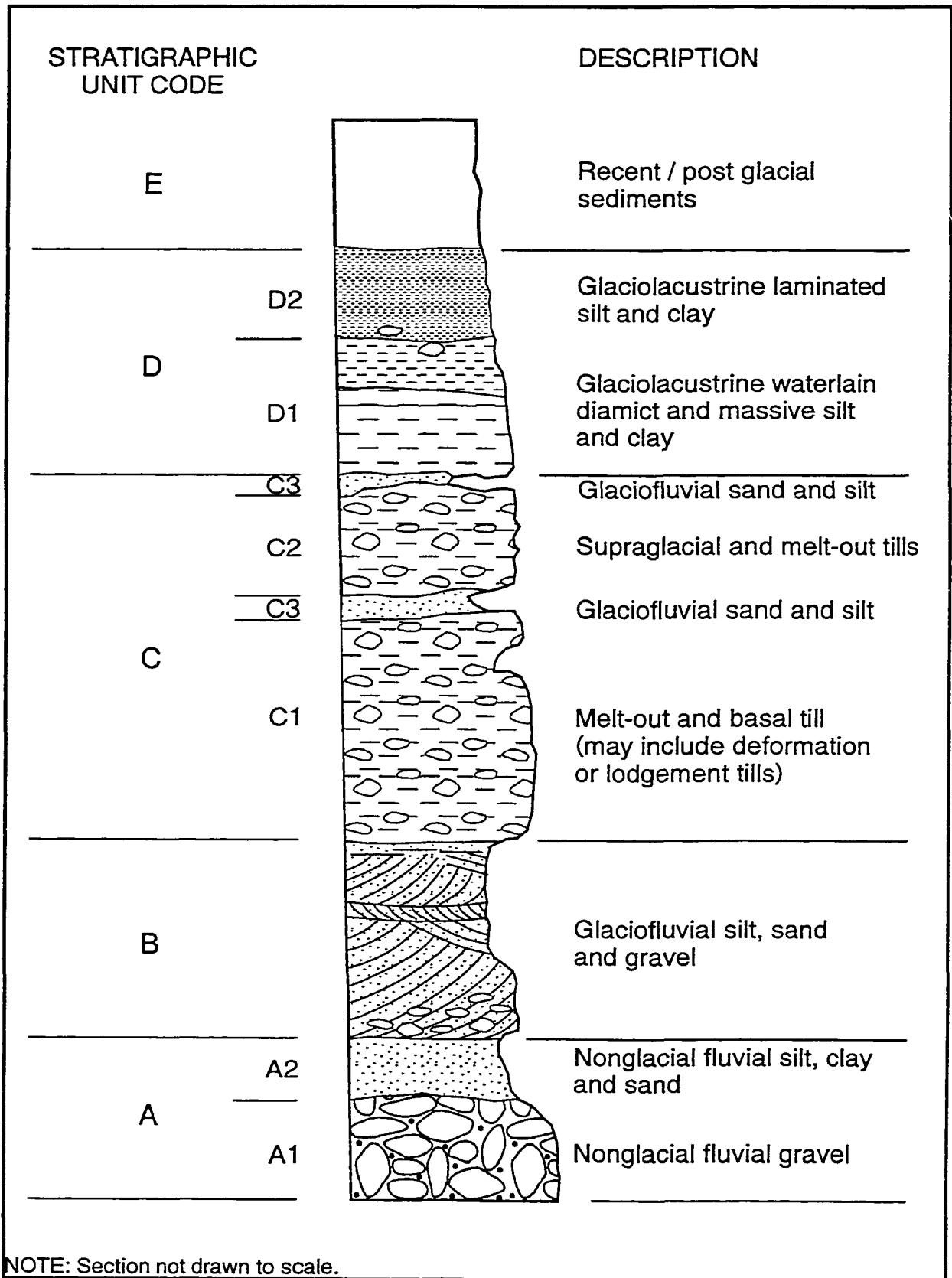
FIGURE 6.1 Composite stratigraphic section of study area.
