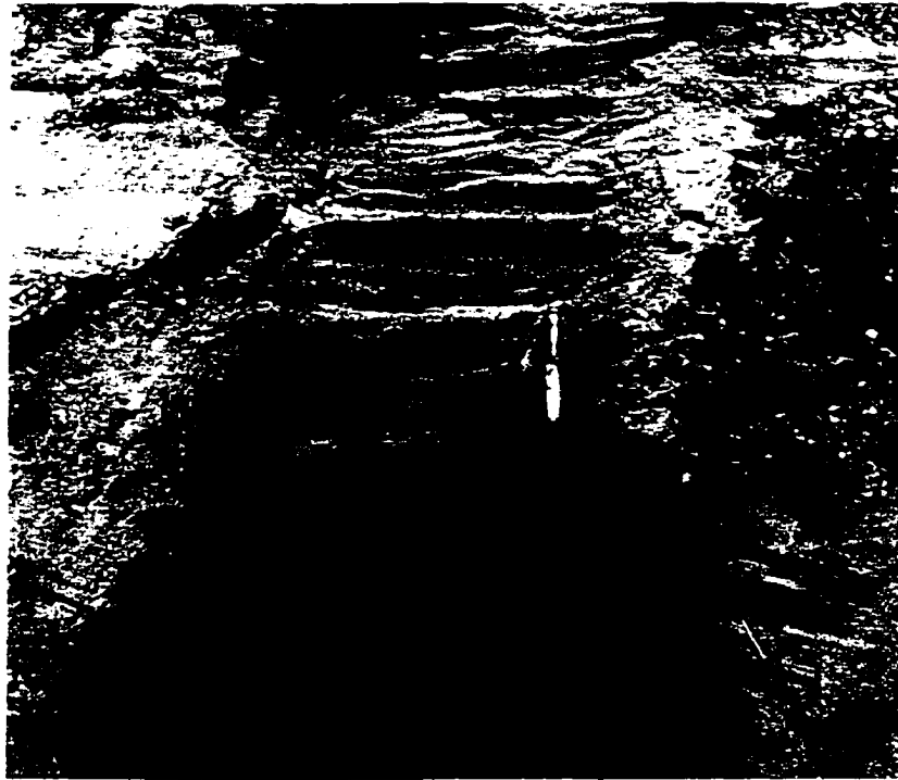
PLATE 6.3 - Mid-Wisconsinan fluvial sediments (sub-unit A-2) in the Watino section.
