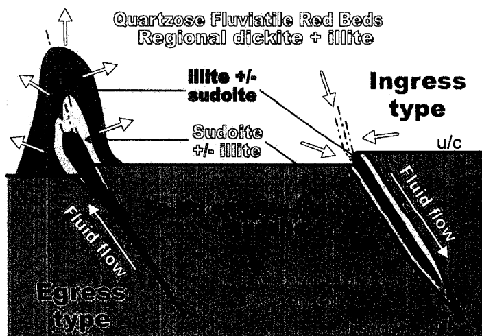
Figure 2-6. Ingress and egress type uranium deposits (Figure taken from Jefferson et al., 2007).
