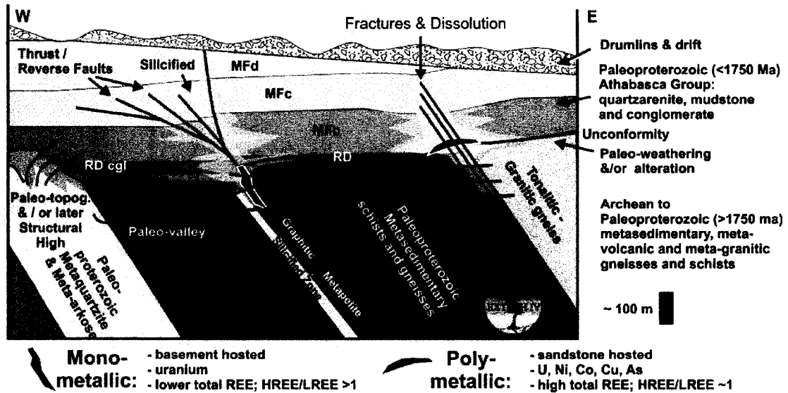
Figure 2-5. Monometallic and polymetallic type unconformity related uranium deposits in the Athabasca Basin (Figure taken from Jefferson et al., 2007).
