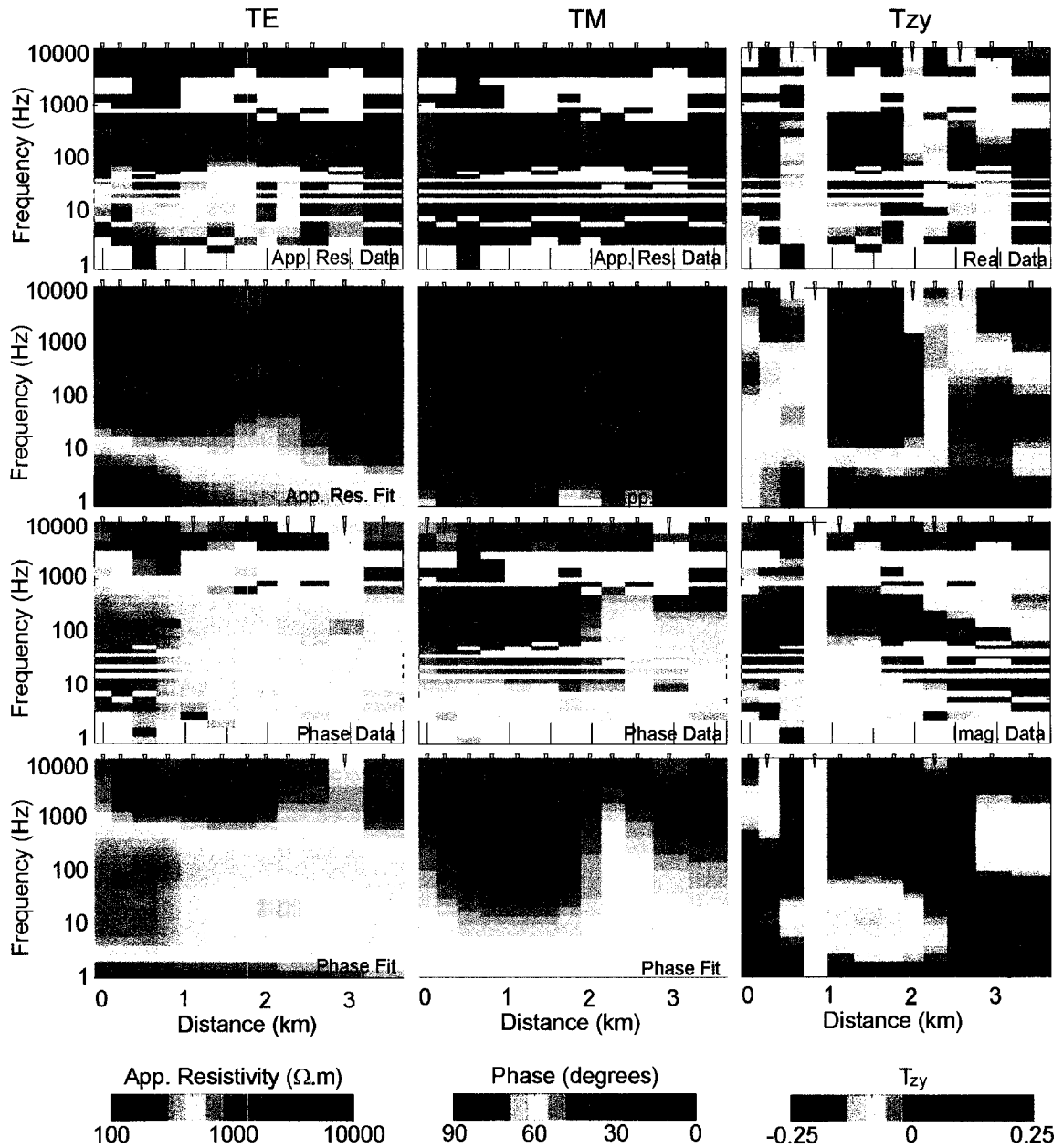
Figure A-6. Pseudosections of the measured data and fits of the 2D inversions for profile 266. Note that \alpha = 1 and \tau = 10 in the inversion.
