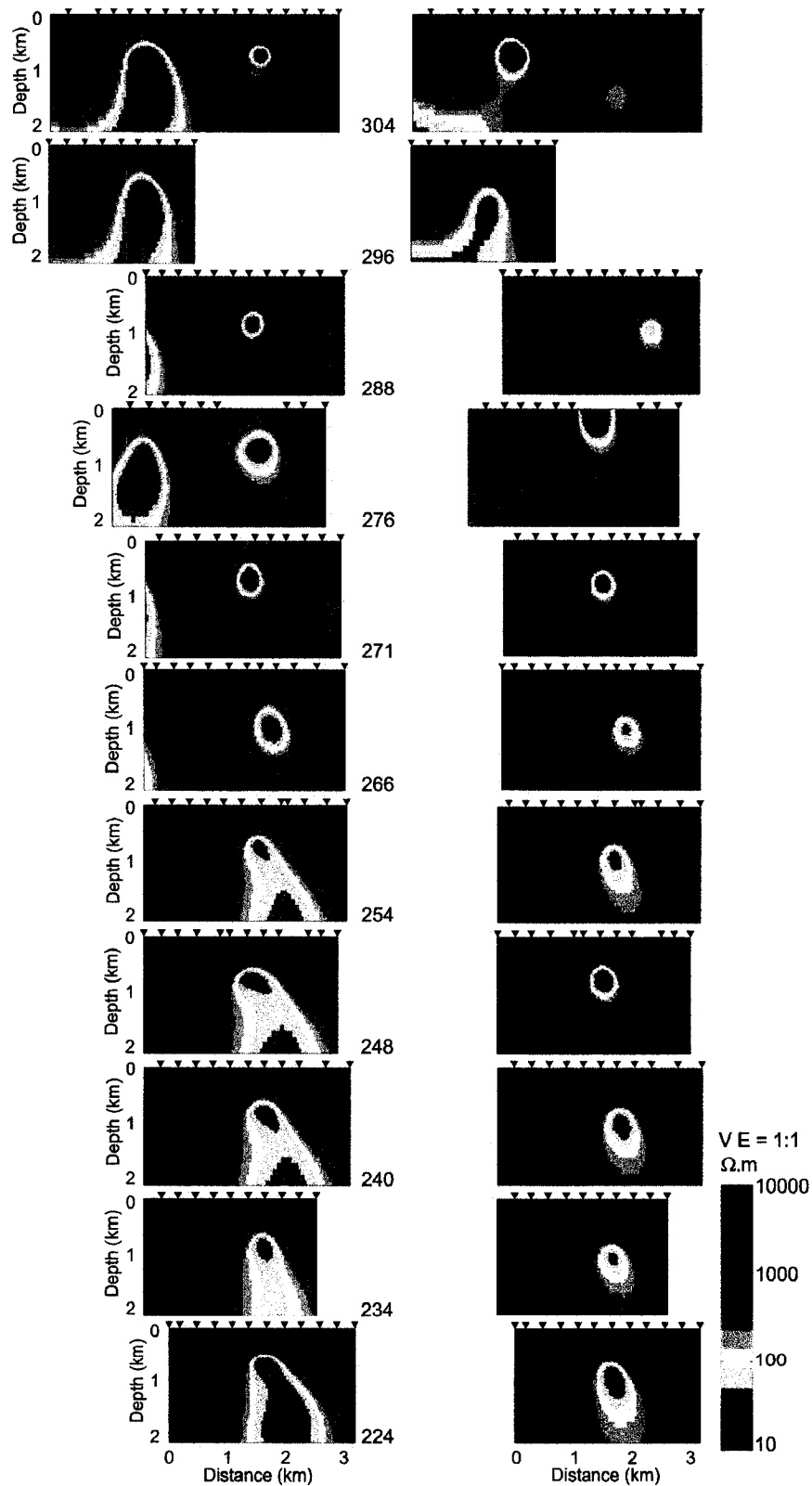
Figure 6-4. Resistivity models for all profiles derived with 2D inversions. Left column shows the TE-TM-T z inversions and the right column shows the TE-TM inversions (Figure is taken from Tuncer et al, 2006a).
