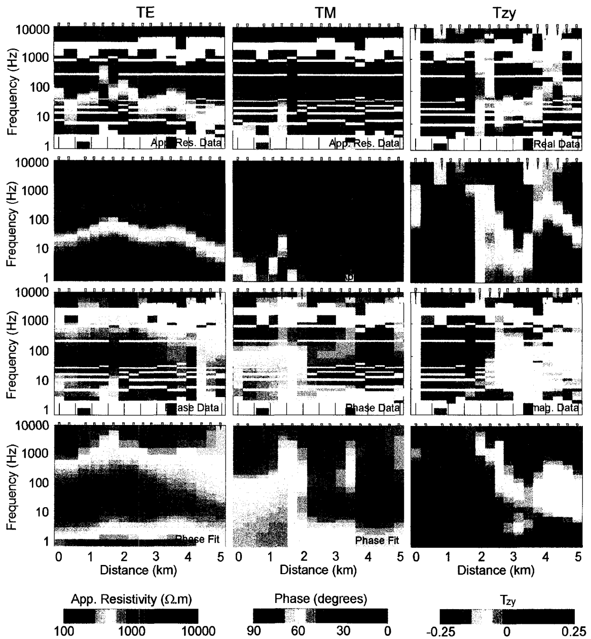
Figure A-11. Pseudosections of the measured data and fits of the 2D inversions for profile 304. Note that \alpha = 1 and \tau = 10 in the inversion.
