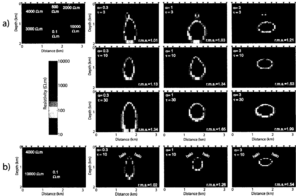
Figure 7-1. Synthetic inversion study showing the effect of different smoothing parameters. (a) This model represents the alteration chimney (500 \Omega.m ) beneath a 25 m thick, 2000 \Omega.m resistive overburden and shows a resistivity contrast across the fault with different smoothing parameters. (b) This model shows a basic two-layer model with a graphitic conductor that has an artificial resistive halo around the conductor.
