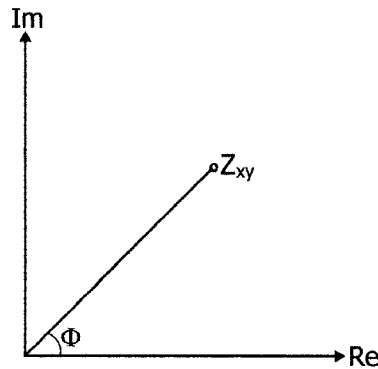
Figure 4-3. The definition of phase in an Argand diagram.
