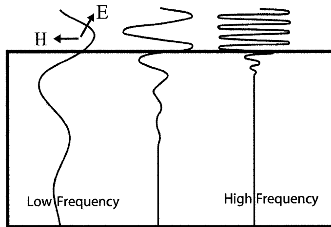
Figure 4-2. Physics of electromagnetic waves in a halfspace (Figure is modified from http://www-geo.phys.ualberta.ca/~unsworth/MT/MT.html ). High frequencies penetrate to the shallow depths where low frequencies penetrate to the deeper parts of the earth.
