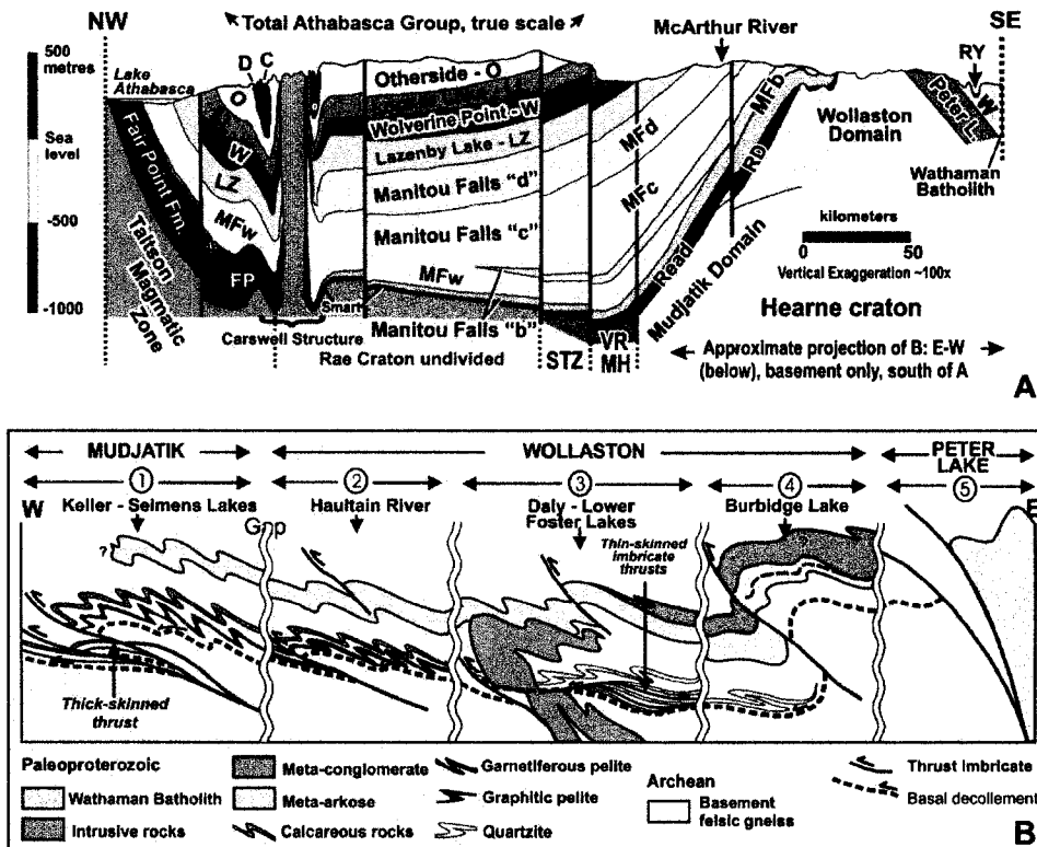
Figure 2-2. A) Lithostatigraphic cross section of the Athabasca basin. B) Structural cross section of the Athabasca basin that illustrates structural geometry of the Wollaston – Mudjatik transition zone (Figure taken from Jefferson et al., 2007).
