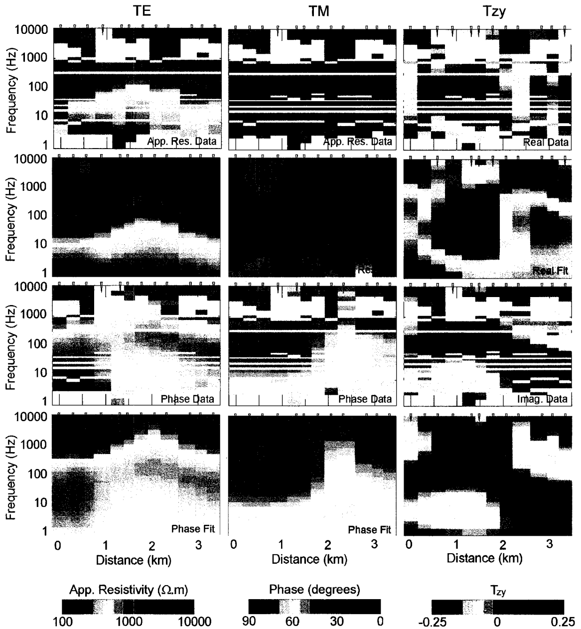
Figure A-4. Pseudosections of the measured data and fits of the 2D inversions for profile 248. Note that \alpha = 1 and \tau = 10 in the inversion.
