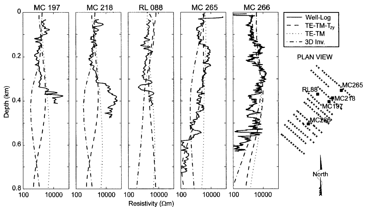
Figure 6-13. Comparison of borehole-log resistivity data (from Mwenifumbo et al., 2004) and the of 2D and 3D joint inversion models (Figure is modified from Tuncer et al., 2006a). A 7-point moving average filter was applied to the resistivity log data to allow a more objective comparison of the two measures of subsurface resistivity.
