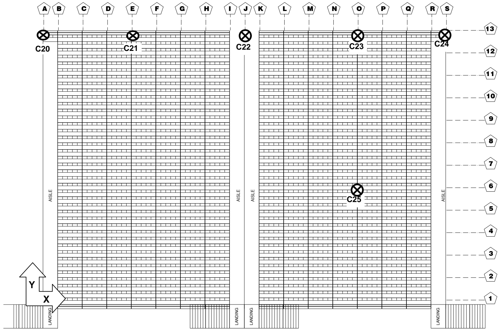
Figure 3.16. Location of cable transducers measuring vertical displacement on plan view of grandstand
