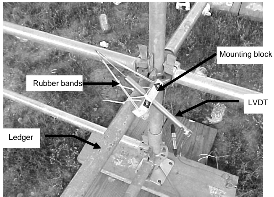
Figure 3.11. LVDT attachment on the ledger near the base of the structure
