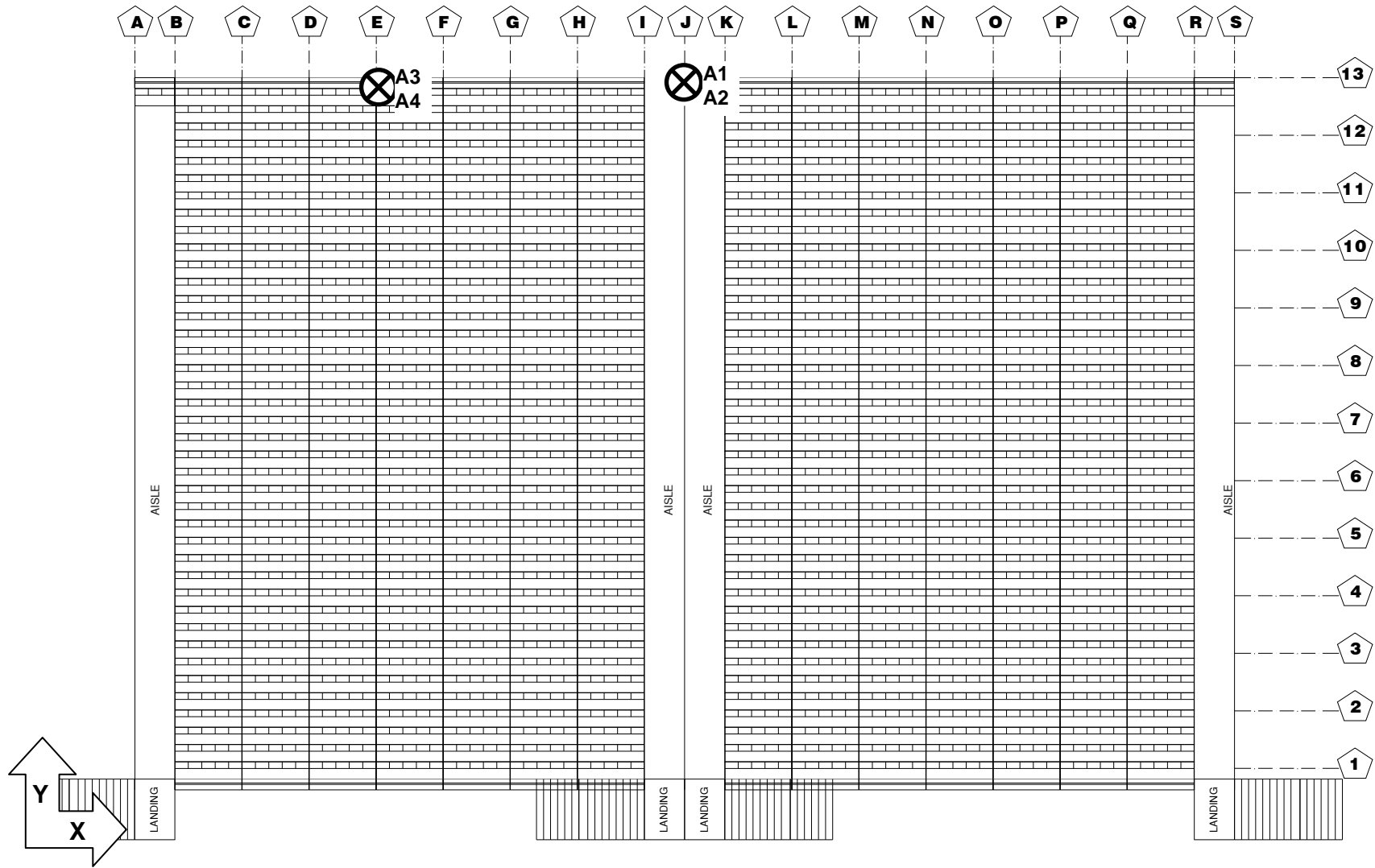
Figure A.8. Location of accelerometers on plan view of grandstand
