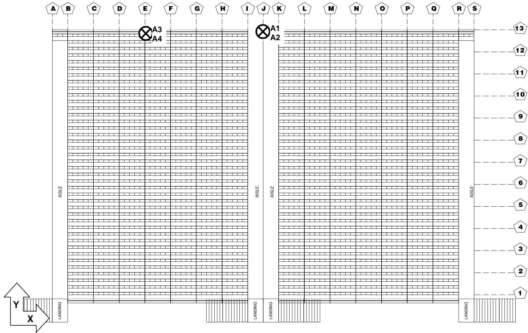
Figure 3.18. Location of accelerometers on plan view of grandstand
