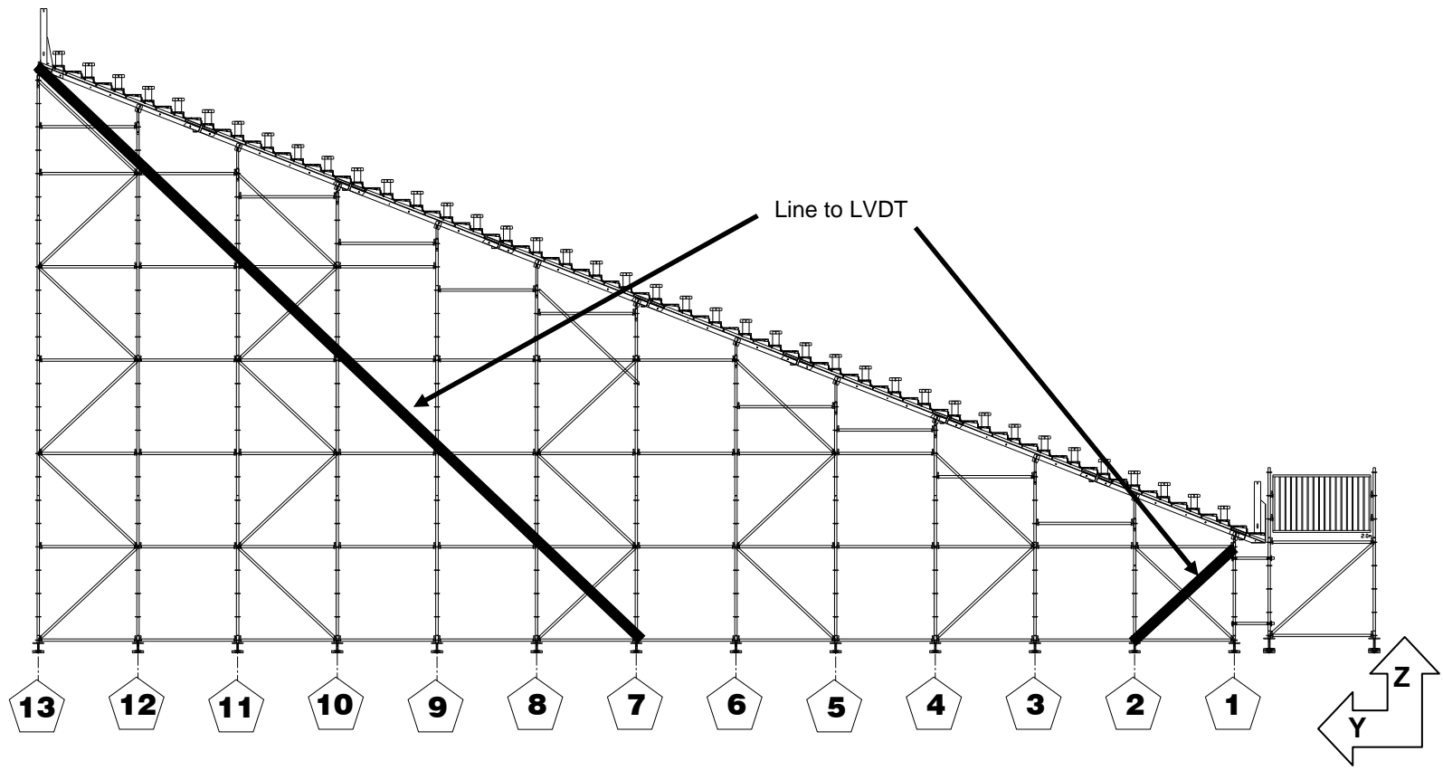
Figure A.3. Side cross section showing line to LVDT to measure front-back sway motion
