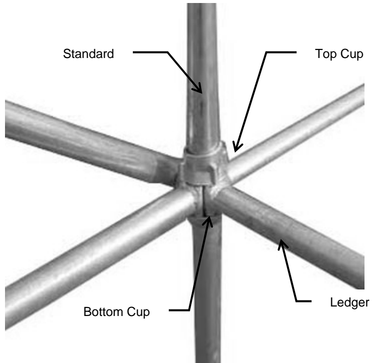
Figure 2.4 Connection for Cuplock scaffold
