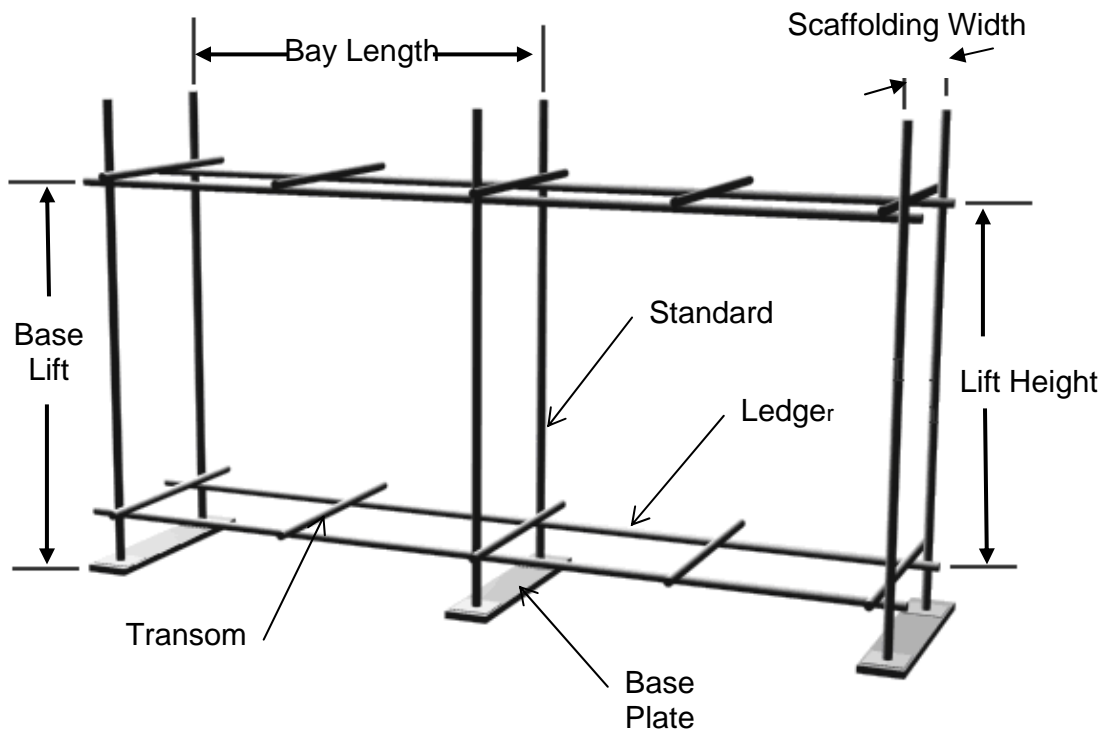
Figure 2.1 Scaffold bays
