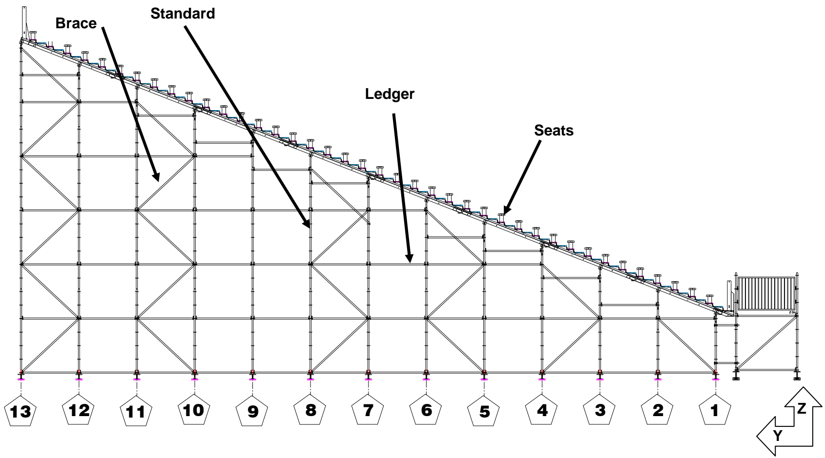
Figure 3.5. Typical cross section of temporary grandstand
