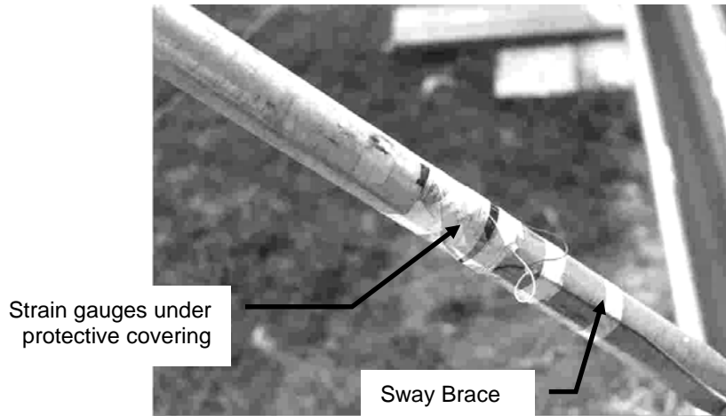
Figure 3.9. Strain gauges mounted on brace
