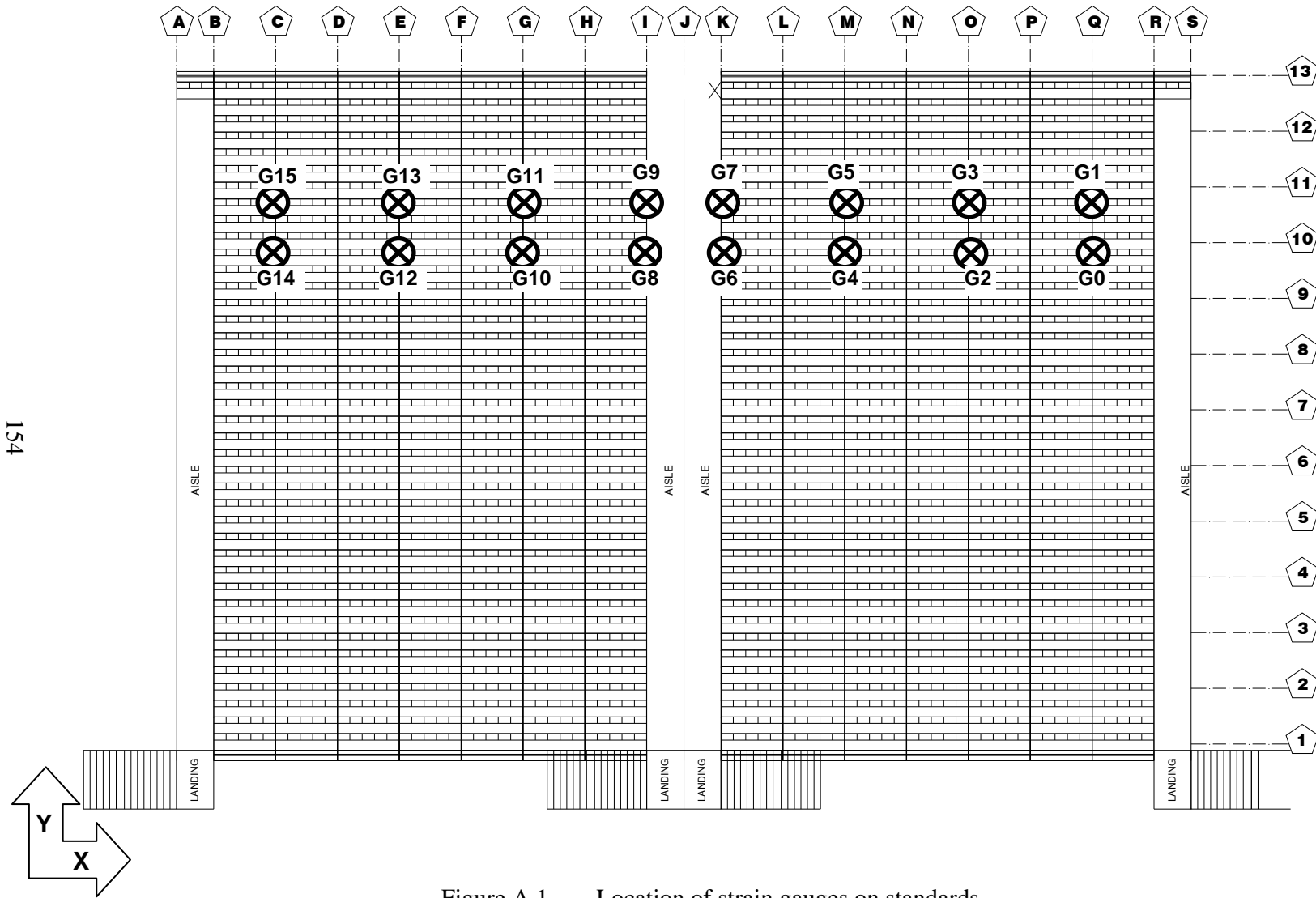
Figure A.1. Location of strain gauges on standards
