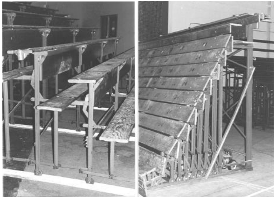
Figure 2.9 Accordion bleacher
