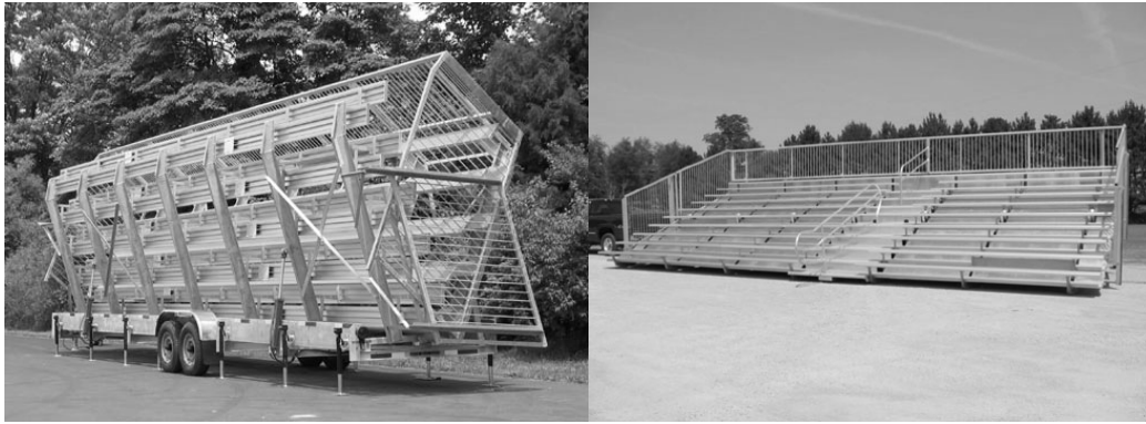
Figure 2.8 Folding bleacher
