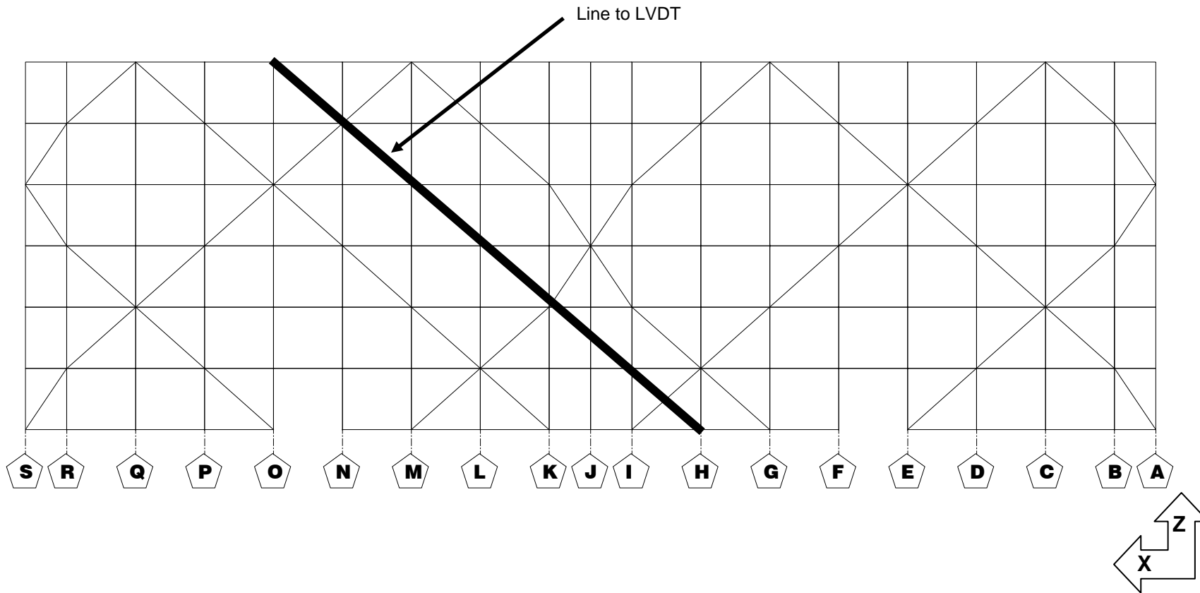
Figure A.4. Rear cross section showing line to LVDT to measure side-side sway
