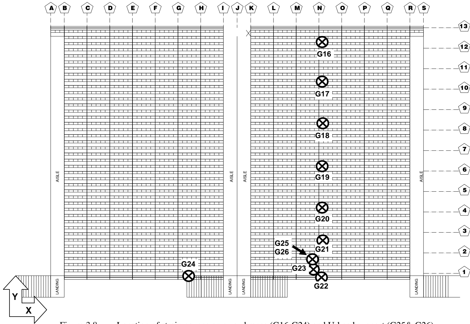
Figure 3.8. Location of strain gauges on sway braces (G16-G24) and U-head support (G25& G26)
