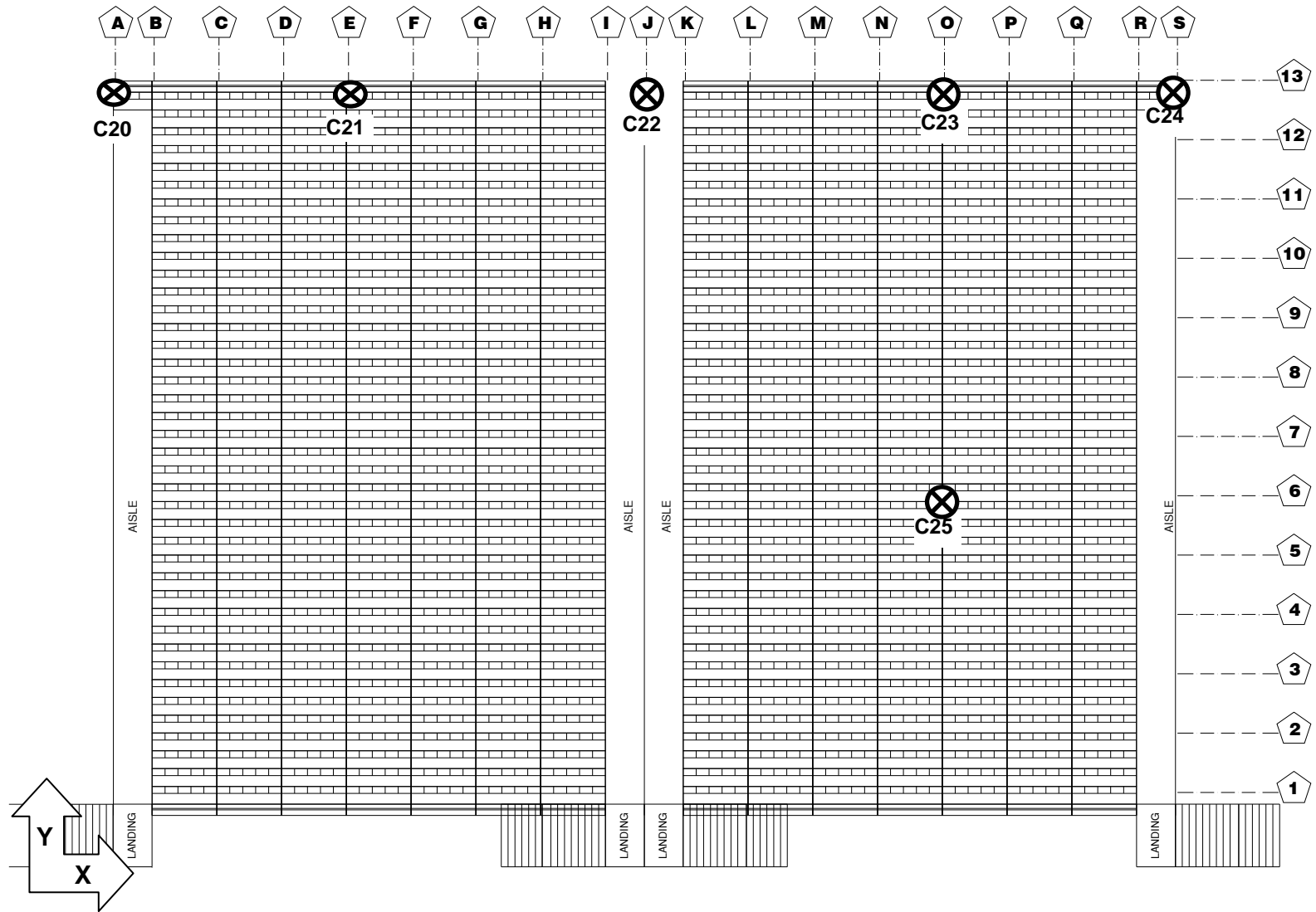
Figure A.7. Location of cable transducers measuring vertical displacement on plan view of grandstand
