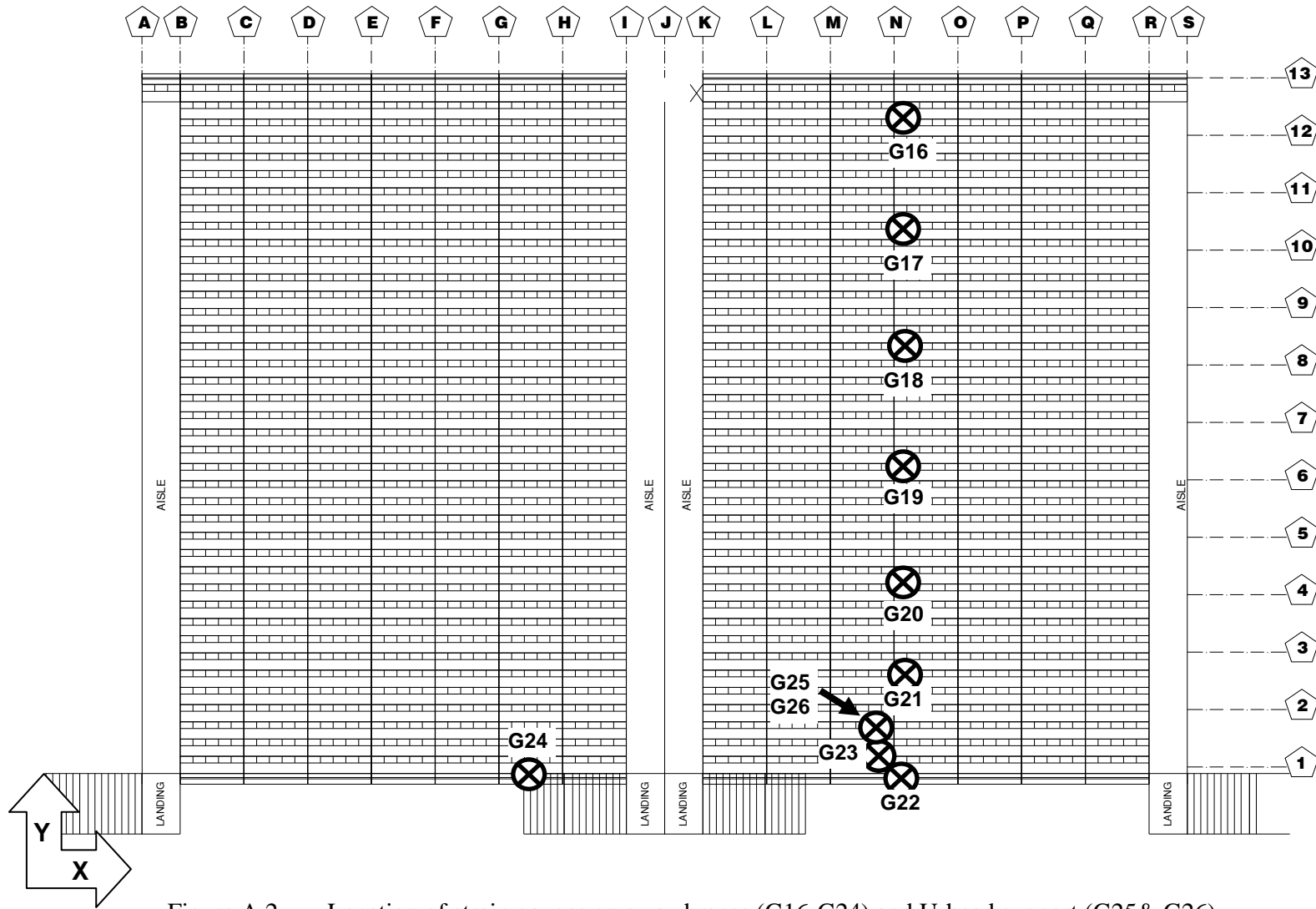
Figure A.2. Location of strain gauges on sway braces (G16-G24) and U-head support (G25& G26)
