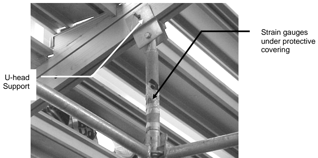
Figure 3.10. Strain gauges mounted on U-head post
