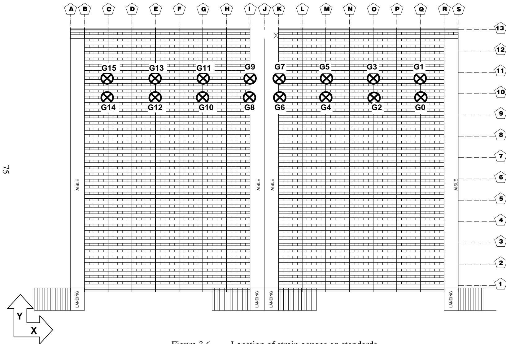
Figure 3.6. Location of strain gauges on standards
