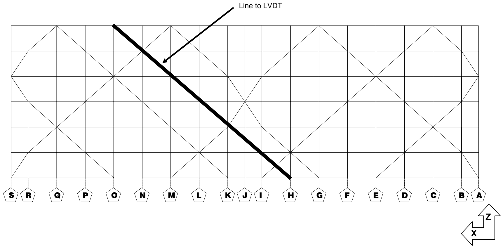
Figure 3.13. Rear cross section showing line to LVDT to measure side-side sway
