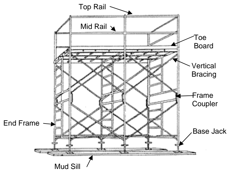
Figure 2.2 Frame scaffolding
