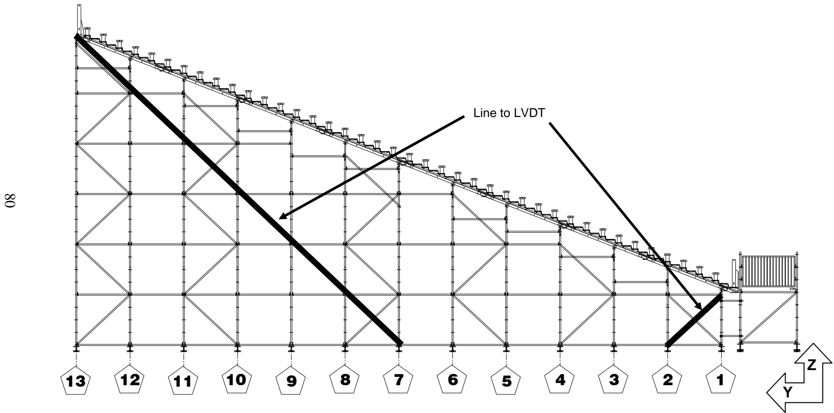
Figure 3.12. Side cross section showing line to LVDT to measure front-back sway motion
