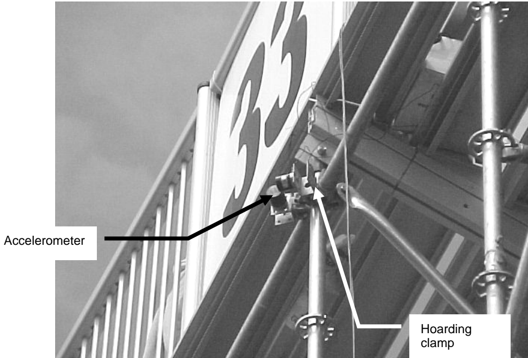
Figure 3.19. Accelerometers
