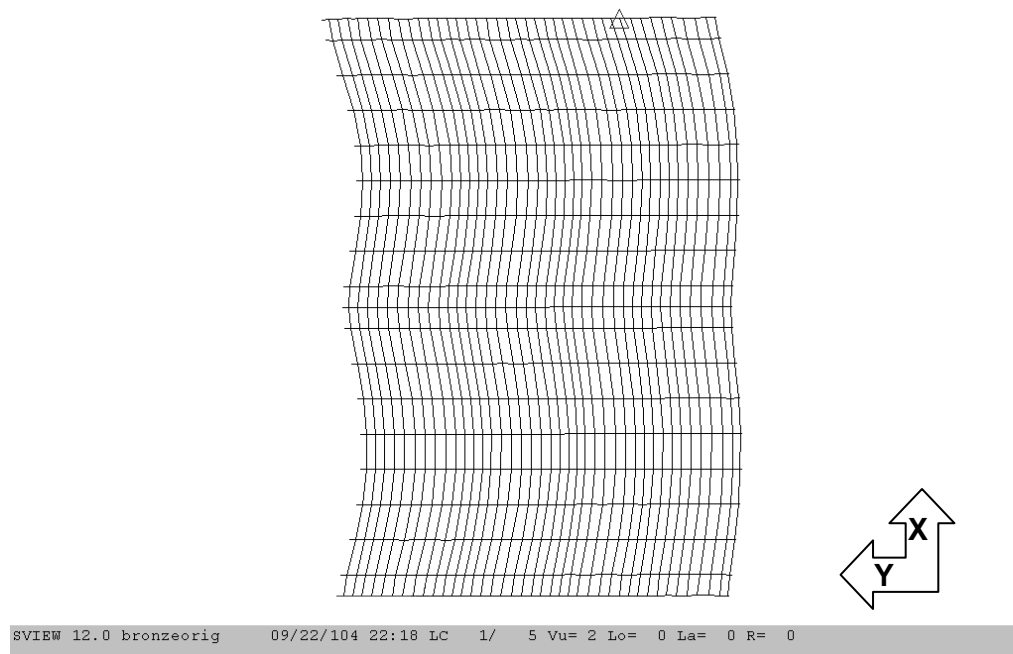
Figure 5.3. Preliminary FEA model, first mode shape
