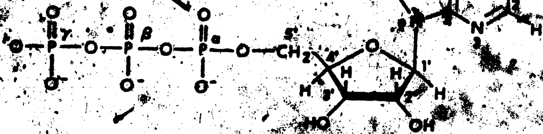
Adenosine 5' - Triphosphate - ATP
