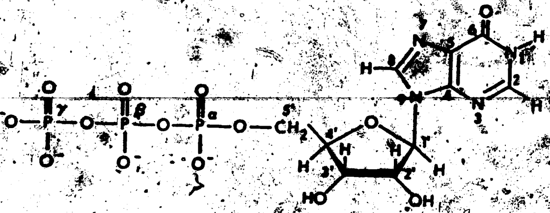
Inosine 5' - Triphosphate - ITP
