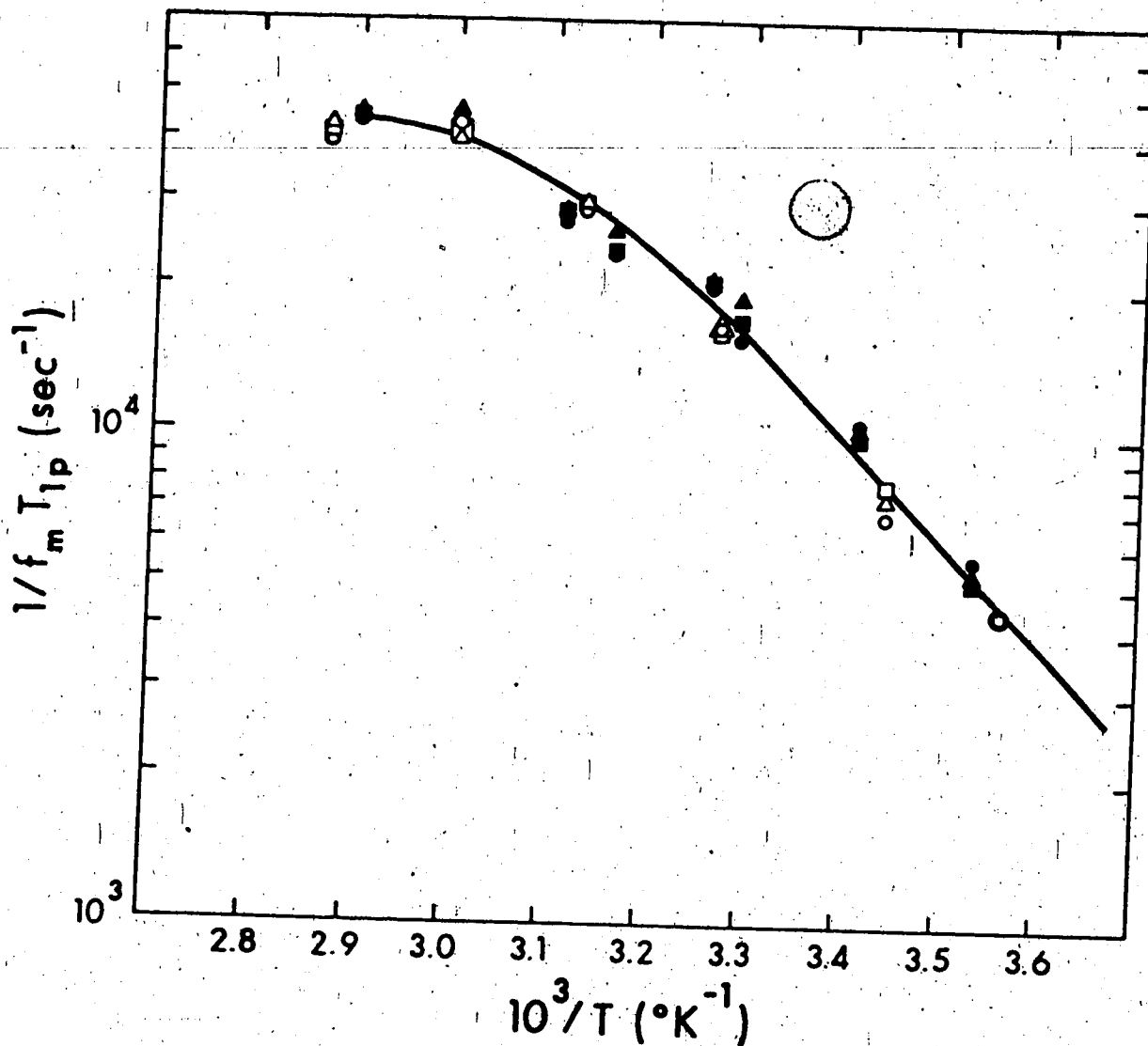
FIGURE 7: Temperature dependence of the ^{31}P paramagnetic longitudinal relaxation times for Gd(III)-ITP (see Table IV).
