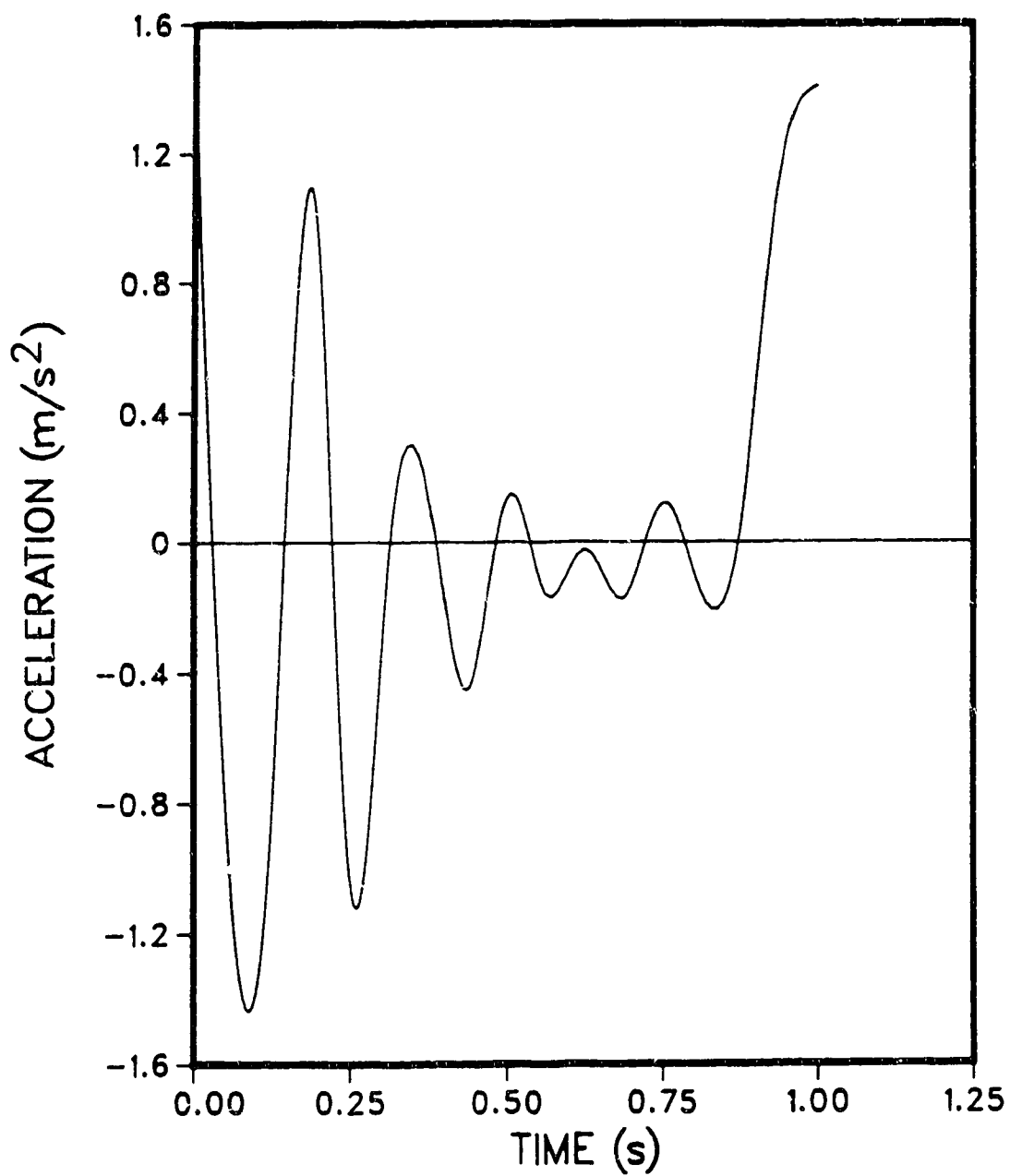
Figure 4.10 Acceleration Response - Loaded Side
