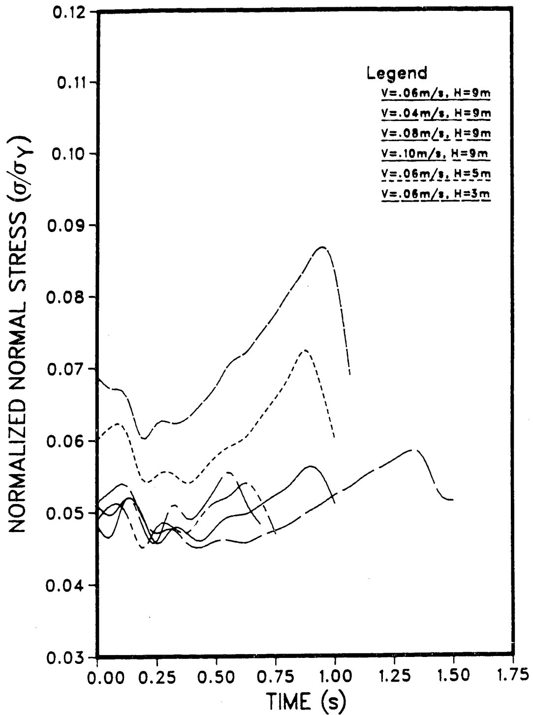
Figure 5.17 Normalized Normal Stress - Stiffener
