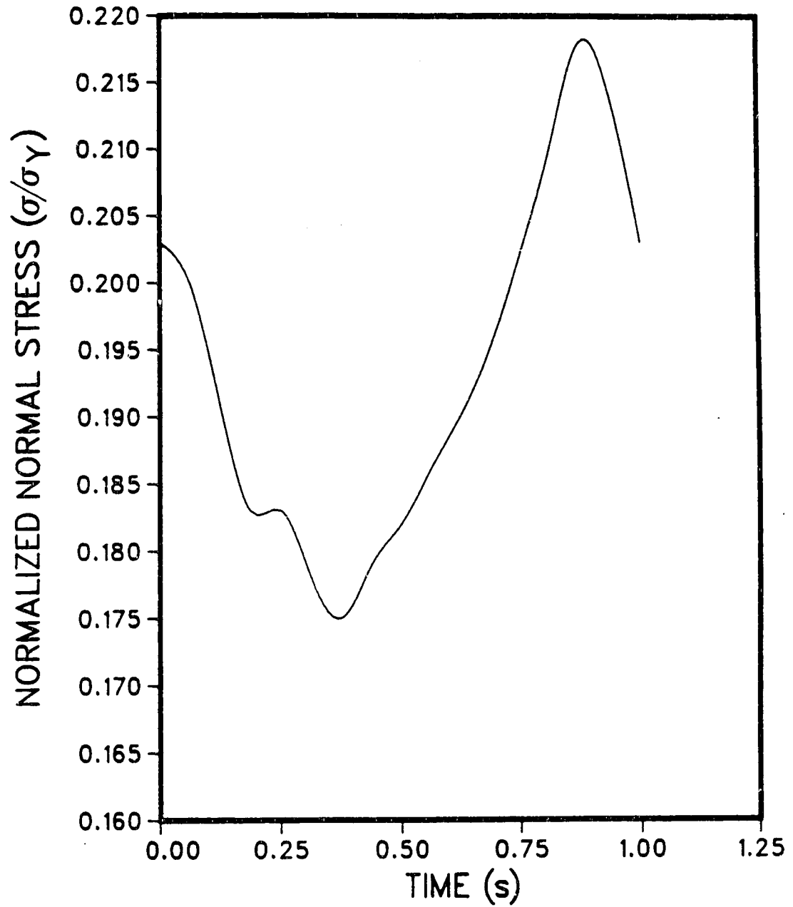
Figure 4.18 Normalized Normal Stress - Bulkhead
