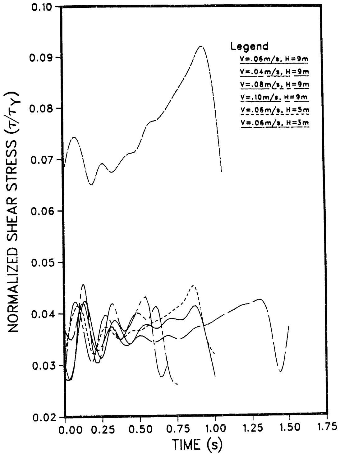
Figure 5.24 Normalized Shear Stress - Bulkhead
