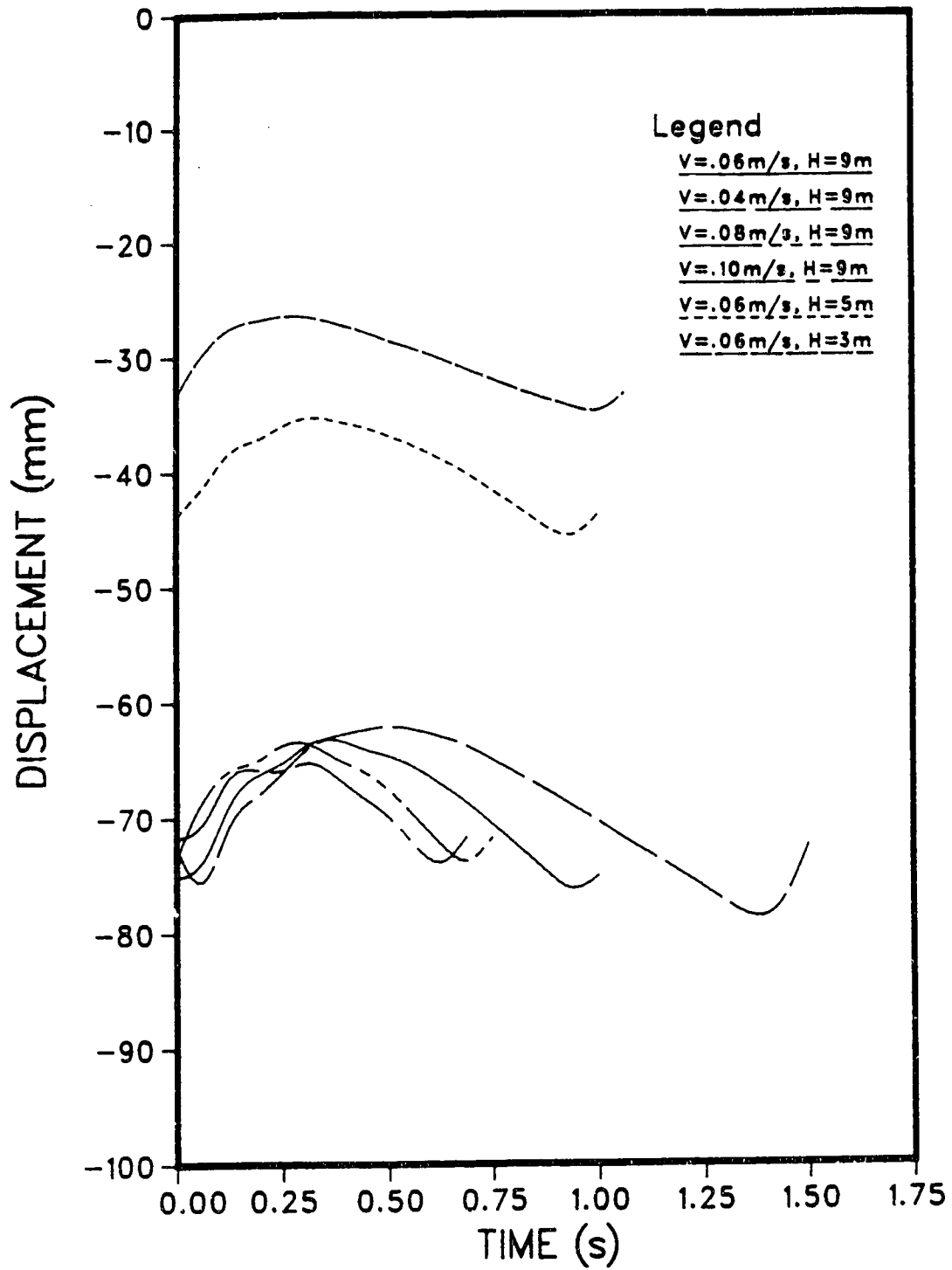
Figure 5.10 Displacement Response - Loaded Side
