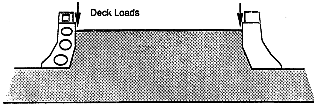
Step 1, Static Vertical Loads
