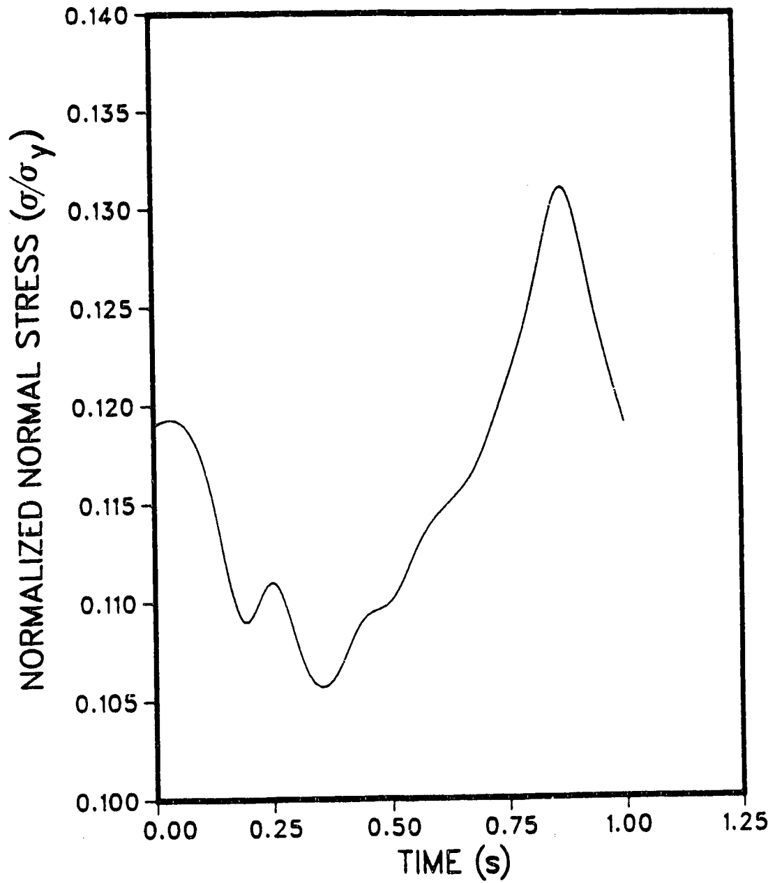
Figure 4.12 Normalized Normal Stress - Stiffener
