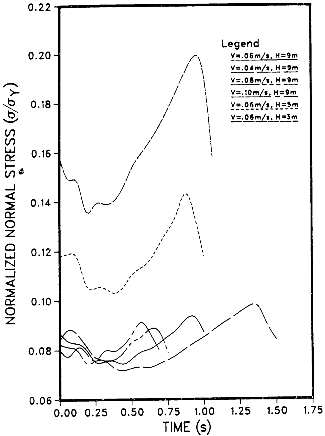
Figure 5.19 Normalized Normal Stress - Intermediate Frame
