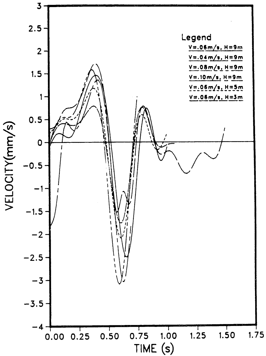
Figure 5.13 Velocity Response - Unloaded Side
