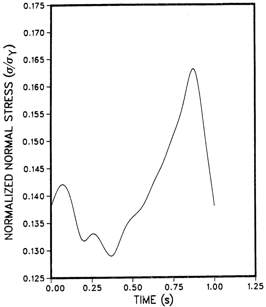
Figure 4.17 Normalized Shear Stress - Horizontal Frame
