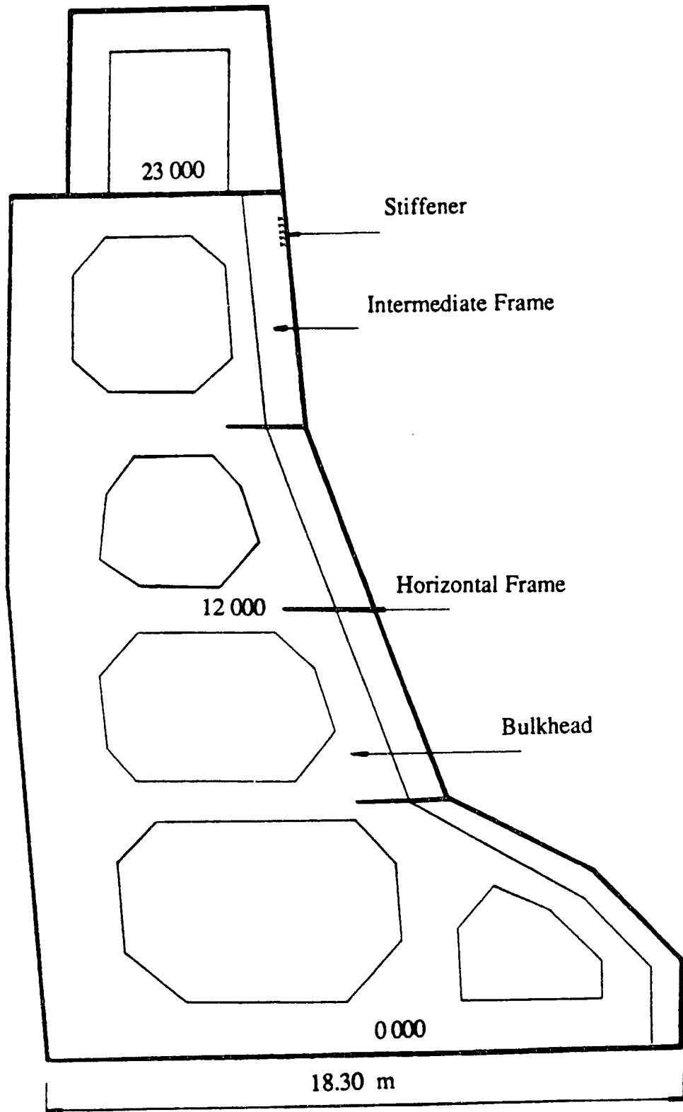
Figure 3.2 Structural Arrangement of The Caisson
