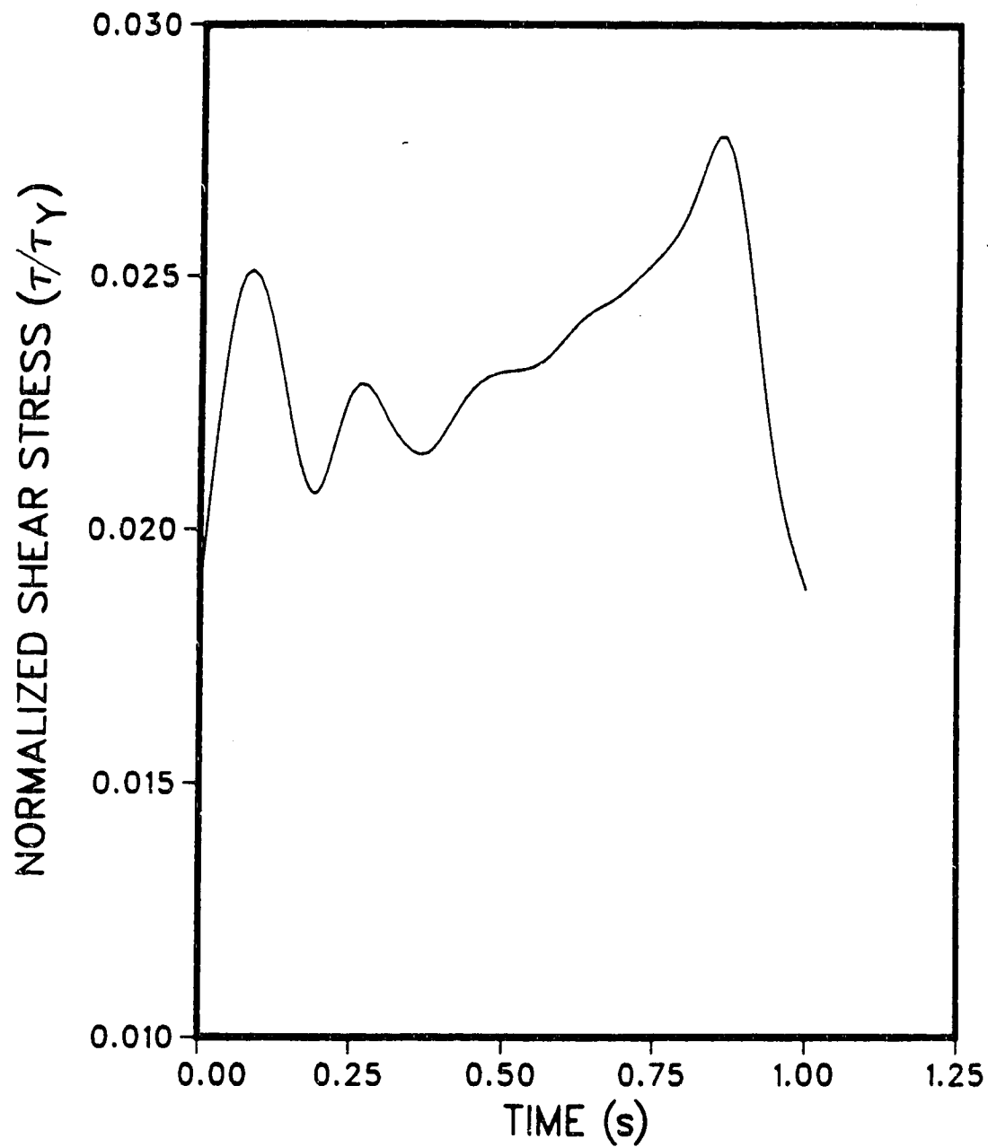
Figure 4.15 Normalized Shear Stress - Intermediate Frame
