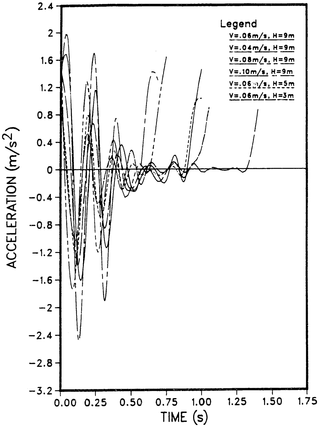
Figure 5.14 Acceleration Response - Loaded Side
