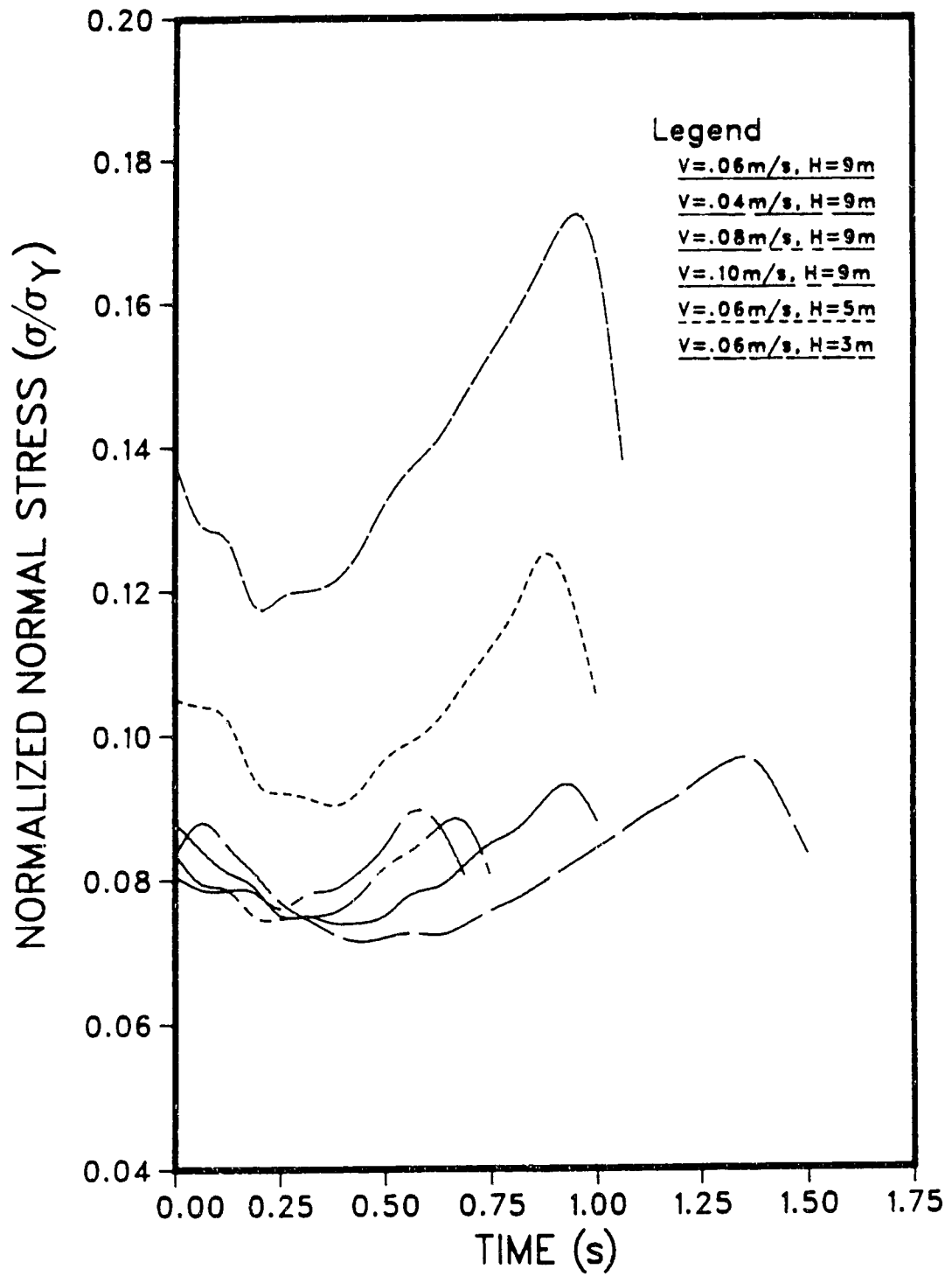
Figure 5.23 Normalized Normal Stress - Bulkhead
