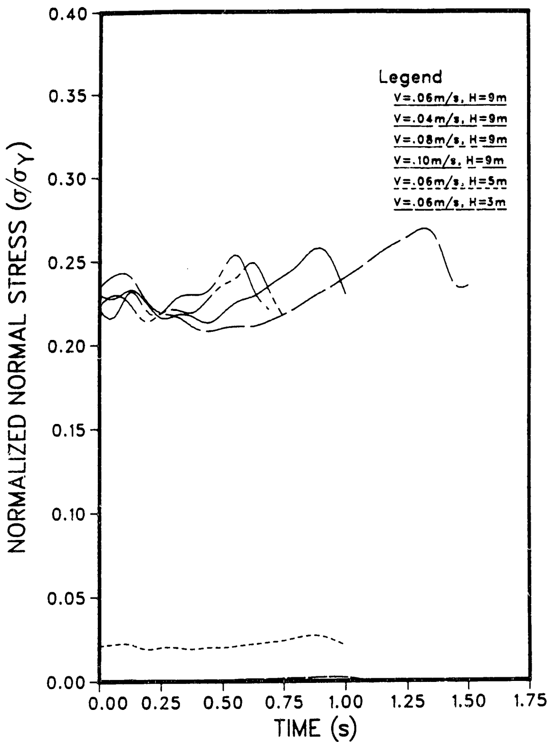
Figure 5.21 Normalized Normal Stress - Horizontal Frame
