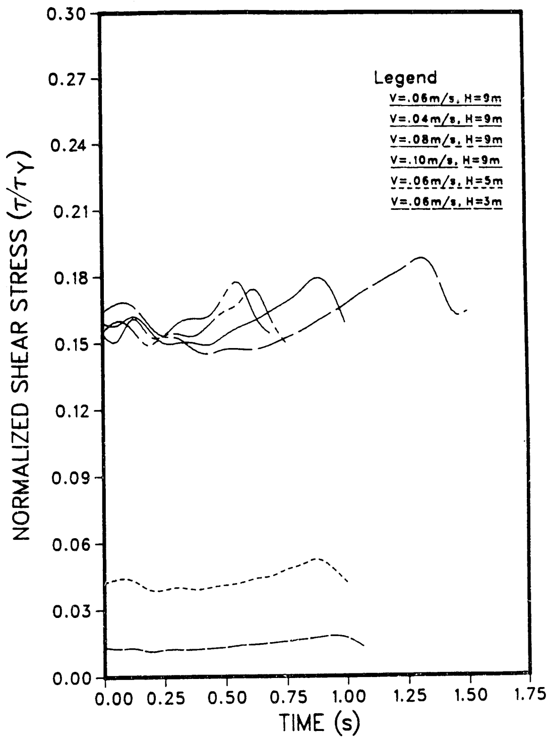
Figure 5.22 Normalized Shear Stress - Horizontal Frame
