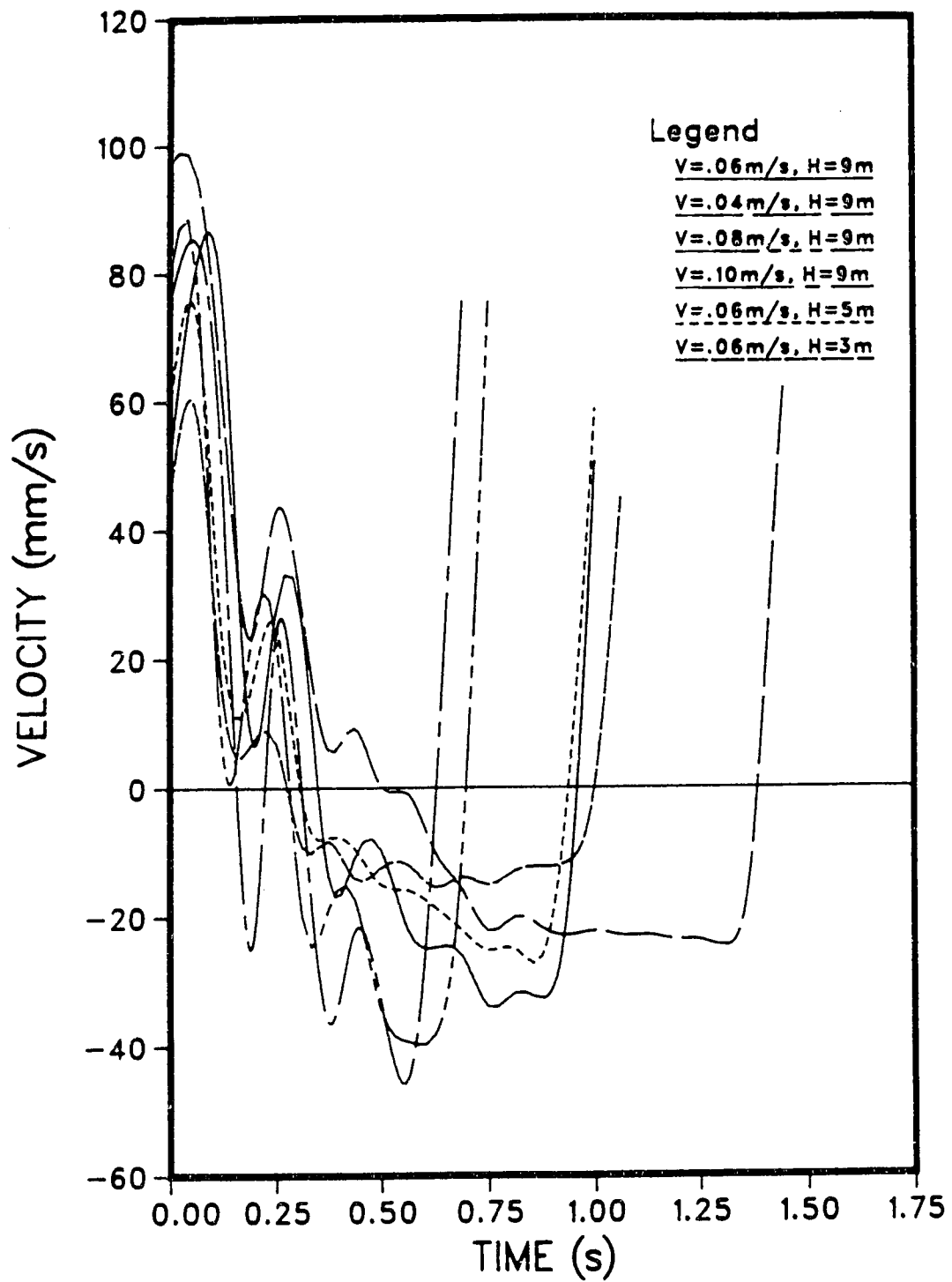
Figure 5.12 Velocity Response - Loaded Side
