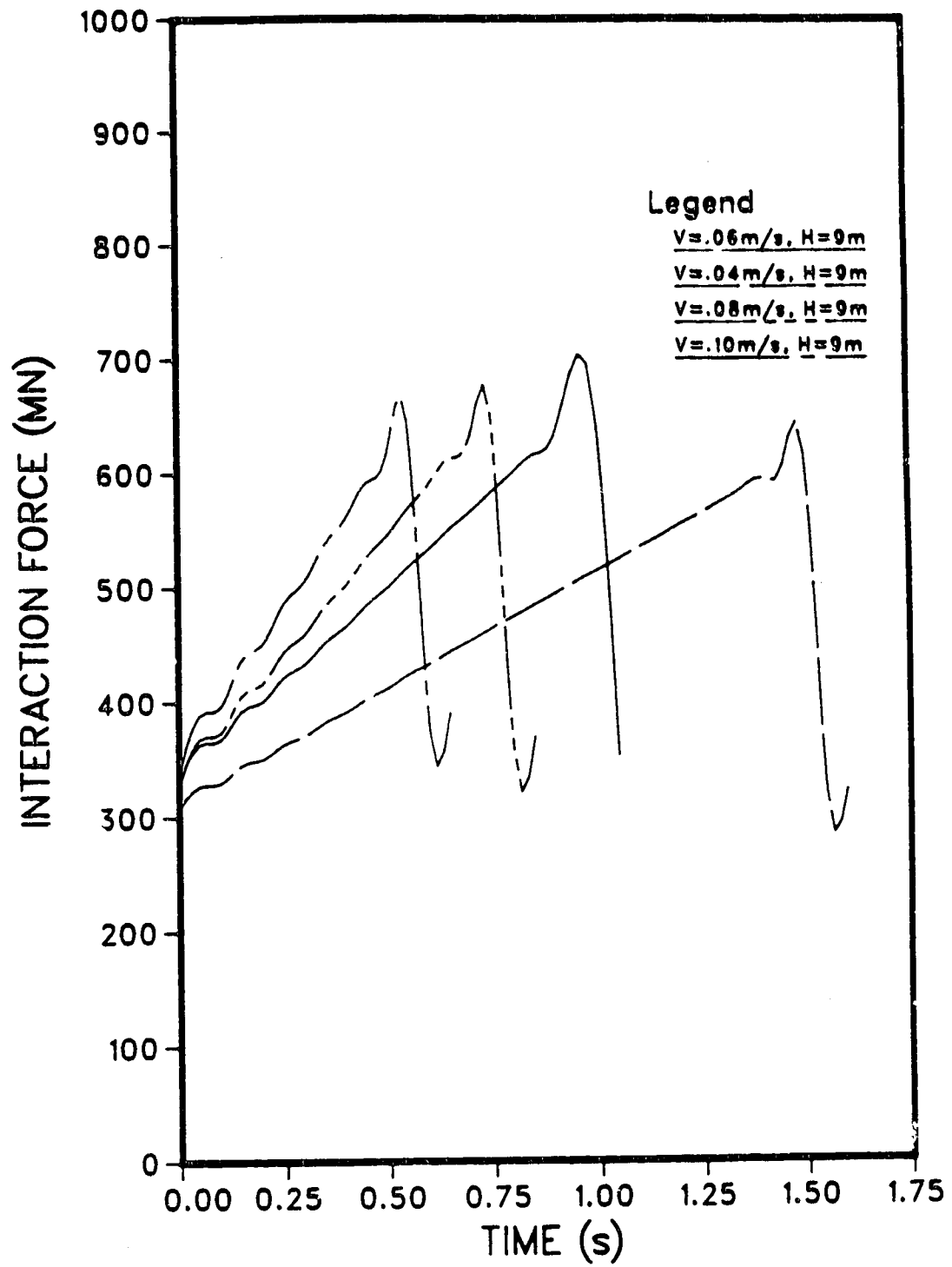
Figure 6.7 Interaction Force from Viscoelastic Model
