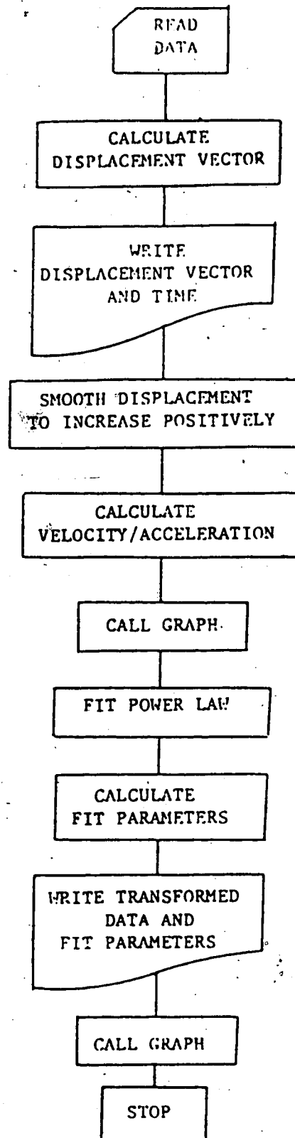
Figure 5.7 Power Law(velocity/acceleration) flow diagram
