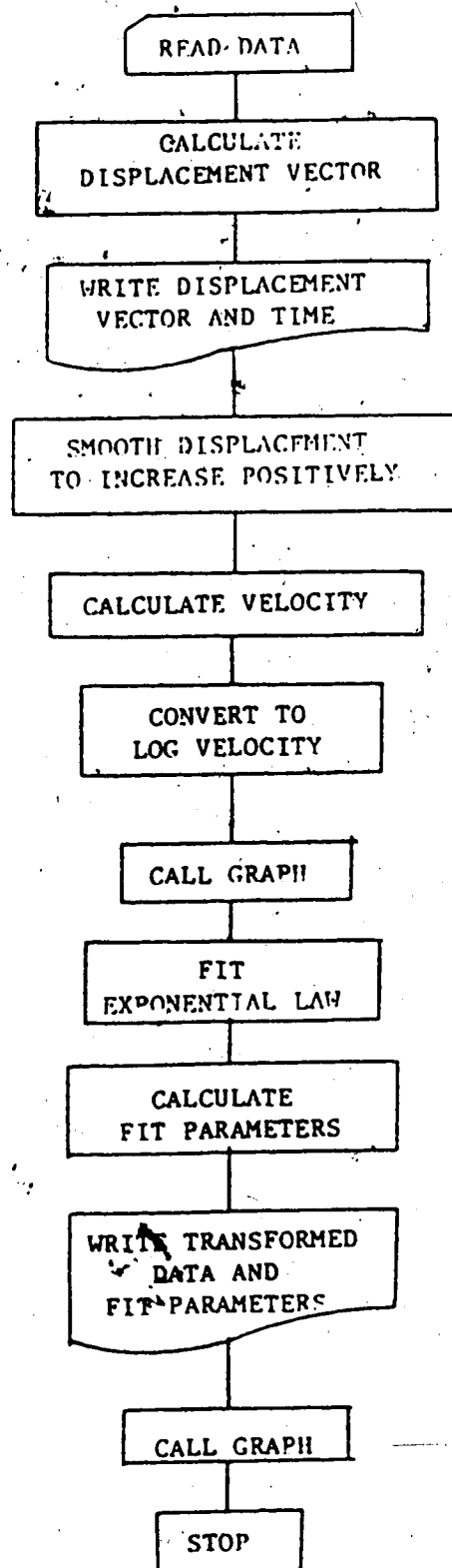
Figure 5.8 Exponential law flow diagram
