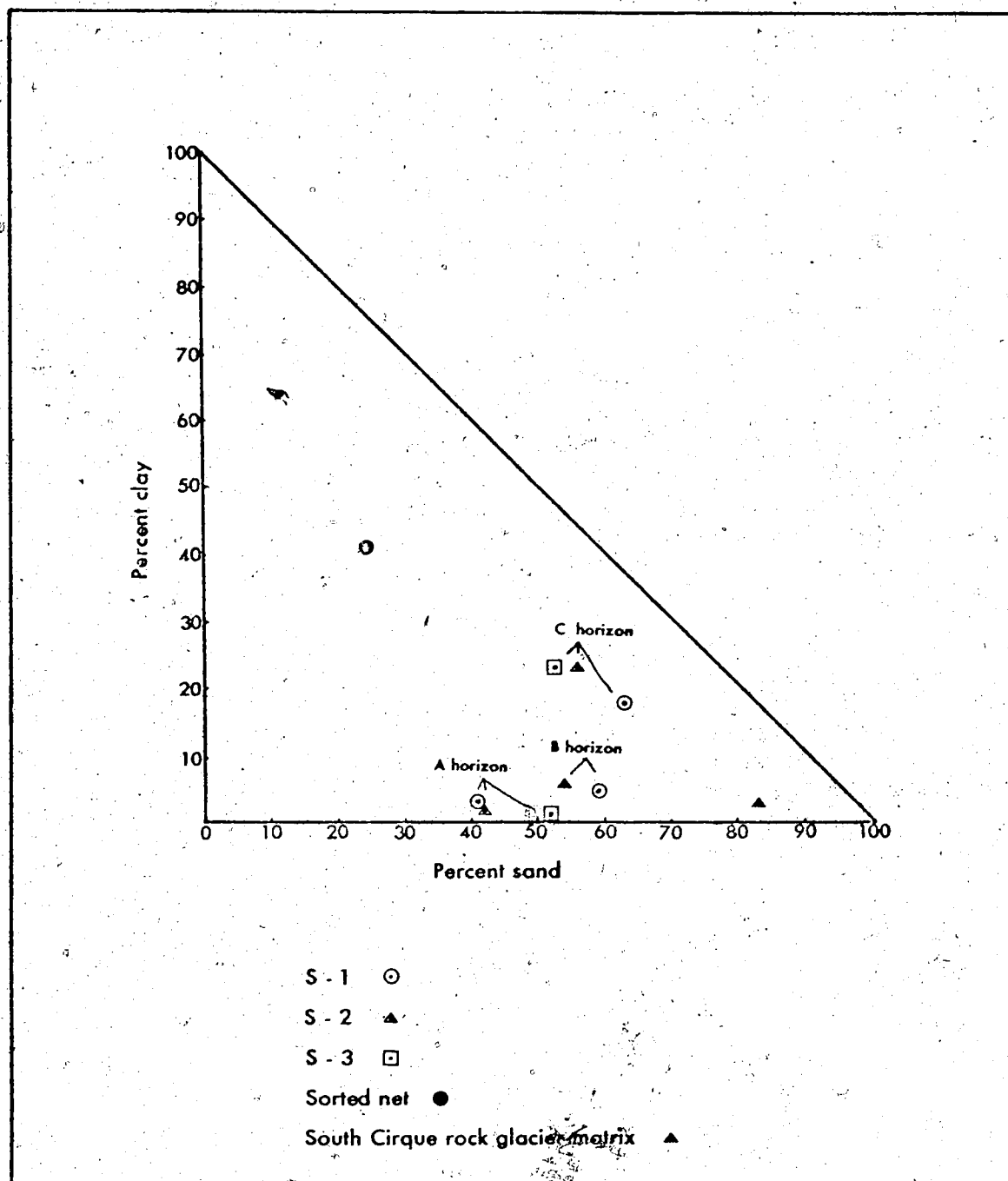
FIGURE 5.6 Textural classification of the soils.
