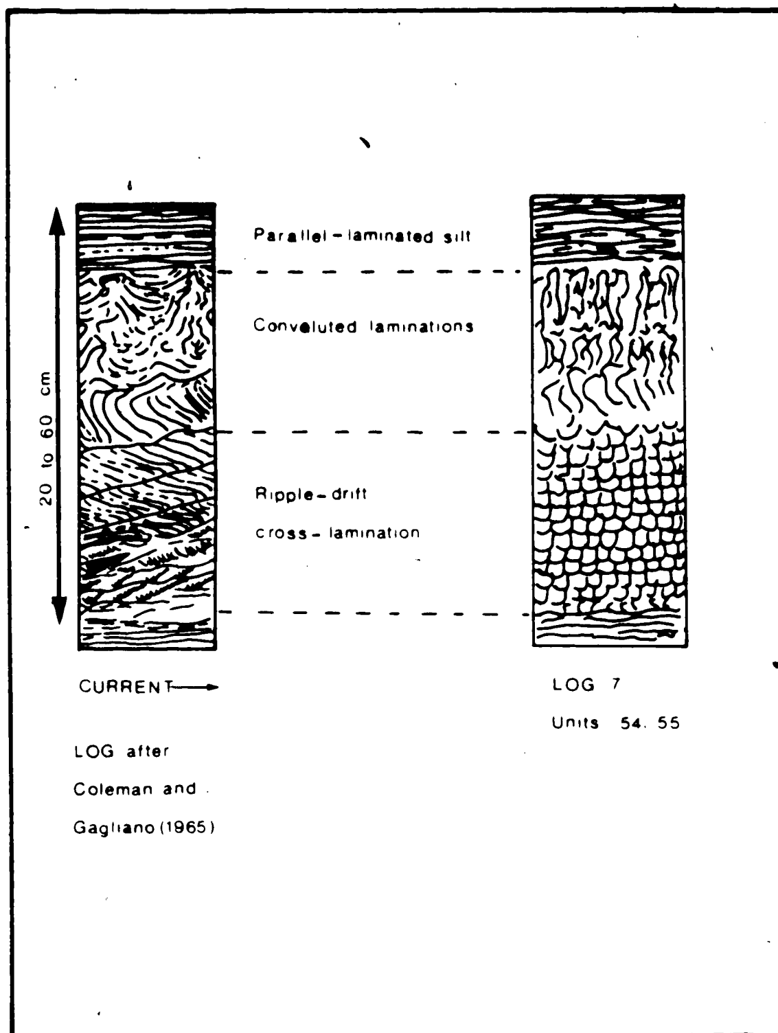
Figure 5 - 2 Comparison between convolute lamination sequences found in fluvial and lacustrine environments.
