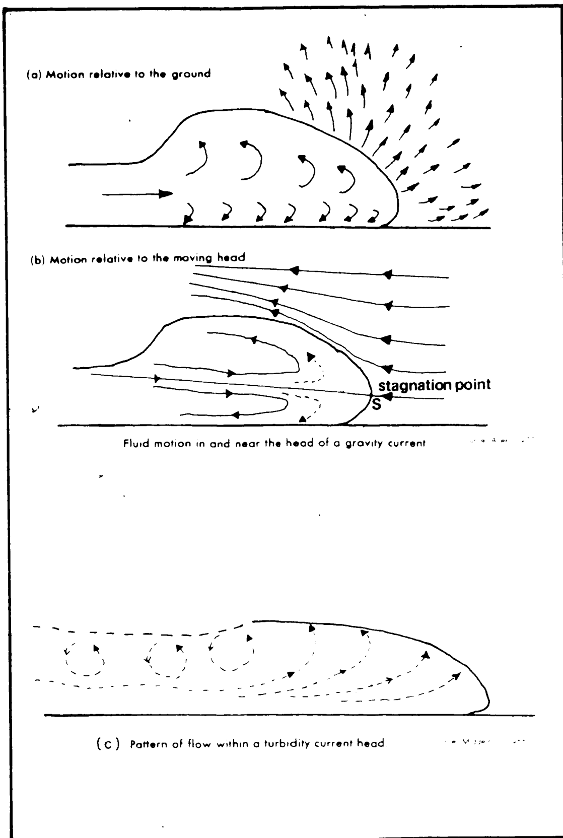
Figure 2-1 Showing fluid motion outside and within an underflow.
