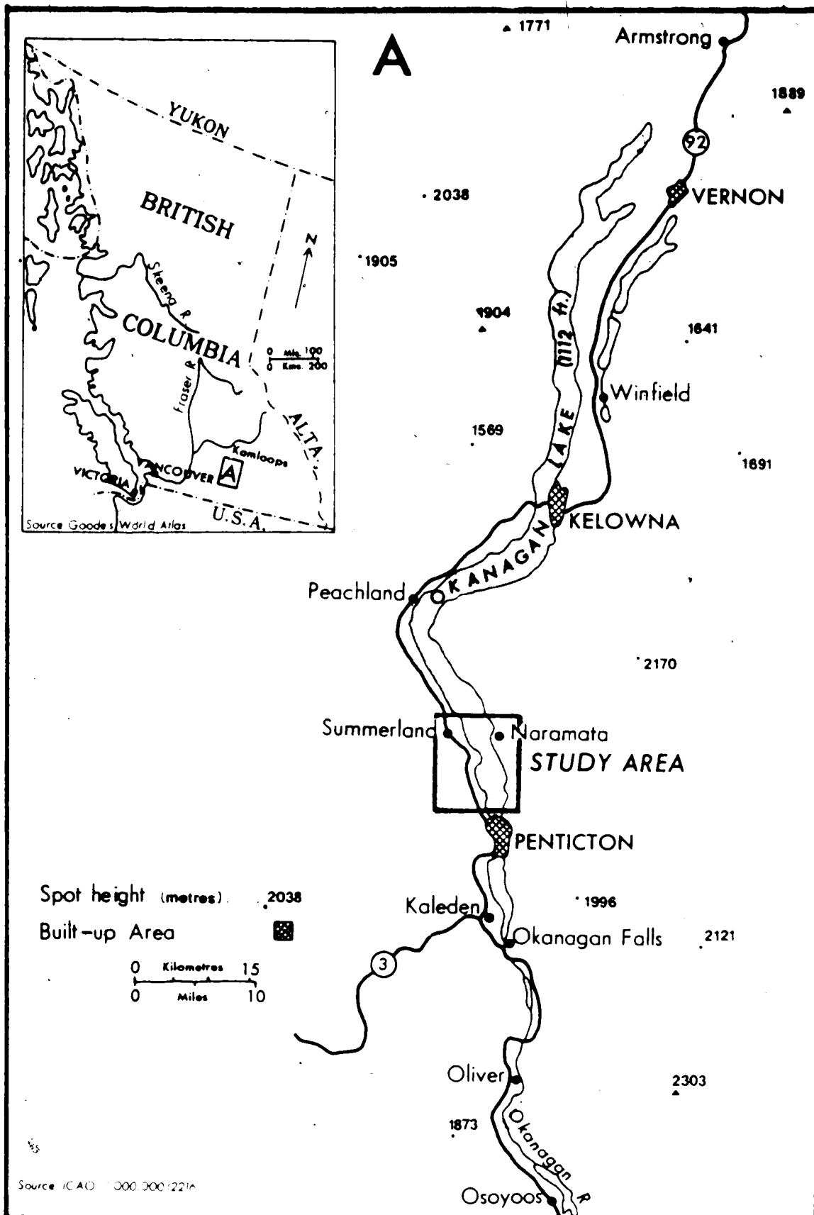
Figure 1-2 Study Area Location
