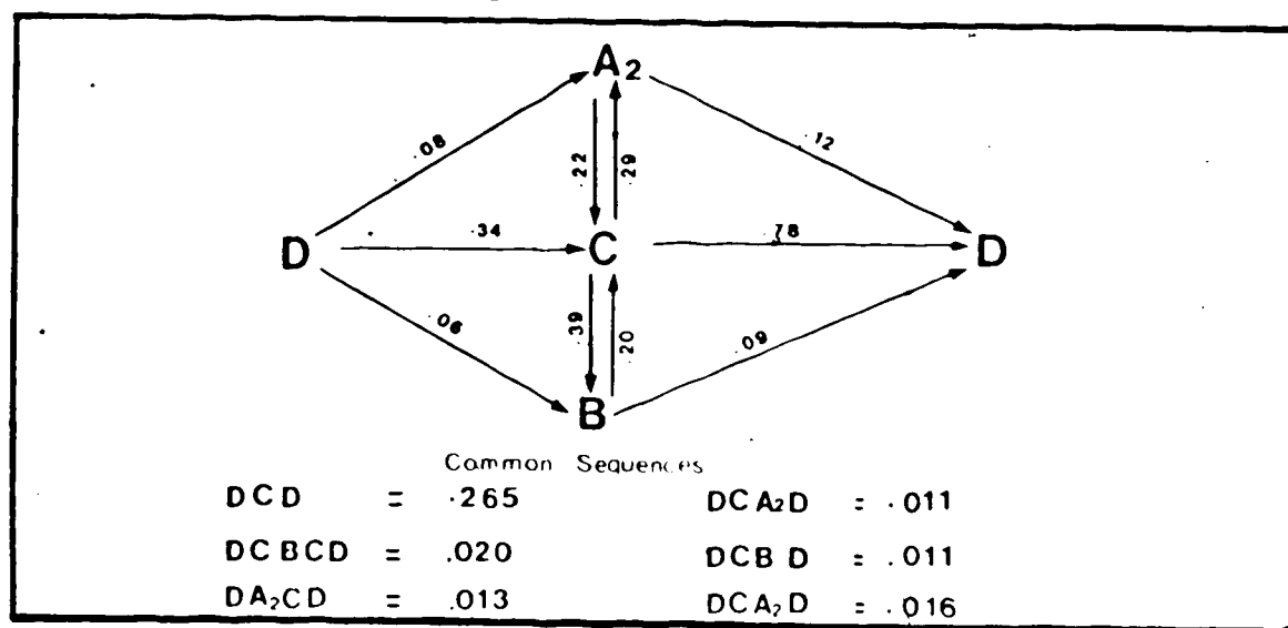
Figure 4-12 Transition tree diagram showing upward facies transitions for selected sections
