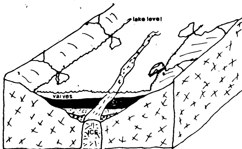
STAGE 3 Deposition of varved sediments as the sediment source becomes more distal and Lake Penticton develops
