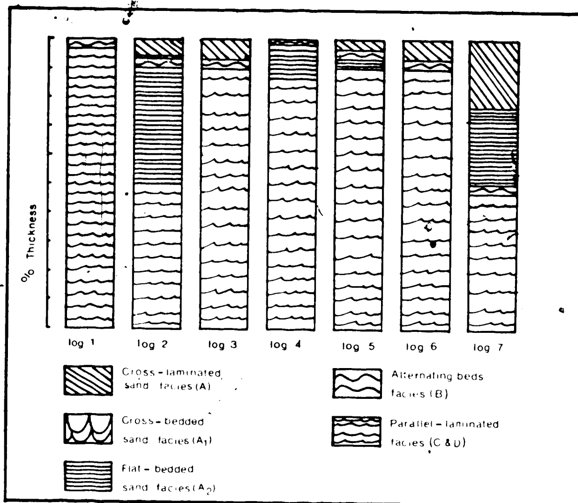
Figure 4-1.1 Proportional thickness of facies in each section
