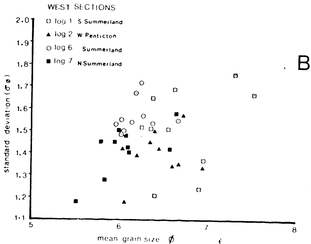
Figure 4-13 Scatter plot mean grain vs standard deviation
