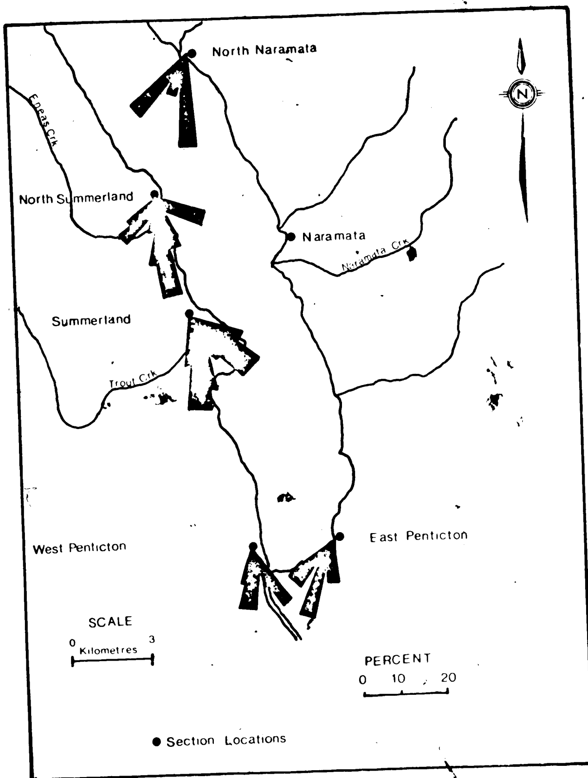
Figure 4-17 Paleocurrent directions
