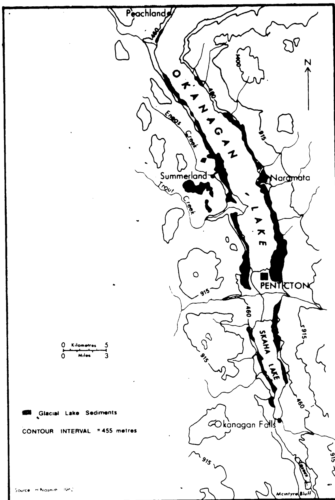
Figure 1-3 Physiography and Glacial Lake Sediment Distribution
