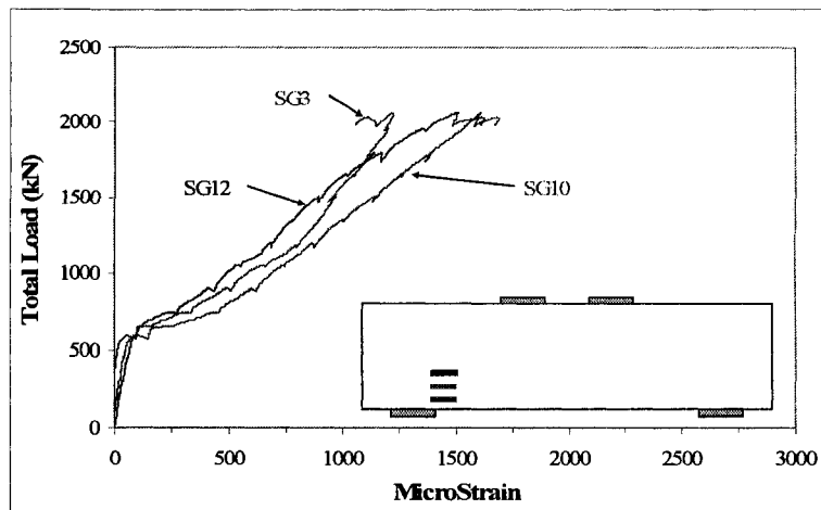
Figure A-55 Strain at the interior edge of one support for the three layers of tension reinforcement of specimen MS2-3
