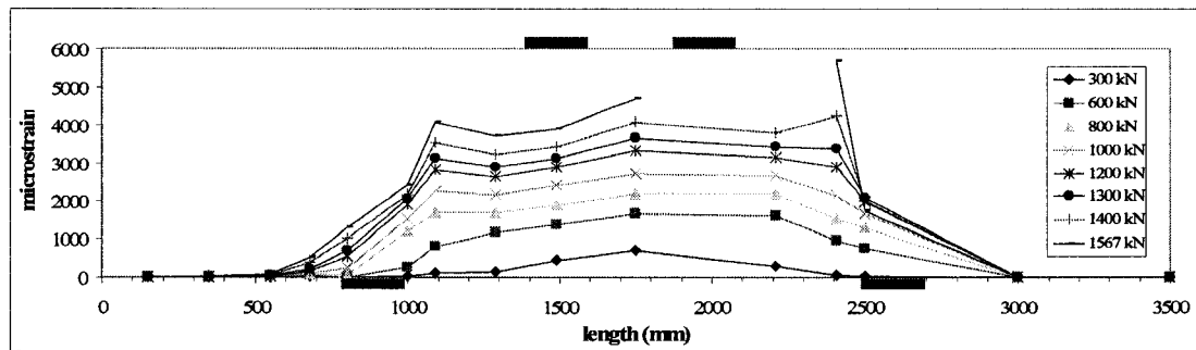
Figure 4-41 Strain distribution along the bar located in the lowest layer of main tension reinforcement of specimen MW1-2
