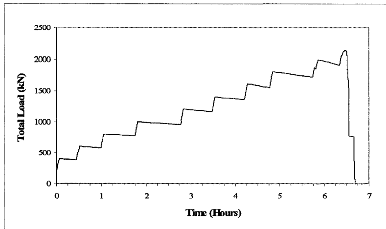
Figure A-12 Load-time response of specimen MS1-2
