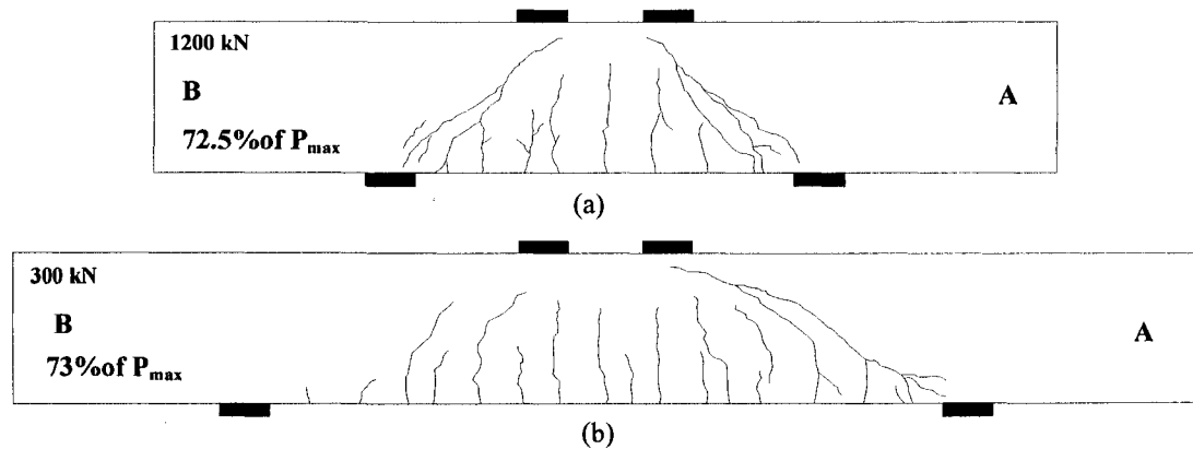
Figure 5-22 (a) Crack development of MW1-2 at 1200 kN (72.5% of P_{max} ) and (b) Crack development of MW3-2 at 300 kN (73% of P_{max} )
