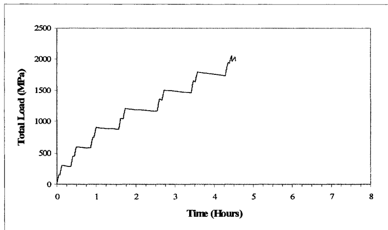
Figure A-47 Load-time response of specimen MS2-3
