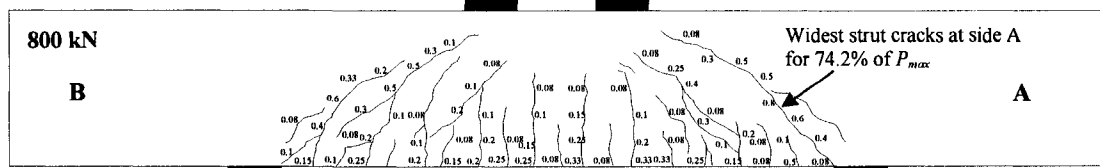
Figure 4-57 Crack development at 74.2 % of P_{max} for specimen NS2-4
