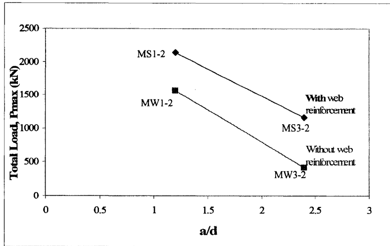
Figure 5-23 Influence of web reinforcement on member strength
