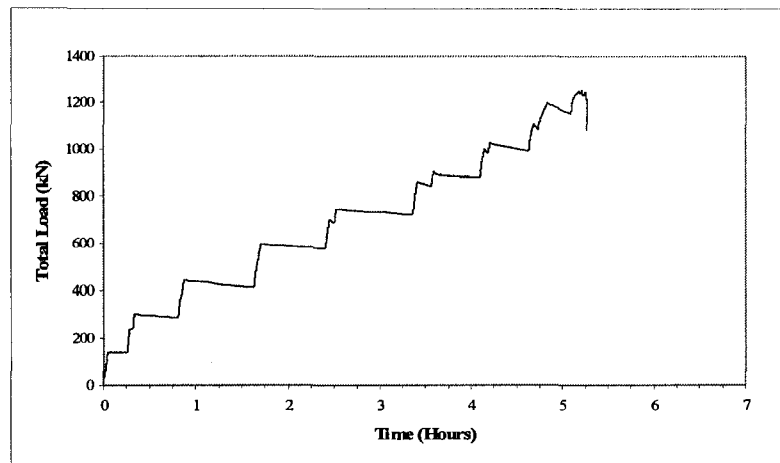
Figure A-1 Load-time response of specimen MS1-1
