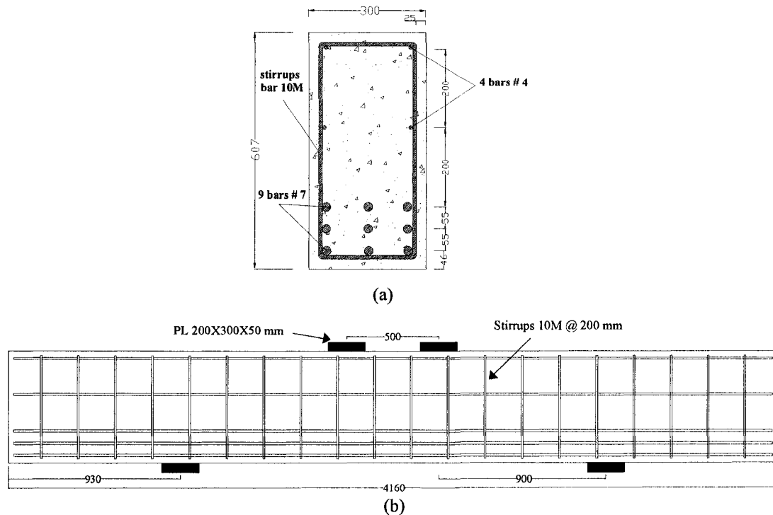
Figure 3-6 Beam MS2-3: (a) Cross section (b) Elevation
