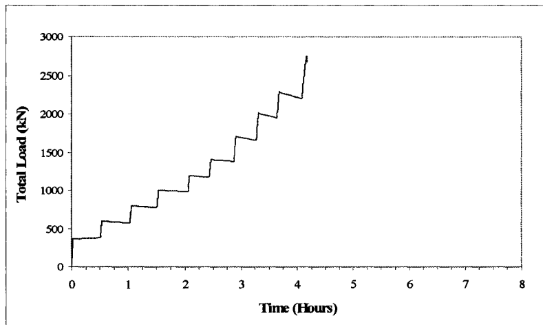
Figure A-24 Load-time response of specimen MS1-3
