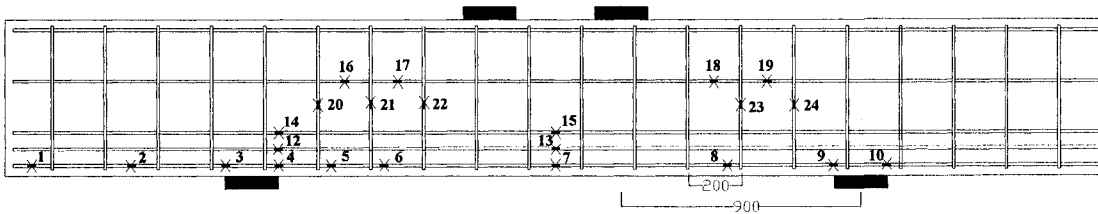
Figure 3-25 Strain gauge locations of beam MS2-2
