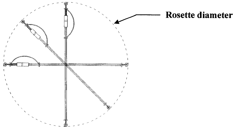
Figure 3-32 LVDT rosettes
