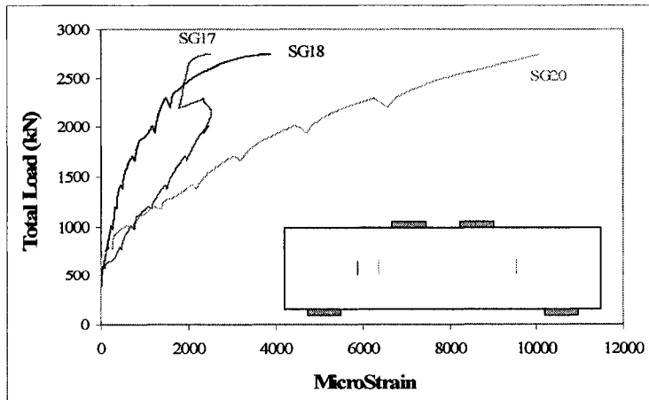
Figure A-30 Strains of stirrups located in the shear spans of specimen MS1-3
