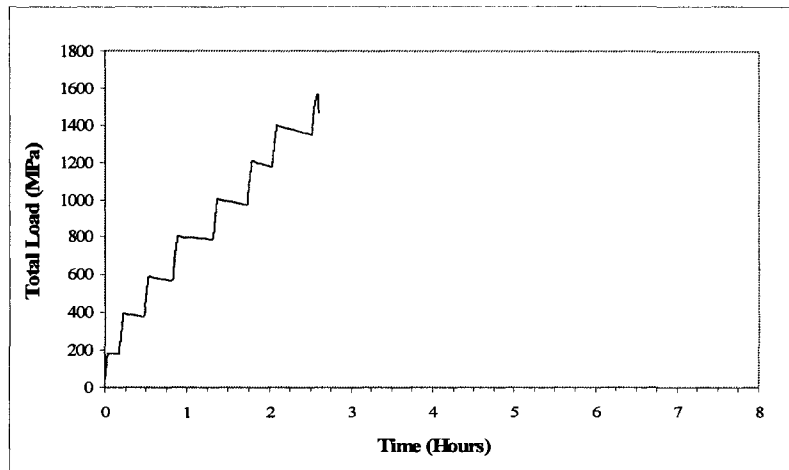
Figure A-70 Load-time response of specimen MS1-1
