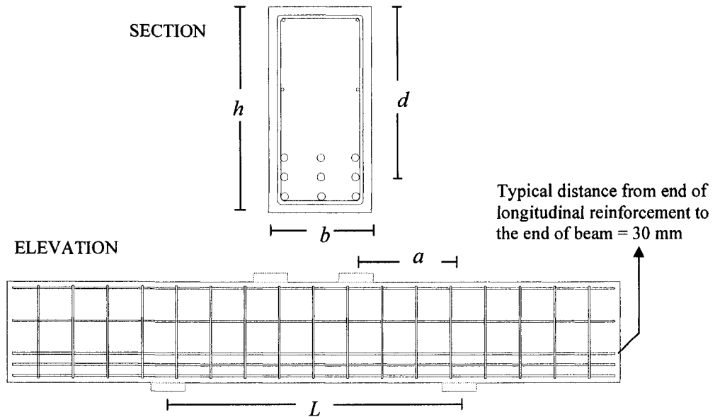
Figure 3-1 Symbolic dimensions of specimens
