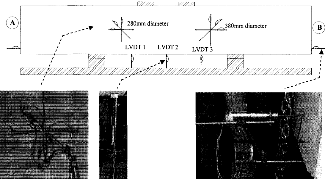
Figure 3-33 LVDT locations
