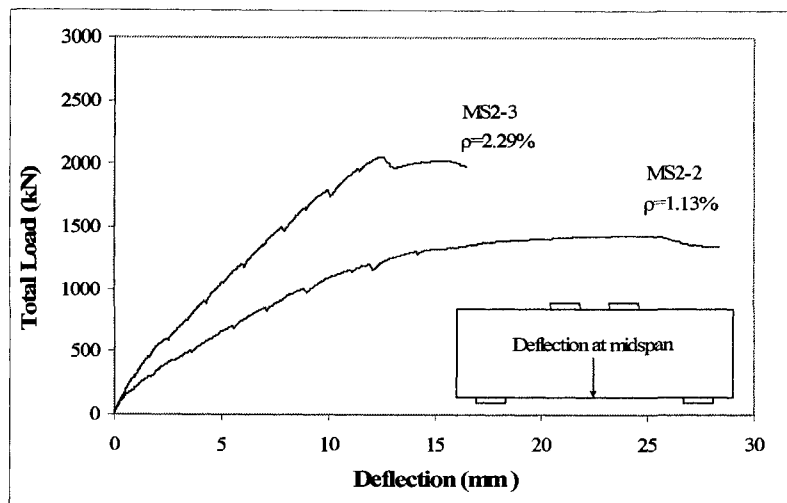
Figure 5-15 Load-deflection response for specimens MS2-2 and MS2-3
