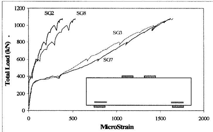
Figure A-108 Strains at the interior and exterior edges of the supports of specimen NS2-4
