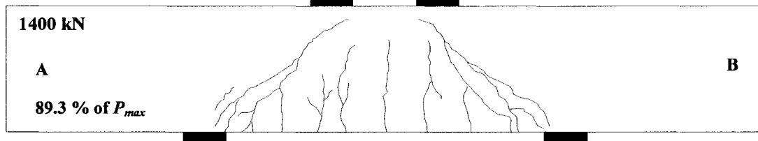
Figure 5-28 Crack development and crack width of MW1-2 at 1400 kN
