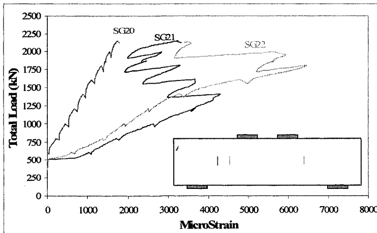
Figure A-18 Strains of stirrups located in the shear spans of specimen MS1-2
