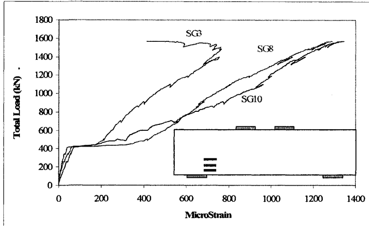
Figure A-98 Strain at the interior edge of one support for the three layers of tension reinforcement of specimen NS1-4
