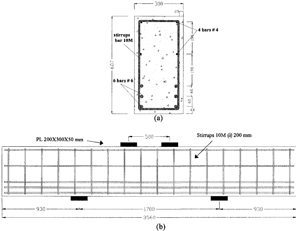
Figure 3-3 Beam MS1-2: (a) Cross section (b) Elevation.
