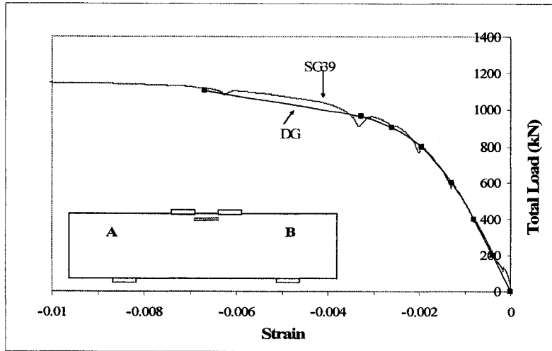
Figure 4-37 Strain in top strut of specimen MS3-2
