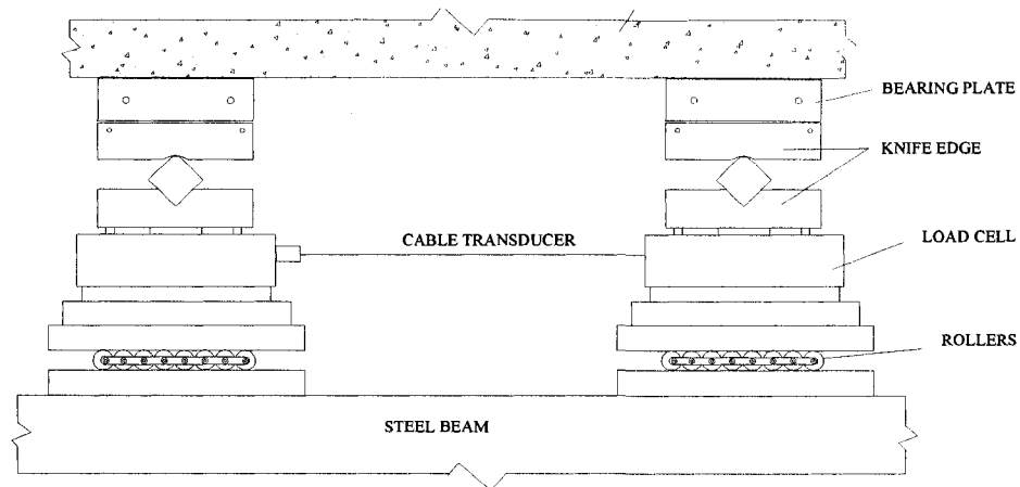
Figure 3-21 Supports details
