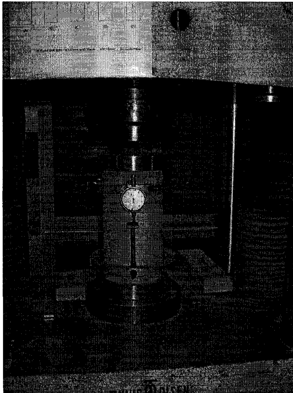
Figure 3-14 Compression test of concrete cylinder
