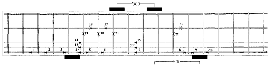
Figure A-3 Strain gages locations of specimen MS1-1
