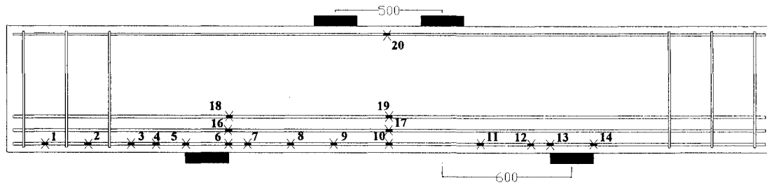
Figure 3-30 Strain gauge locations of beam MW1-2
