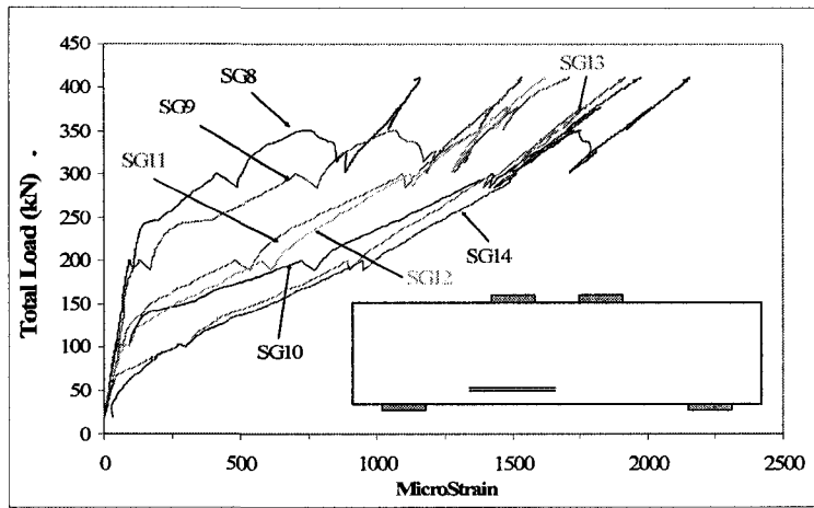
Figure A-83 Strains at a bar located in the lowest layer of main tension reinforcement of specimen MW3-2
