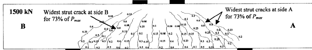
Figure 4-28 Crack development at 73% of P_{max} for specimen MS2-3
