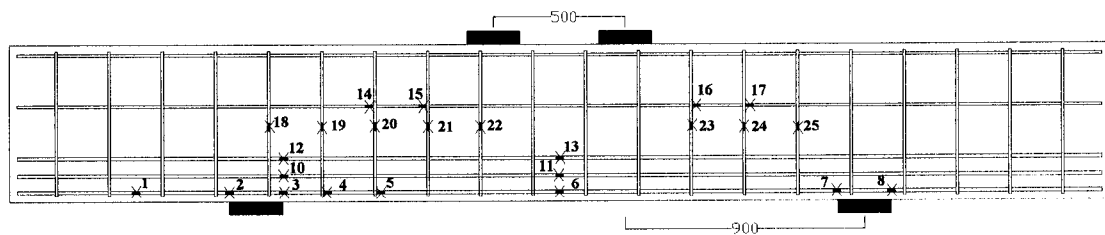
Figure 3-29 Strain gauge locations of beam NS2-4
