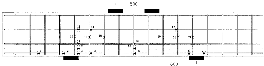
Figure A-27 Strain gages locations of specimen MS1-3
