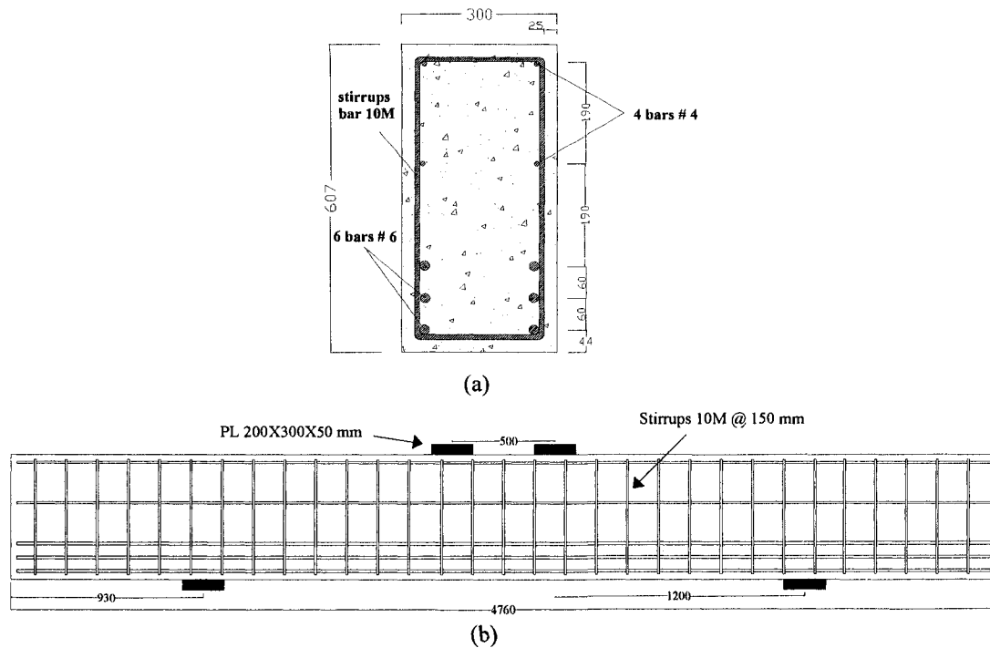
Figure 3-7 Beam MS3-2: (a) Cross section (b) Elevation
