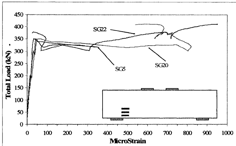
Figure A-86 Strain at the interior edge of one support for the three layers of tension reinforcement of specimen MW3-2
