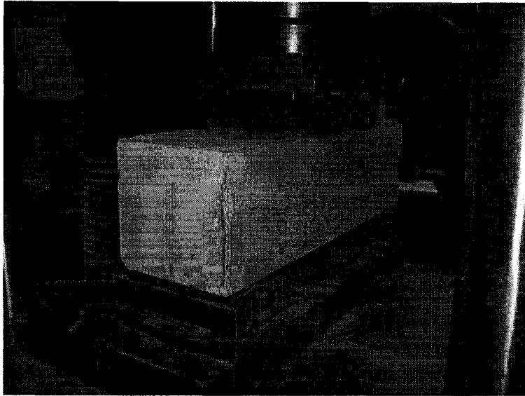
Figure 3-15 Flexural test to obtain the modulus of rupture
