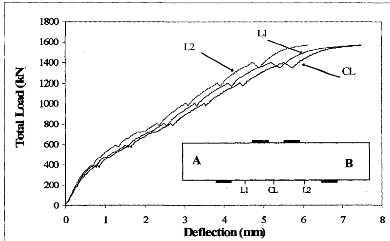
Figure 4-39 Deflection at midspan and 450 mm from midspan of specimen MW1-2
