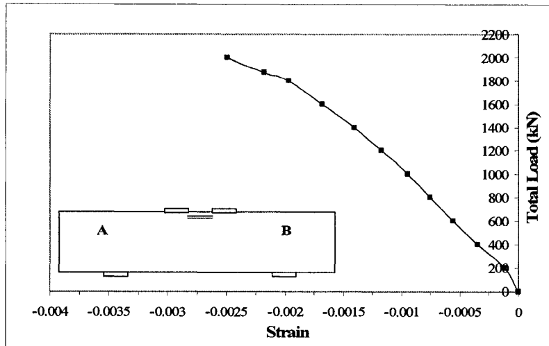
Figure 4-13 Strain in top strut of specimen MS1-2
