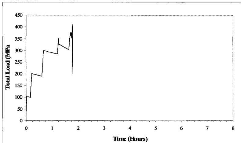
Figure A-80 Load-time response of specimen MW3-2
