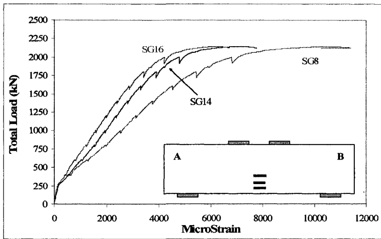
Figure A-17 Strains at midspan of the three layers of main tension reinforcement in specimen MS1-2
