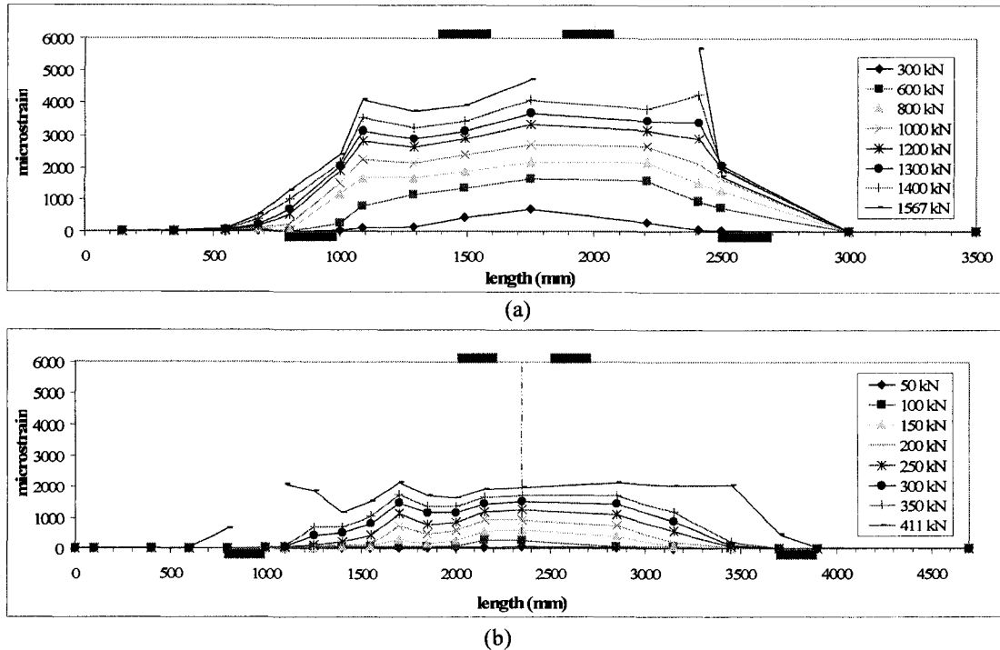
Figure 5-21 Strain distribution along the bottom bar for (a) MW1-2 and (b) MW3-2 at different loading stages
