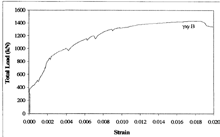
Figure A-46 Maximum shear strain in diagonal struts of specimen MS2-2
