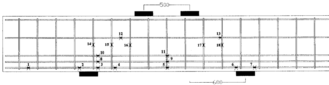
Figure 3-28 Strain gauge locations of beam NS1-4
