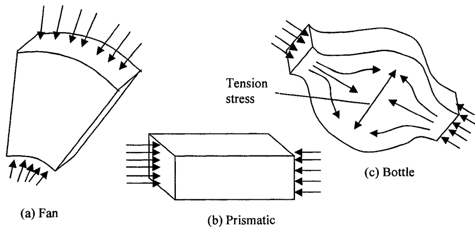
Figure 2-2 Basic compression stress fields or struts
