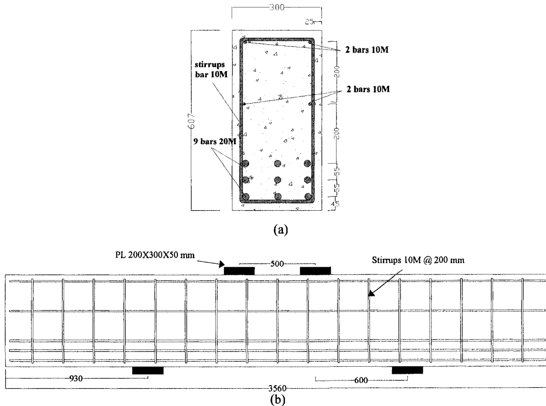
Figure 3-8 Beam NS1-4: (a) Cross section (b) Elevation
