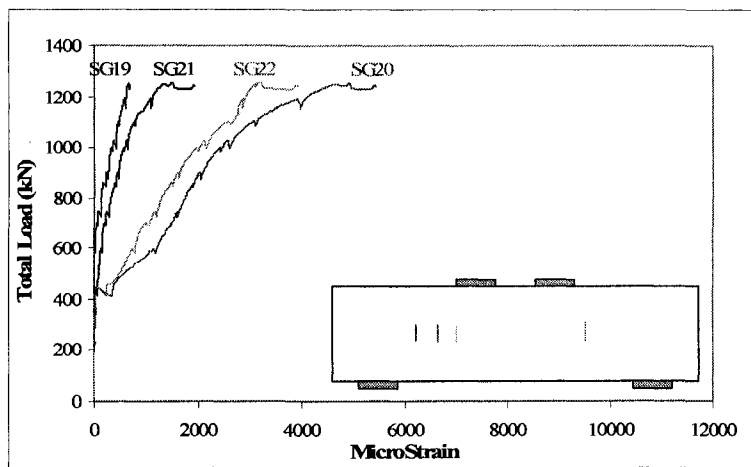
Figure A-6 Strains of stirrups located in the shear spans of specimen MS1-1
