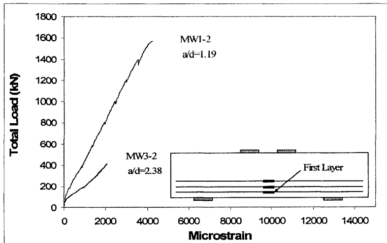
Figure 5-20 Load-strain response for MW1-2 and MW3-2
