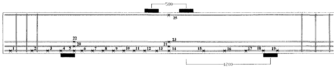
Figure A-82 Strain gauges locations of specimen MW3-2
