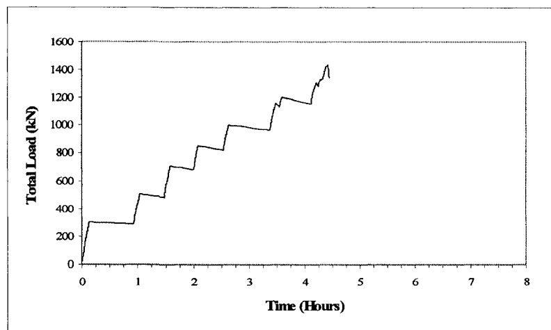
Figure A-36 Load-time response for specimen MS2-2
