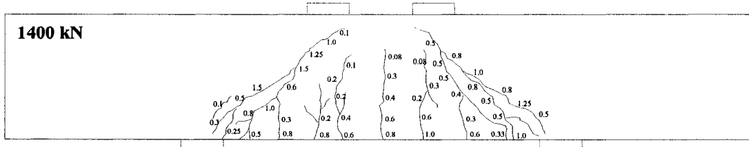
Figure A-72 Crack patterns at 1400 kN of specimen MW1-2
