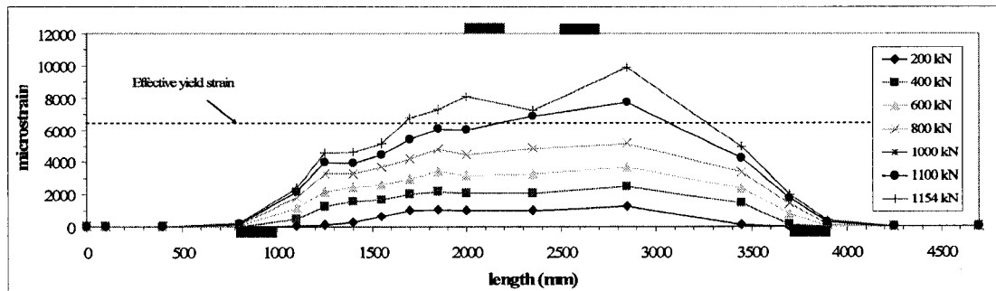
Figure 4-35 Strain distribution along the bar located in the lowest layer of main tension reinforcement of specimen MS3-2
