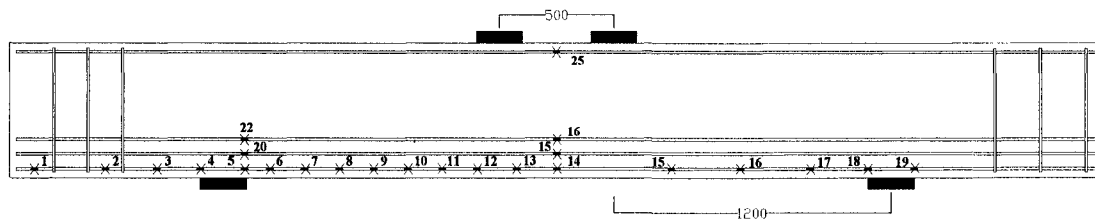
Figure 3-31 Strain gauge locations of beam MW1-3
