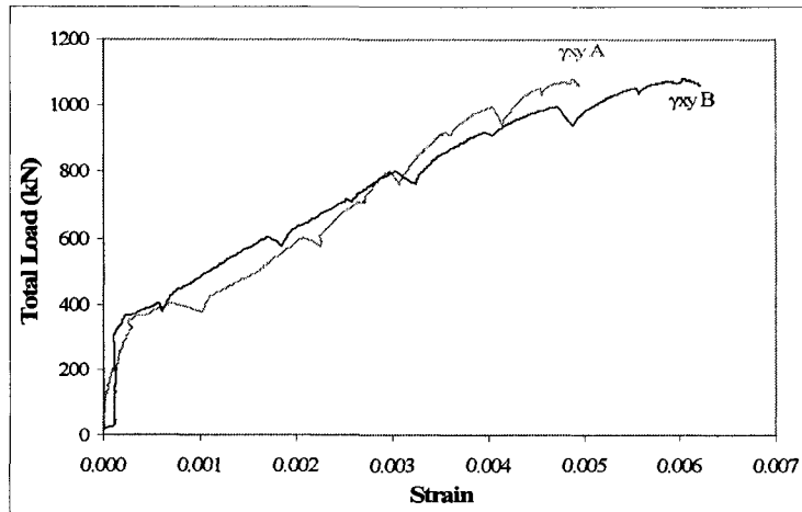
Figure A-111 Maximum shear strain
