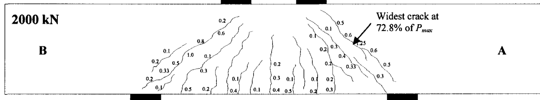
Figure 4-16 Crack development at 72.8% of P_{max} of specimen MS1-3
