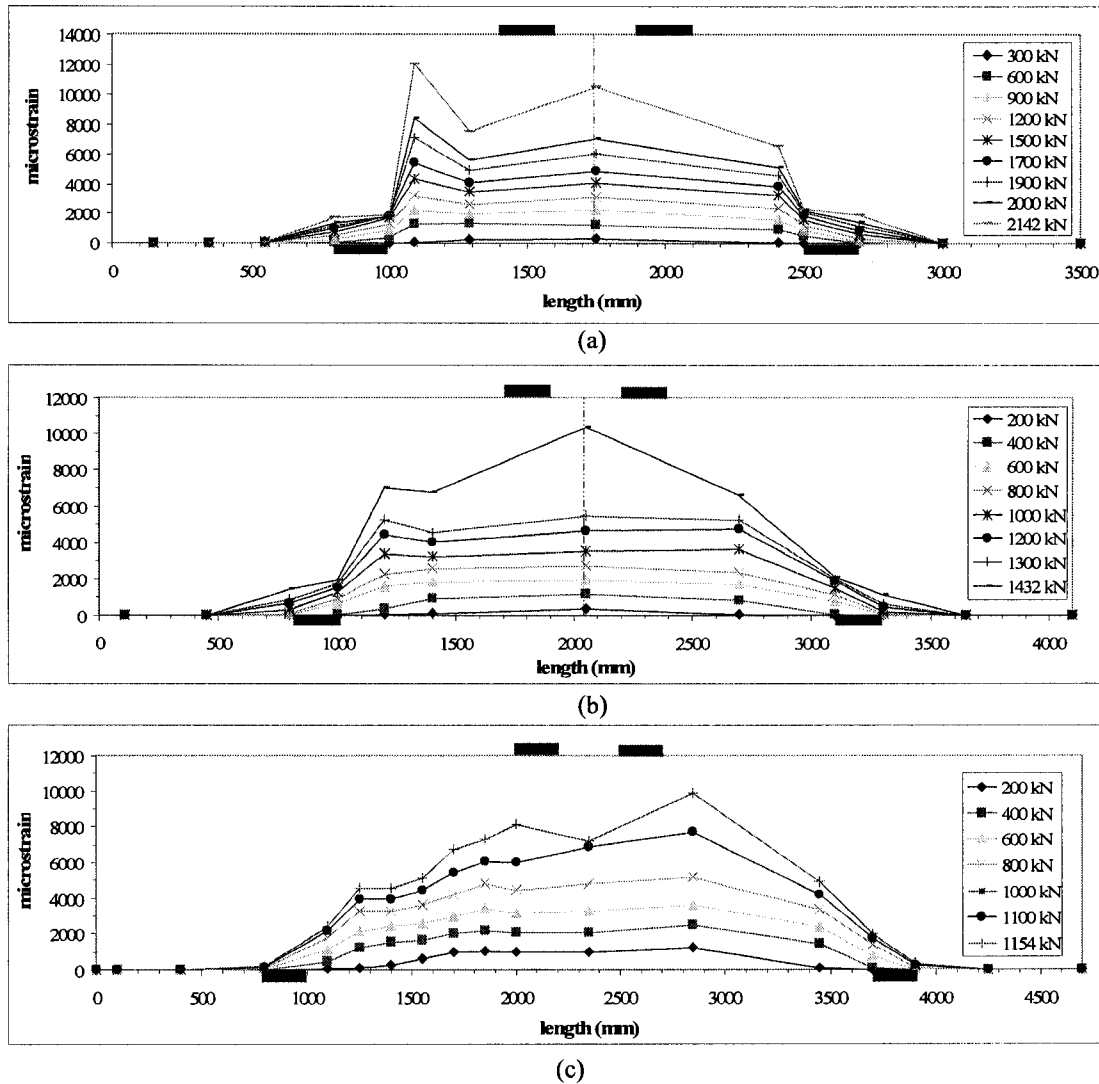
Figure 5-4 Strain distribution along the lowest reinforcement bar for specimens (a) MS1-2, (b) MS2-2 and (c) MS3-2 at different loading stages
