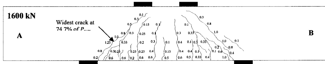
Figure 4-10 Crack development at 74.7% of P_{max} for specimen MS1-2
