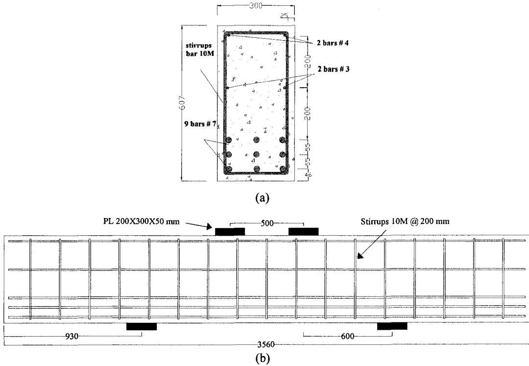
Figure 3-4 Beam MS1-3: (a) Cross section (b) Elevation
