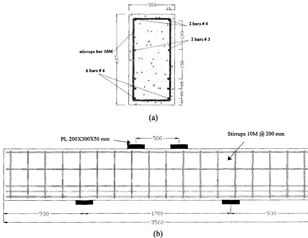
Figure 3-2 Beam MS1-1: (a) Cross section (b) Elevation.
