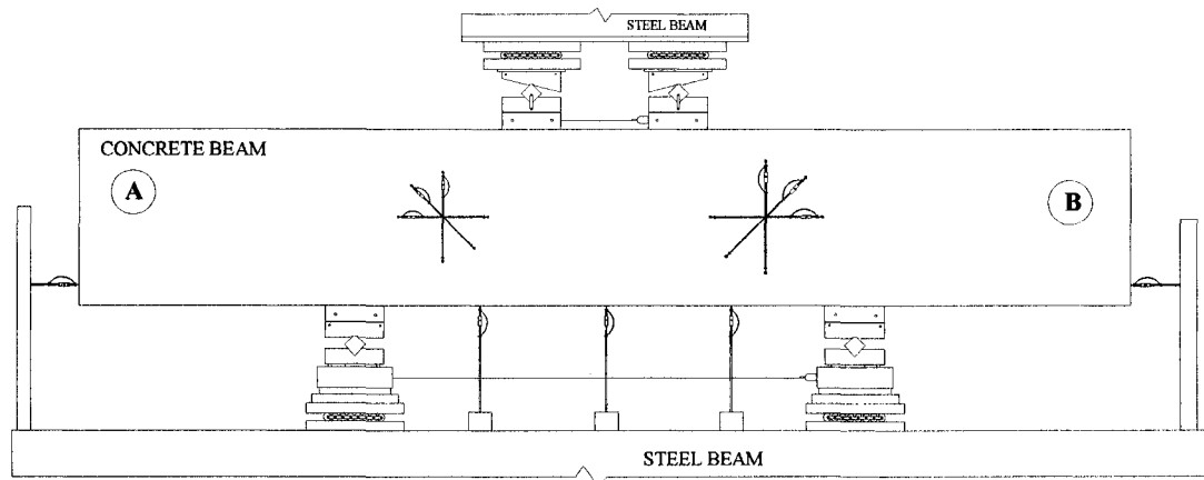
Figure 3-19 General set up
