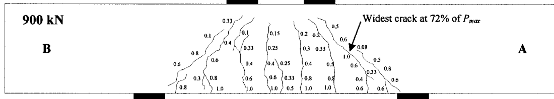
Figure 4-3 Crack development of specimen MS1-1 at 72% of P_{max}
