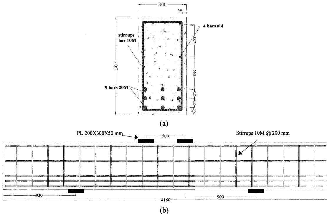
Figure 3-9 Beam NS2-4: (a) Cross section (b) Elevation
