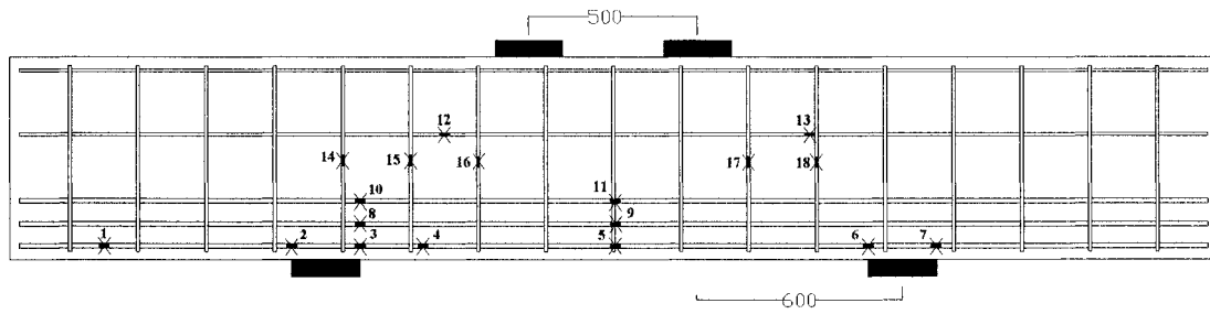
Figure A-92 Strain gauges locations of specimen NS1-4
