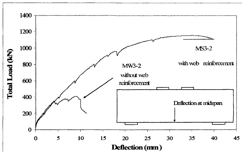
Figure 5-29 Load-deflection response for specimens MS3-2 and MW3-2
