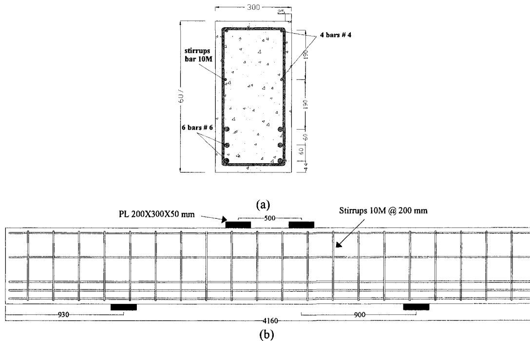
Figure 3-5 Beam MS2-2: (a) Cross section (b) Elevation
