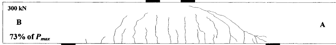
Figure 5-33 Crack development of specimen MW3-2 at 300 kN
