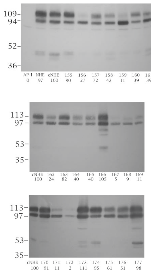
FIG. 3. Western blot analysis of cell extracts from control and stably transfected AP-1 cells. Cell extracts were prepared from control (AP-1) cells and from cells stably transfected with cDNA coding for HA-tagged cells: wild-type NHE1 (NHE), cysteine-less NHE1 (cNHE), F155C, L156C, Q157C, S158C, D159C, V160C, F161C, F162C, L163C, F164C, L165C, L166C, P167C, P168C, I169C, I170C, L171C, D172C, A173C, G174C, Y175C, F176C, and L177C. 100 \mu g of total protein was loaded in each lane. Results are typical of at least two experiments. Numbers below the lanes indicate the values obtained from densitometric scans of the 110-kDa band relative to cNHE1.
