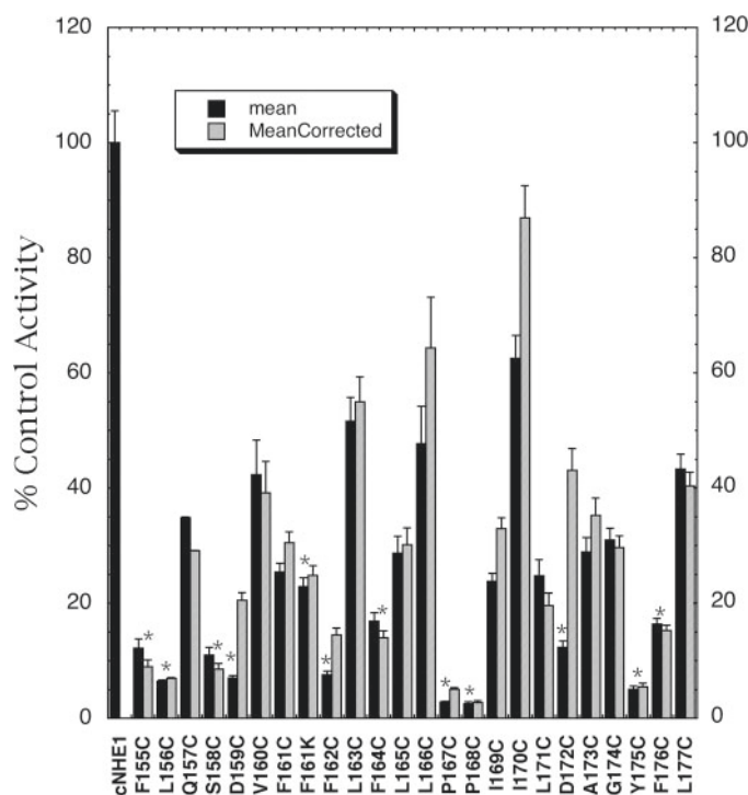
FIG. 2. Rate of recovery from an acid load by AP-1 cells stably transfected with cNHE1, and \text{Na}^+/\text{H}^+ exchanger mutants (Phe 155 to Leu 177 individually changed to Cys plus F161K). \text{Na}^+/\text{H}^+ exchanger activity was measured after transient induction with an acid load as described under "Experimental Procedures." The activity of cNHE1 stably transfected with NHE1 was 3.2 pH units/min, and this value was set to 100%. All mutations to cysteine were done in the background of the cysteine-less NHE1, and activities are percent of those of cNHE. The F161K mutation was done in the wild-type NHE1 background, and its activity is expressed as a percent of the wild-type NHE1 activity (4.25 pH units/min). All results are means \pm S.E. of at least 10 determinations from two independently made stable cell lines. Results are shown for mean activity both uncorrected (black) and normalized for surface processing (hatched). * indicates mutants with unnormalized activity that is less than 20% of cNHE1.
