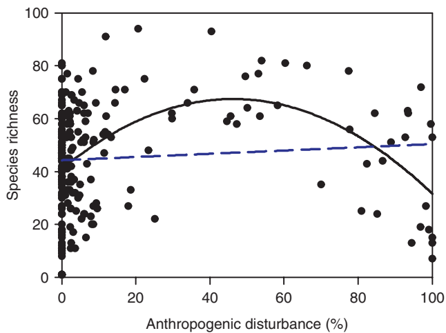
Figure 2 | Species richness to human disturbance relationship. Species richness per hectare of boreal vascular plants as a function of percent total anthropogenic disturbance extent. The black solid curve represents the adopted model, a quadratic curve ( n = 242 , P < 0.001 ), which supports the IDH. The blue dashed line represents another candidate model, a linear regression that was rejected.
