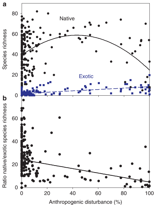
Figure 4 | Native and exotic species richness related to disturbance.
