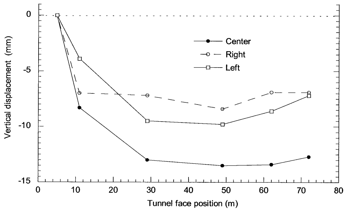
Figure 4.27 - Convergence – Basel tunnel meter 998
