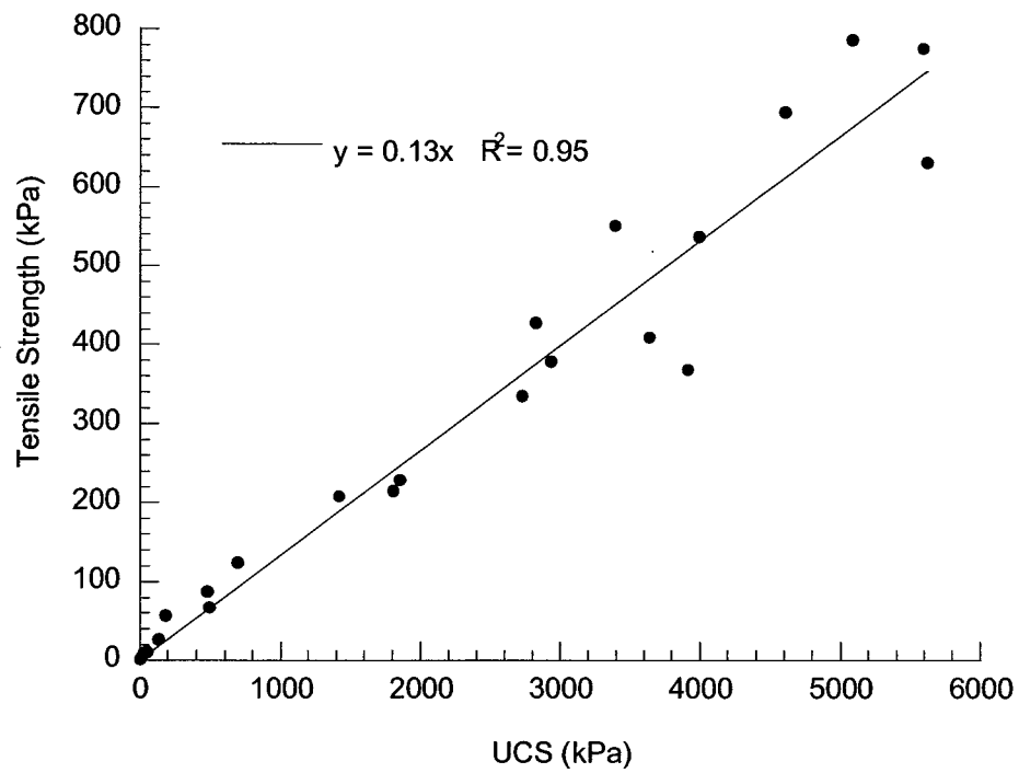
Figure 3.5 - Relationship between tensile strength and unconfined compressive strength for grout.
