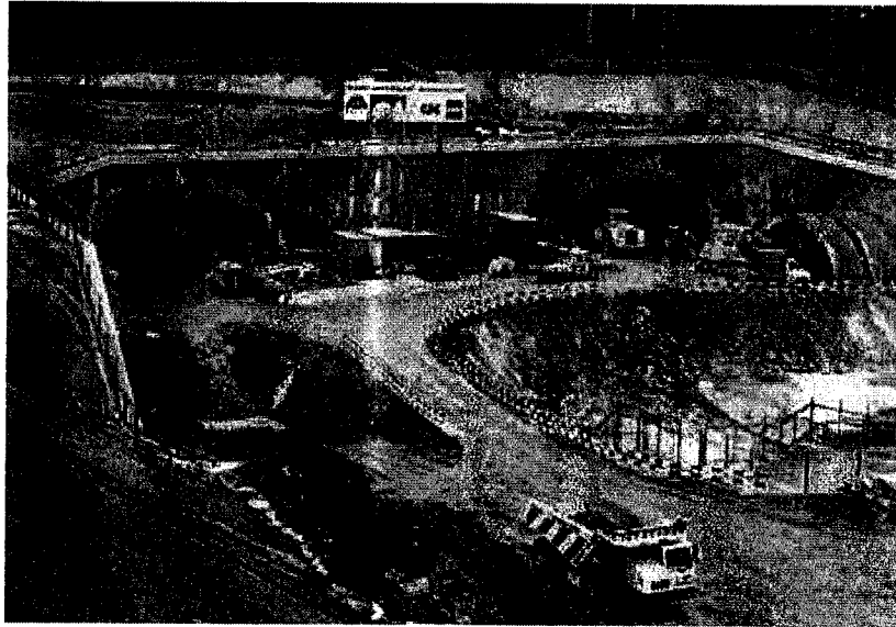
Figure 4.9 - Tantenholtz portal (Southeast) showing tangent pile wall
