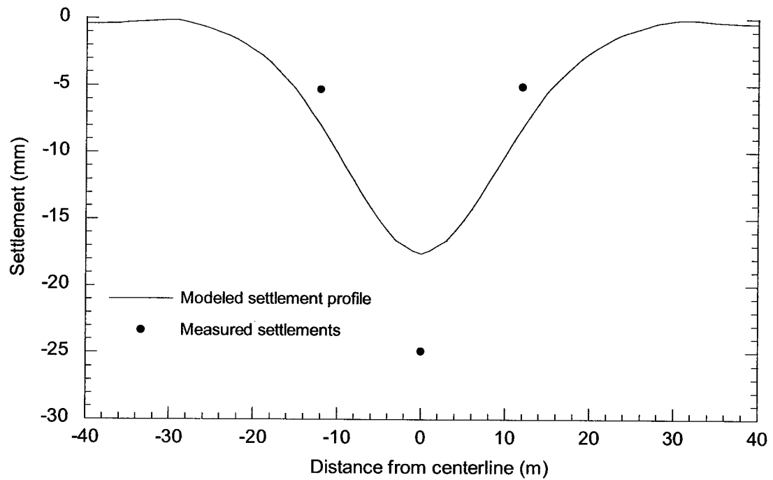
Figure 5.12 - Modeled vs. measured settlements for Basel profile 2, elastic-plastic model
