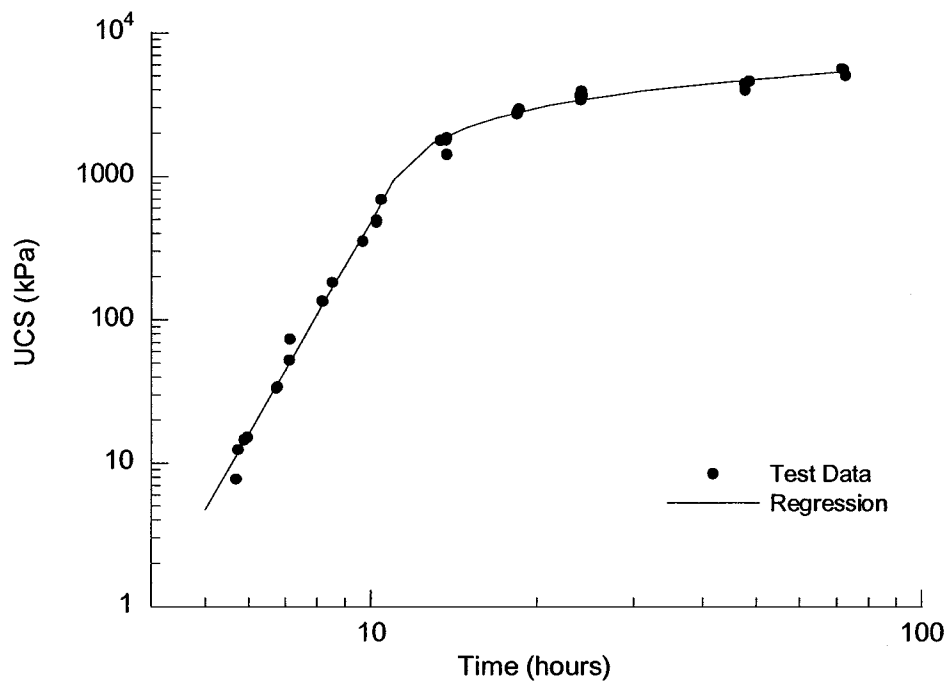
Figure 3.2 - Unconfined compressive strength (UCS) of grout as a function of time
