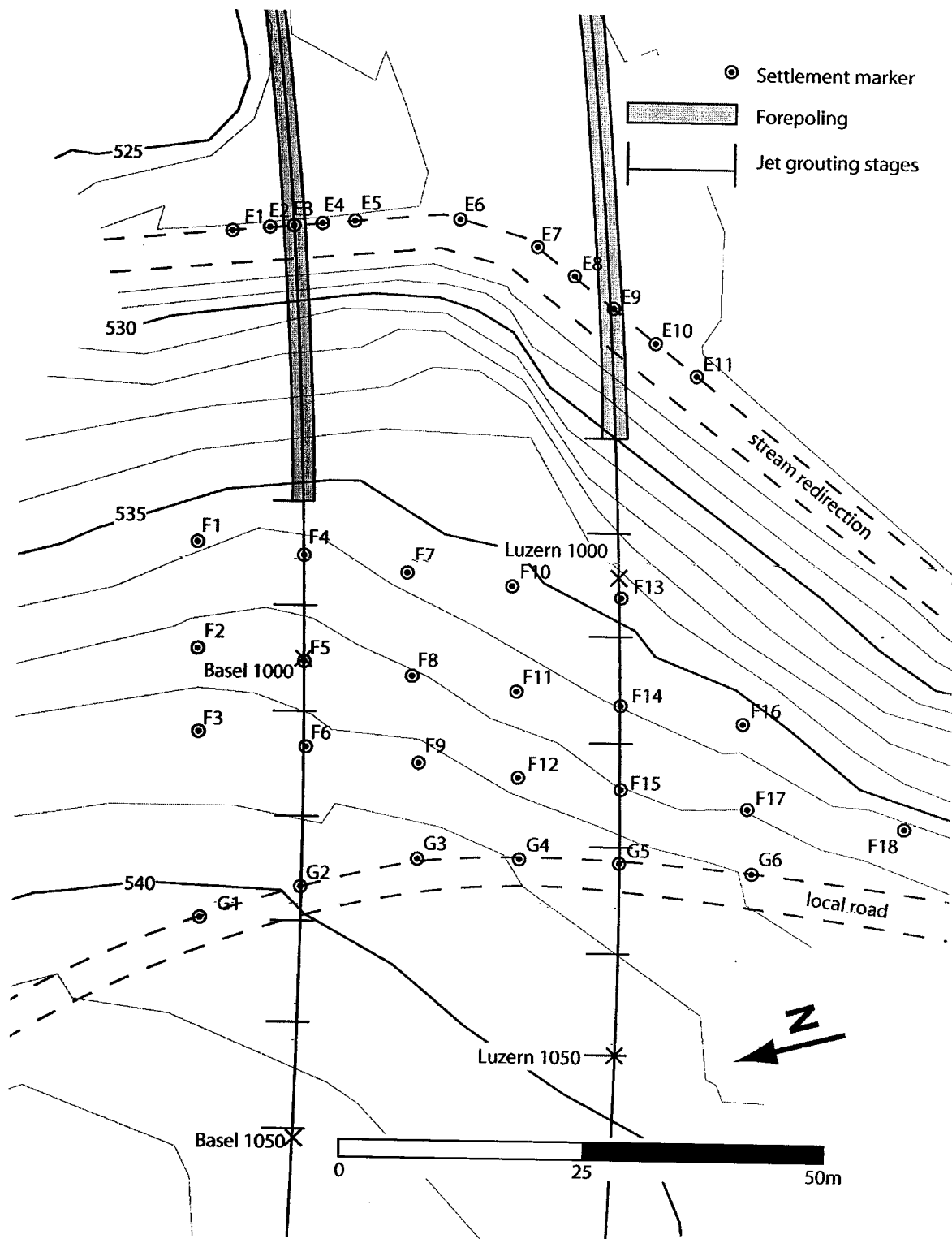
Figure 4.8 - Plan view of the settlement points in the vicinity of Aescherbach
