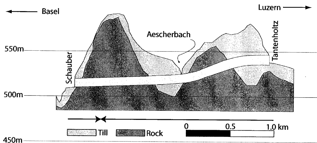
Figure 4.2 - Aeschertunnel profile
