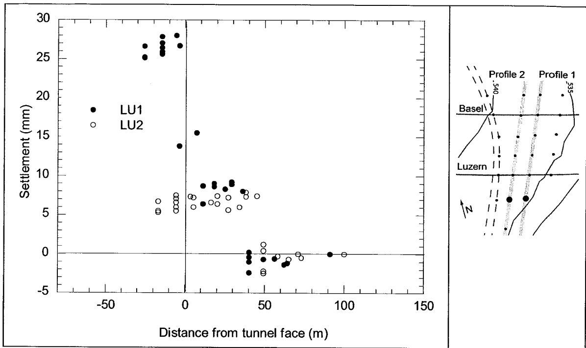
Figure 4.25 - Settlement development 12m South of Luzern axis
