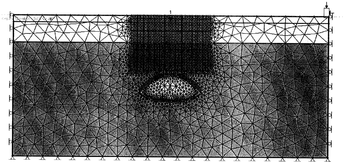
Figure 5.17 - Finite element mesh for strain softening model with high grout pressures
