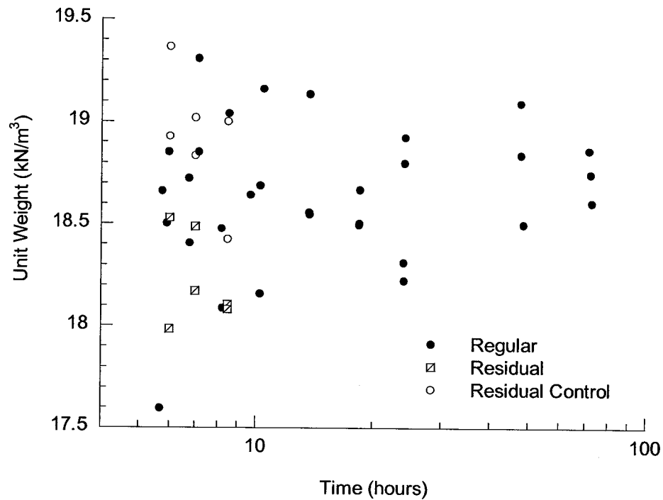
Figure 3.17. - Density of grout samples
