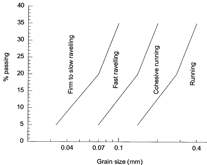
Figure 2.4 - Behavior of dense soil ( N > 30 ) above ground water level, modified from Heuer (1987)
