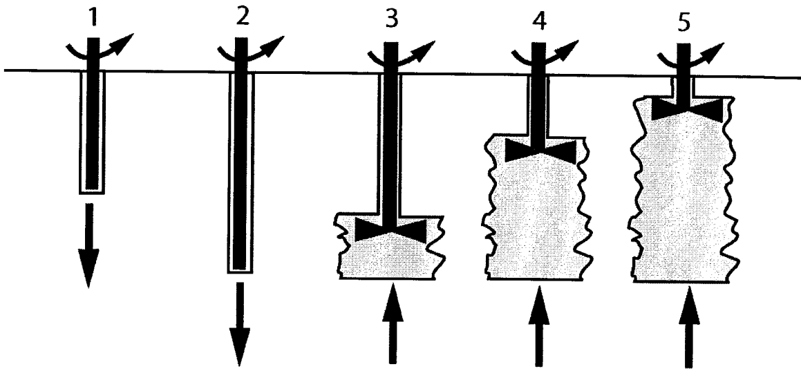
Figure 2.6 - Jet-grouting procedure
