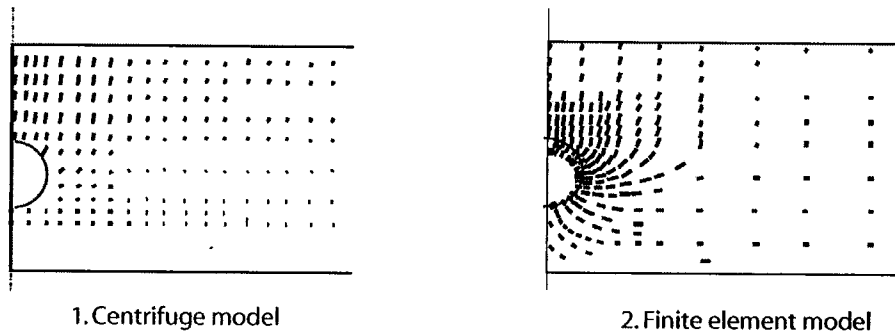
Figure 5.6. - Trough width overestimation with FEM in sand overlying clay Modified from Stallebras (1996)
