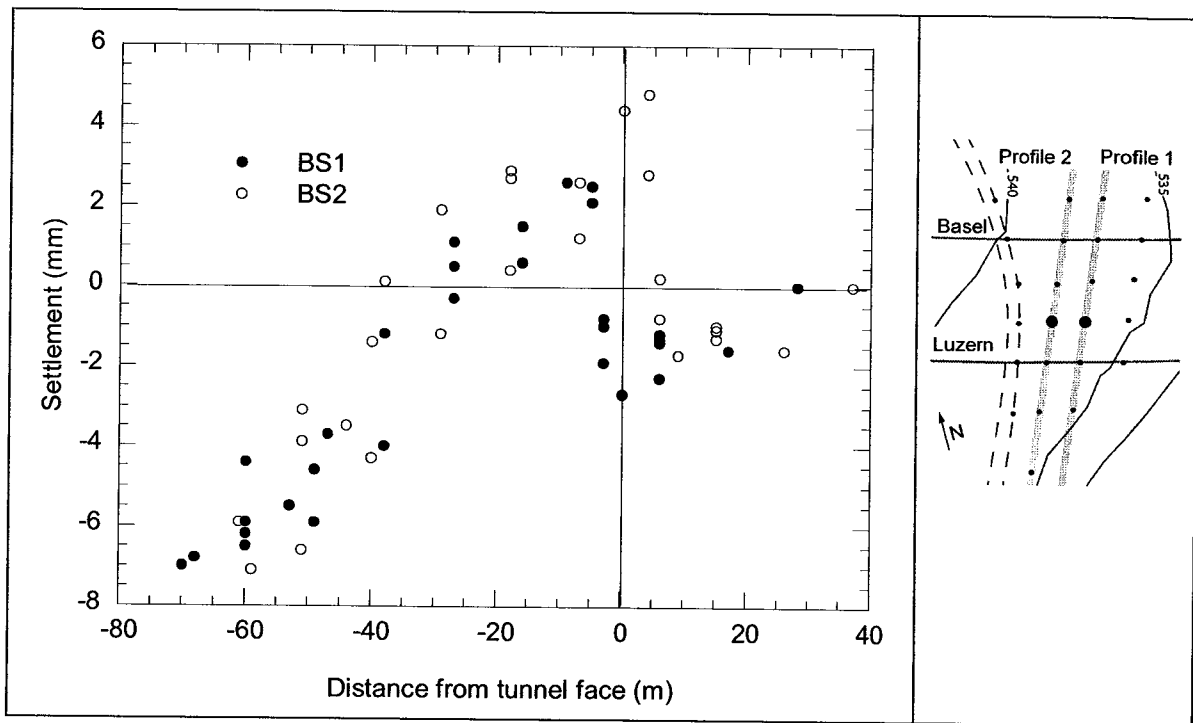
Figure 4.23 - Settlement development 20m South of Basel axis.
