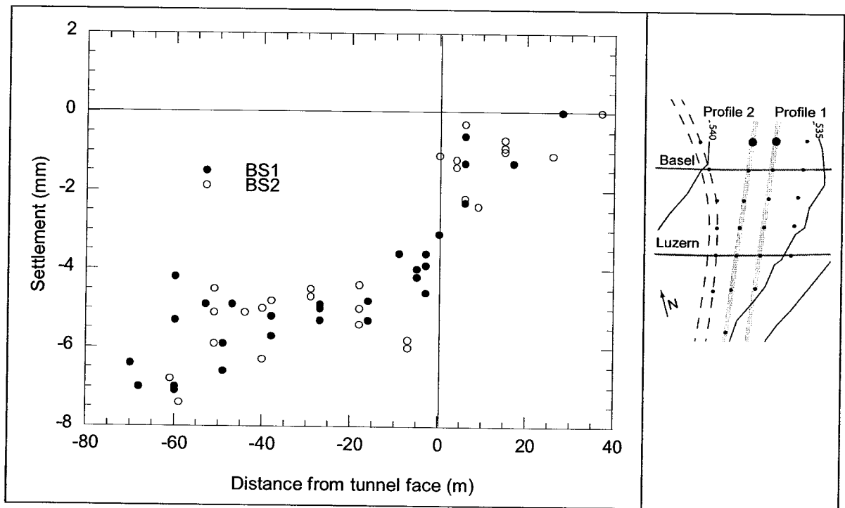
Figure 4.21 - Settlement Development 12m North of Basel axis
