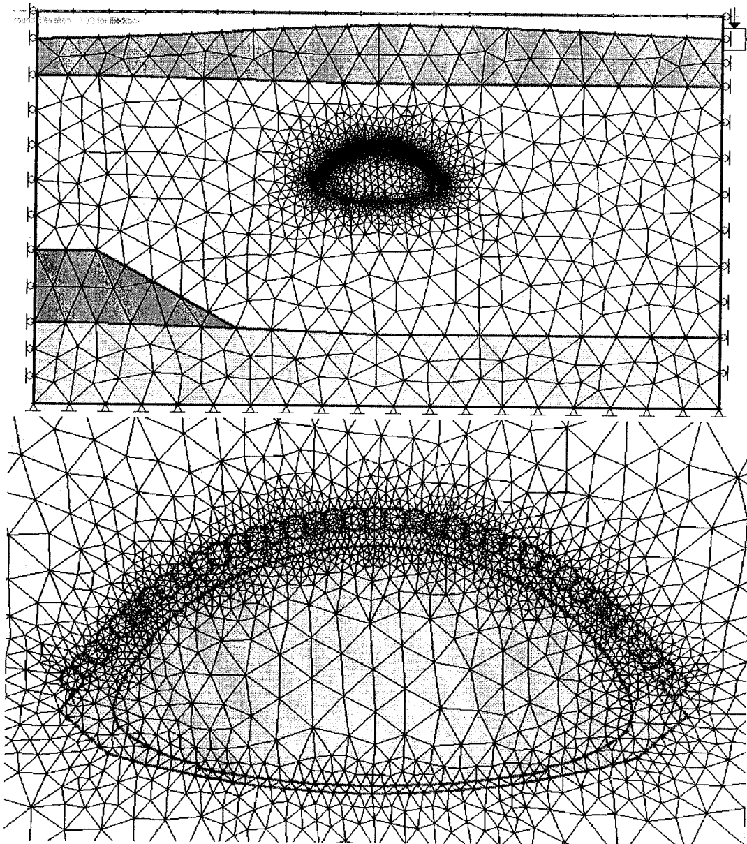
Figure 5.7 – The finite element grade triangular mesh used in the elastic analysis
