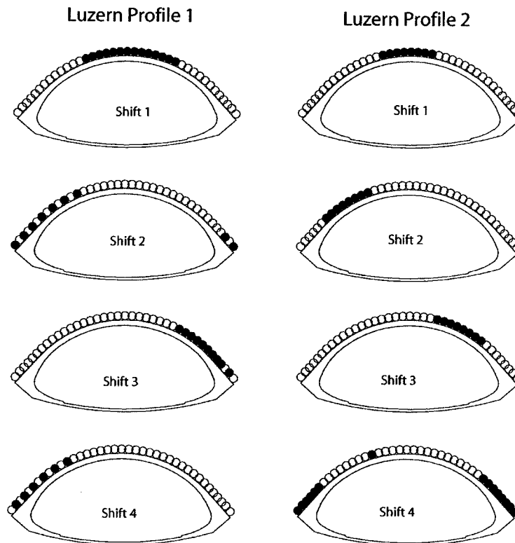
Figure 4.15 - Jet-grout installation sequence for Luzern profiles 1 & 2
