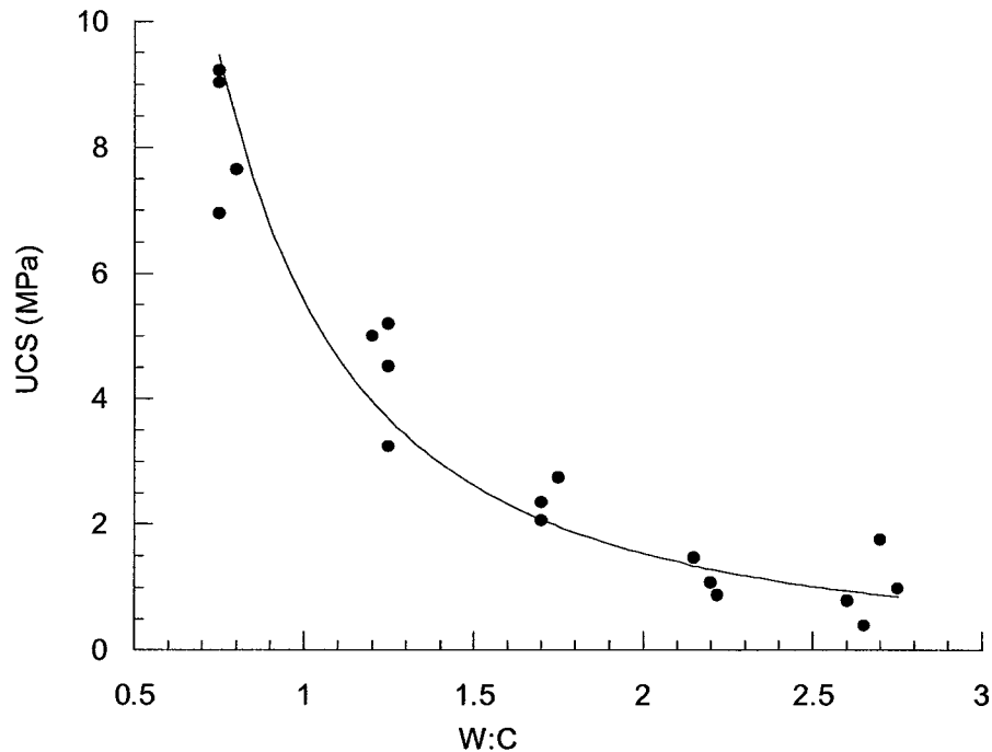
Figure 2.8 - Relationship between uniaxial compressive strength (UCS) and water to cement ratio, by weight, data from Kauschinger (1992)
