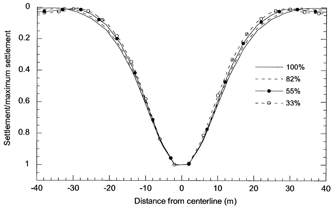
Figure 5.14 - Effect of a reduced softening area, expressed as a percentage of the tunnel cross sectional area, on the trough width
