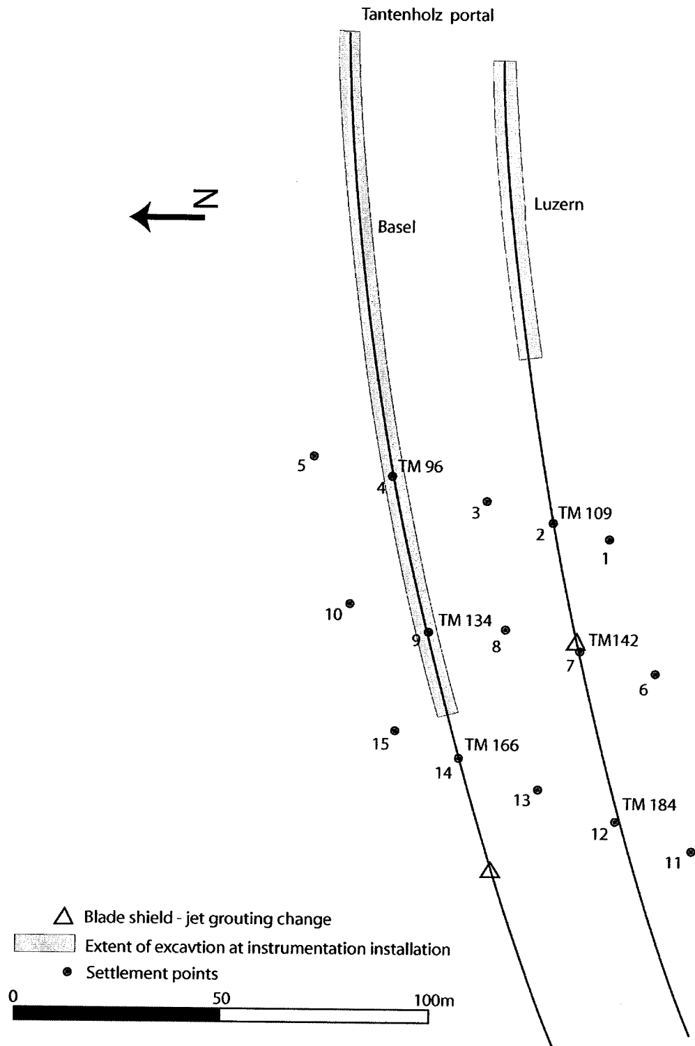
Figure 4.7 - Plan view of the settlement points in the vicinity of the Tantenholz portal
