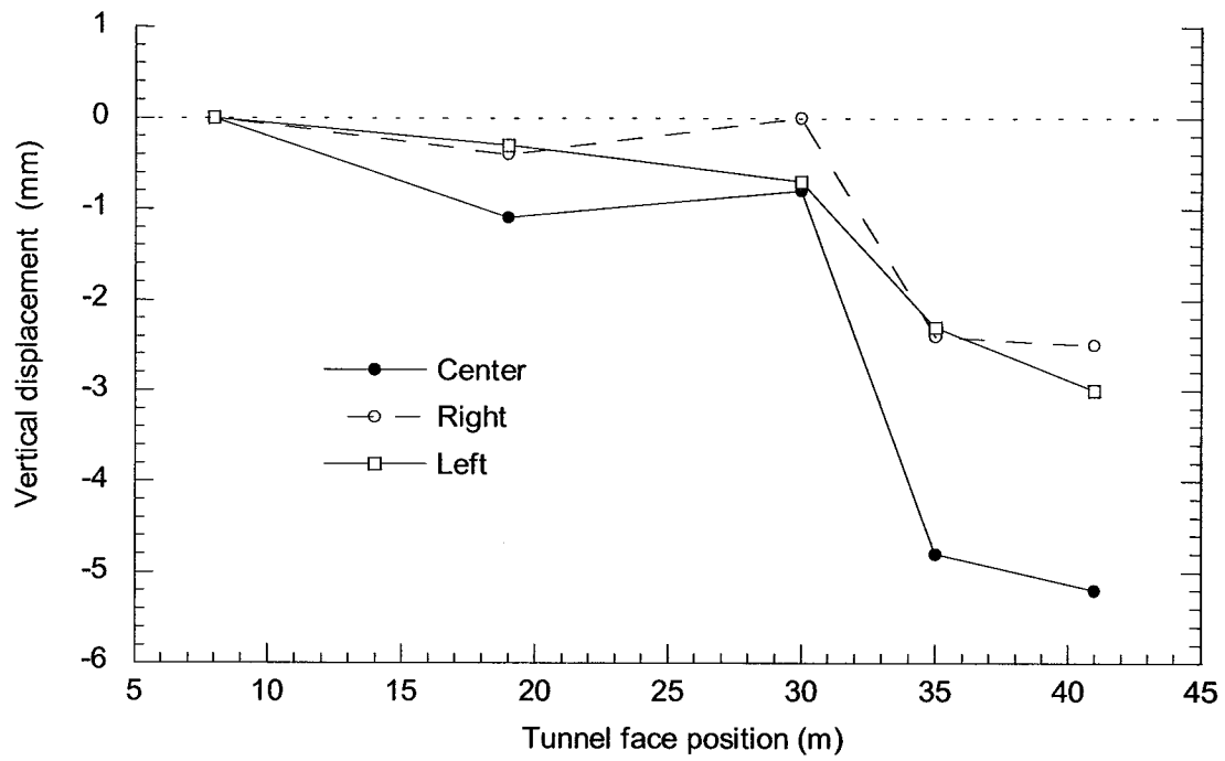
Figure 4.26 - Convergence – Luzern tunnel meter 1020
