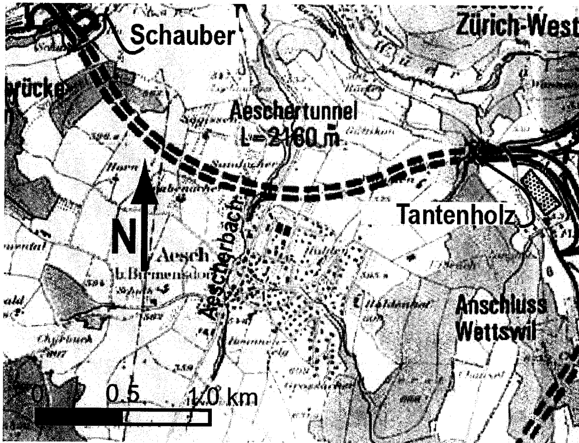
Figure 4.1 - Aeschertunnel route 3
