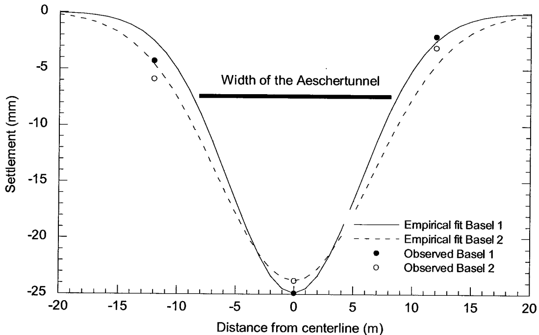
Figure 5.4 - Observed vs. empirical fit settlements for Basel profiles 1 and 2
