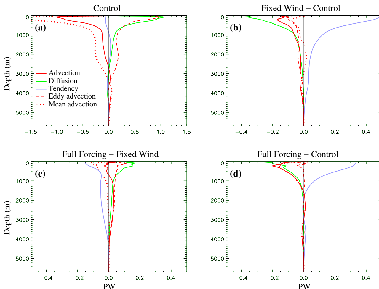
Figure 8. Global vertical heat transport (positive upward, except for the tendency) in (a) Control and its changes, (b) Fixed Wind relative to Control, (c) Full Forcing relative to Fixed Wind, and (d) Full Forcing relative to Control due to the net resolved advection (“Advection” = -\int_{-H}^z \int_{\Omega} A_z d\Omega dz = \overline{w\bar{c}} ) and the combined effect of all subgrid-scale processes (“Diffusion” = -\int_{-H}^z \int_{\Omega} \mathcal{D} d\Omega dz ). Also shown is the rate of heat content change below level z (“Tendency” = \int_{-H}^z \int_{\Omega} \frac{\Delta C}{\Delta t} d\Omega dz , where H is the depth of the ocean and \Omega is the ocean area). In addition, the “Advection” is decomposed into the contributions arising due to the time average temperature and velocity (“Mean advection” = \int_{-H}^z \int_{\Omega} A_z^M d\Omega dz = \int_{-H}^z \int_{\Omega} \overline{w\bar{c}} d\Omega dz ) and due to transient motions (“Eddy advection” = -\int_{-H}^z \int_{\Omega} A_z^E d\Omega dz = \int_{-H}^z \int_{\Omega} \overline{w'\bar{c}'} d\Omega dz , with the prime representing a deviation from the corresponding time-mean quantity). Note the difference in the scale between Figure 8a and Figures 8b–8d.
