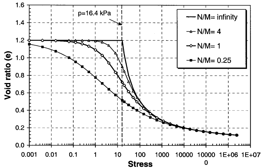
Figure 7-9 The effects of N/M on the compression curve when MN is a constant (Eq. 7-9 and Eq. 7-13)
