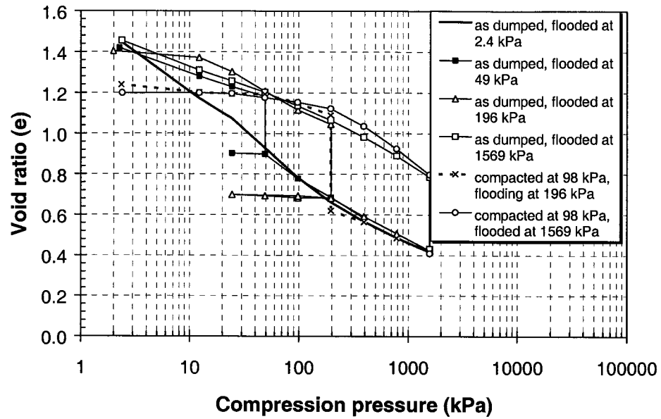
Figure 6-19 Compression curves of air-dried samples with different loading-wetting sequences
