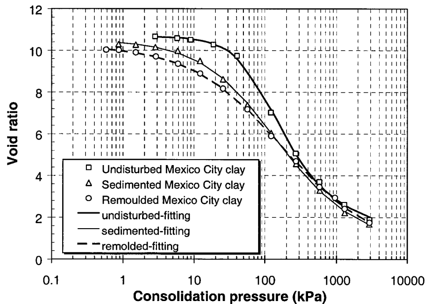
Figure 7-14 Fitting structured Mexico City clay by proposed Equation 7-9 (Mesri et al. 1975)
