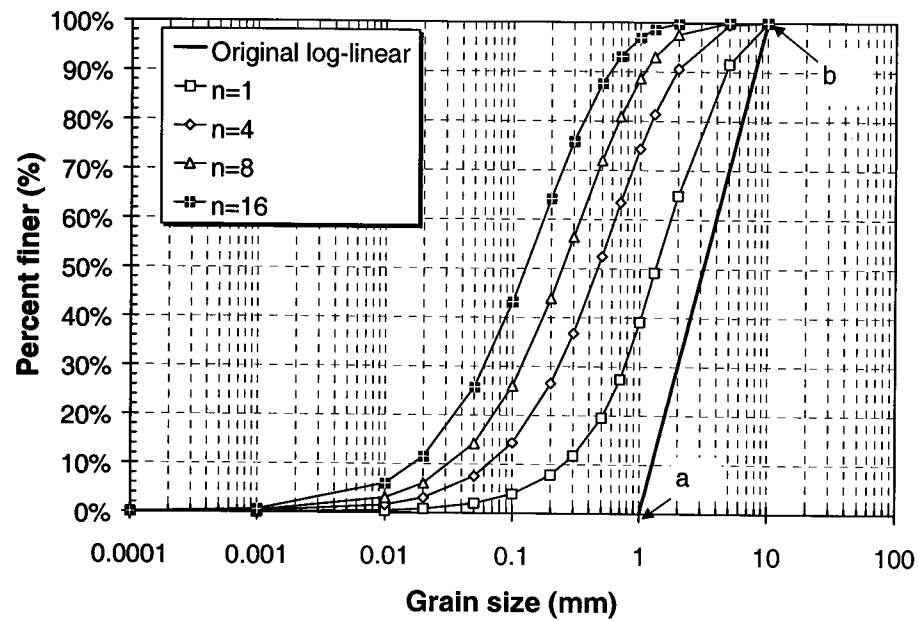
Figure 5-2 Evolution of particle size distributions from an original log-linear distribution curve
