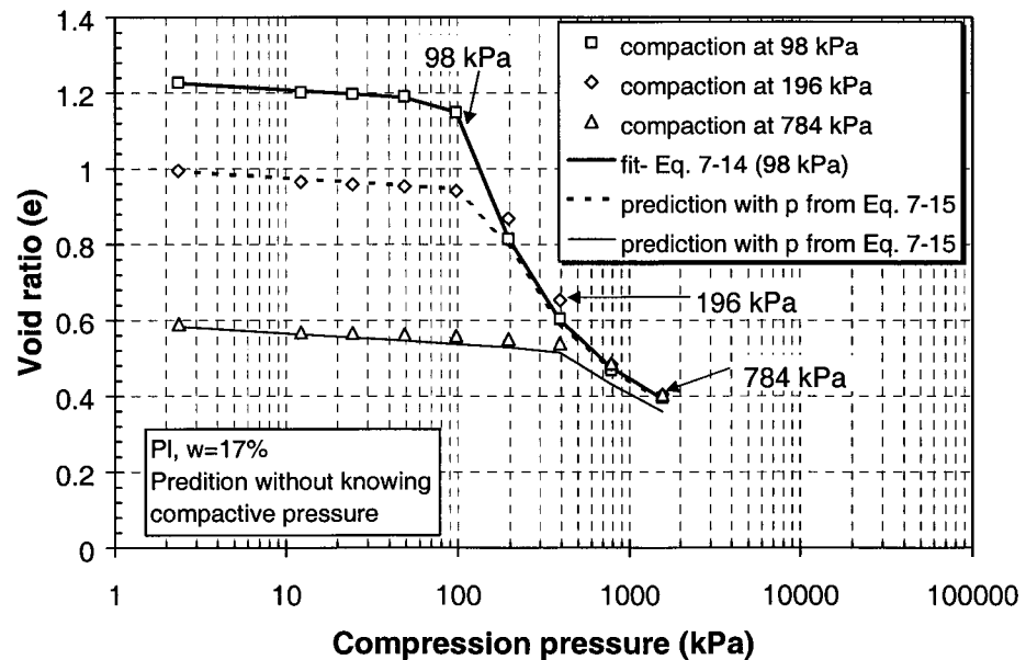
Figure 7-21 The prediction of compression curves for P_1 -17% without knowing the previous compactive pressure
