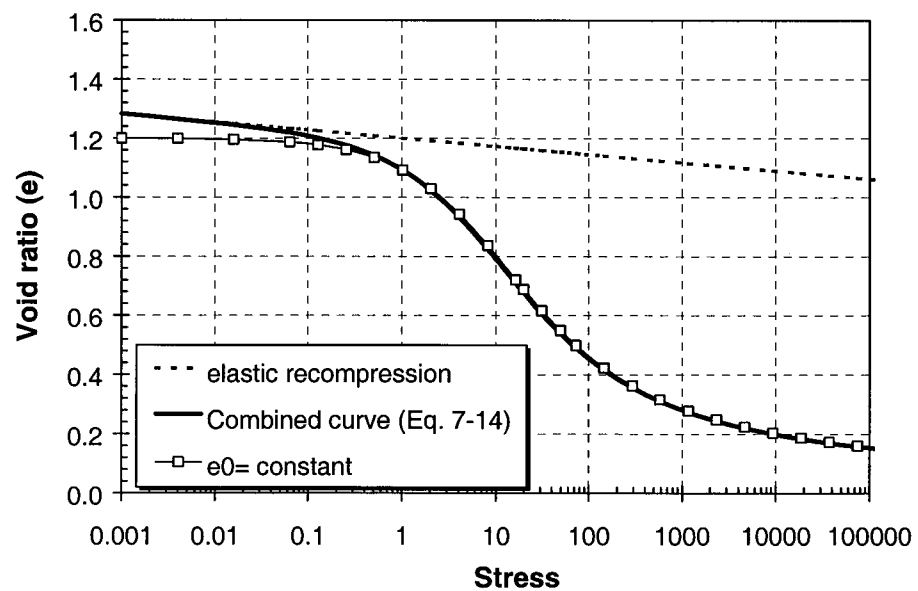
Figure 7-10 The compression curve with consideration of elastic recompression effects (Eq. 7-14 and Eq. 7-9)
