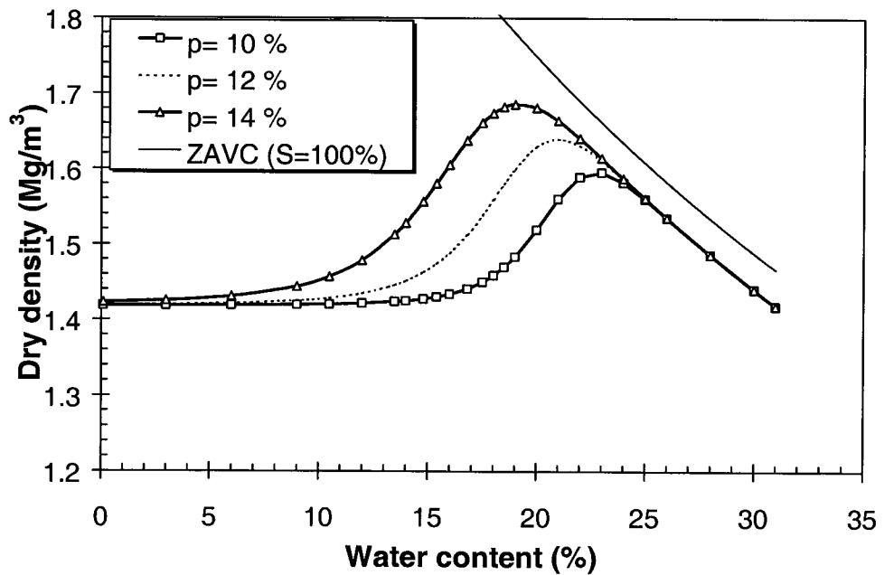
Figure 2-11 Effect of parameter p on compaction curves ( S_m = 93\% , w_m = 31\% , and n = 9 )
