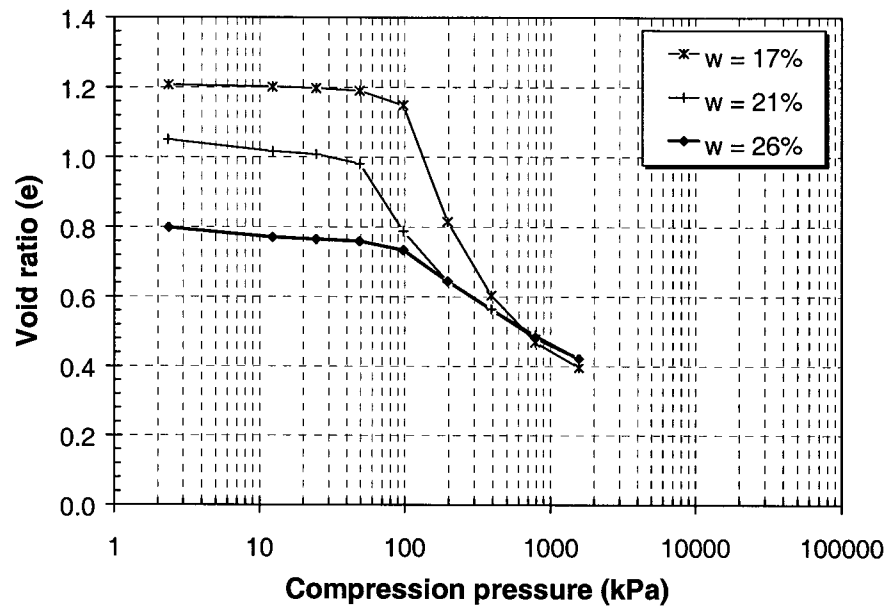
Figure 6-8 Compression curves of compacted soil prepared with water content at transition zone (between CST and OWC)
