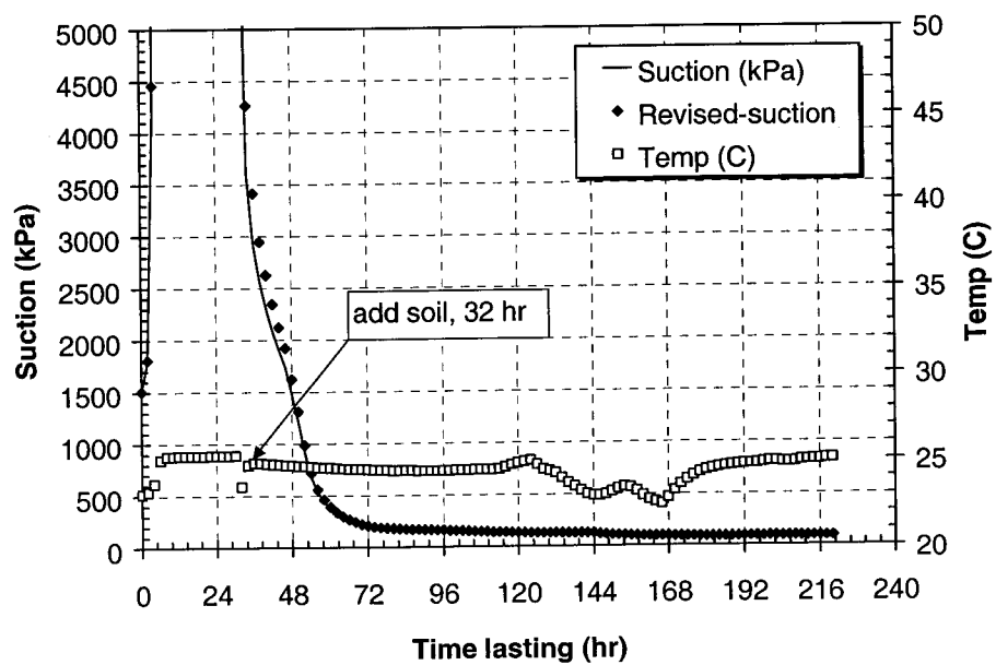
Figure A- 11 The suction measurement of lacustrine clay (P 1 ): sample suc-P2l-24%- a4
