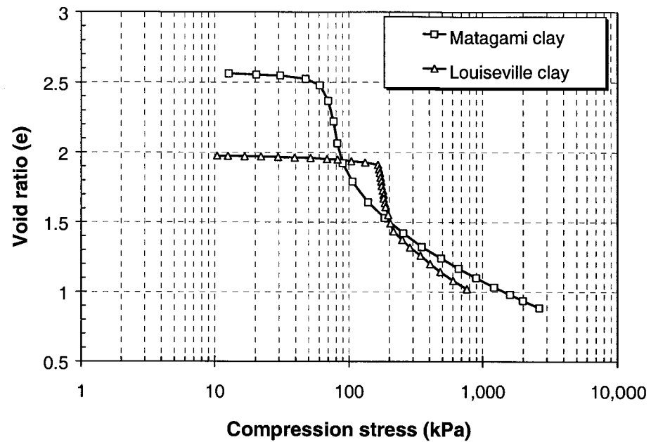
Figure 7-18 The consolidation curve of two Eastern Canadian marine clays (Tavenas et al. 1981)
