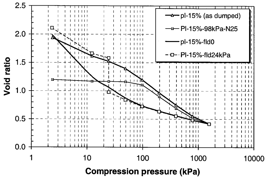
Figure 6-16 Compression curves of various samples prepared with water content at 17% (sample identification as Fig. 6-13)
