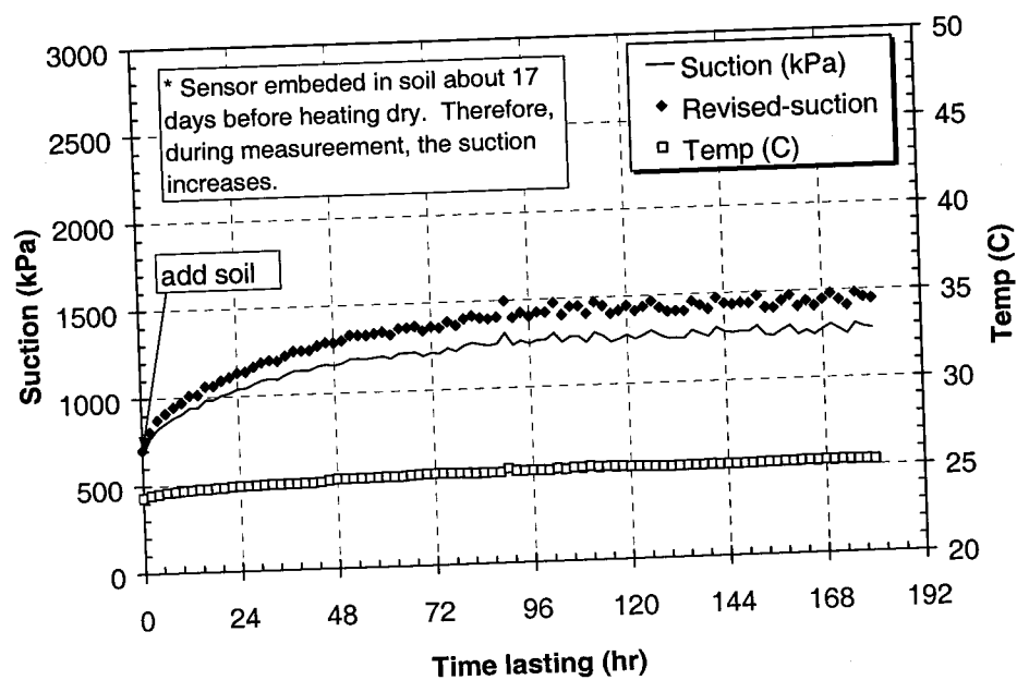
Figure A- 9 The suction measurement of lacustrine clay (P 1 ): sample suc-P2l-14%- a2
