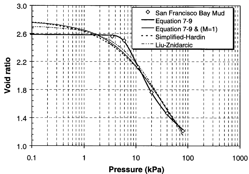
Figure 7-12 Fitting over consolidated San Francisco Bay Mud by equations from proposed Equation 7-9 with or without M = 1 , simplified Hardin (1989), and Liu-Znidarcic (Holtz and Kovacs 1981)
