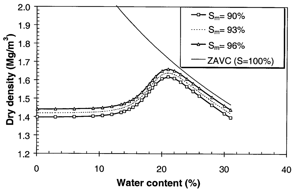
Figure 2-5 Effect of parameter S_m on compaction curves ( w_m=31\% , n=9 , and p=12\% )
