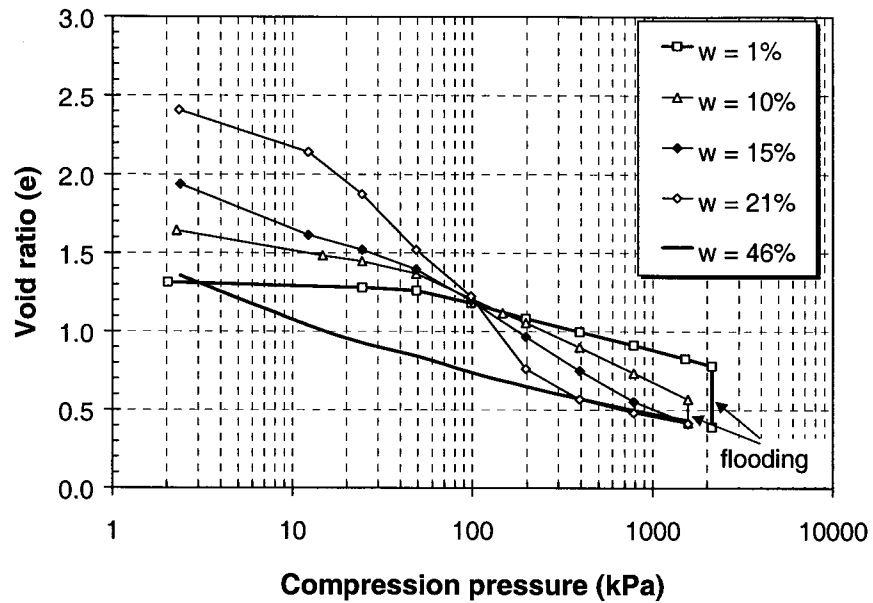
Figure 6-2 Compression curves of as-dumped soils prepared at different water content
