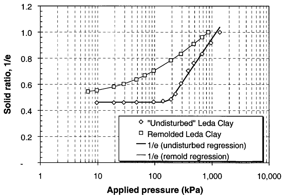
Figure 7-17 The curve of solid ratio ( 1/e ) versus stress of Canadian marine clay - Leda clay (Quigley and Thompson 1966)
