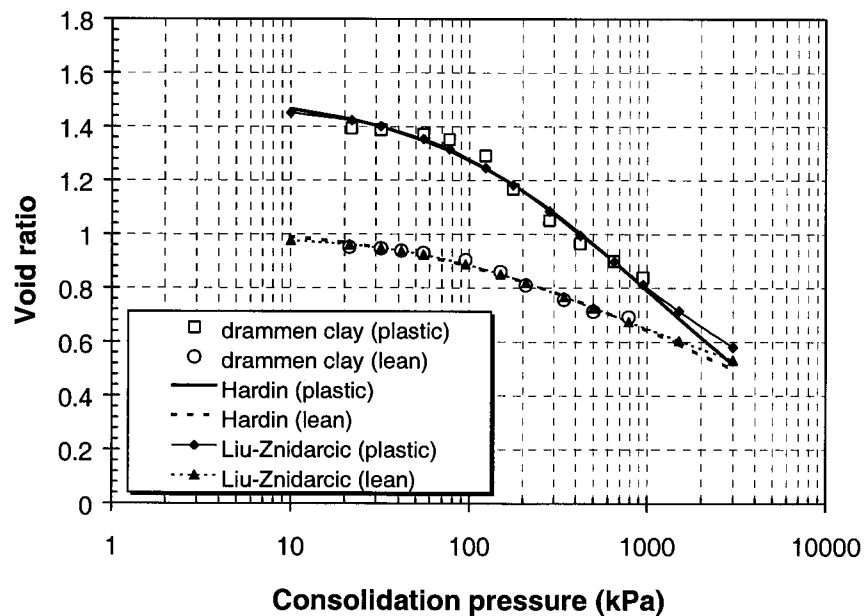
Figure 7-2 The fitting curves by Hardin (1989) and Liu and Znidarcic (1991) on field samples of overconsolidated Drammen Clay (data from Butterfield 1979)
