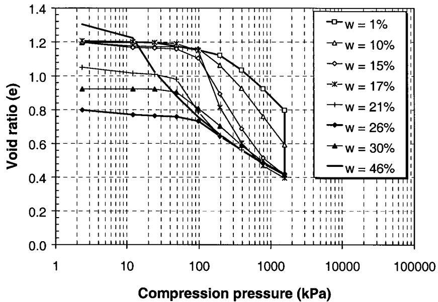
Figure 6-7 Compression curves of compacted soil prepared with water content at dry zone (dry of CST)
