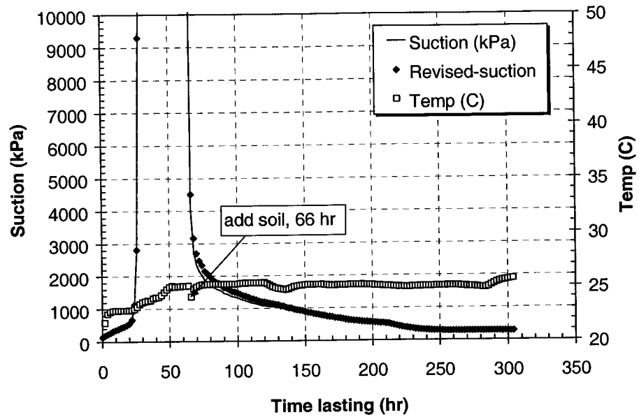
Figure A- 10 The suction measurement of lacustrine clay (P 1 ): sample suc-P2l-18%- a3
