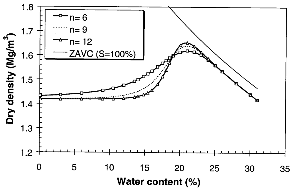
Figure 2-9 Effect of parameter n on compaction curves ( S_m = 93\% , w_m = 31\% , p = 12\% )
