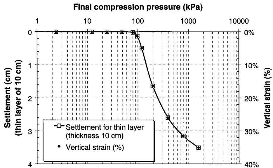
Figure 8-3 The calculated settlement and vertical strain ( \epsilon = \Delta s/H_0 ) for thin compacted layer of Pleistocene Lacustrine Clay using Equation 8-10
