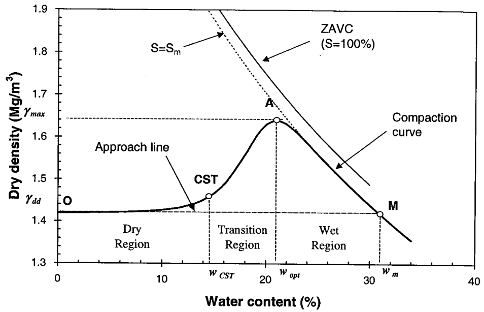
Figure 2-1 Characteristics of a typical complete compaction curve for fine-grained soils
