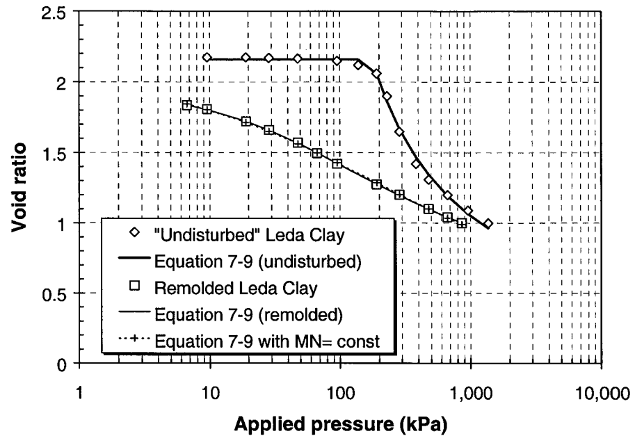
Figure 7-16 The regression of consolidation curve of Canadian marine clay - Leda clay (Quigley and Thompson 1966)
