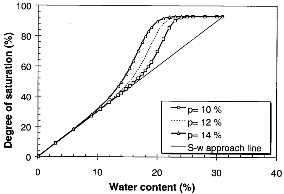
Figure 2-10 Effect of parameter p on S versus w curves ( S_m = 93\% , w_m = 31\% , and n = 9 )
