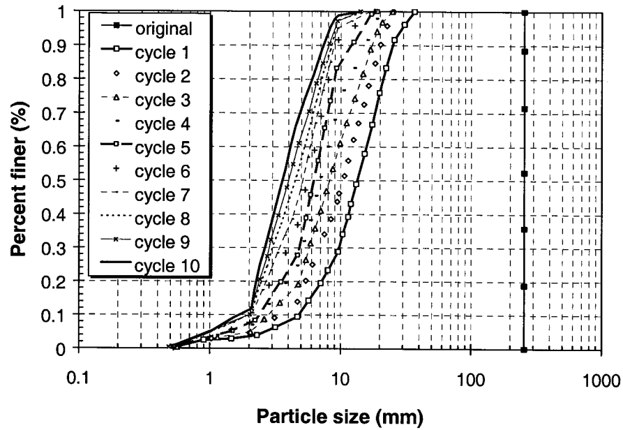
Figure 5-5 The particle size distribution of alluvial deposits in Anderson Exploration Ltd., Alberta, Canada (Sego and Li 1999)
