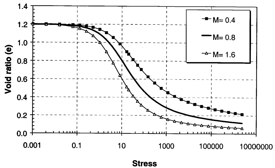
Figure 7-7 The effects of parameter M on the compression curve ( N = 0.8 ) (Eq. 7-9)
