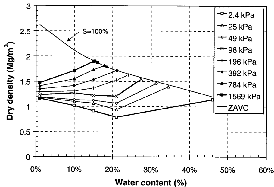
Figure 6-4 Progress of dry density as-dumped soil during one-dimensional compression test
