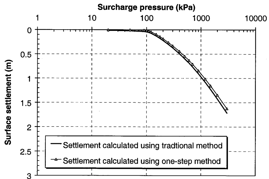
Figure 8-7 The settlement estimation for thick compacted layer (10 m) under different surcharge loading using Equation 8-12
