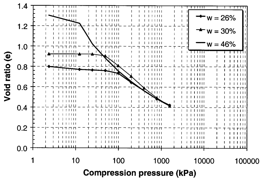
Figure 6-9 Compression curves of compacted soil prepared with water content at wet zone (wet of OWC)
