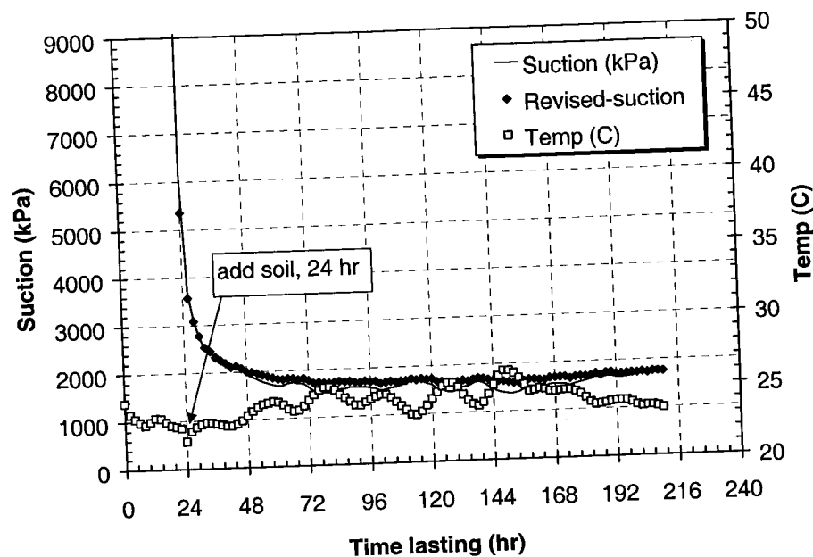
Figure A- 8 The suction measurement of lacustrine clay (P 1 ): sample suc-P2l-11%- a1
