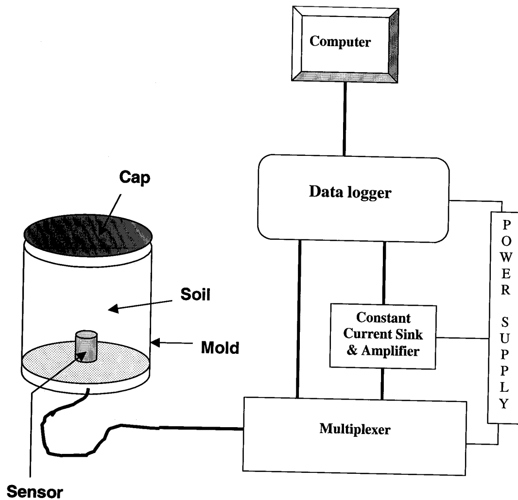
Figure 4-2 A schematic of general arrangement for measurement of matrix suction
