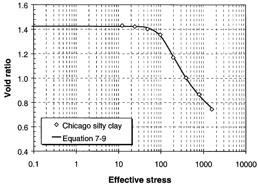
Figure 7-13 Fitting over consolidated Chicago silty clay (Taylor 1948) by proposed Equation 7-9
