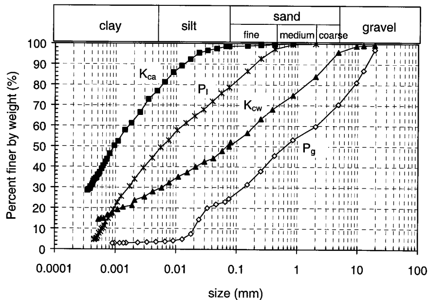
Figure 3-4 Particle size distribution of Syncrude overburden soils
