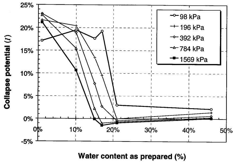
Figure 6-21 Collapse potential versus as-prepared water content under different compression pressure
