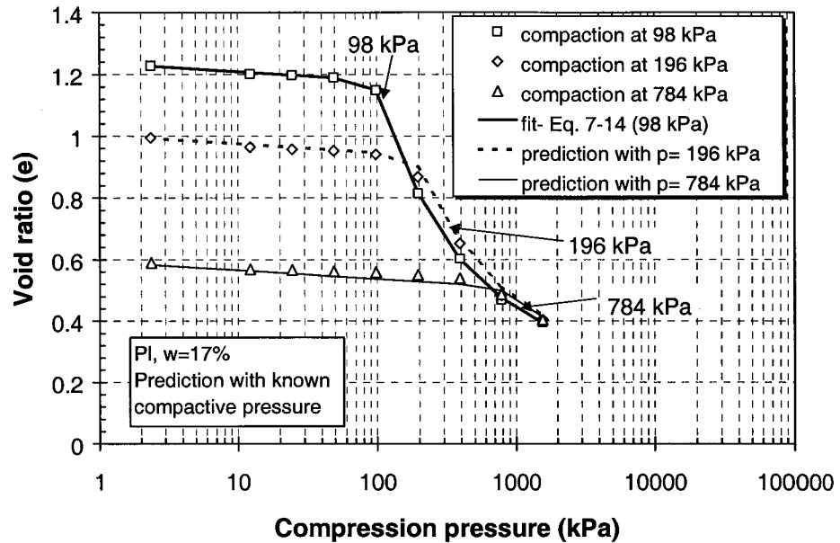
Figure 7-20 The prediction of compression curves for P_1 -17% with known previous compactive pressure
