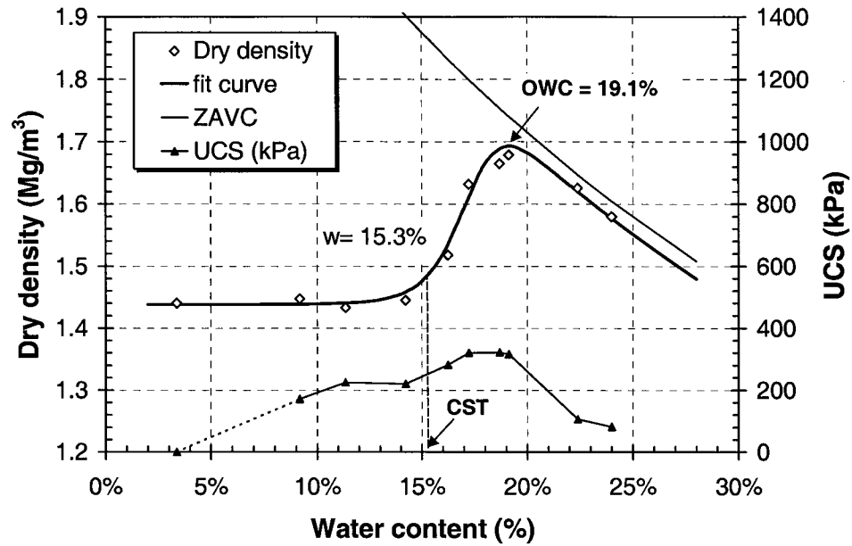
Figure 4-4 Complete compaction curve and unconfined compression strength (UCS) for glacial till ( P_g )
