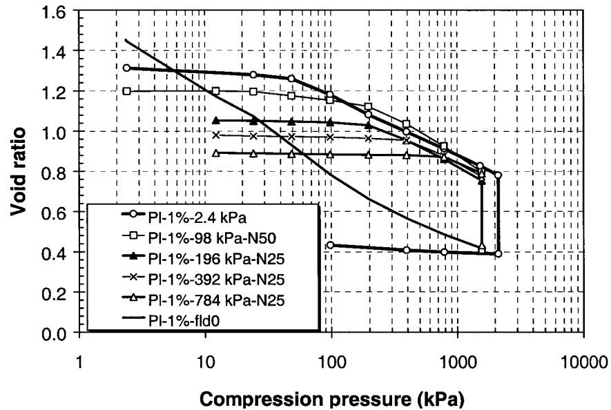
Figure 6-14 Compression curves of various samples prepared with water content at 10% (sample identification as Fig. 6-13)
