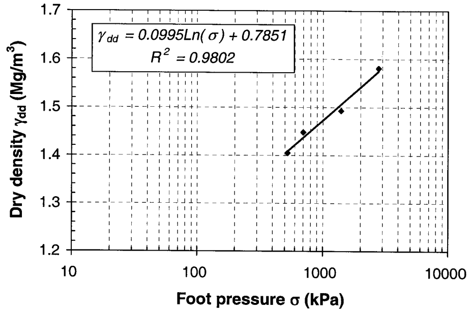
Figure 2-19 Effect of numbers of applications of 700 kPa foot pressure in kneading compaction test for as-air-dried lacustrine clay
