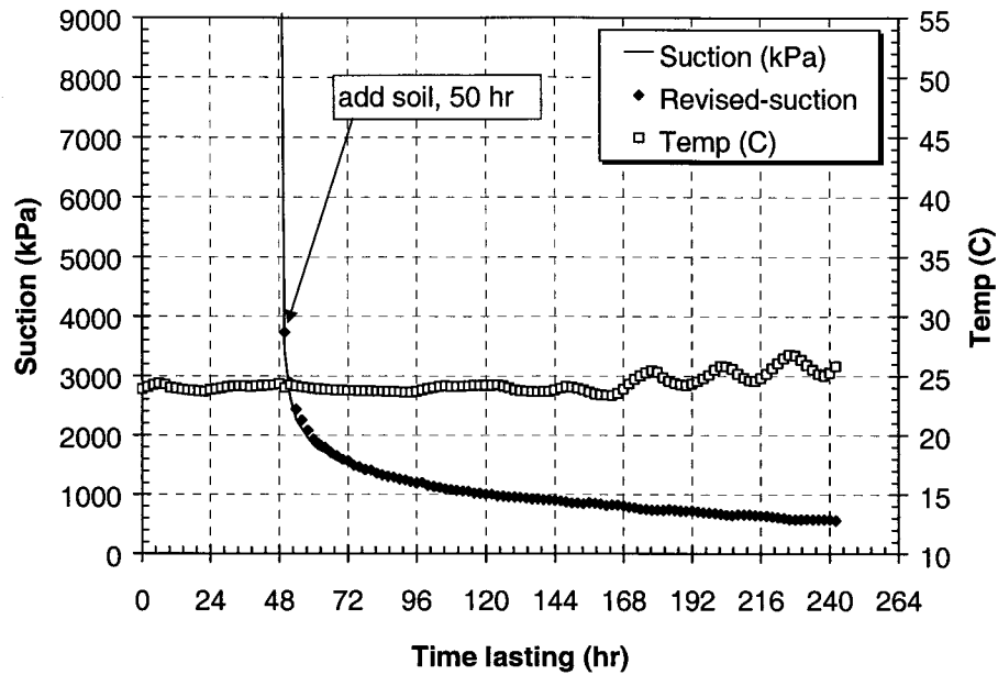
Figure A- 6 The suction measurement of glacial till ( P_g ): sample suc-P2g-9%-c3
