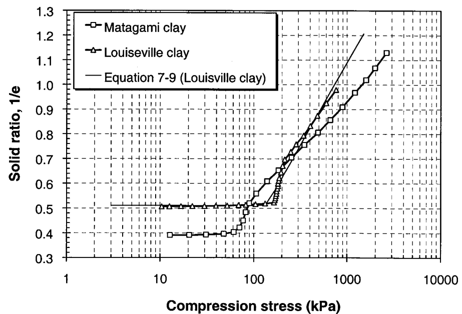
Figure 7-19 The curve of solid ratio ( 1/e ) versus stress of two Eastern Canadian marine clay (Tavenas et al. 1981)
