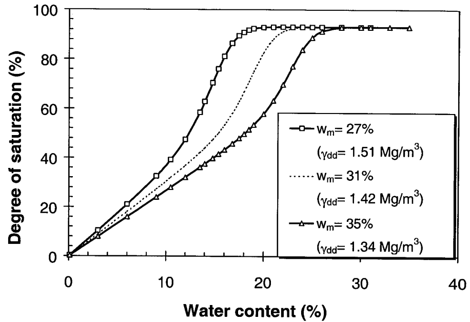
Figure 2-7 Effect of parameter w_m (or \gamma_{dd} ) on compaction curves ( S_m=93\% , n=9 and p=12\% )
