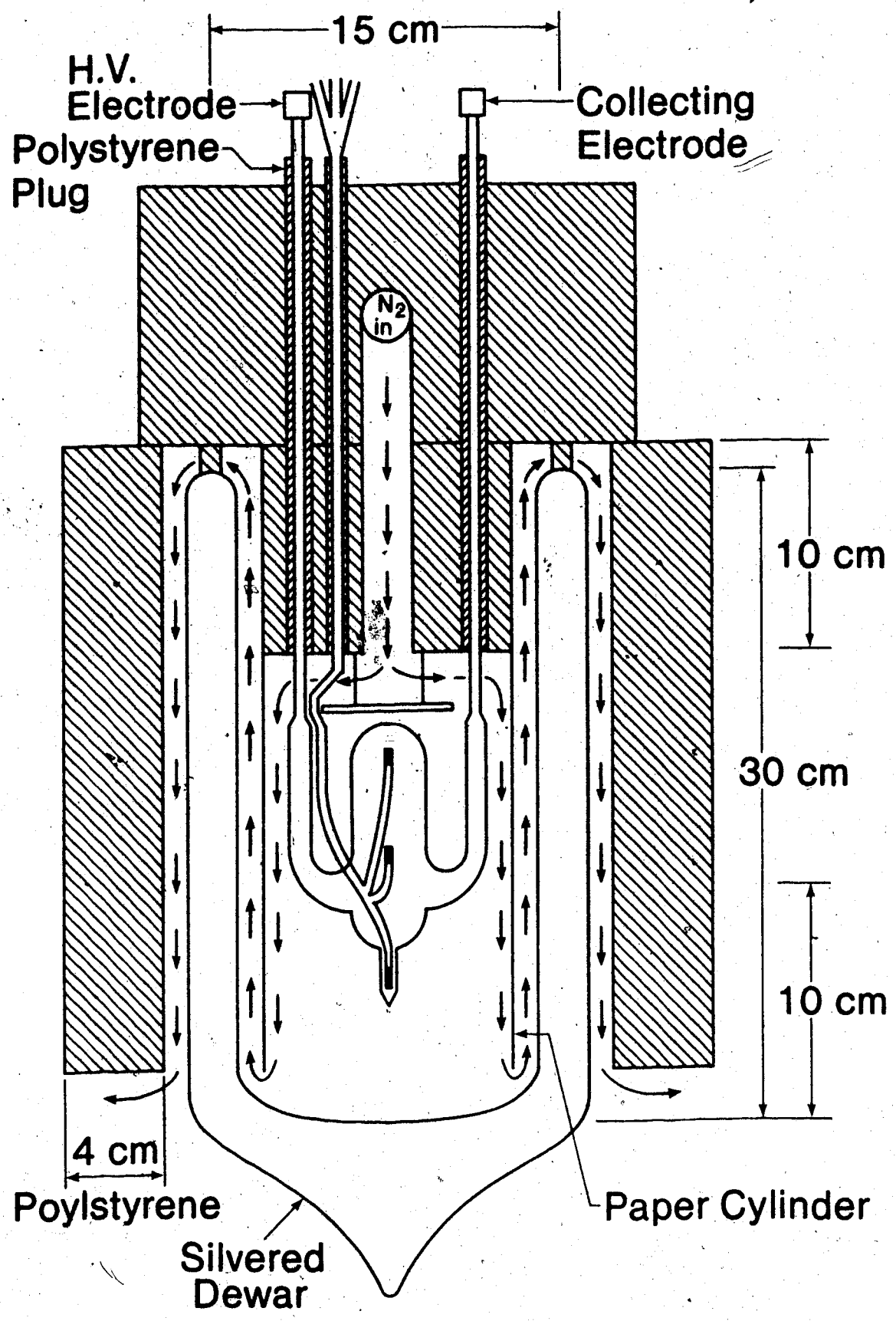
Figure II-7 Cooling Apparatus
