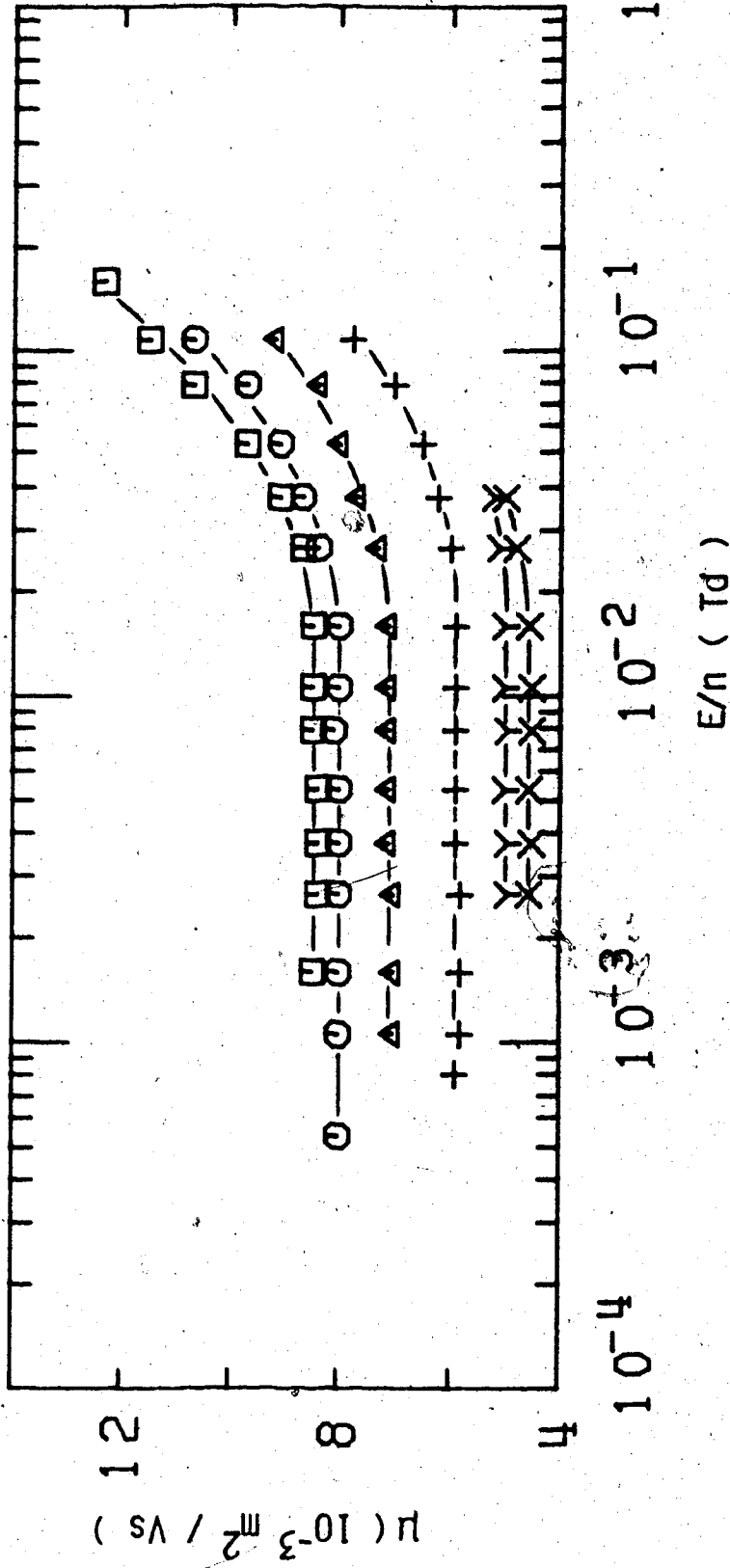
Fig. 3-11. Electron mobilities in supercritical \text{CH}_2\text{D}_2 gas at n_c = 6.1 \times 10^{27} molecules/cm 3 and different temperatures (K). X, 189.6; Y, 189.8; +, 190.5; Δ, 191.7; O, 192.9; □, 193.9. T_c = 189.2 .
