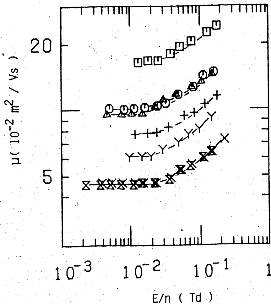
Figure III-5-4. Electron mobilities in saturated \text{CD}_4 vapor at different densities ( 10^{26} molec/ \text{m}^3 ) and temperatures (K). \square , 1.23, 119.3; \circ , 2.00, 127.0; \Delta , 2.16, 128.2; +, 2.66, 132.0; Y, 3.23, 135.7; X, 4.21, 141.0; \otimes , 4.46, 142.0.
