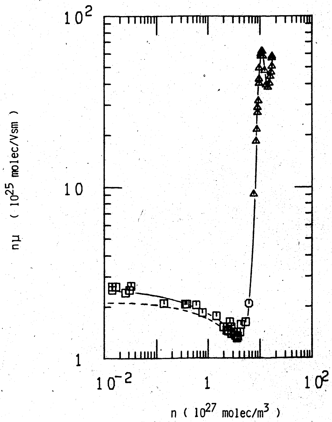
Figure IV-14. Density normalized electron mobility (low field) for thermal electrons in coexistence vapor ( \square ) and liquid ( \Delta ) CH_2D_2 . \circ represents the supercritical fluid at n_c and T_c . The dashed line is for CH_4 from Figure IV-1.
