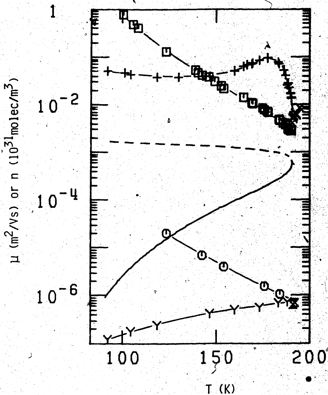
Figure IV-46. Electron and ion mobilities in coexistence vapor and liquid \text{CH}_4 as functions of temperature.
