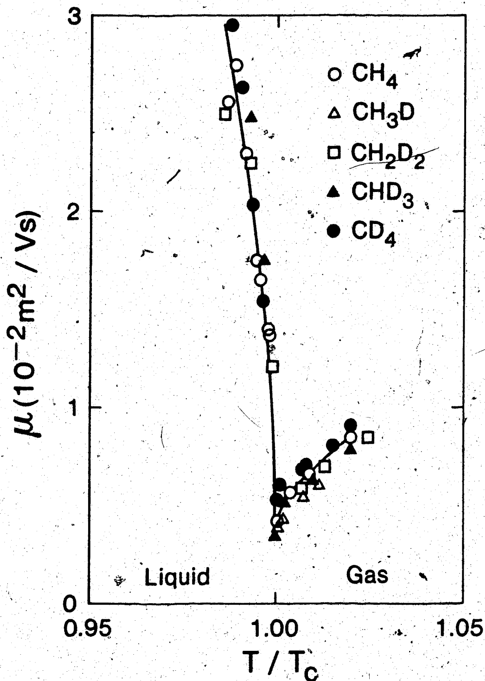
Figure IV-31. Thermal electron mobilities (low field) in coexistence liquid and supercritical methanes as functions of the reduced temperature T/T_c in the vicinity of T_c . Symbols as in Figure IV-24.
