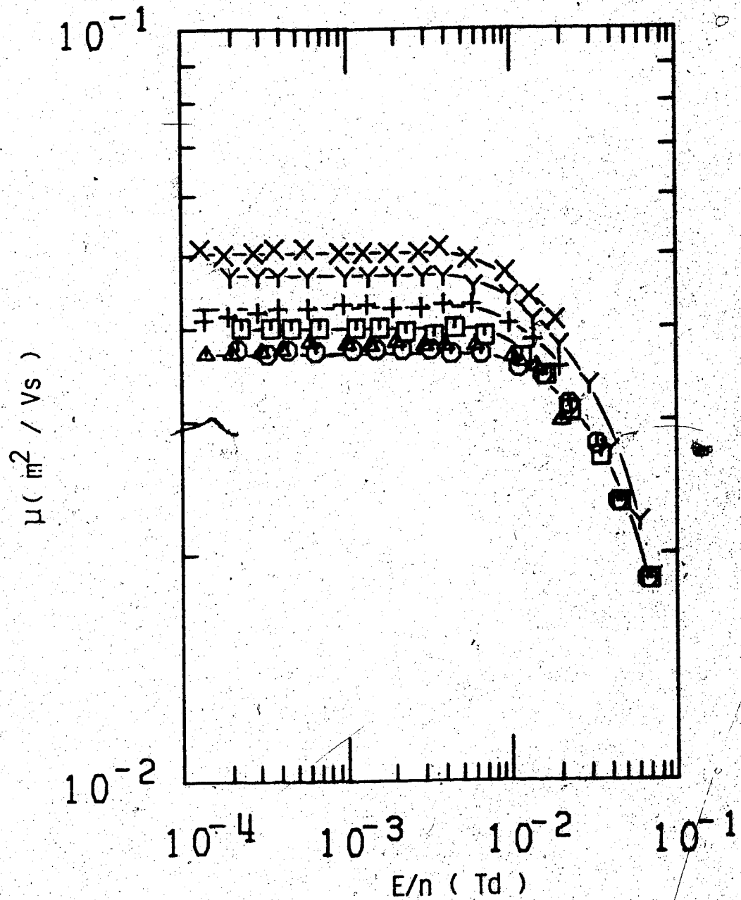
Figure III-1-17. Electron mobilities in liquid \text{CH}_4 at different densities ( 10^{27} molec/ \text{m}^3 ) and temperatures (K). \square , 14.0, 143.0; \circ , 14.7, 130.3; \Delta , 15.5, 118.5; +, 16.2, 104.5; Y, 16.4, 101.5; X, 17.0, 92.0.
