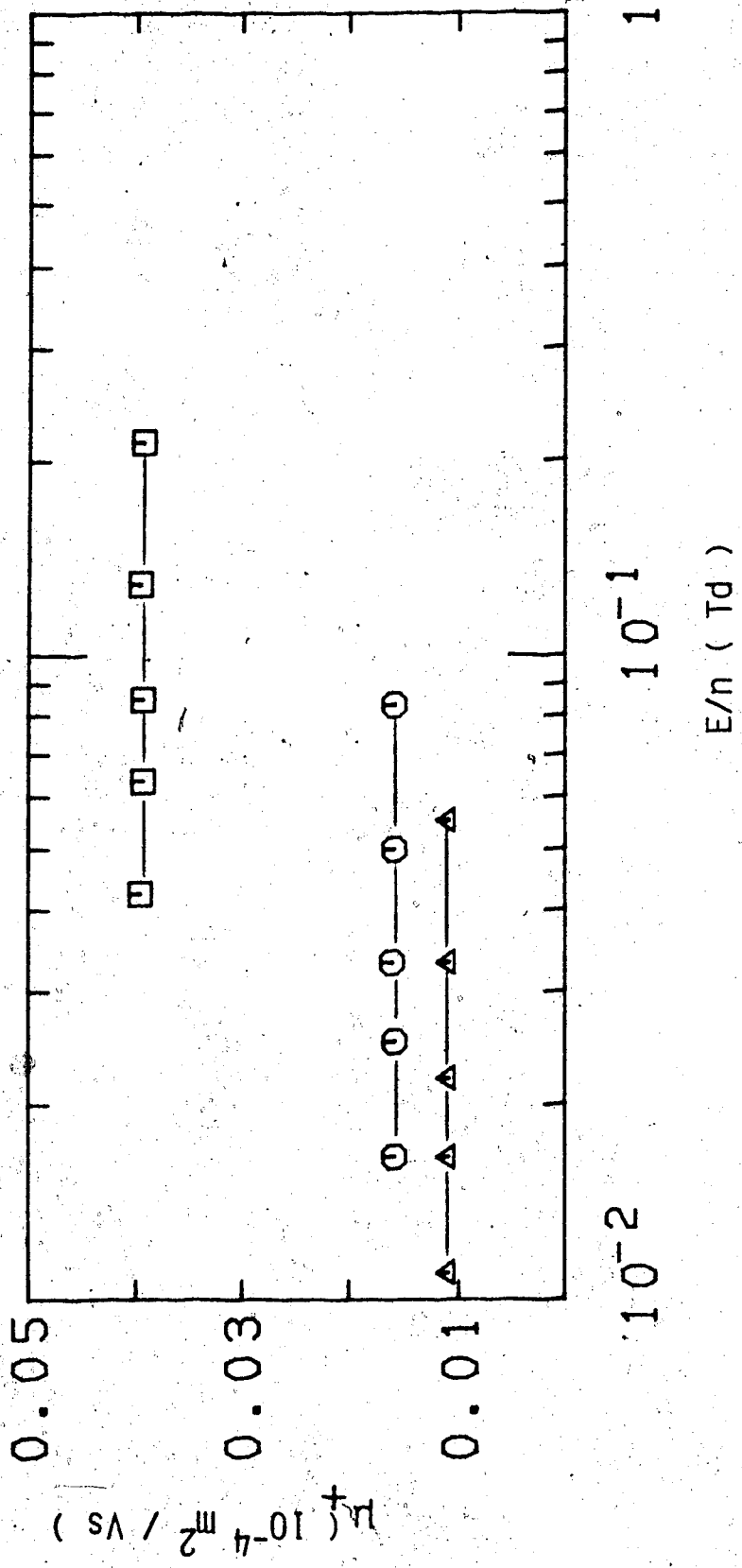
Figure III-1-23. Ion mobilities in saturated \text{CH}_4 vapor at different densities ( 10^{27} \text{ molec/m}^3 ) and temperatures (K). \square , 0.74, 154.0; \circ , 1.89, 175.7; \triangle , 2.85, 184.0.
