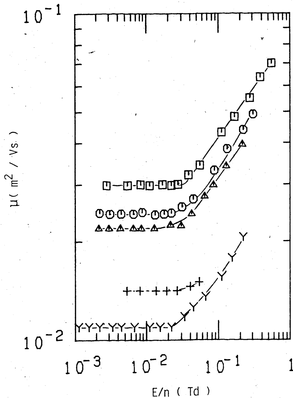
Figure III-1-8. Electron mobilities in saturated \text{CH}_4 vapor at different densities ( 10^{26} \text{ molec/m}^3 ) and temperatures (K). \square , 5.7, 149.0; \circ , 7.0, 152.8; \triangle , 7.4, 154.0; + , 11.7, 164.6; Y , 14.2, 169.1.
