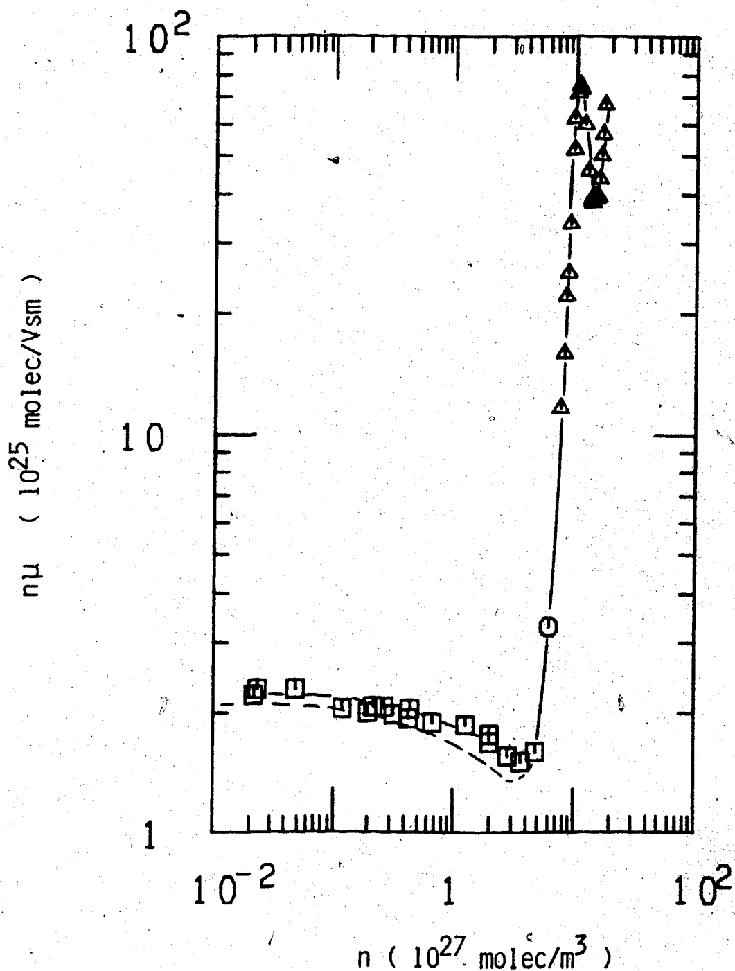
Figure IV-16. Density normalized mobilities (low field) against n for thermal electrons in coexistence vapor ( \square ) and liquid ( \Delta ) \text{CD}_4 . \circ represents the supercritical fluid at n_c and T_c + 0.1\text{K} . The dashed line is for \text{CH}_4 from Figure IV-1.
