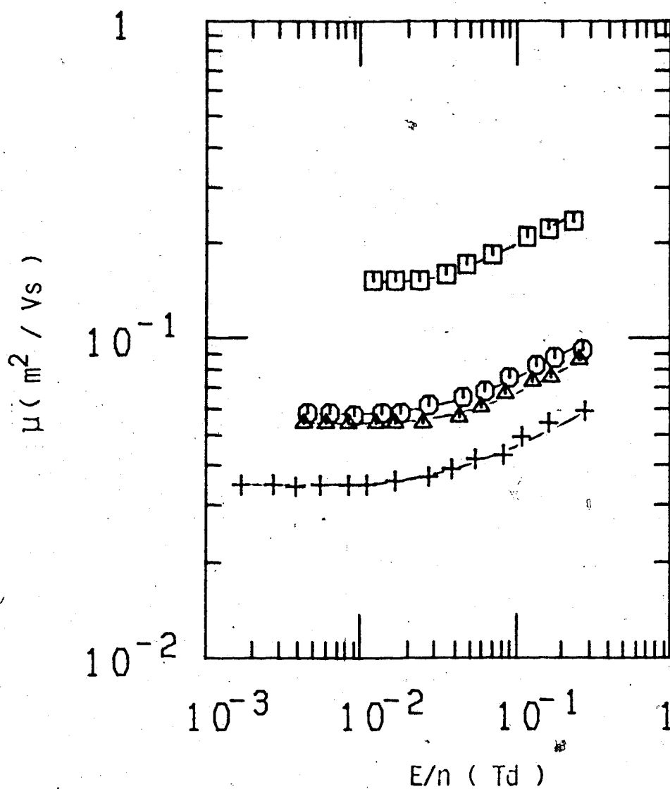
Figure III-3-4. Electron mobilities in saturated \text{CH}_2\text{D}_2 vapor at different densities ( 10^{26} molec/ \text{m}^3 ) and temperatures (K). \square , 1.37, 120.8; \circ , 3.58, 137.7; \triangle , 3.82, 139.0; + , 5.9, 147.8.
