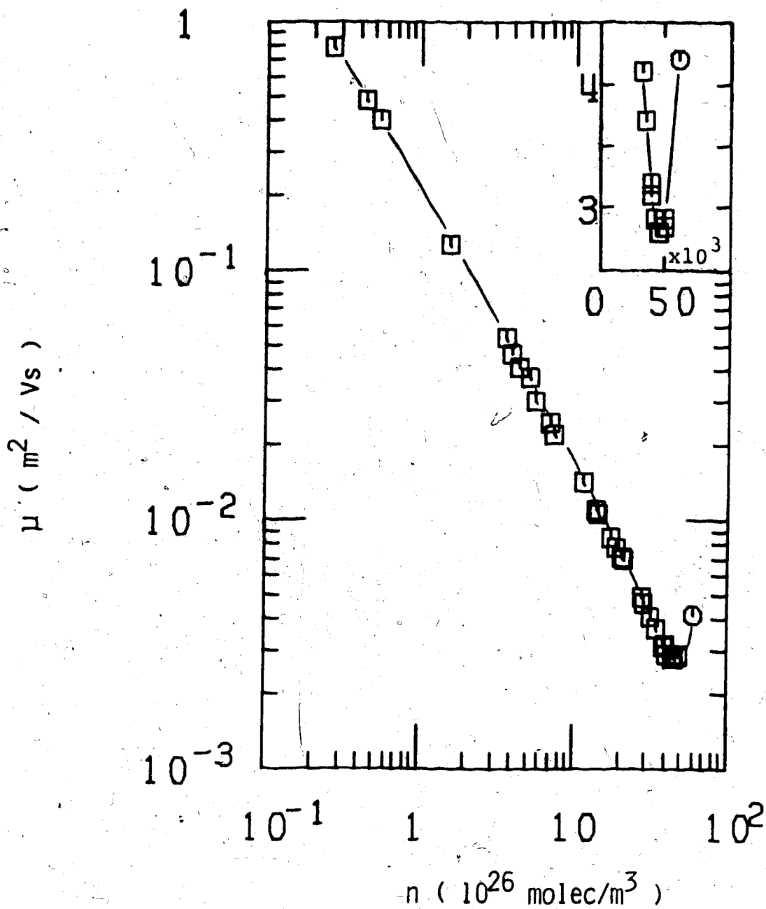
Figure IV-27. Plot of the electron mobility (low field) against the density in saturated \text{CH}_4 vapor. \circ represents the supercritical fluid at n_c and T_c + 0.1\text{K} . The insert is an expansion of the critical region. These points have been multiplied by 1000.
