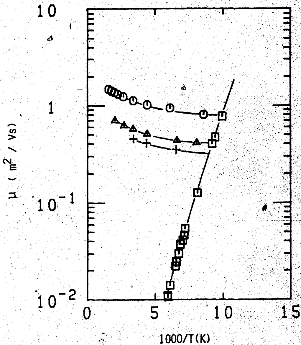
Figure IV-11. Arrhenius plot of thermal electron mobilities (low field) in \text{CH}_4 gas at different densities ( 10^{25} \text{ molec}/\text{m}^3 ). Mobilities in the gas along the vapor-liquid coexistence curve are represented by \square . \circ , 2.95; \Delta , 5.3; +, 7.5.
