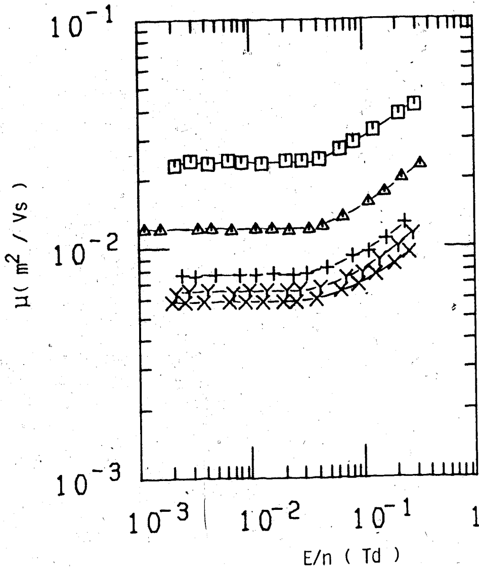
Figure III-3-7. Electron mobilities in saturated \text{CH}_2\text{D}_2 vapor at different densities ( 10^{26} molec/ \text{m}^3 ) and temperatures (K). \square , 7.7, 154.0; \Delta , 14.6, 168.9; + , 19.8, 175.3; \gamma , 22.8, 178.5; \times , 24.8, 180.1.
