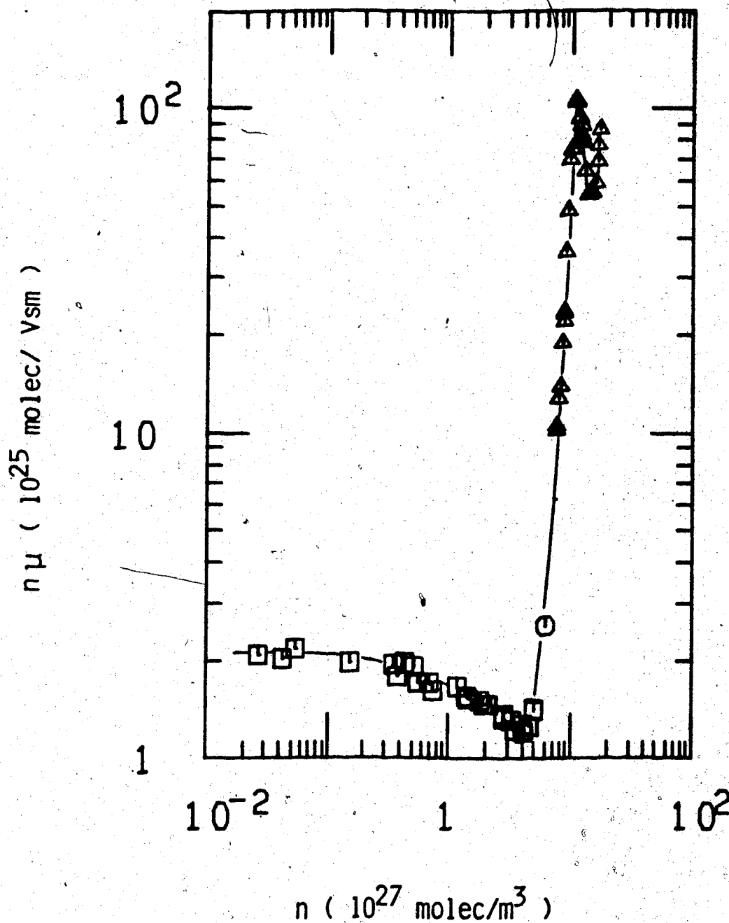
Figure IV-1. Density dependence of the density normalized electron mobility (low field) in the coexistent vapor (□) and liquid (Δ) phases of CH 4 . ○ represents the slightly supercritical fluid at n_c and T_c + 0.1K .
