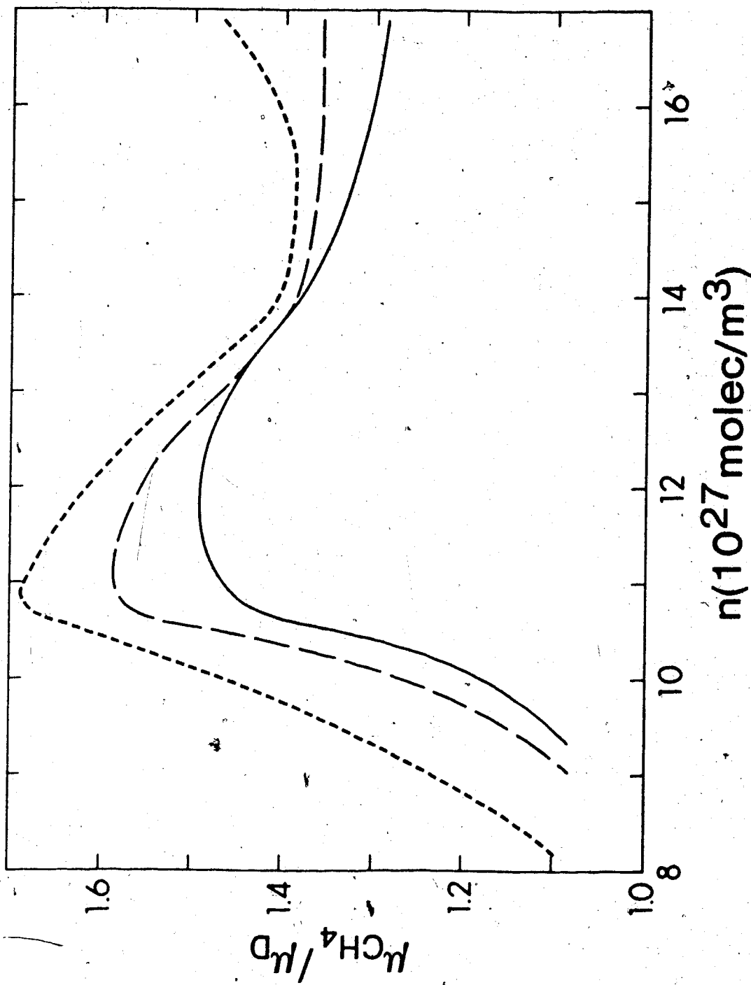
Figure IV-33. Ratios of the mobility in liquid CH_4 to that in the deuterated compounds {}^1CH_4 / {}^2H , as functions of density n . —, CHD_3 and CD_4 ; - - -, CH_3D ; ····, CH_2D_2 .
