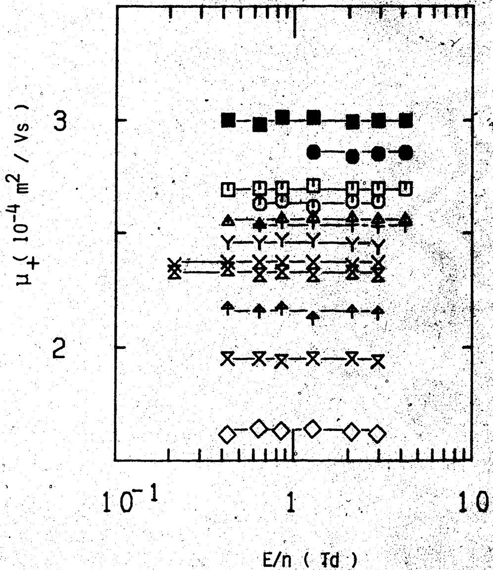
Figure III-2-21. Ion mobilities in \text{CH}_3\text{D} gas at n = 2.35 \times 10^{25} \text{ molec/m}^3 and different temperatures (K). \diamond , 108.2; \bowtie , 146.3; \uparrow , 185.5; \boxtimes , 225.7; \times , 293.7; \gamma , 337.8; + , 385.8; \triangle , 404.4; \circ , 435; \square , 474; \bullet , 504; \blacksquare , 535.
