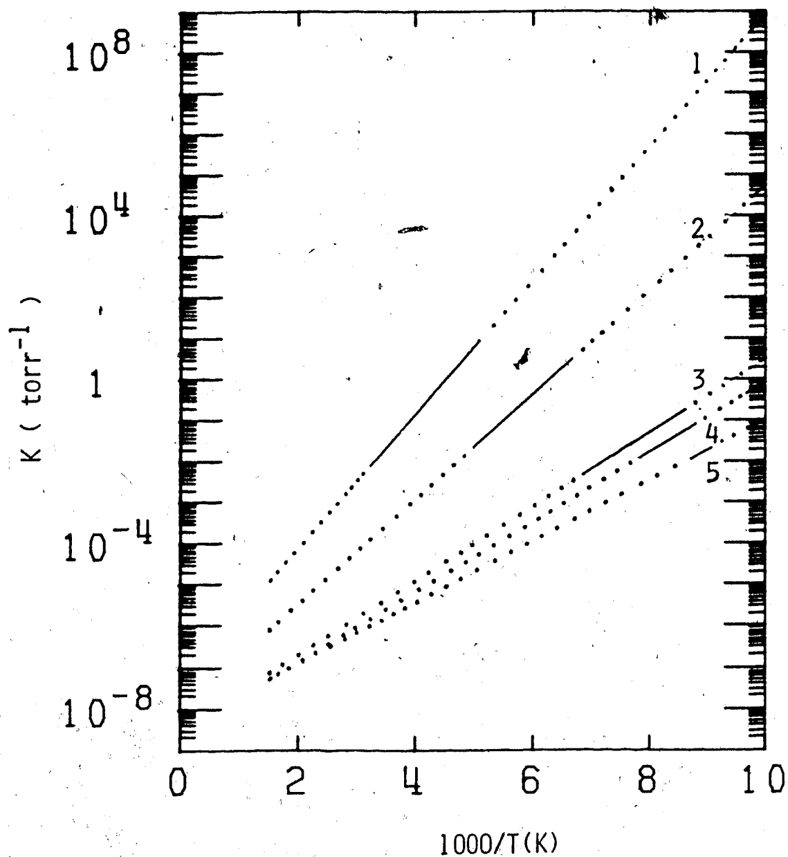
Figure IV-39. Van't Hoff plots for reactions \text{CH}_5^+(\text{CH}_4)_{m-1}^+ + \text{CH}_4 = \text{CH}_5^+(\text{CH}_4)_m . The numbers labeling the lines are values of m . The solid lines represent experimental values from Reference 202. The dotted lines represent the extrapolations used in this work.
