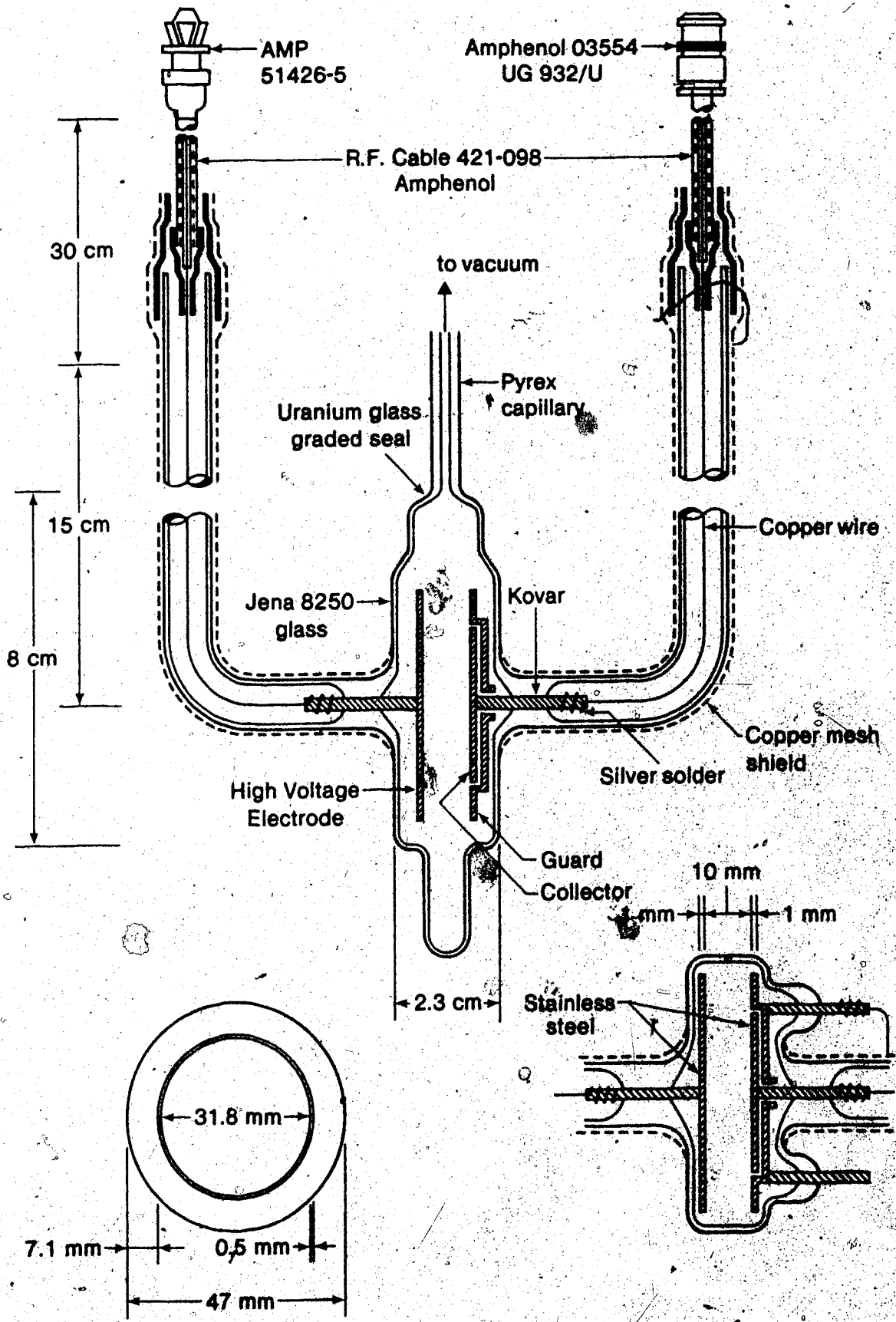
Figure II-3 Low Pressure Gas Cell
