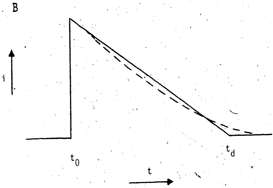
Figure II-14 A: Drift of a charge (-) between two plates at different times t_1 and t_2 . B: Idealized current transient signal. The dashed line represents space charge distortion.
