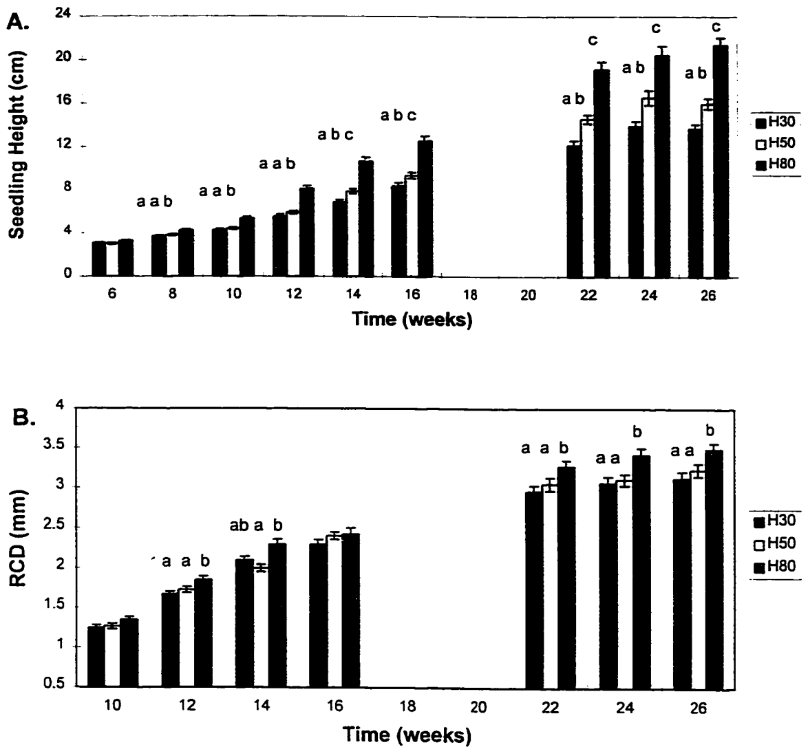
Figure 2.1. Mean shoot height (A) and RCD (B) growth of seedlings reared under 30% (H30), 50% (H50) or 80% (H80) RH. Means ( \pm SE) with the same letter are not significantly different at the 0.05 level, based on a Tukey's test; n=45 per treatment.
