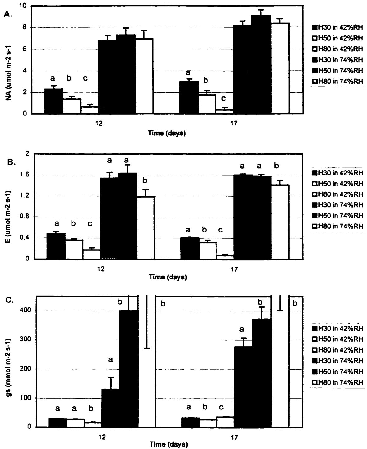
Figure 2.4. Net assimilation (A), transpiration (B) and stomatal conductance (C) of white spruce seedlings initially grown under either 30% (H30), 50% (H50) or 80% (H80) RH, then subsequently flushed and grown under 42% or 74% RH. Measurements were made 12 and 17 days after potting seedlings. Values are means ( \pm SE), and n=6 seedlings per treatment.
