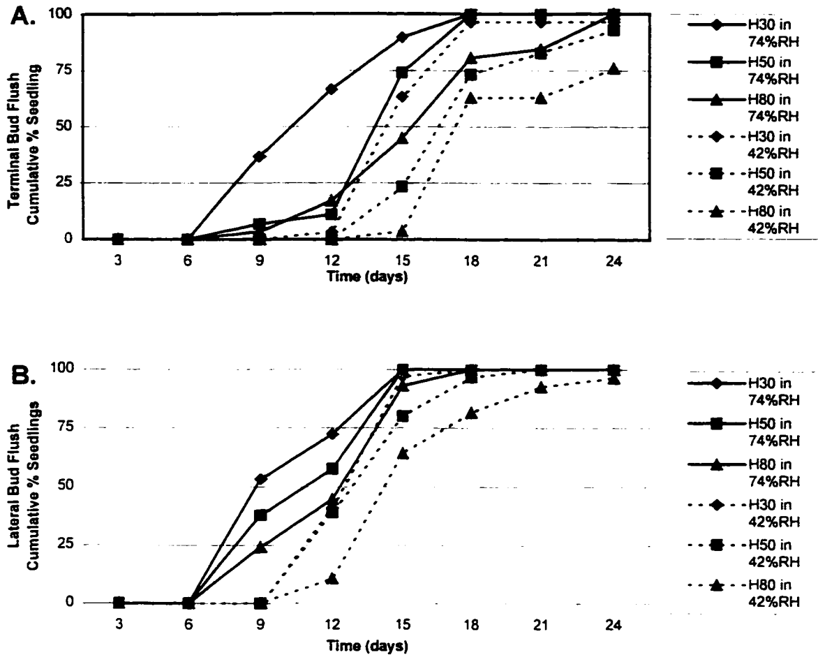
Figure 2.2. Effects of humidity on terminal (A) and lateral (B) bud flush of white spruce seedlings. The seedlings were originally grown under 30% (H30), 50% (H50) or 80% (H80) RH conditions, set dormant, then subsequently flushed under 42% RH and 74% RH. N=30 seedlings per treatment.
