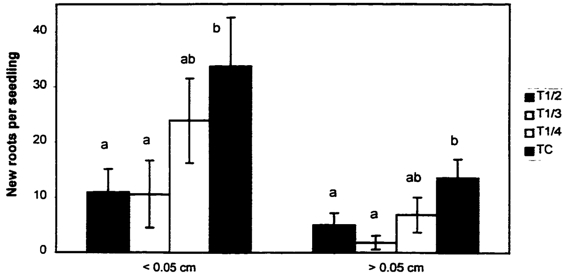
Figure 3.4. Root growth capacity of seedlings grown under one of four temperature treatments, then re-flushed under 10°C. Means ( \pm SE) are reported, n=30 seedlings per treatment. Means with the same letter within each size class are not statistically different at the 0.05 level based on a Tukey's test.
