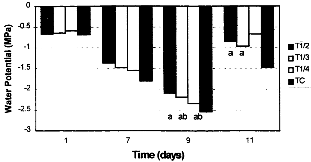
Figure 3.2 Shoot water potentials for seedlings subjected to a water stress for nine days. Seedlings were re-watered on day nine. Means ( \pm SE) are reported; n=9 seedlings per treatment. Means with the same letter on each sampling date are not statistically different at the 0.05 level based on a Tukey's test.
