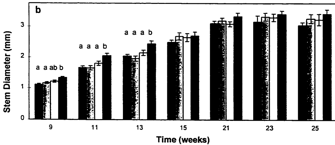
Figure 3.1. Shoot height (A) and RCD (B) of white spruce seedlings subjected to four temperature regimes. Means ( \pm SE) are reported; n=45 seedlings per treatment. Means with the same letter on each sampling date are not statistically different at the 0.05 level, based on a Tukey's test.
