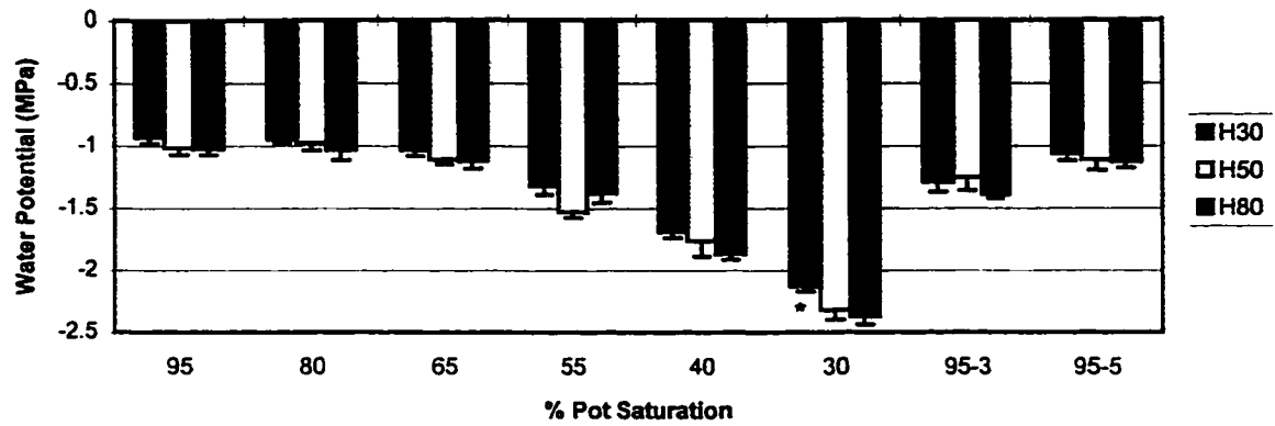
Figure 2.3 Shoot xylem water potentials in 21-week-old seedlings during a water stress experiment. Recovery from drought is indicated three days after re-watering (95-3) and five days after watering (95-5). Values are mean ( \pm SE); n=6 seedlings per treatment. * indicates significance at the 0.05 level based on a Tukey's test.
