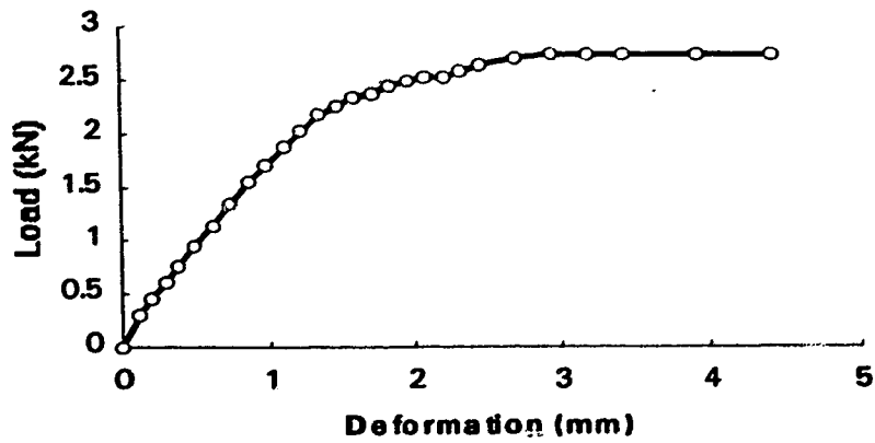
Figure 2.7(b) Compression test load-deflection curve, specimen S16
