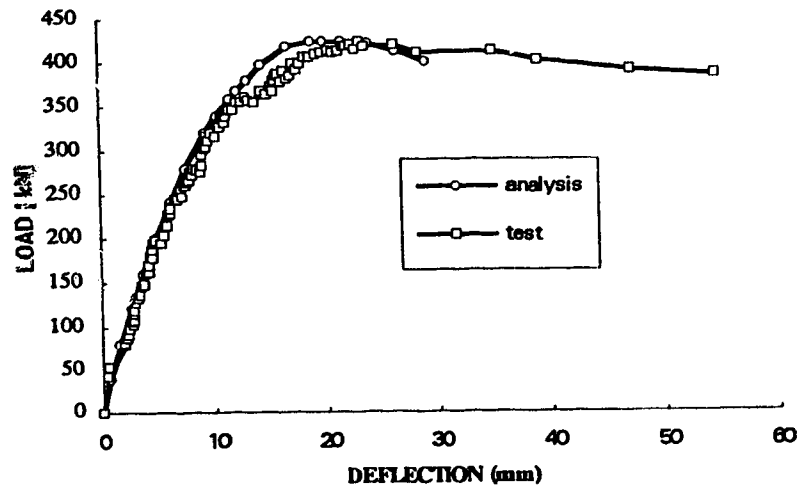
Figure 4.5 Mid-height deflection of specimen W7
