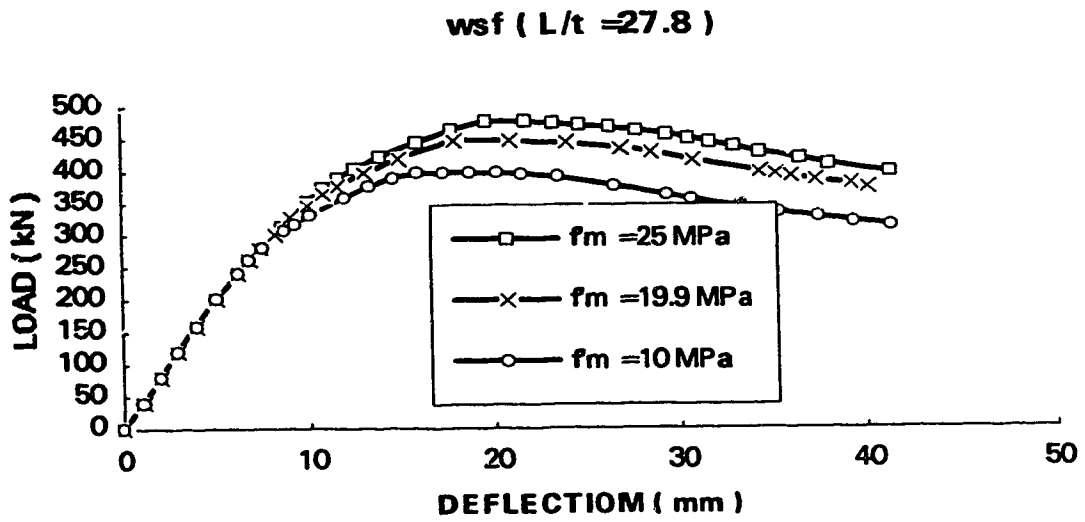
Figure 5.4 Load-deflection curves of specimens WSF1, WSF2, and WSF3
