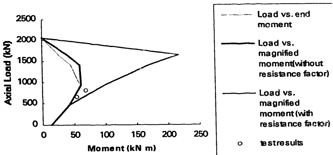
Figure 6.9(d) Comparison of proposed approach to test results
