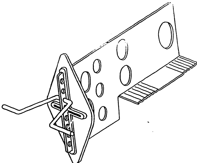
Figure 2.1 Shear connector (Courtesy K.Papanikolas)
