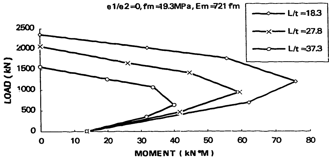
Figure 6.2 (b) Slender wall interaction diagram
