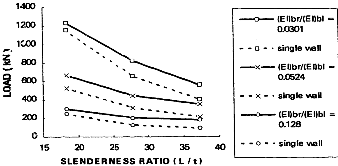
Figure 6.6 Effect of the ratio of (EI)_{brick}/(EI)_{block}
