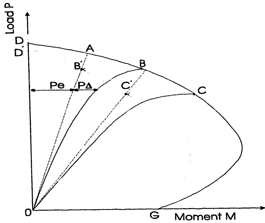
Figure 6.1 Interaction diagram
