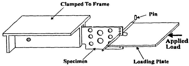
Figure 2.6(a) Compression test set-up
