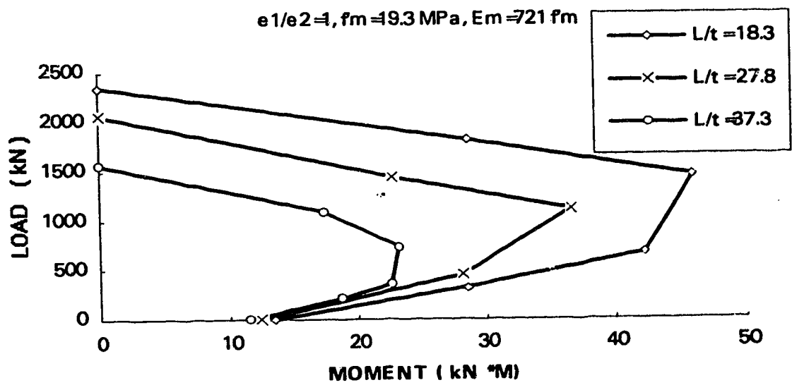
Figure 6.2 (a) Slender wall interaction diagram
