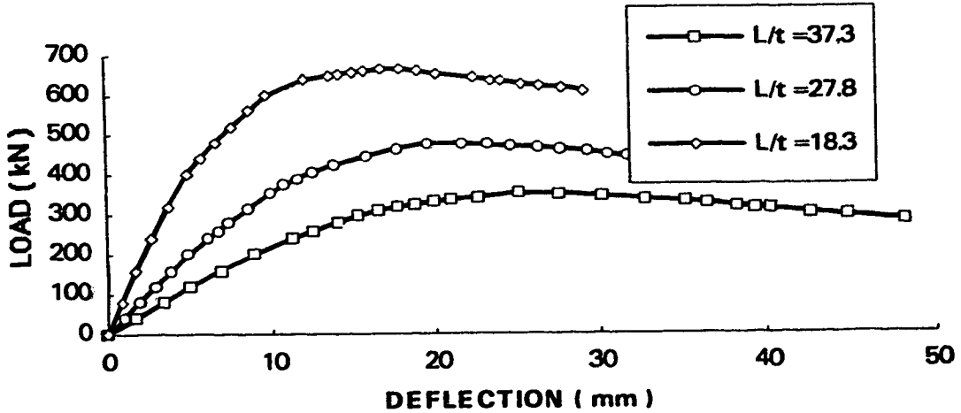
Figure 5.2 Load deflection curves of specimens WSL3, WS5, and WSS1
