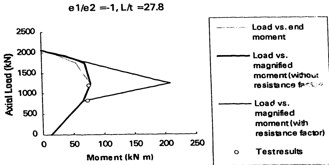
Figure 6.9(e) Comparison of proposed approach to test results
