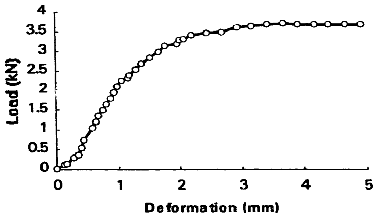
Figure 2.7(a) Tension test load-deflection curve, specimen S3
