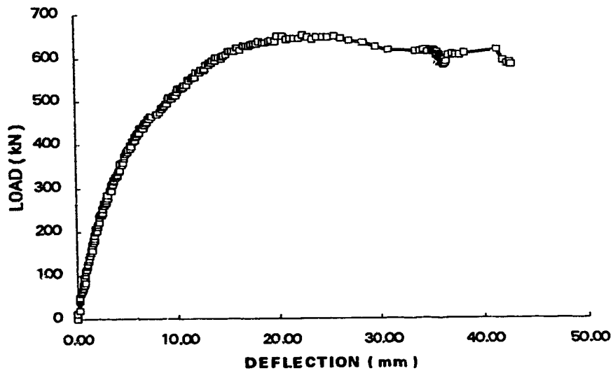
Figure 3.8 Load vs. mid-height deflection of specimen W3
