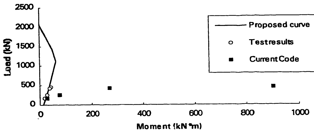
Figure 6.9(c) Comparison of proposed approach ( \phi_c = 0.65 ) to the current Code CAN3-304.1-94 and test results
