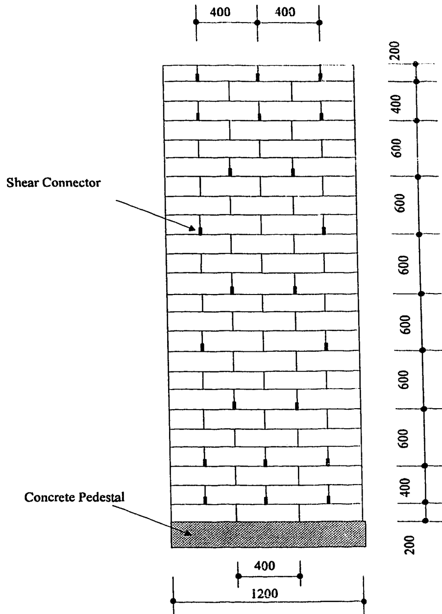
Figure 3.3 The pattern of placement of the shear connectors
