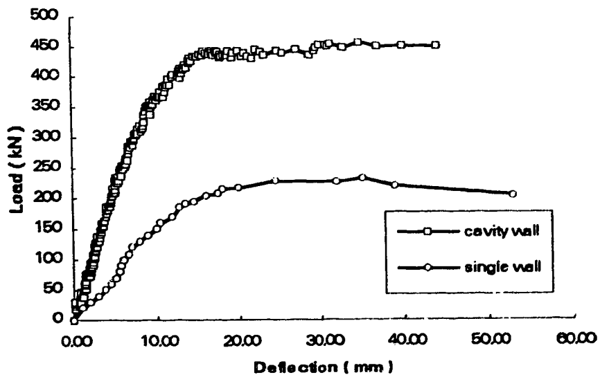
Figure 3.6 Load - deflection curves of single and cavity walls of W1
