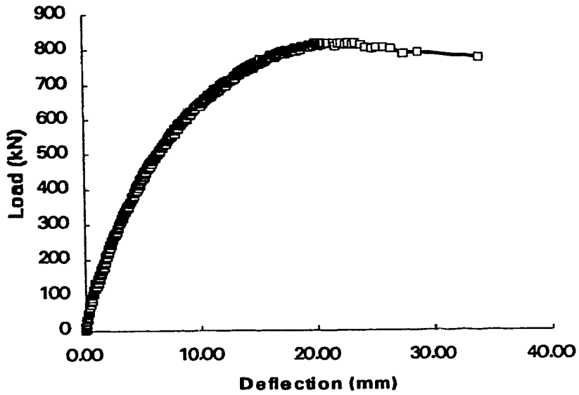
Figure 3.7 Load vs. mid-height deflection of specimen W2
