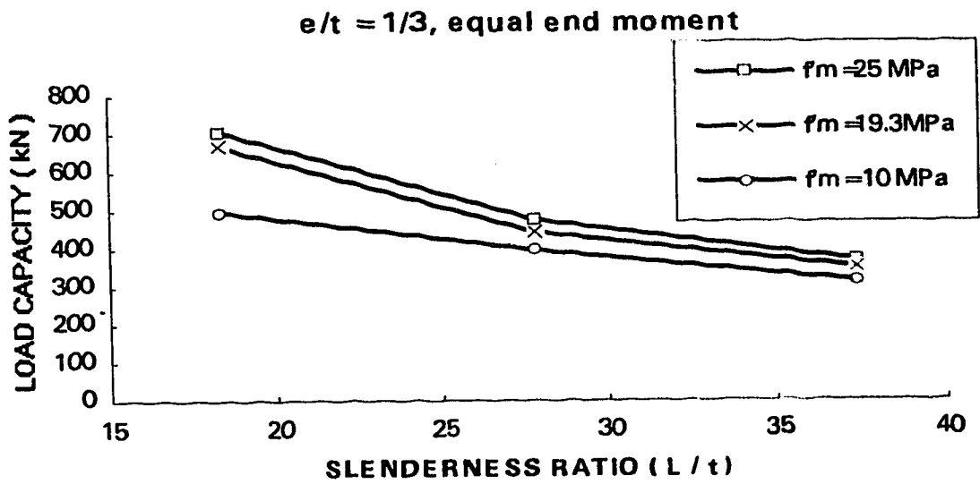
Figure 6.4 Effect of block strength
