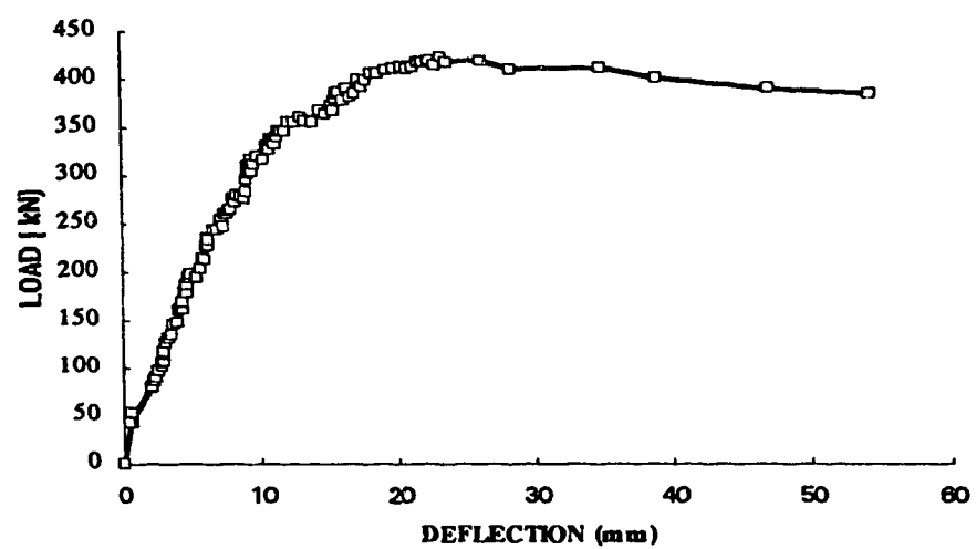
Figure 3.12 Load vs. mid-height deflection of specimen W7
