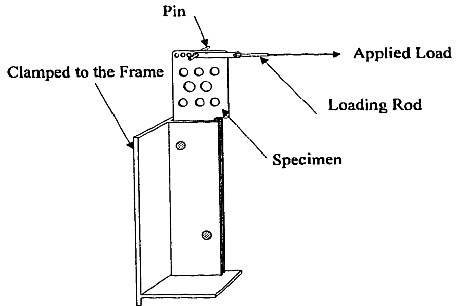
Figure 2.6 (b) Shear test set-up
