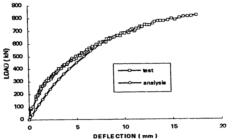
Figure 4.11 Relative displacement between height = 0.88 m and height = 4.4 m of specimen W9
