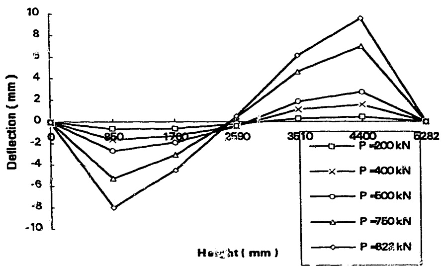
Figure 3.13 Deflected shape of specimen W9
