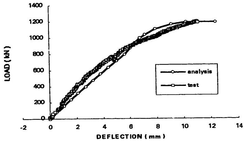
Figure 4.10 Relative displacement between height = 0.88 m and height = 4.4 m of specimen W4
