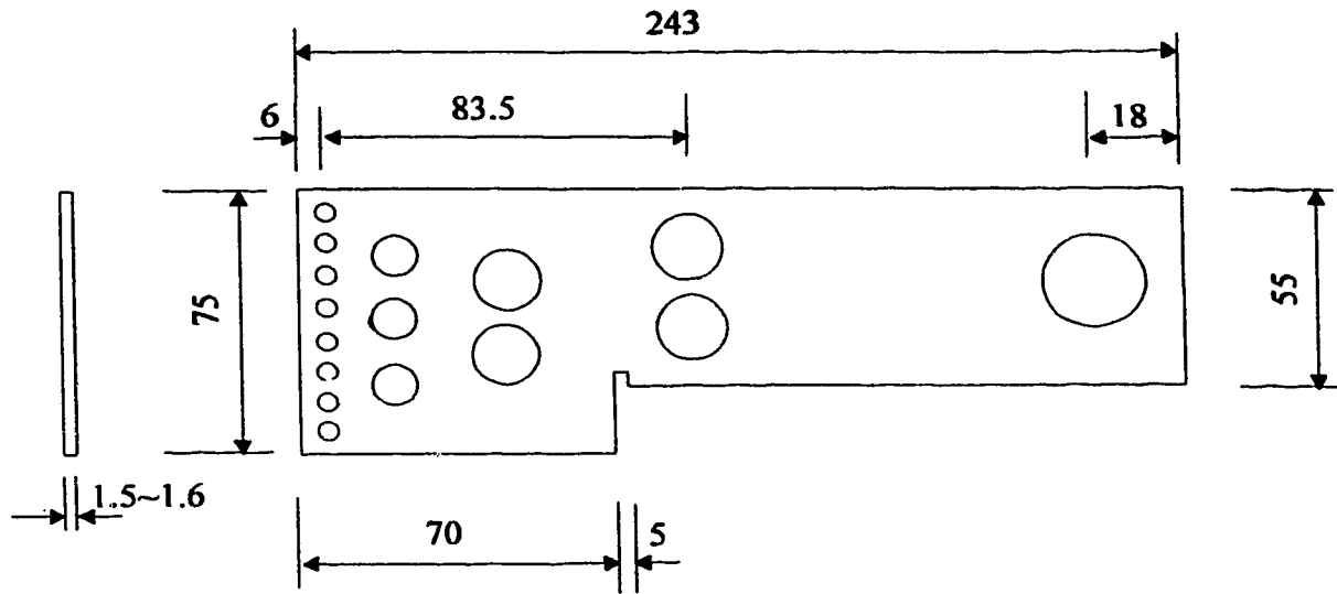
Figure 2.3 (a) Shear connector for 75 mm cavity
