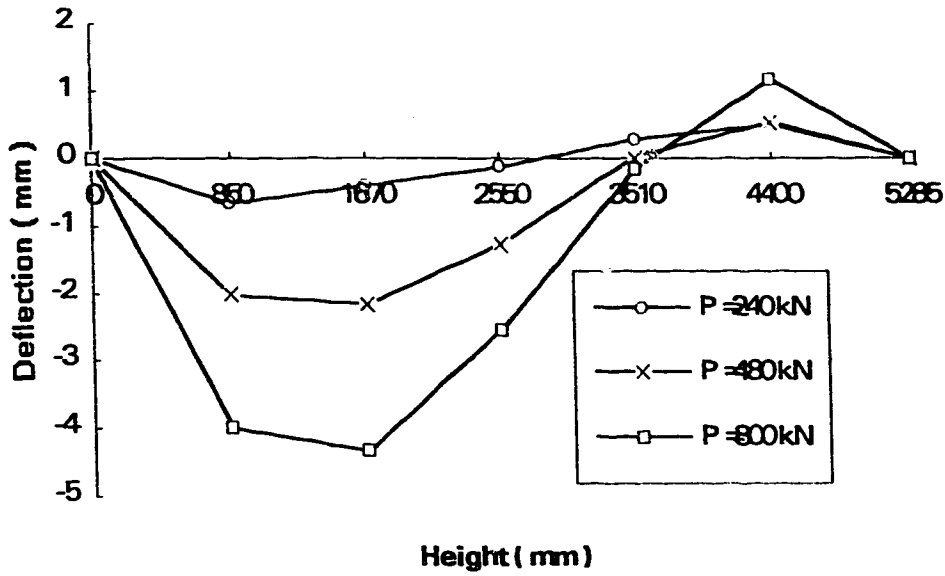
Figure 3.9 ( a ) Deflected shapes of specimen W4 ( P \leq 800 kN )
