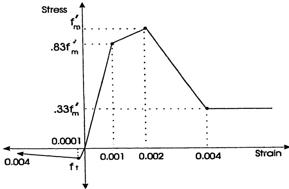
Figure 4.2 Stress-strain curve for masonry
