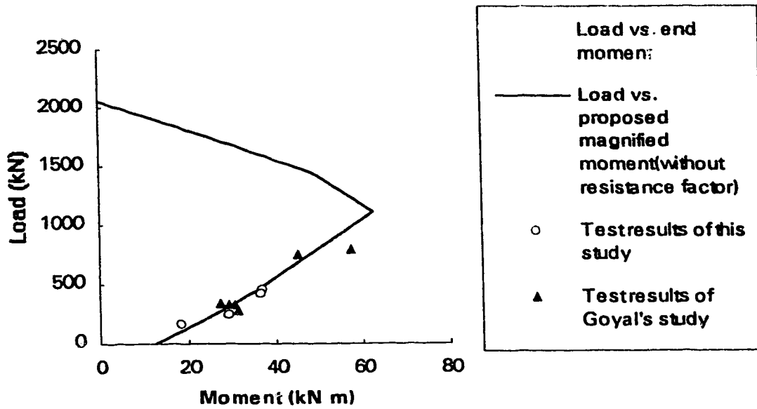
Figure 6.9(a) Comparison of proposed approach ( \phi_e = 1.0 ) to test results
