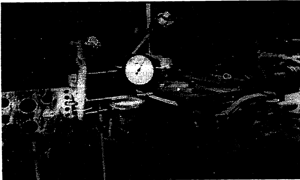
Plate 2.1 Tension test set-up
