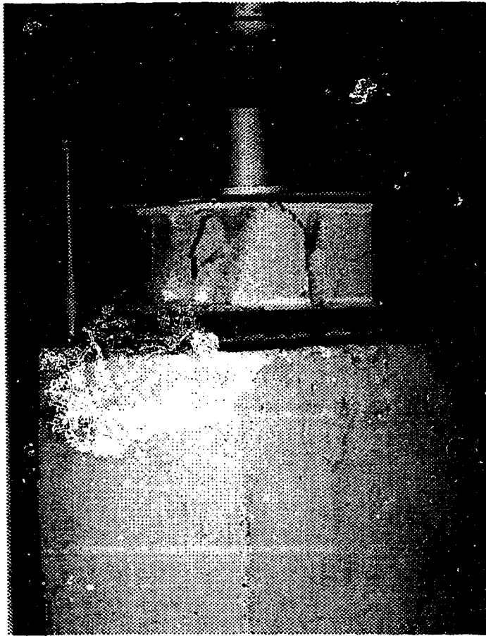
Plate 3.1 Failure of concrete block unit in compression
