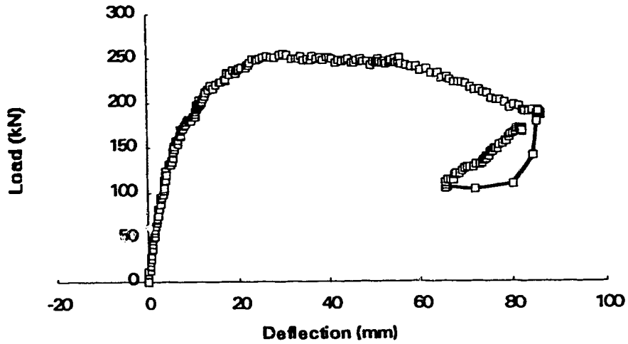
Figure 3.10 Load vs. mid-height deflection of specimen W6
