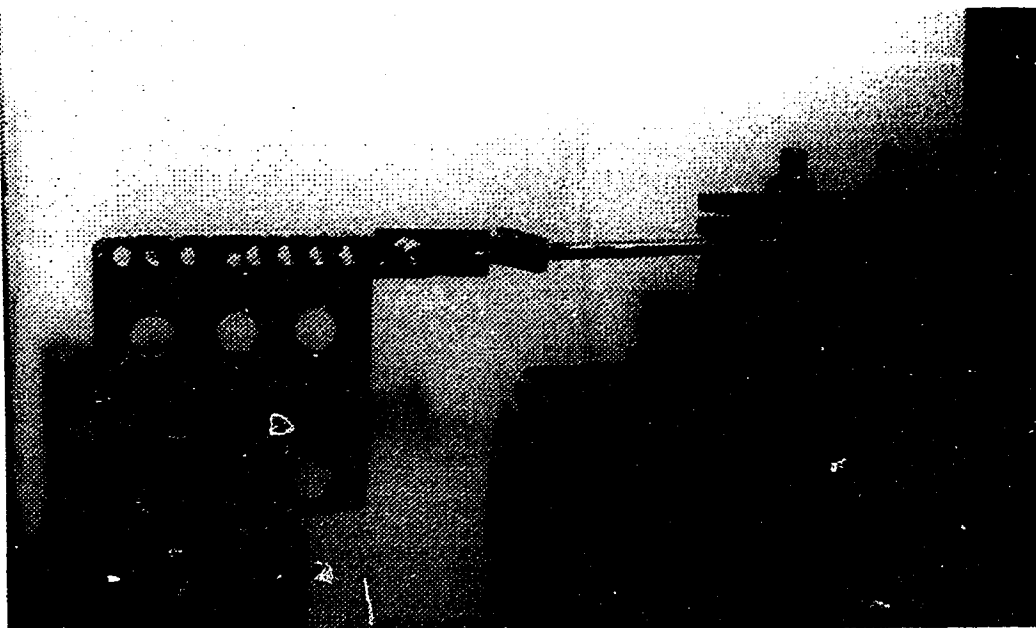
Plate 2.4 Shear test set-up
