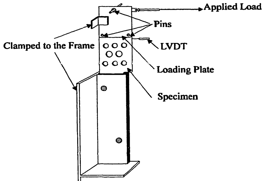
Figure 2.6 (c) Bending test set-up
