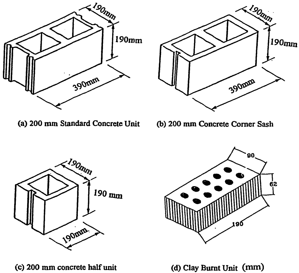
Figure 3.1 Dimensions of concrete block units and burnt clay unit
