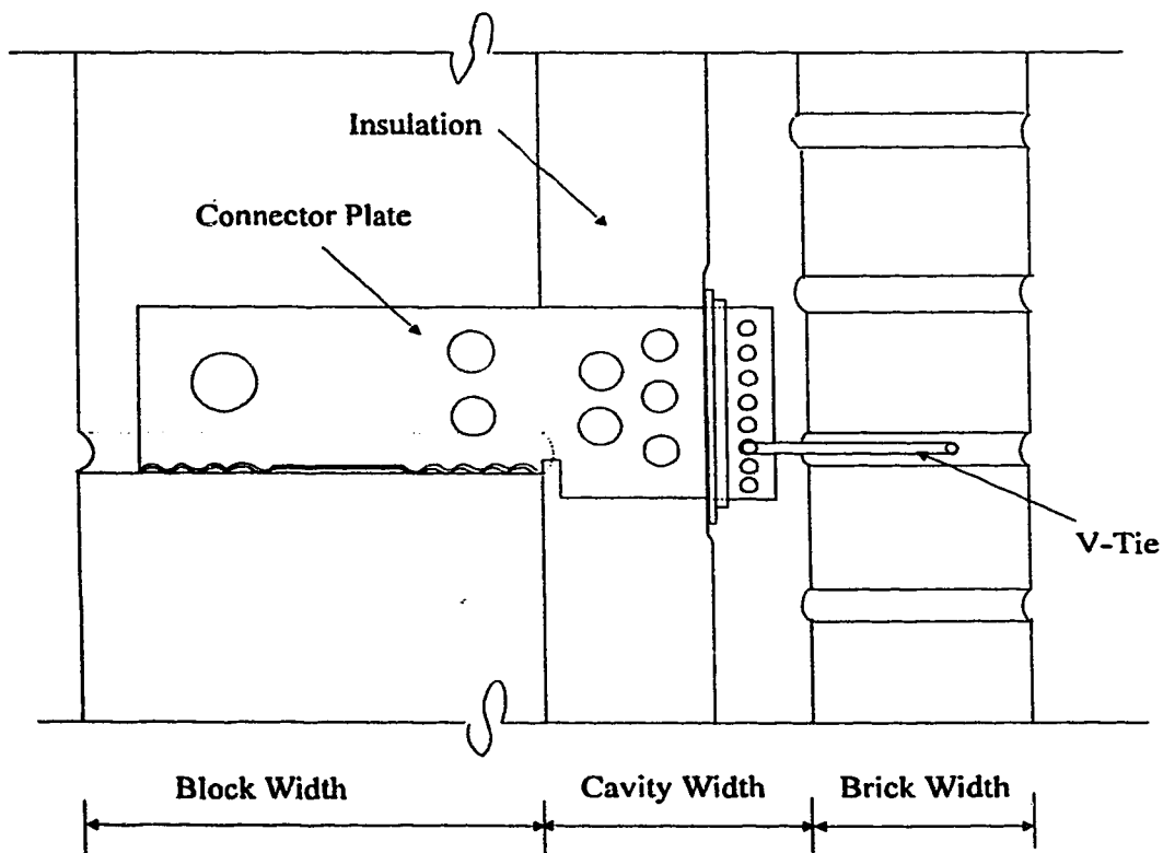
Figure 2.2 Shear connector in the cavity wall
