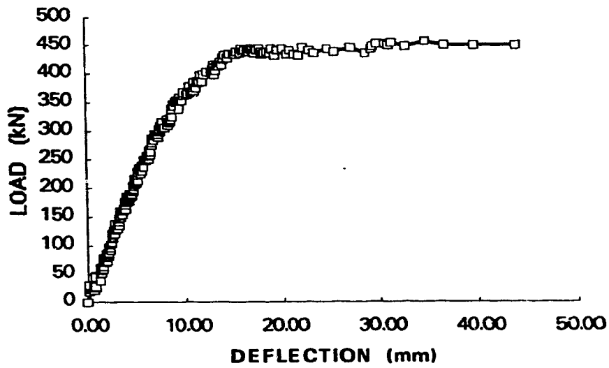
Figure 3.5 Load vs. mid-height deflection of specimen W1
