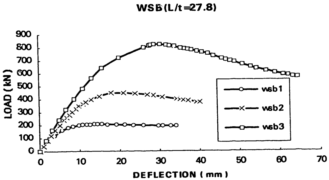
Figure 5.6 Load-deflection curves of specimens WSB1, WSB2, and WSB3
