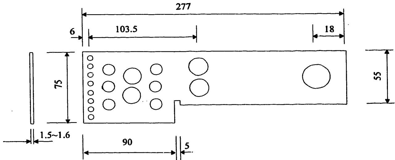
Figure 2.3 (b) Shear connector for 100 mm cavity
