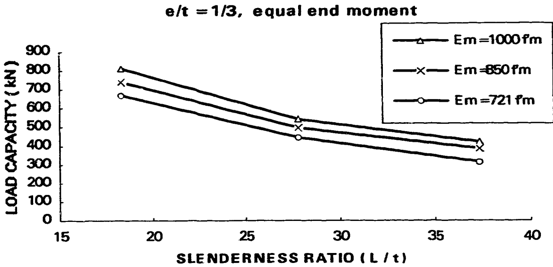
Figure 6.5 Effect of modulus of elasticity
