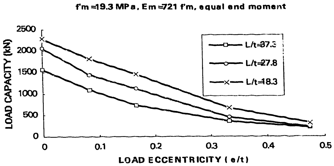
Figure 6.3 Effect of loading eccentricity
