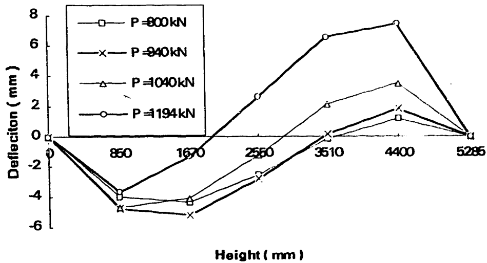
Figure 3.9 ( b ) Deflected shapes of specimen W4 ( P \geq 800 kN )
