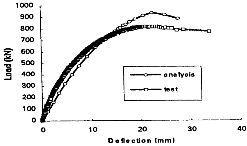
Figure 4.8 Mid-height deflection of specimen W2
