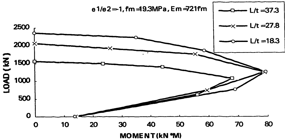
Figure 6.2 (c) Slender wall interaction diagram
