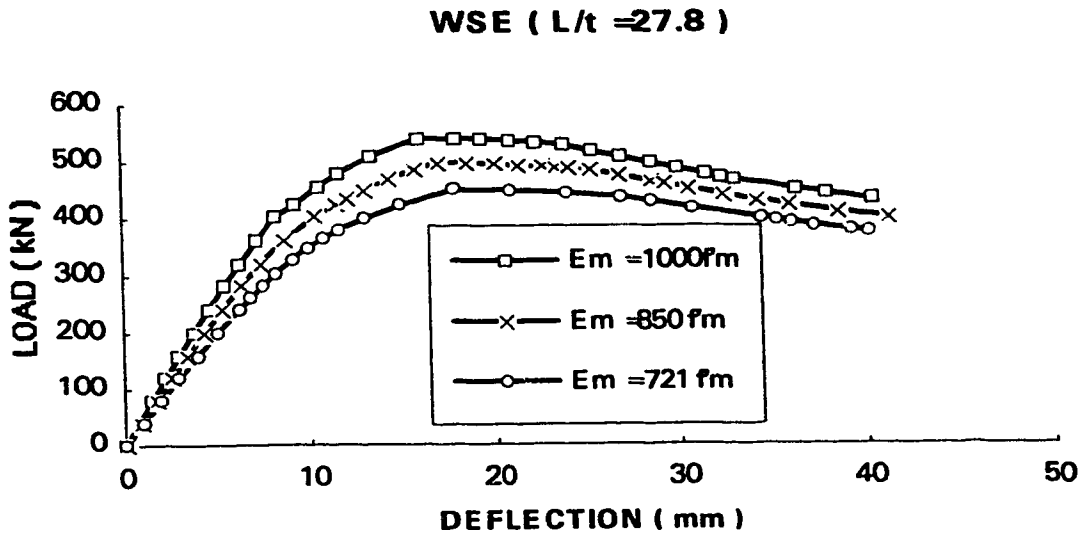
Figure 5.5 Load-deflection curves of specimens WSE1, WSE2, and WSE3
