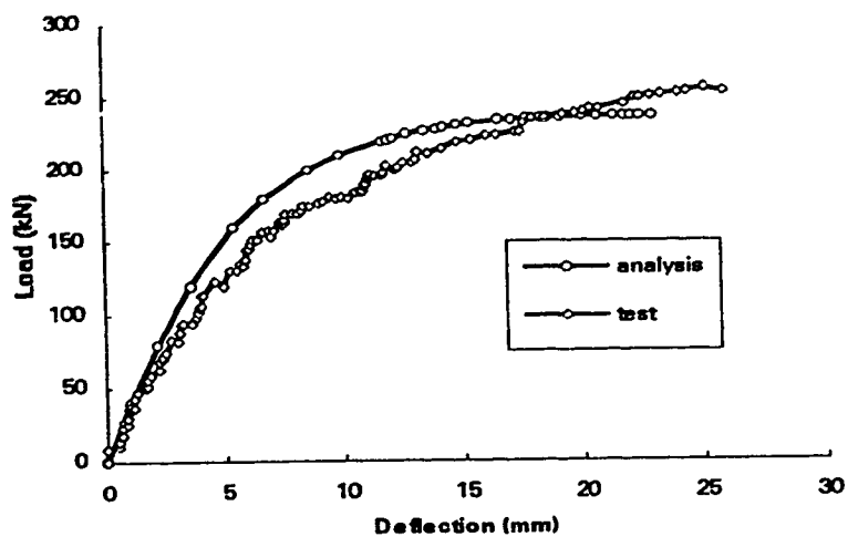
Figure 4.6 Mid-height deflection of specimen W6
