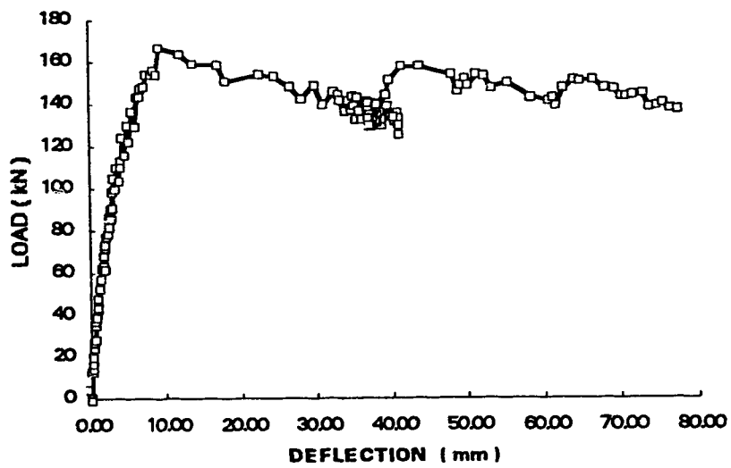
Figure 3.11 Load vs. mid-height deflection of specimen W8
