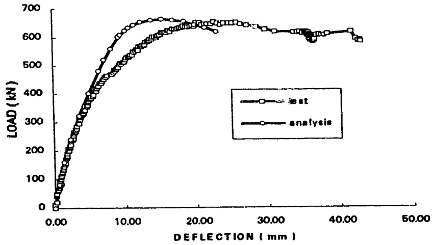
Figure 4.9 Mid-height deflection of specimen W3
