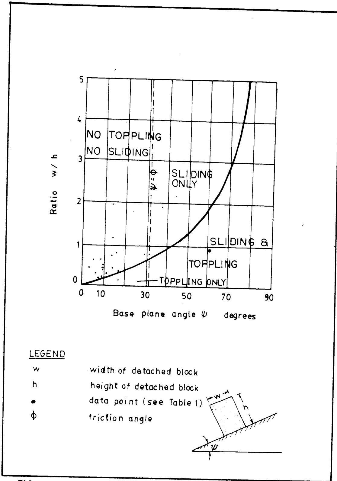
FIGURE 31. A PLOT OF WIDTH/HEIGHT RATIO OF DETACHED BLOCKS VS INCLINATION OF THESE BLOCKS (after Hoek & Bray, 1977)
