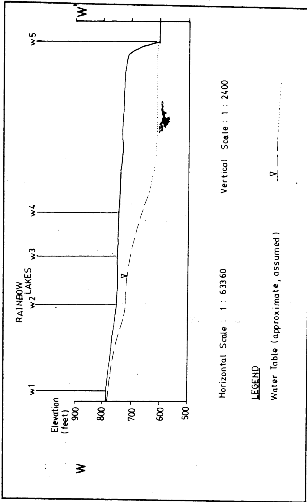
FIGURE 27 HYPOTHETICAL GROUNDWATER TABLE ALONG W - W'
