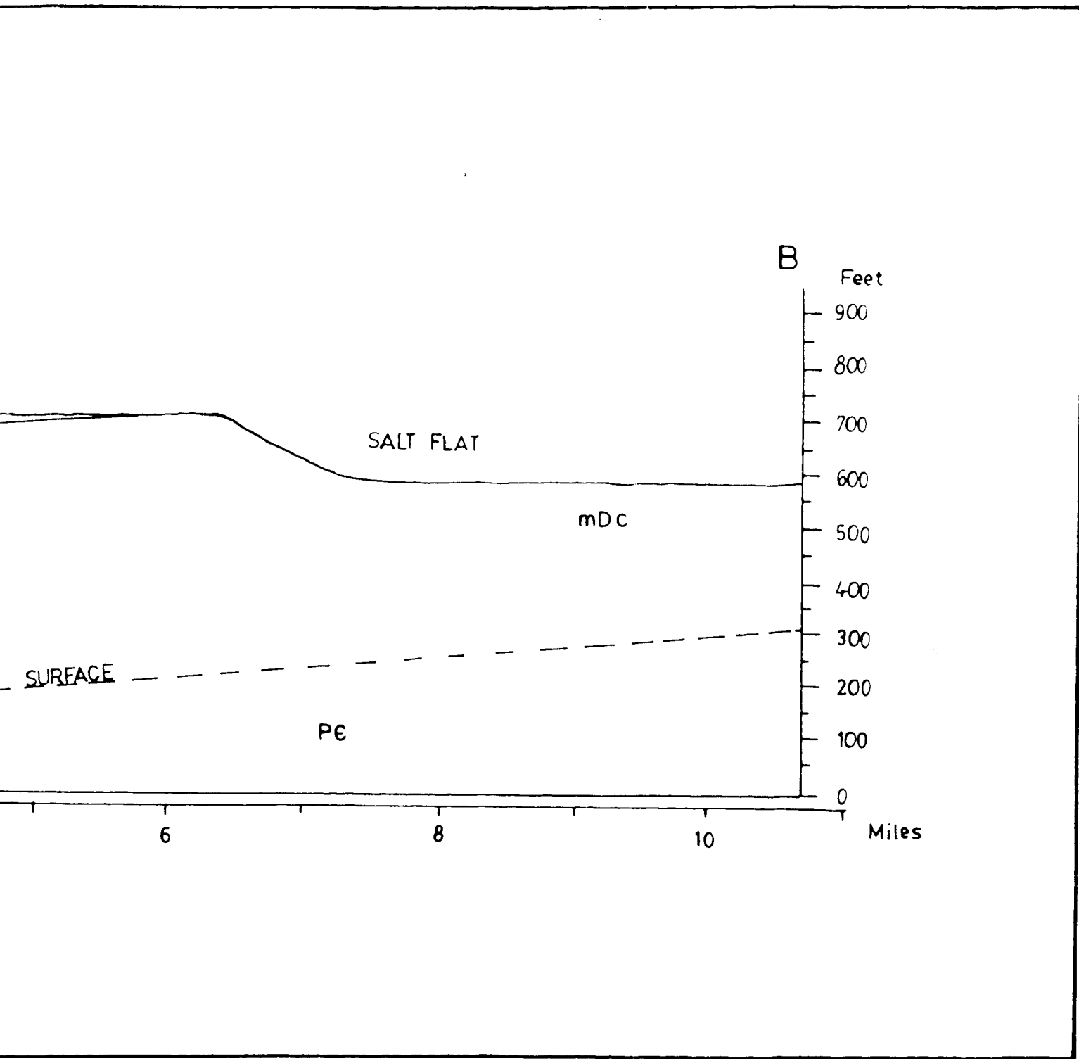
CROSS SECTION ALONG B-B' (see Figure 6)
