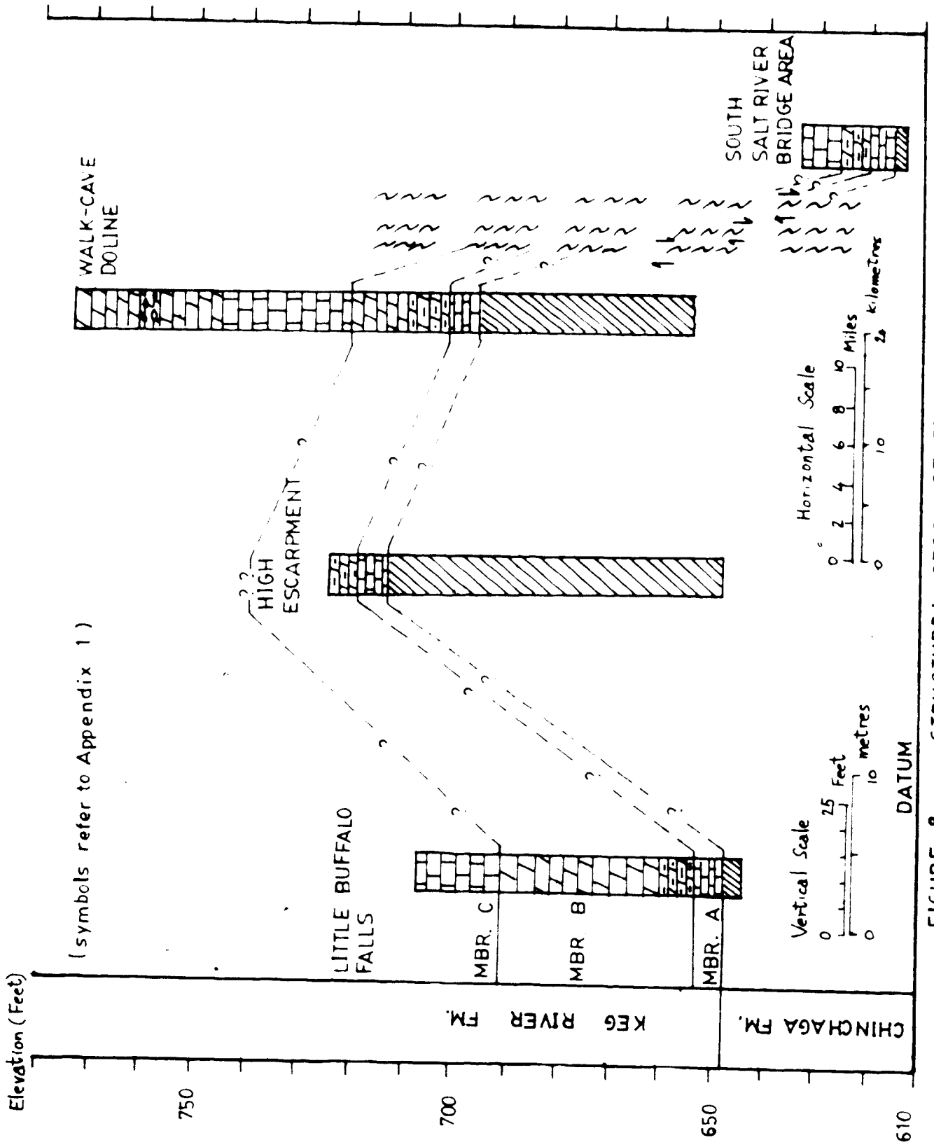
FIGURE 8. STRUCTURAL CROSS-SECTION ON A 610-FOOT DATSUM
