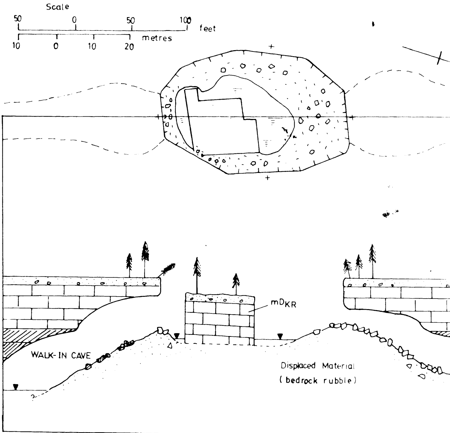
FIGURE 22. COLLAPSE DOLINE EXPOSED HOMOCLINE CAVES
