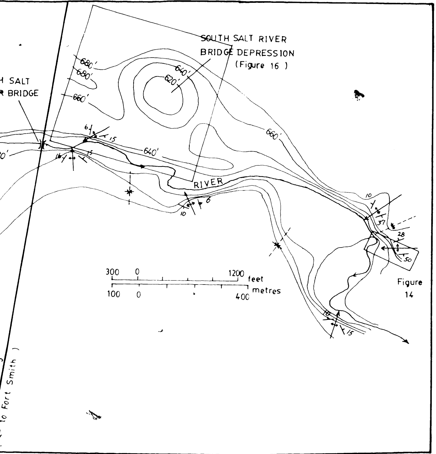
OF DEFORMED STRUCTURES EXPOSED ALONG SALT RIVER
