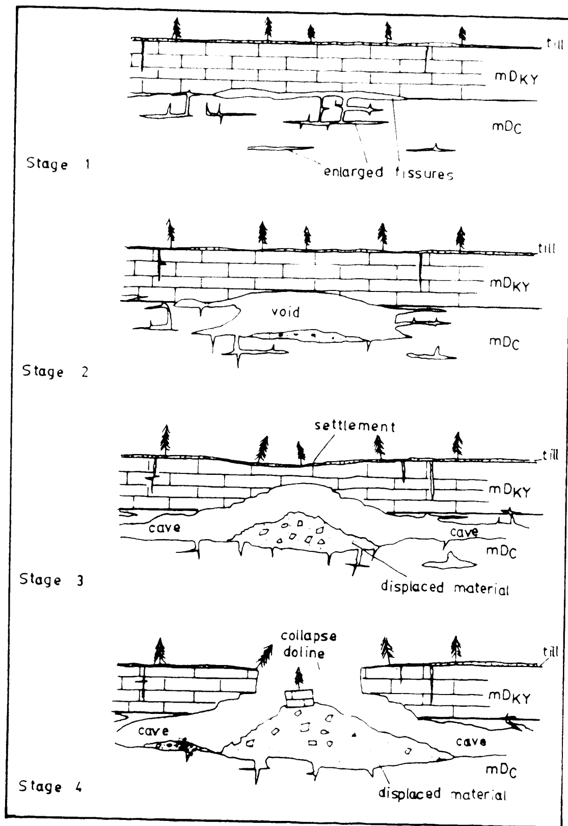
FIGURE 23. FORMATION OF A TYPICAL COLLAPSE DOLINE
