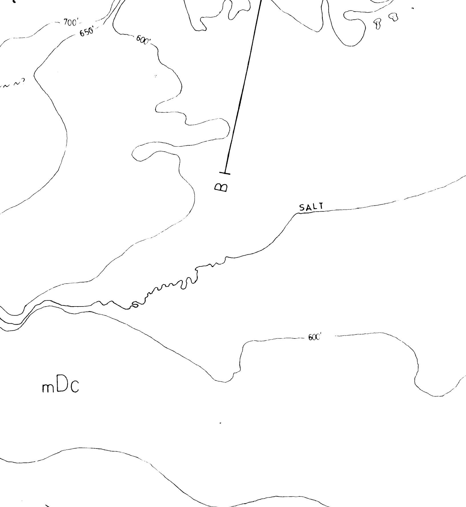
LOGIC MAP OF THE STUDY AREA, WOO
