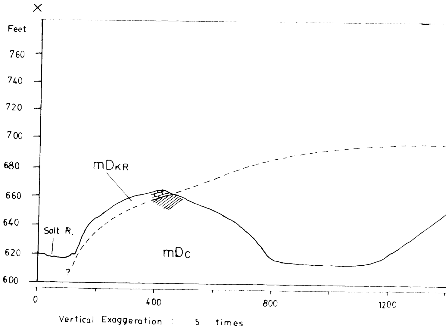
FIGURE 17. CROSS-SECTION ALONG X-X', SOUTH S
