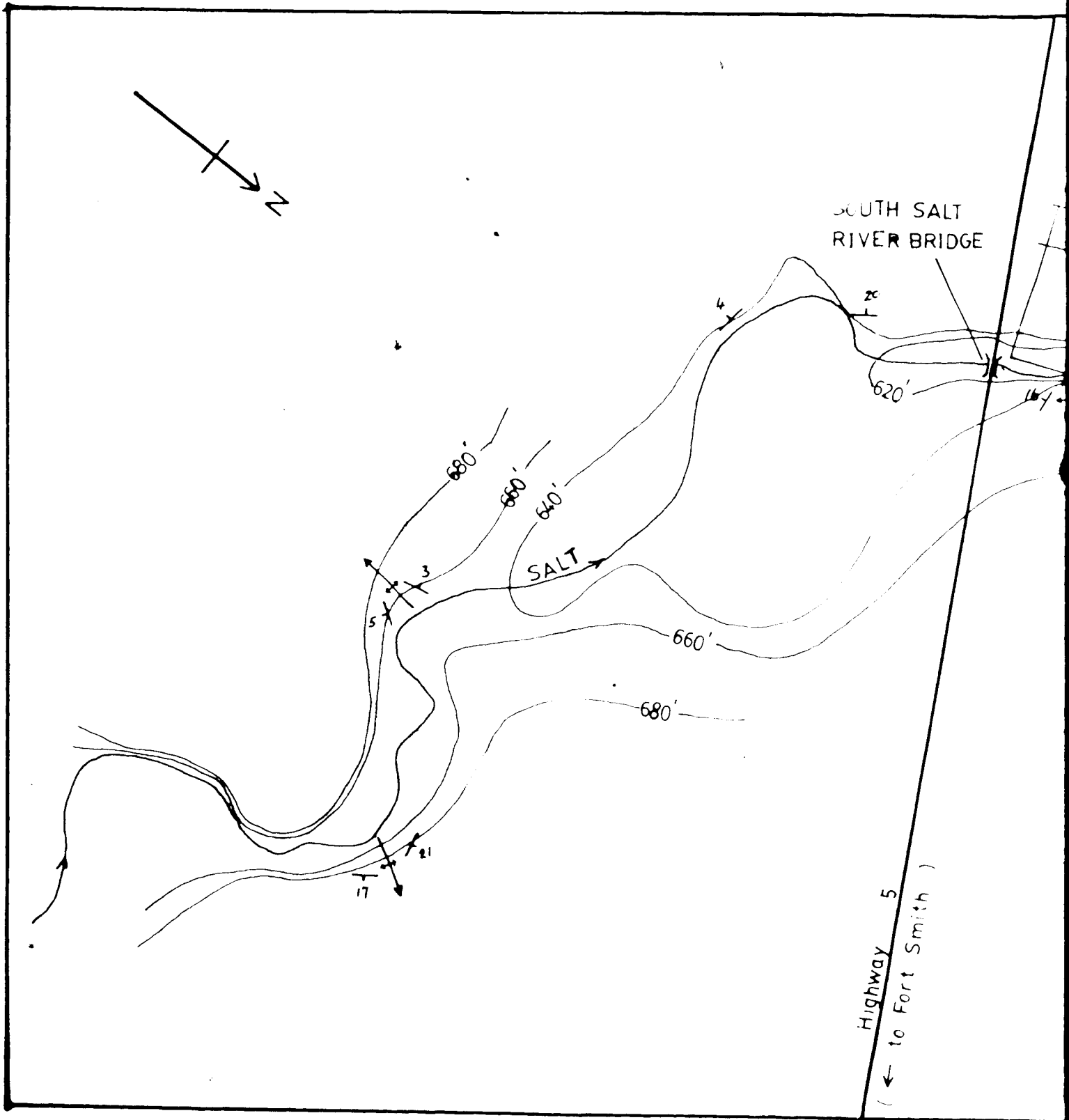
FIGURE 13. A SUMMARY PLOT OF FOLD AXES OF DEFORM
