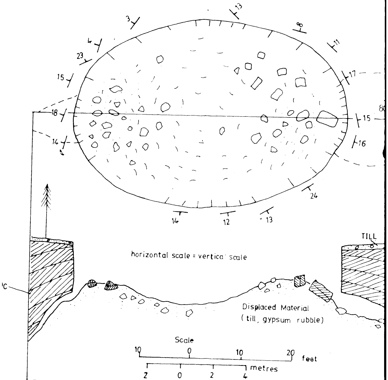
FIGURE 15. COLLAPSE DOLINE EXPOSING ANTICLINE CAVES IN THE SOUTH
