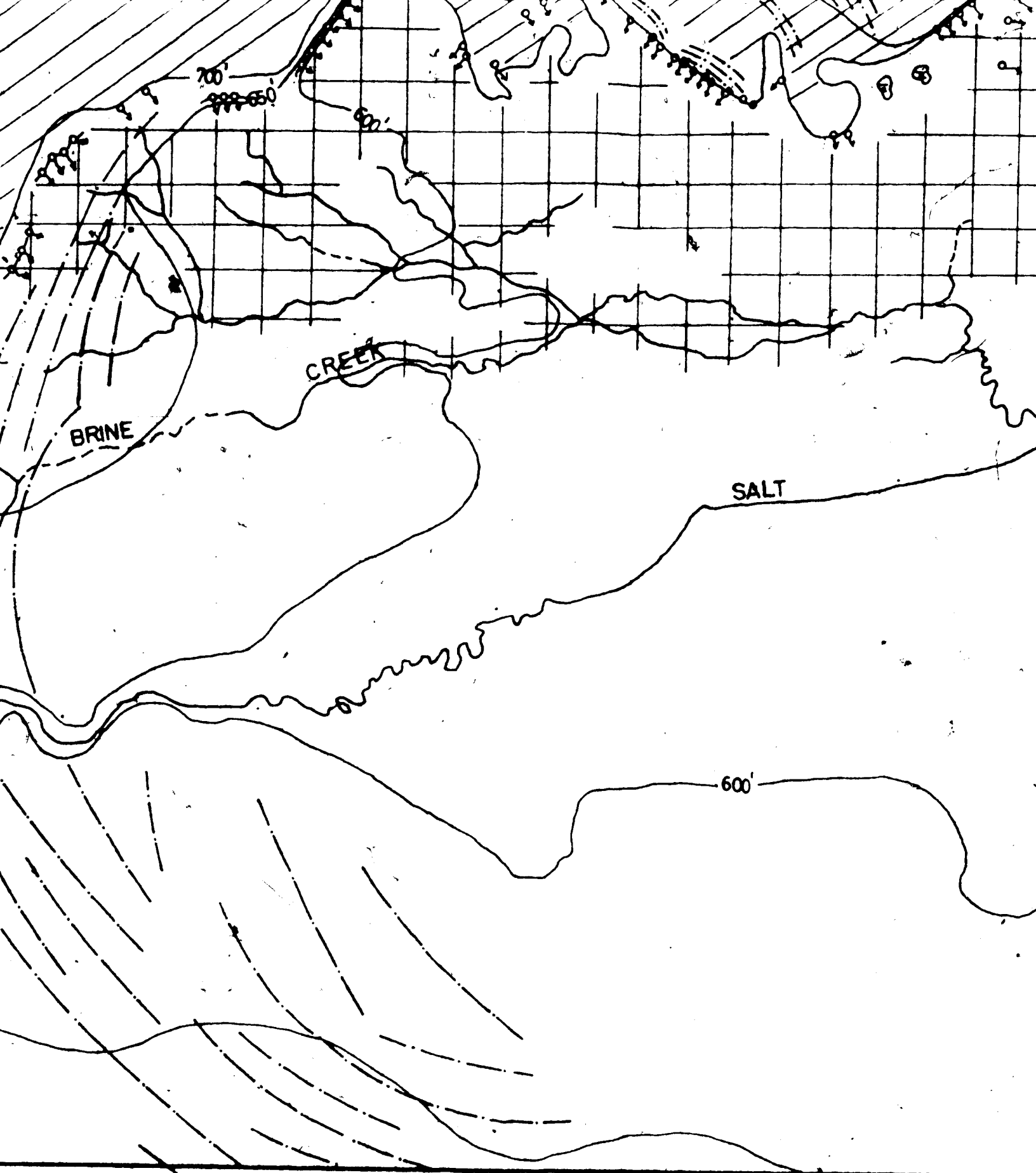
LOGICAL MAP OF THE STUDY AREA,
