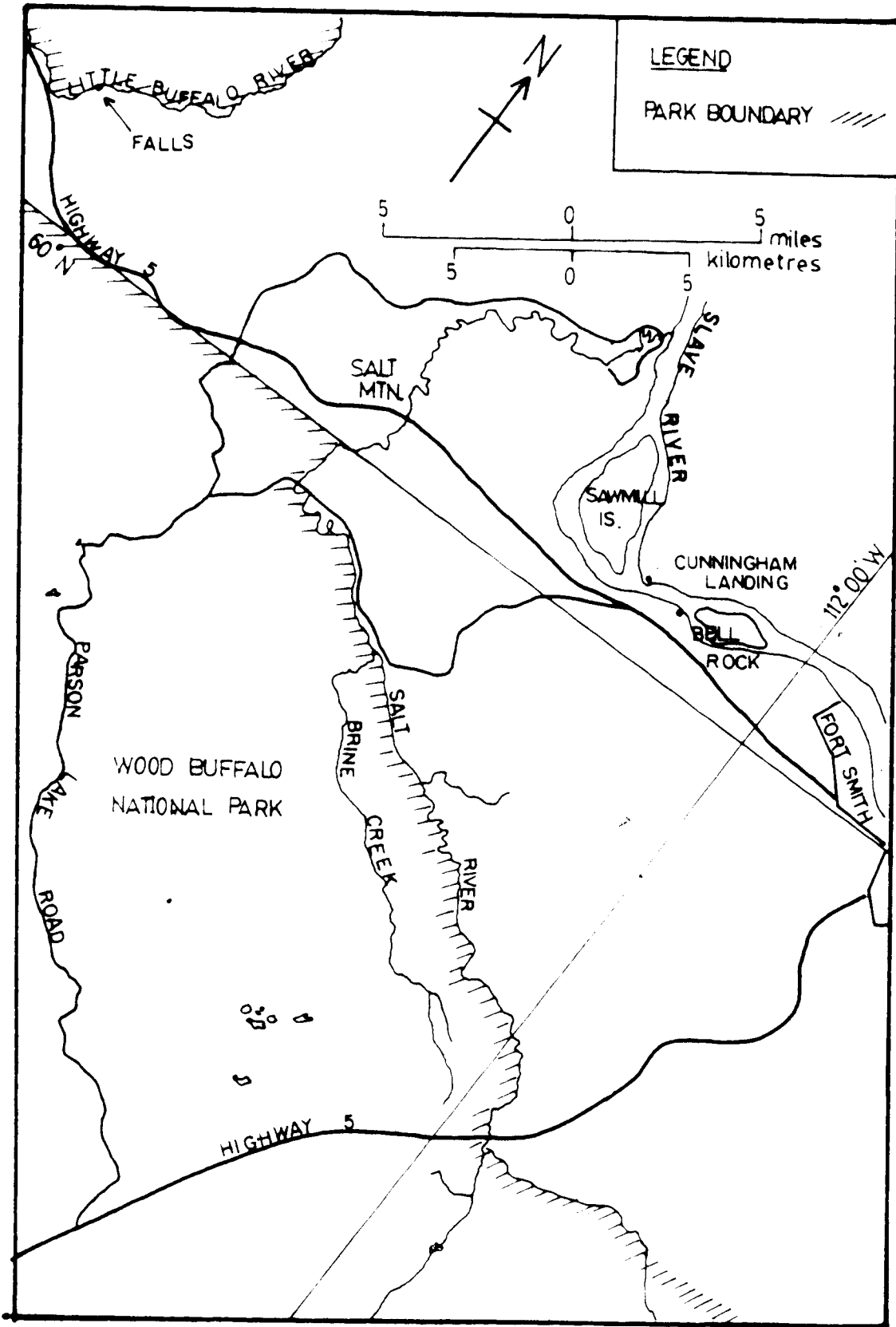
FIGURE 2. SIMPLIFIED GEOGRAPHY— OF THE STUDY AREA
