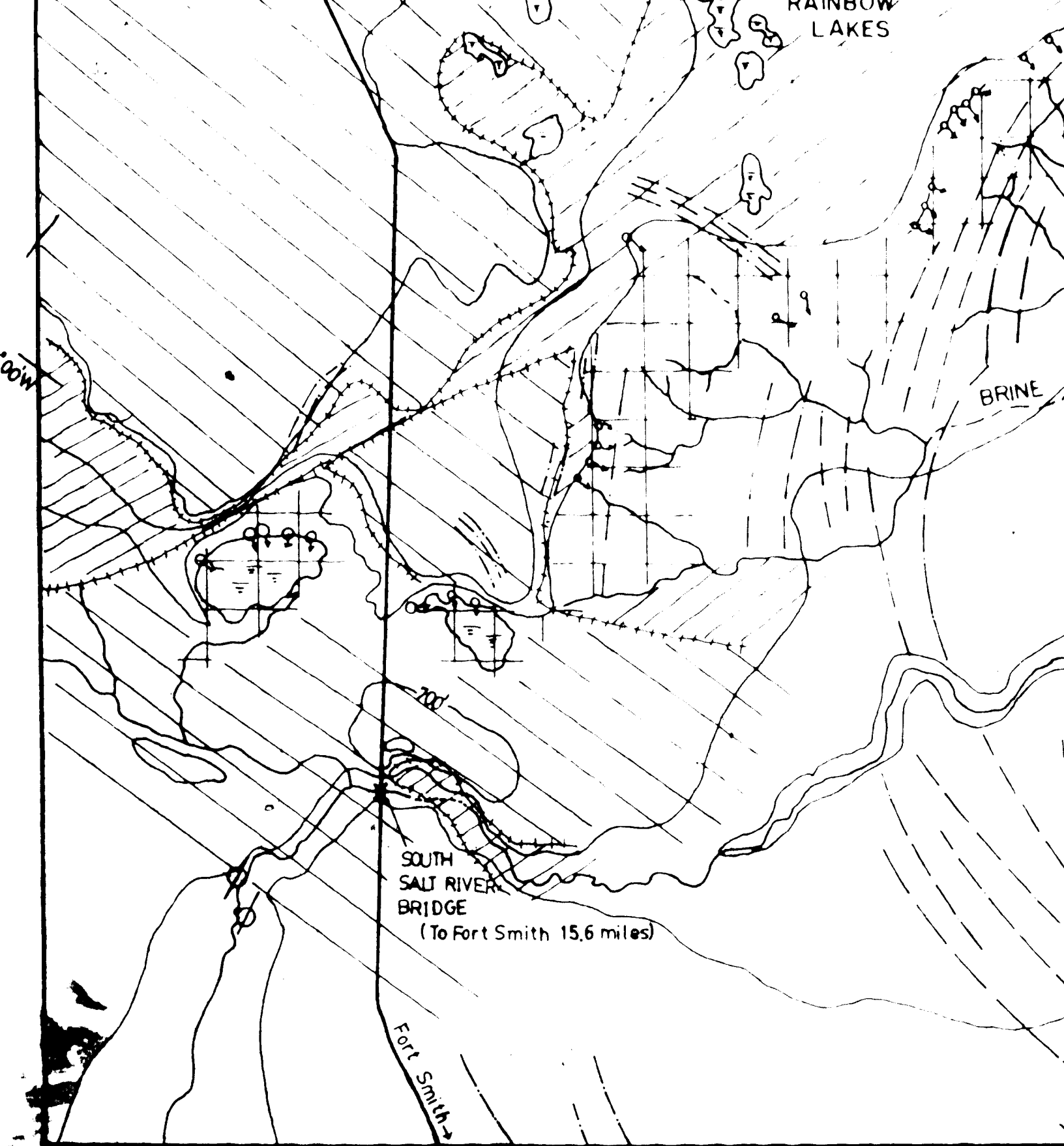
FIGURE 9 : GEOMORPHOLOGIC
