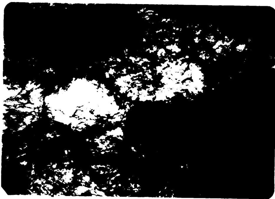
Plate 2. Gypsum nodules in outcrop near South Salt River Bridge.
