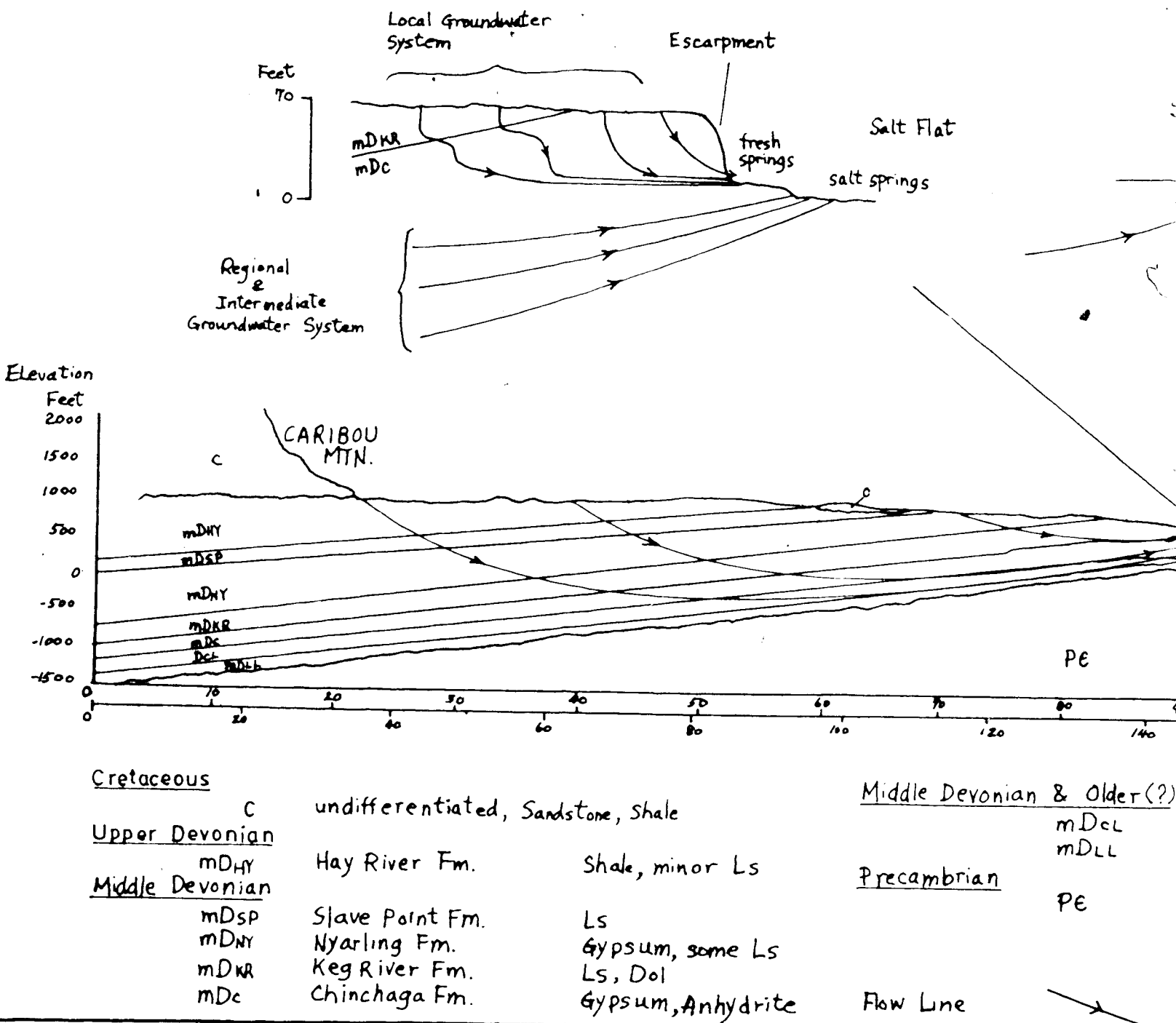
FIGURE 26. HYPOTHETICAL GROUNDWATER SYSTEMS IN WOOD BUFFALO
