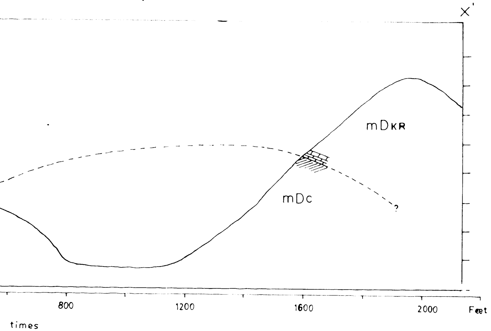
CROSS-SECTION ALONG X-X', SOUTH SALT RIVER BRIDGE DEPRESSION
