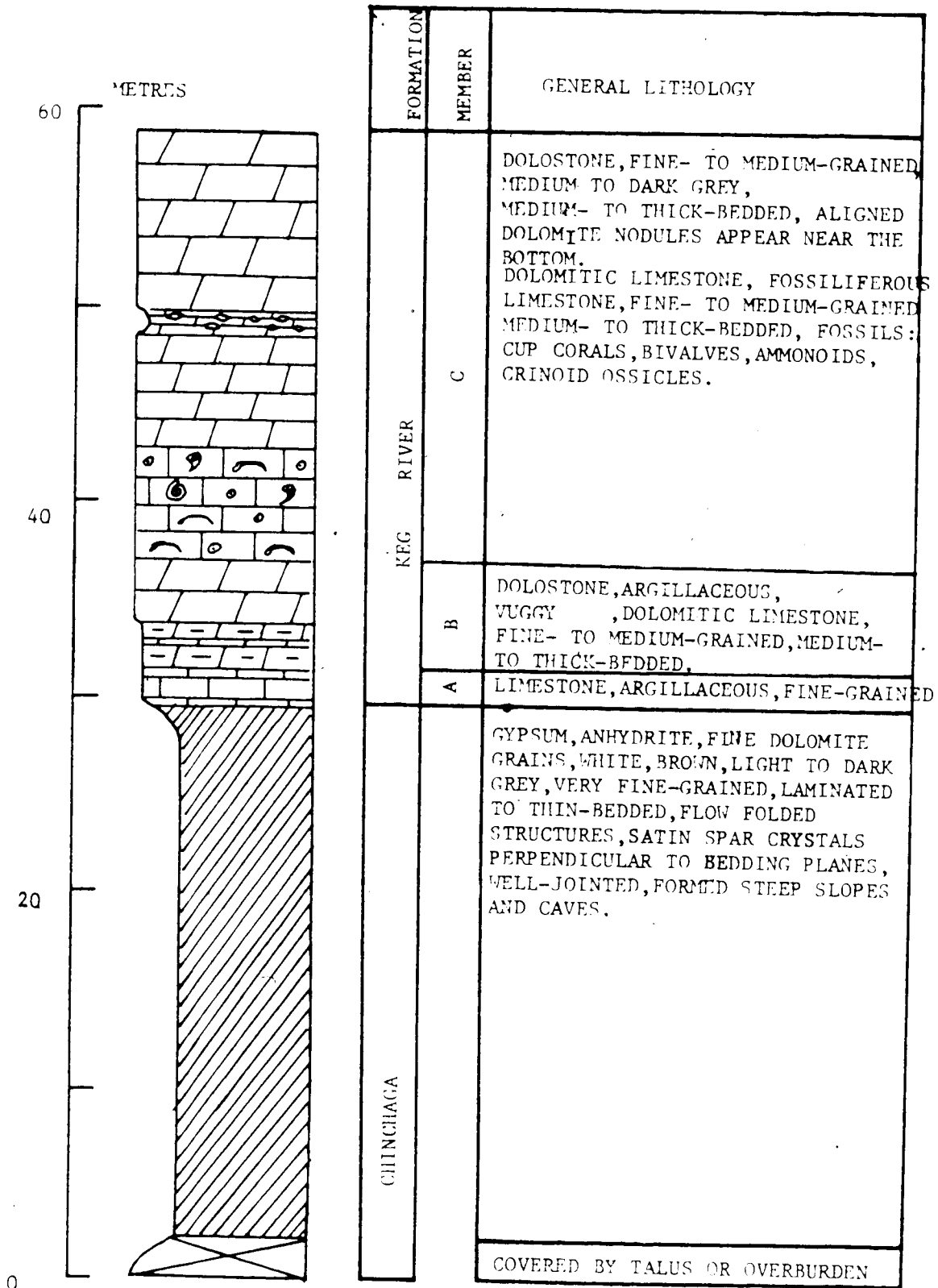
FIGURE 5. STRATIGRAPHY OF THE STUDY AREA
