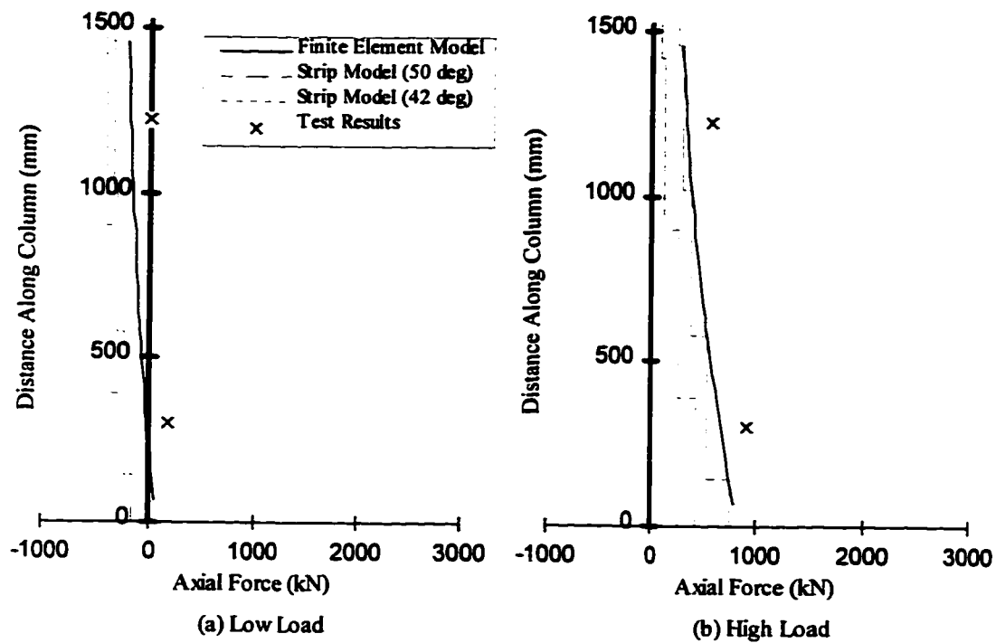
Fig. 10.9 Axial Force Diagrams – Storey 2 / East Column
