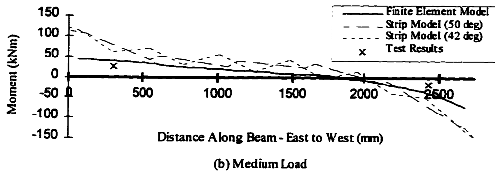
Fig. 10.5 Bending Moment Diagrams – Level 1 Beam
