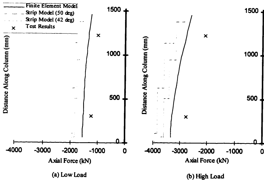
Fig. 10.10 Axial Force Diagrams – Storey 2 / West Column
