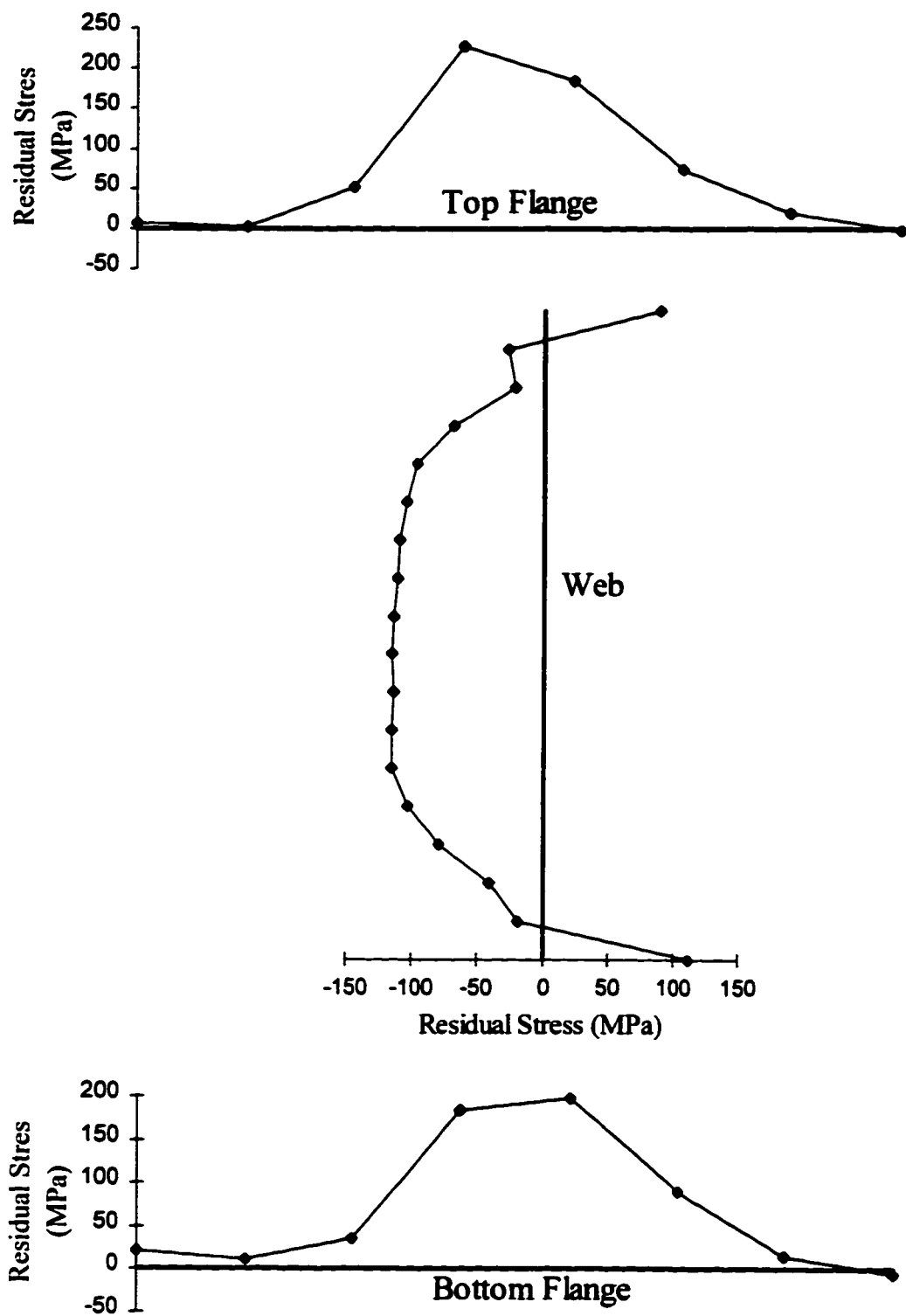
Fig. 5.6 W530x82 Residual Stress Distribution
