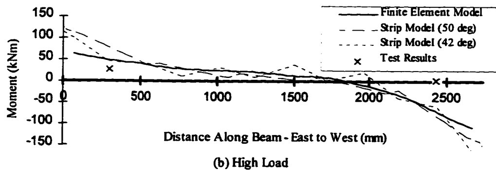
Fig. 10.6 Bending Moment Diagrams – Level 2 Beam
