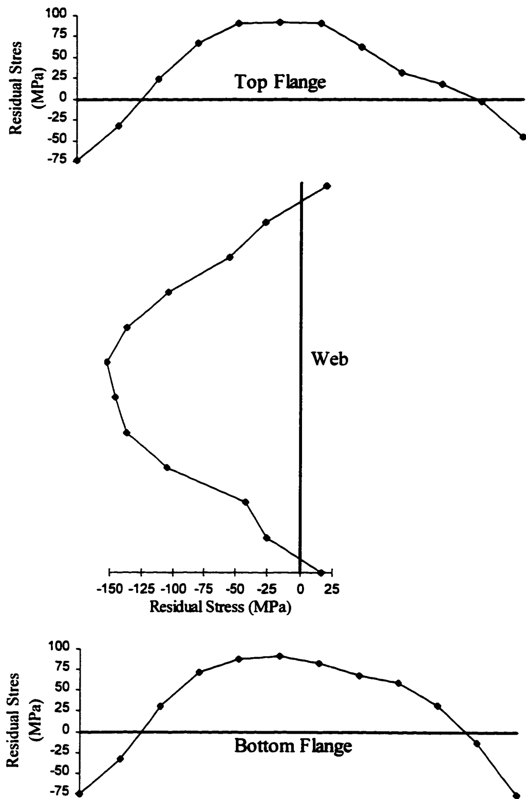
Fig. 5.4 W310x118 Residual Stress Distribution
