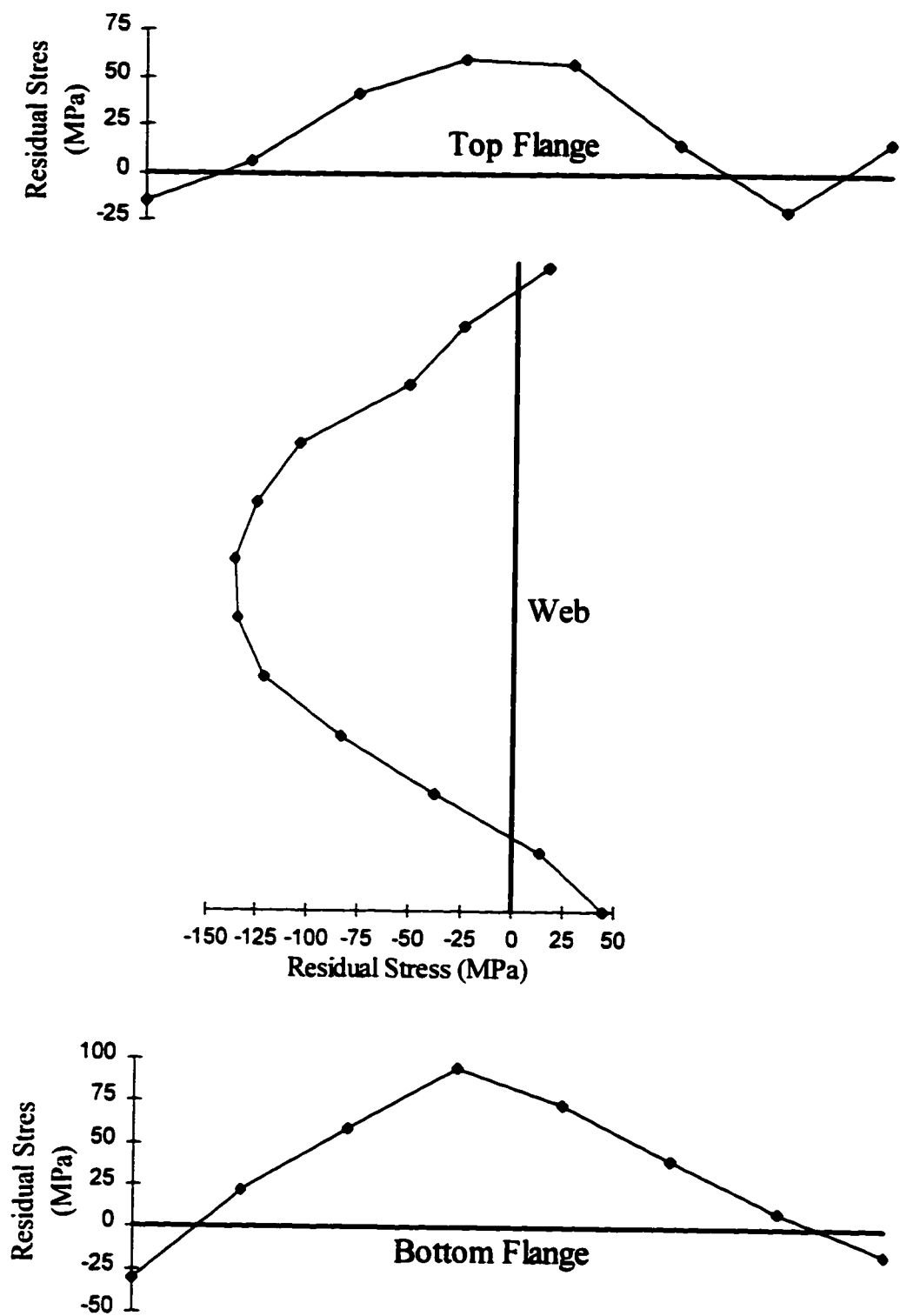
Fig. 5.5 W310x60 Residual Stress Distribution
