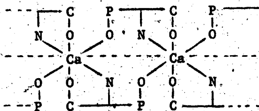
(phosphatidylserine)
