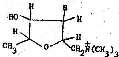
Muscarine
