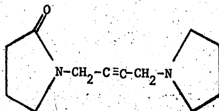
oxotremorine
