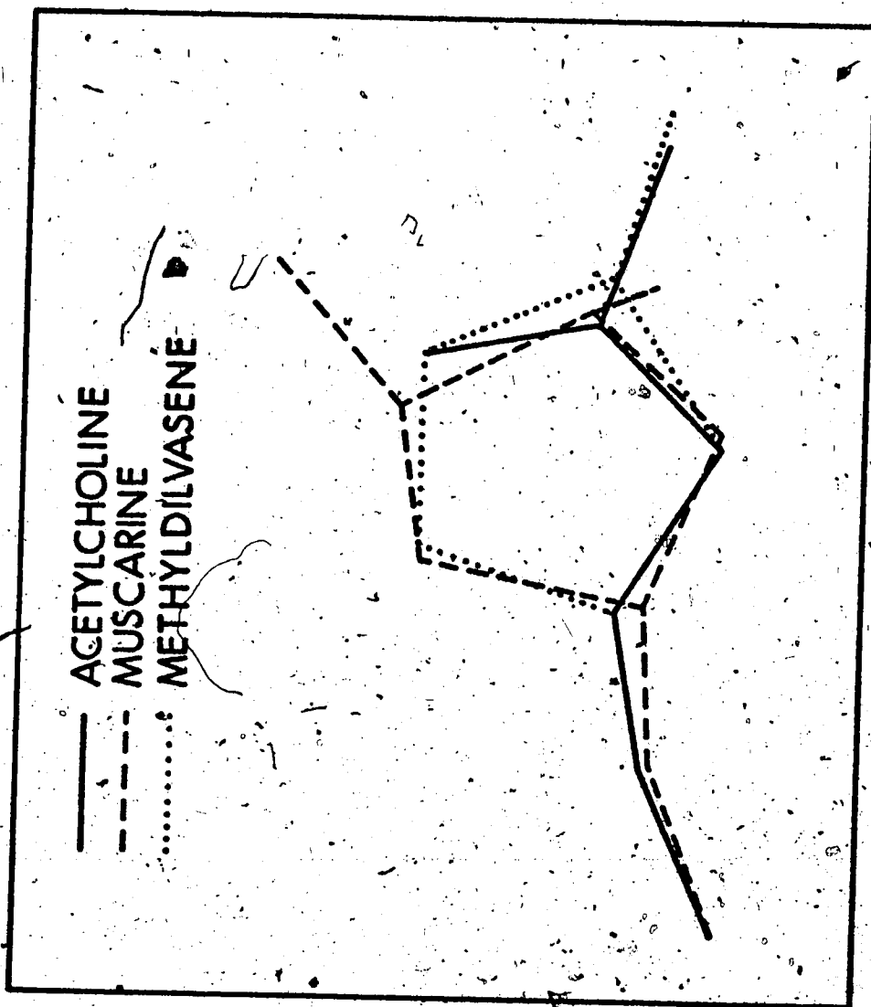
FIG. II STRUCTURAL SIMILARITIES
