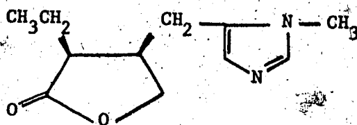
pilocarpine
