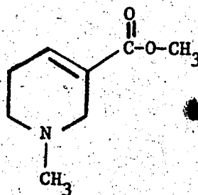
arecoline
