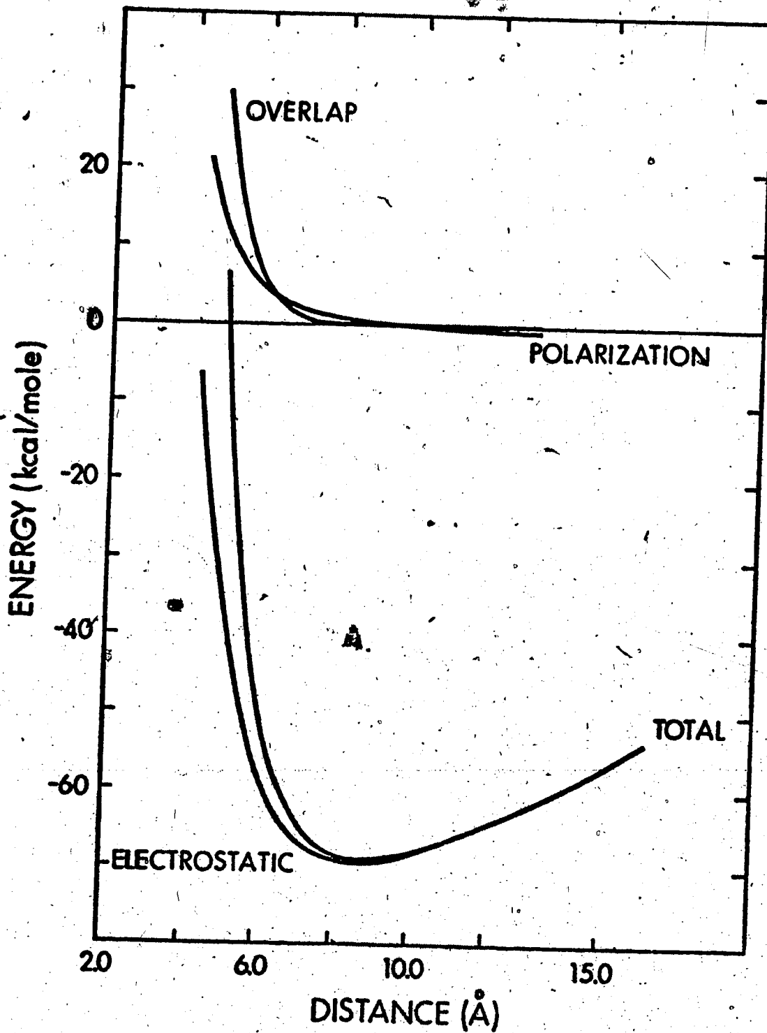
FIG. IV ACH-ACETATE ION INTERACTION
