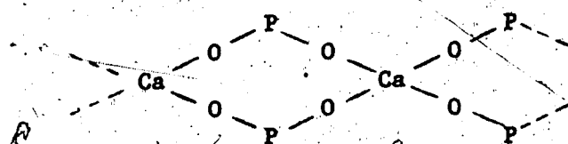
(phosphatidic acid)
