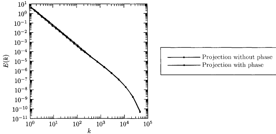
Figure 6.4: E(k) vs. k for forced-dissipative DN turbulence showing the effect of phase communication.
