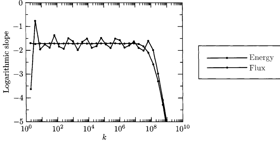
Figure 1.1: Comparison of the logarithmic slopes of the energy and flux spectra for the GOY model.
