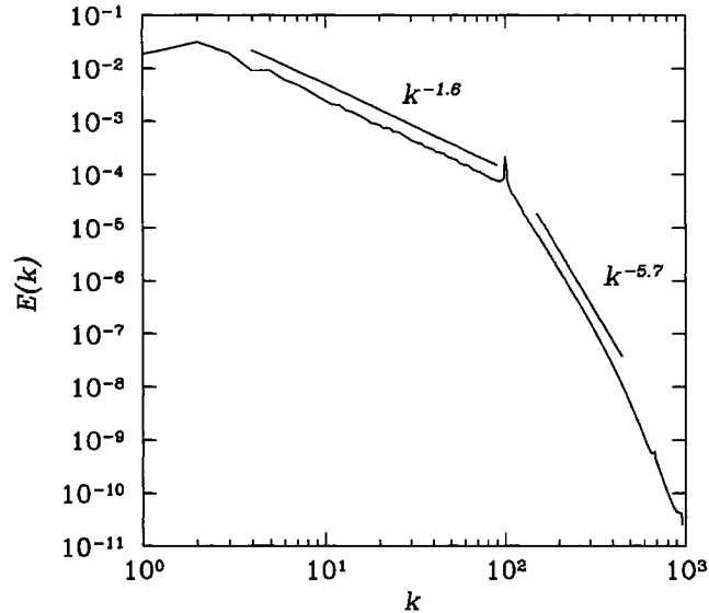
Figure 2.2: The 2D Navier–Stokes energy spectrum at intermediate times.
