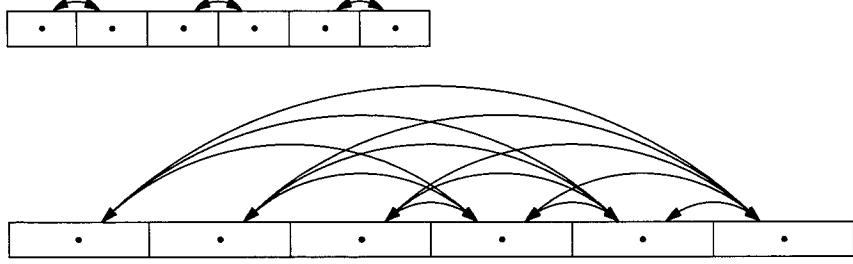
Figure 5.3: Arrangement of grids for the multi-spectral method, showing non-redundant interactions for a general shell model.
