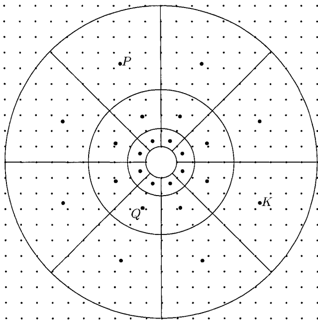
Figure 4.1: Polar wavenumber bin geometry.
