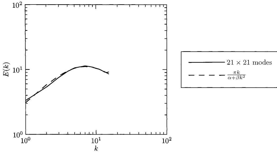
Figure 3.1: Equipartition energy spectrum of two-dimensional Navier-Stokes turbulence.
