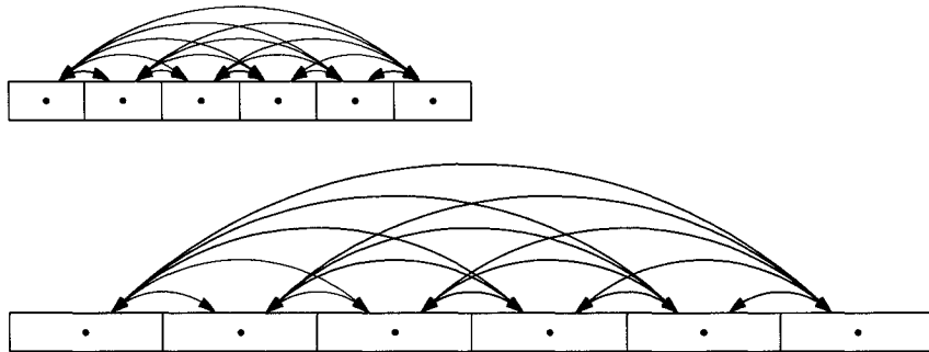
Figure 5.2: Arrangement of grids for the multi-spectral method, showing interactions for a general shell model.
