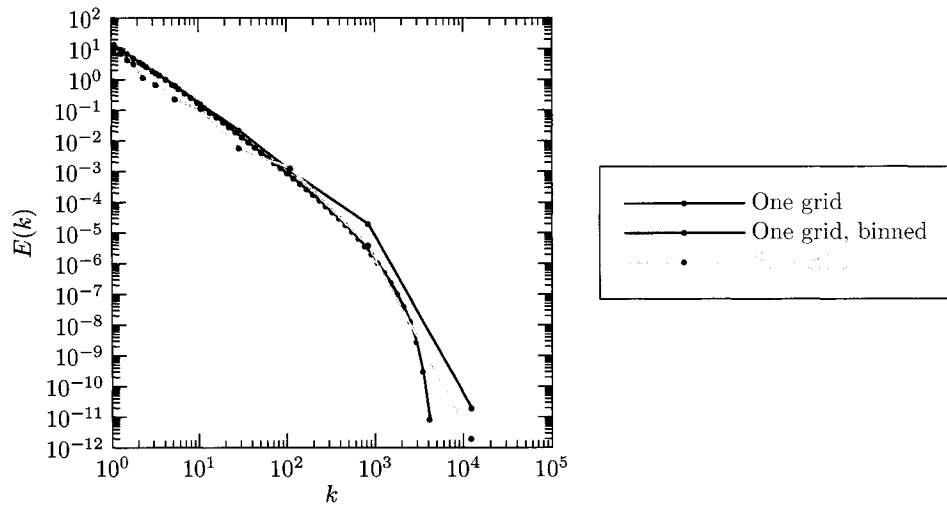
Figure 6.10: Multi-spectral simulation of forced-dissipative turbulence with five grids.
