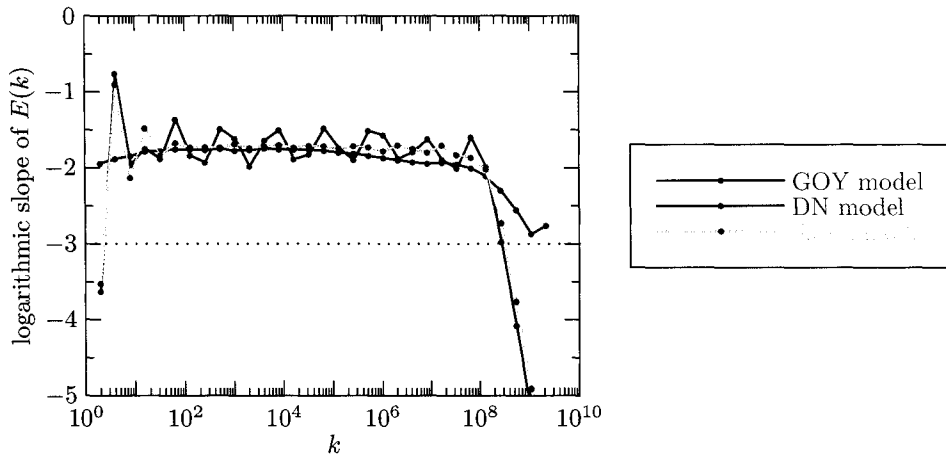
Figure 2.6: Logarithmic slopes for DN, GOY, Sabra turbulence.
