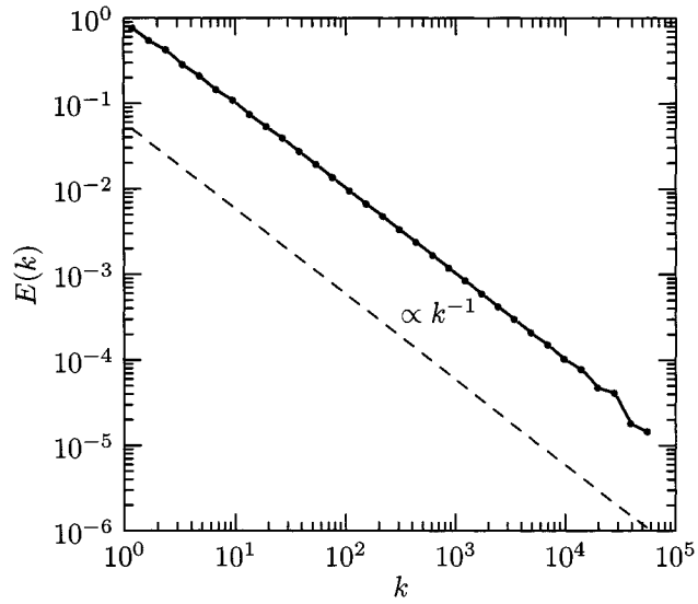
Figure 3.2: Equipartition energy spectrum of “3D” GOY turbulence.
