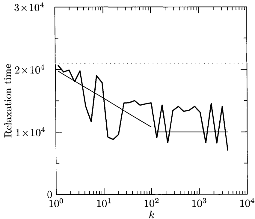
Figure 5.1: Relaxation time to equipartition for the GOY model.
