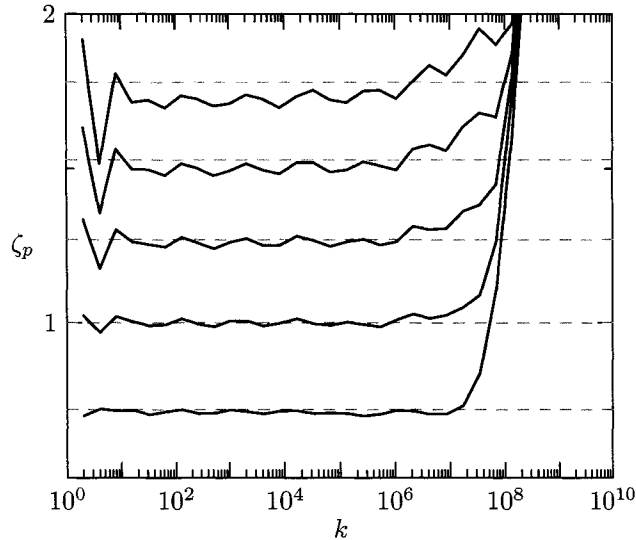
Figure 2.4: A comparison of structure-function exponents \zeta_p , p = 2, \dots, 6 (bottom to top) for the GOY model with experimental results.
