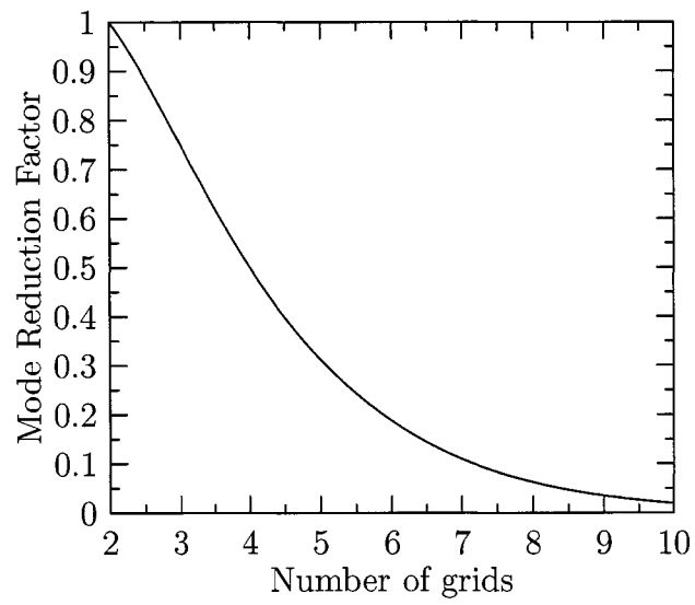
Figure 5.8: The ratio of the number of modes in a spectrally reduced system to the number of modes in the original system.
