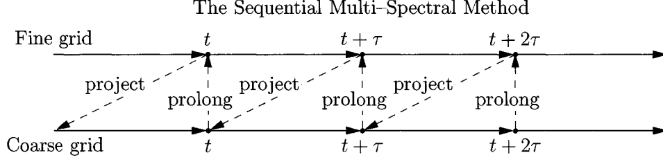
Figure 5.6: Diagram of sequential multi-spectral method.
