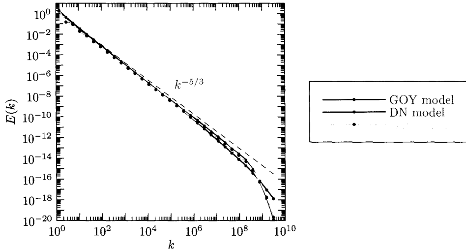
Figure 2.5: Comparison of DN, GOY, and Sabra turbulence.
