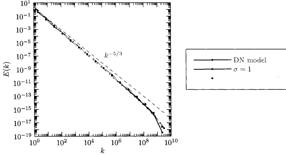
Figure 4.3: Energy spectra computed with interpolated spectral reduction.
