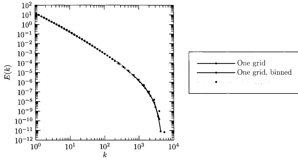
Figure 6.7: Multi-spectral simulation of forced-dissipative turbulence with two grids.
