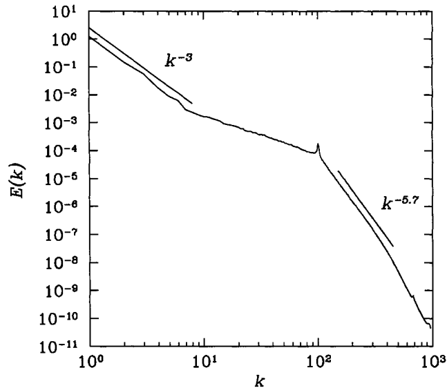
Figure 2.3: The 2D Navier–Stokes energy spectrum at late times.
