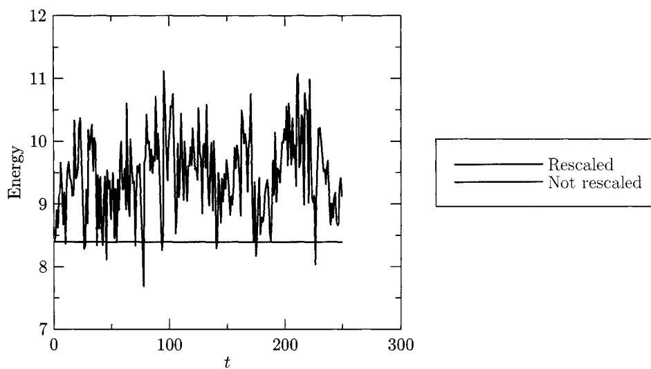
Figure 6.2: Energy vs. time for inviscid unforced turbulence with two grids and source transfer.
