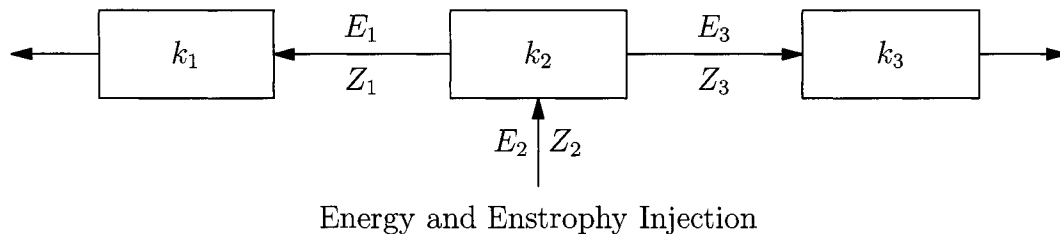
Figure 2.1: Fjørtoft diagram.
