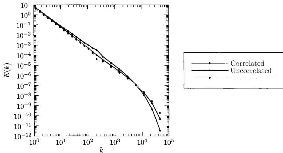
Figure 6.5: E(k) vs. k for forced-dissipative DN turbulence showing the effect of assumptions of adjacent-mode correlation given by (6.1), (6.2), and (6.3).
