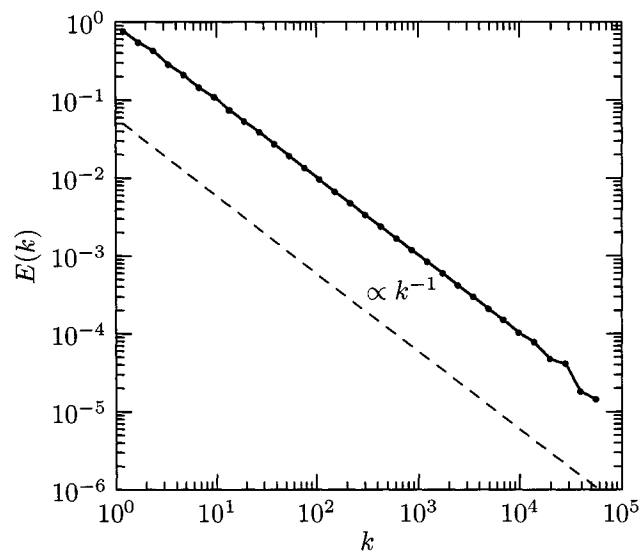
Figure 3.3: Equipartition energy spectrum of DN turbulence.
