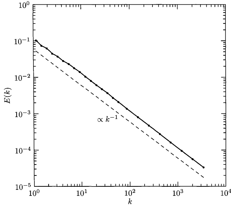
Figure 6.3: E(k) vs. k for inviscid unforced turbulence with two grids with projection/prolongation.
