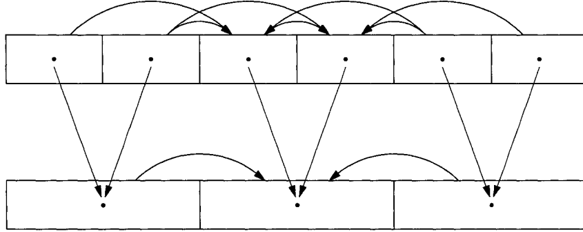
Figure 4.2: Spectral reduction of the GOY model showing emergence of nearest-neighbour interactions.
