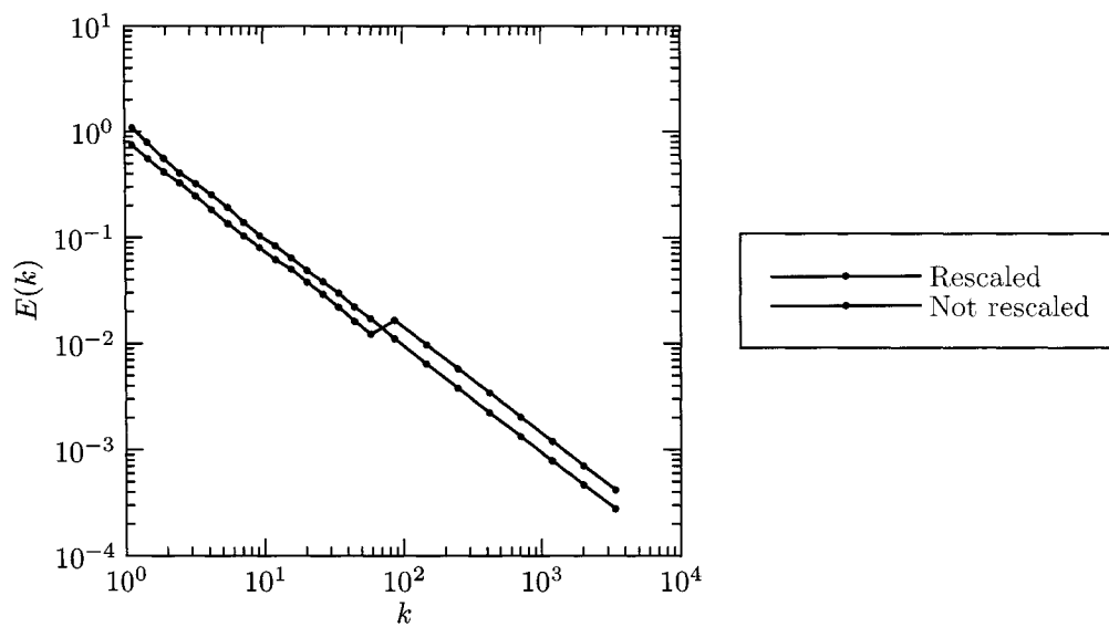
Figure 6.1: E(k) vs. k for inviscid unforced turbulence with two grids and source transfer.
