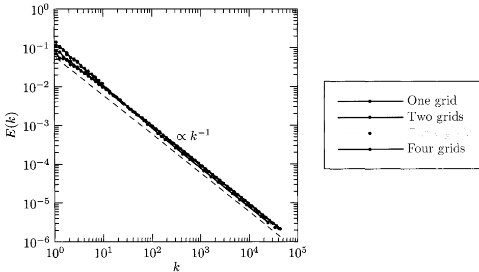
Figure 6.6: Multi-spectral simulations of inviscid turbulence with one, two, three, or four grids.
