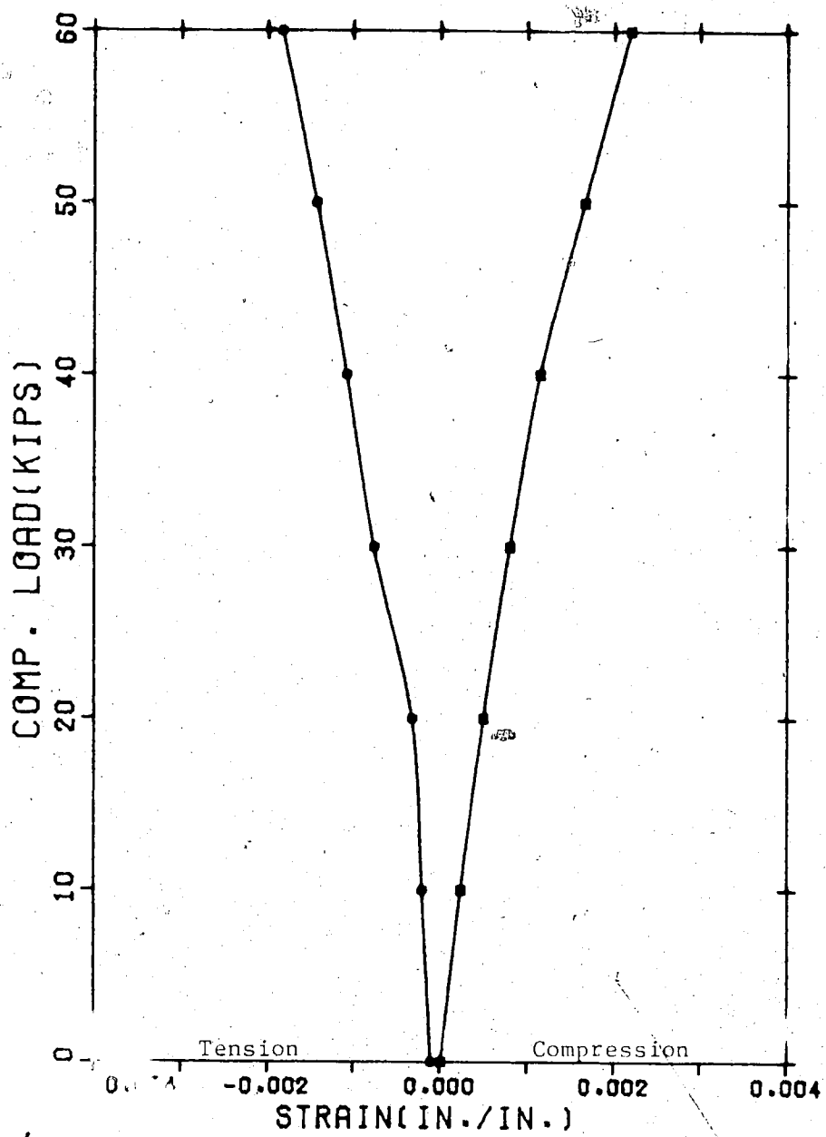
Figure 4.7 Load vs Strain for Specimen 7
