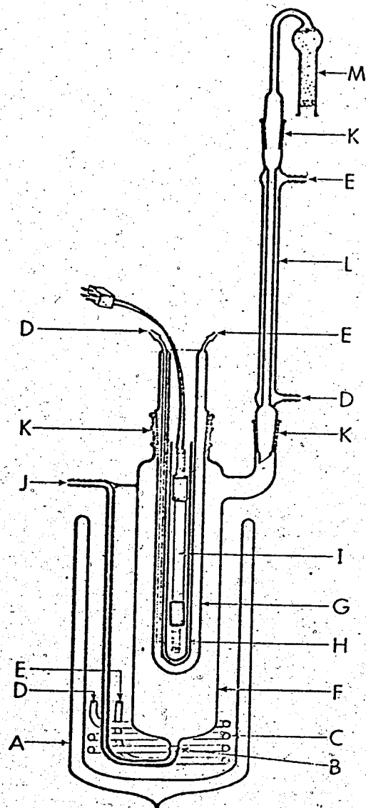
Fig. 1. A. Dewar flask; B. sintered glass filter; C. metal cooling coil; D. water inlet; E. water outlet; F. reaction vessel; G. quartz immersion well; H. pyrex filter; I. lamp; J. nitrogen gas inlet; K. ground glass joint; L. condenser; M. calcium chloride drying tube.
