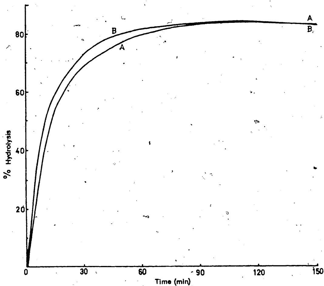
Figure 4.8. Progress curves for the hydrolysis of lactose in whey using neutral lactases. Enzyme concentration=2.0 g/l, T=38^{\circ}\text{C} and \text{pH}=6.8 .
