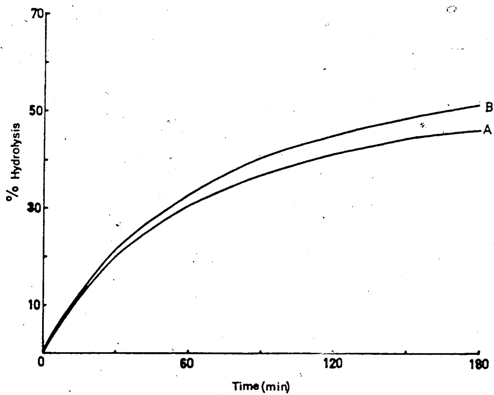
Figure 4.4. Progress curves for the hydrolysis of lactose in whey using neutral lactases. Enzyme concentration=0.1 g/l, T=38°C and pH=6.8.
