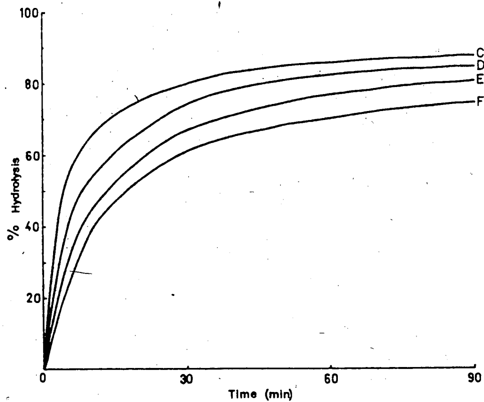
Figure 4.14. Progress curves for the hydrolysis of lactose in whey using acid lactases. Enzyme concentration=2.0 g/l, T=55°C and pH=4.6.
