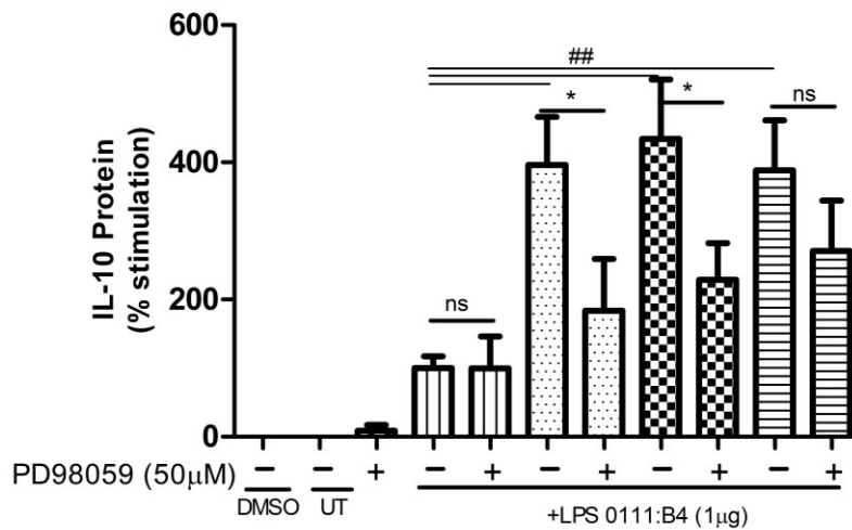
Figure 3.17 Salmeterol and vilanterol-mediated enhancement of IL-10 response is ERK1/2-dependent. BV-2 cells were treated with the ERK1/2 inhibitor PD98059 for 30 minutes, then treated with \beta 2-AR agonist ( 10^{-9} M) for 45 minutes, and then stimulated with LPS for 4 hours. Data represents mean \pm SEM from two independent experiments. * p < 0.05 and ## p < 0.001 . UT= untreated BV-2 cells.
