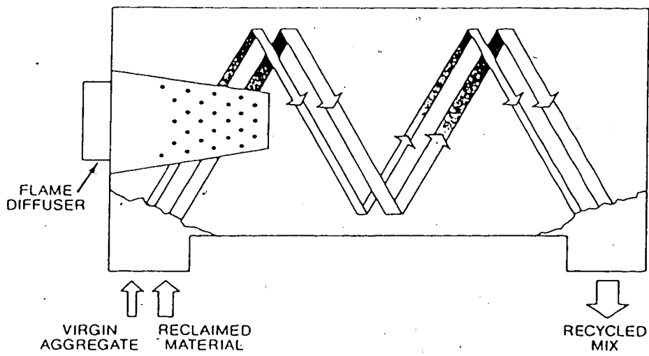
Figure 2.5 Pyrocone System
