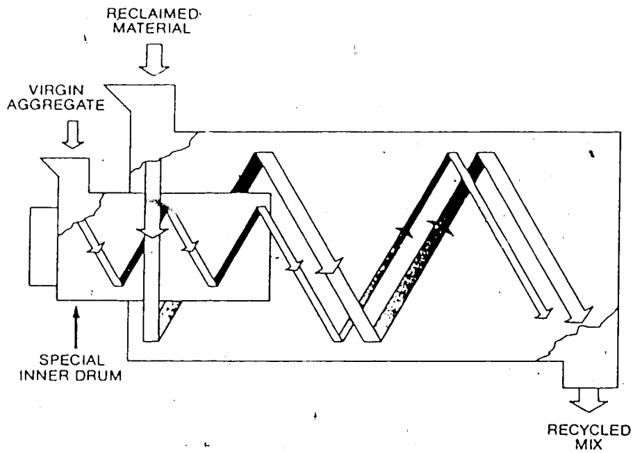
Figure 2.2 Drum-Within-A-Drum System
