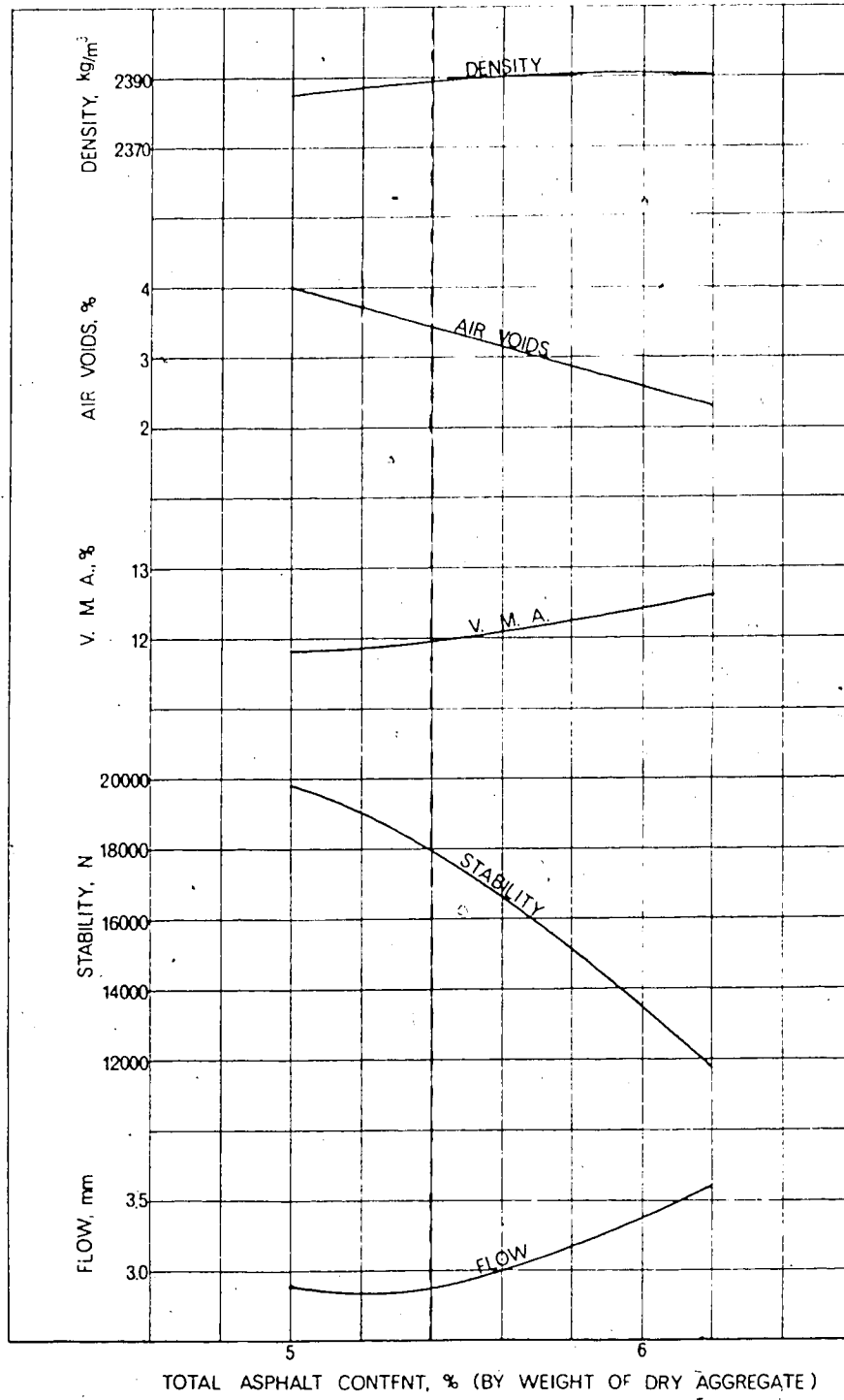
Figure 7.5 Marshall Mix Design Summary, R/V = 50/50 - Project 2:18, 2:20
