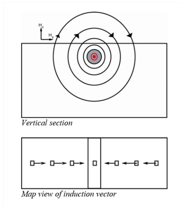
Figure 2.3: Induction vector visualization for a two-dimensional Earth. The shallow conductor creates magnetic fields that deflect Earth's magnetic field (top). The directions of the arrows reflect the location of the conductivity anomaly, in this example they are plotted in Parkinson convention, pointing towards the conductor (bottom). Figure from (Unsworth, 2014).
