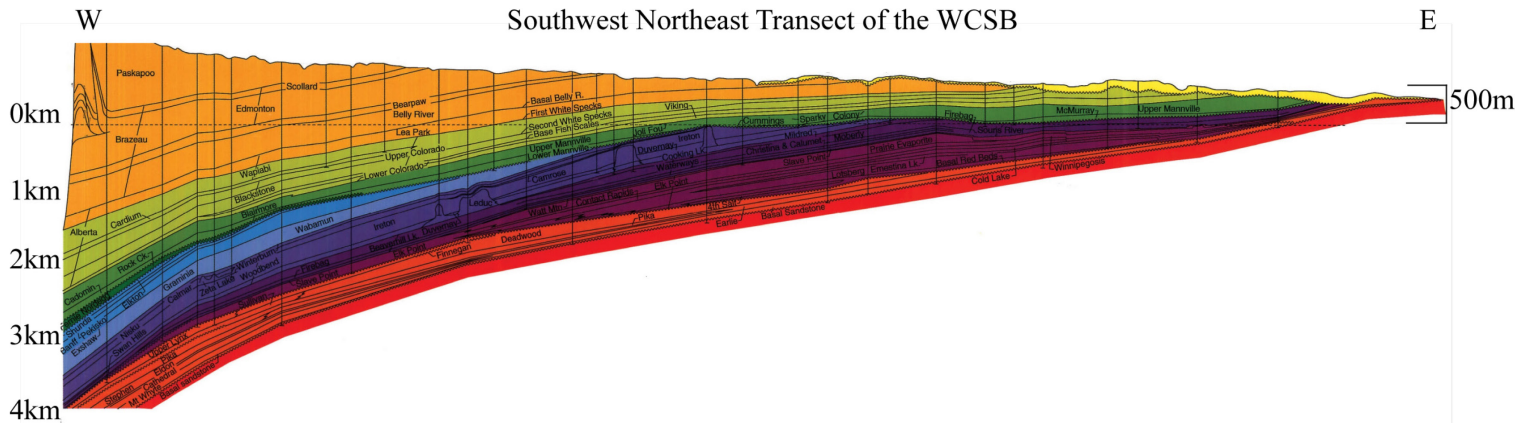
Figure 3.5: Southwest to Northeast transect of the WCSB in Alberta from the Rocky Mountains to the Canadian Shield outcrop. Colours reflect the age of the depositional formation, ranging from Cambrian on the bottom to Cenozoic strata on top. Modified from (Wright et al., 1994).
