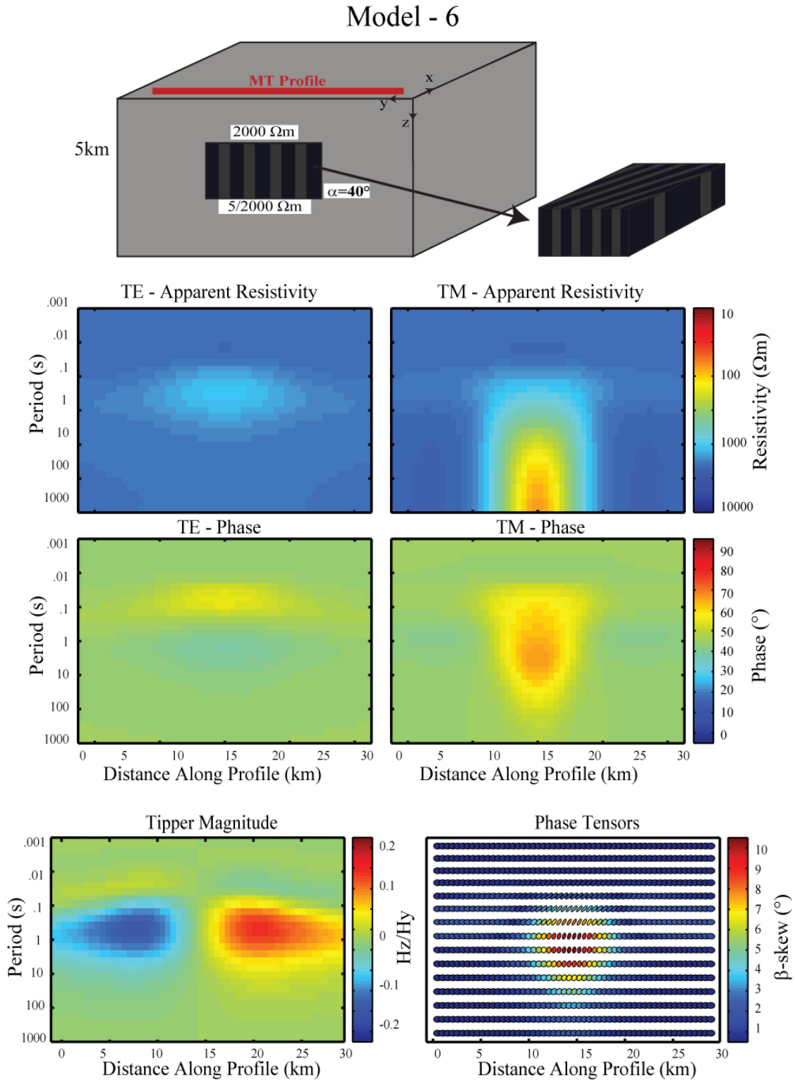
Figure 2.11: Pseudosection results for Model-6, for a 2-D earth with an anisotropic prism with anisotropic strike aligned 40^\circ clockwise from the x-direction. The orientation of the MT profile is indicated in red. The upper group of four pseudosections are the apparent resistivity and phase of the TE and TM mode. Tipper magnitude is the ratio between the vertical magnetic field H_z and the in-profile horizontal component H_y .
