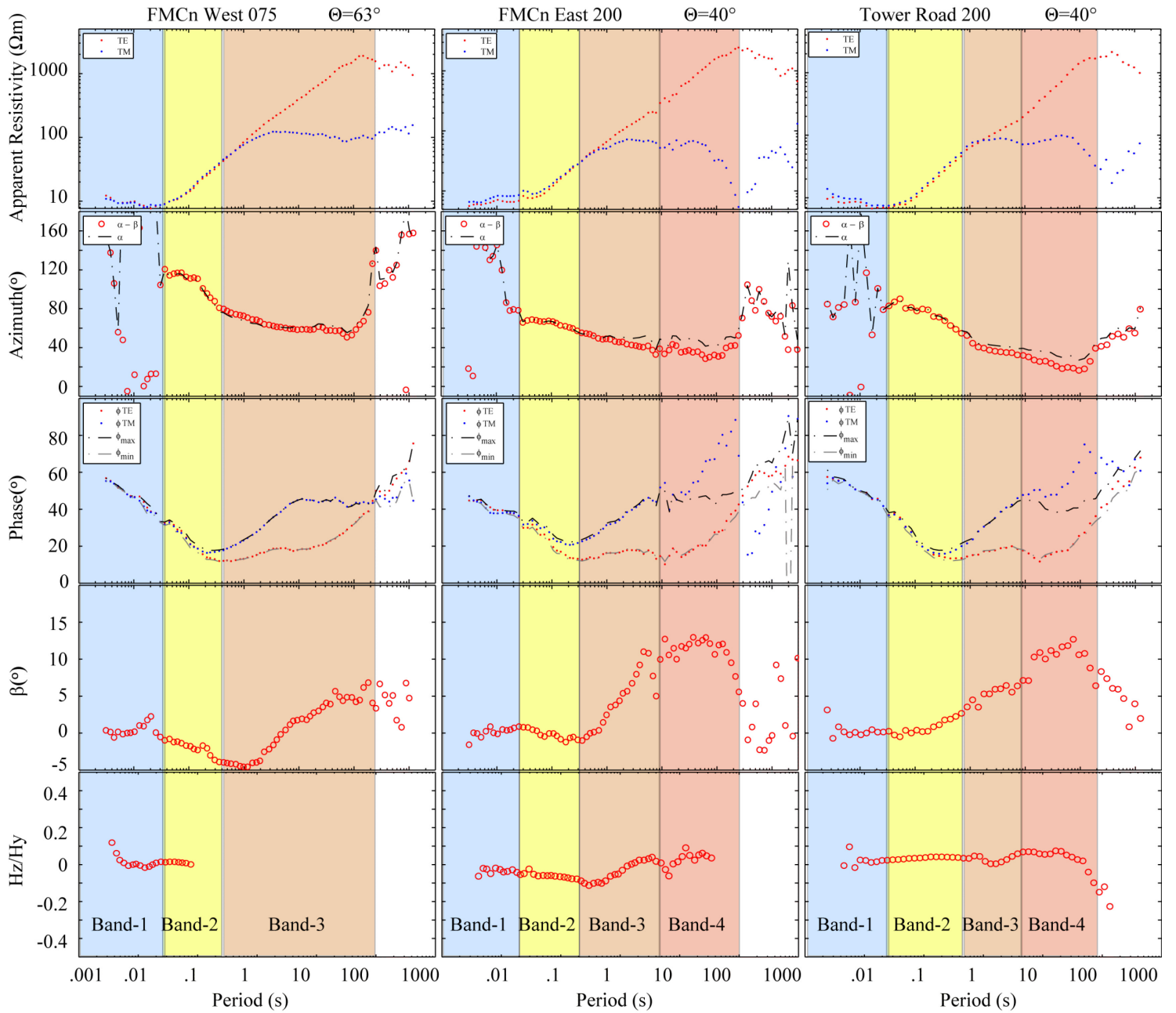
Figure 7.6: Phase tensor and distortion parameters from three stations typifying each of the three identified regions. (Left) FMCn West (Middle) FMCn East (Right) Tower Road. Upper panel is the TE/TM apparent resistivity post rotation to azimuthal coordinates. Second panel shows the ideal phase tensor azimuth as a function of period (red) and the distorted result due to skew (dashed line). Panel three plots the values of \phi_{max} and \phi_{min} against the natural TE/TM phase. Panel four shows the change in phase tensor skew \beta as a function of period. Panel 5 is the y-component tipper magnitude.
