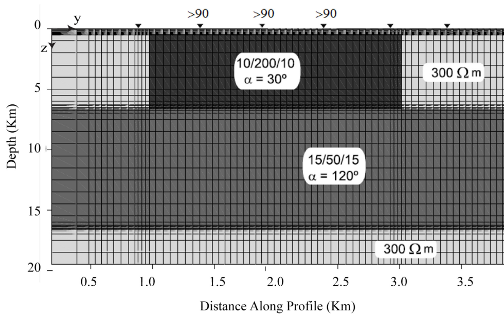
Figure 2.14: From Heise & Pous (2003). 2-D anisotropic model used to create higher than 90^\circ phase in stations places above the shallow block, marked by "> 90". Regional 2-D strike set to 0^\circ (into page). Numbers represent anisotropic resistivity values in directions following the pattern X/Y/Z. The angle \alpha represents the clockwise rotation of the anisotropic axes from the 2-D axes.
