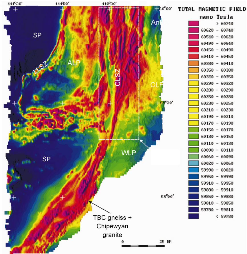
Figure 8.4: Total field aeromagnetic map for the exposed Canadian Shield in northern Alberta. ALP, Arch Lake pluton; AnLP, Andrew Lake pluton; CLSZ, Charles Lake shear zone; CLP, Colin Lake pluton; SP; Slave pluton, WLP, Wylie Lake pluton, TBC; Taltson basement complex. Modified from McDonough et al., (2000).
