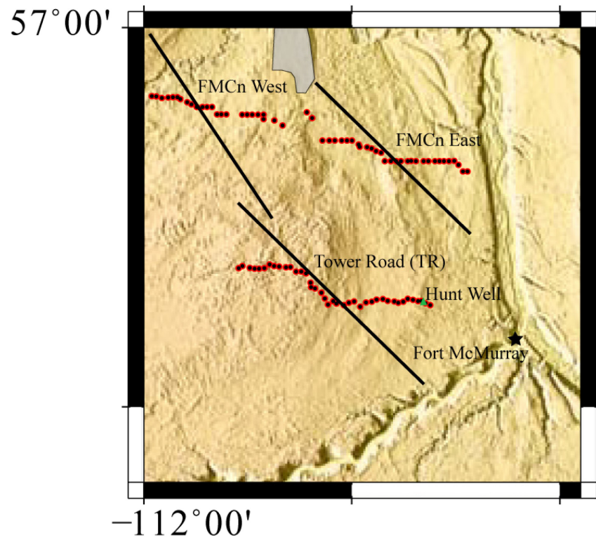
Figure 6.1: Location of the three 2-D MT profiles. The red dots show the location of the all of the MT stations in the FMC region. The black lines are oriented perpendicular to the strikes of each section, N40°E for FMCn East and TR, N63°E for FMCn West. The Hunt Well is indicated by the green triangle
