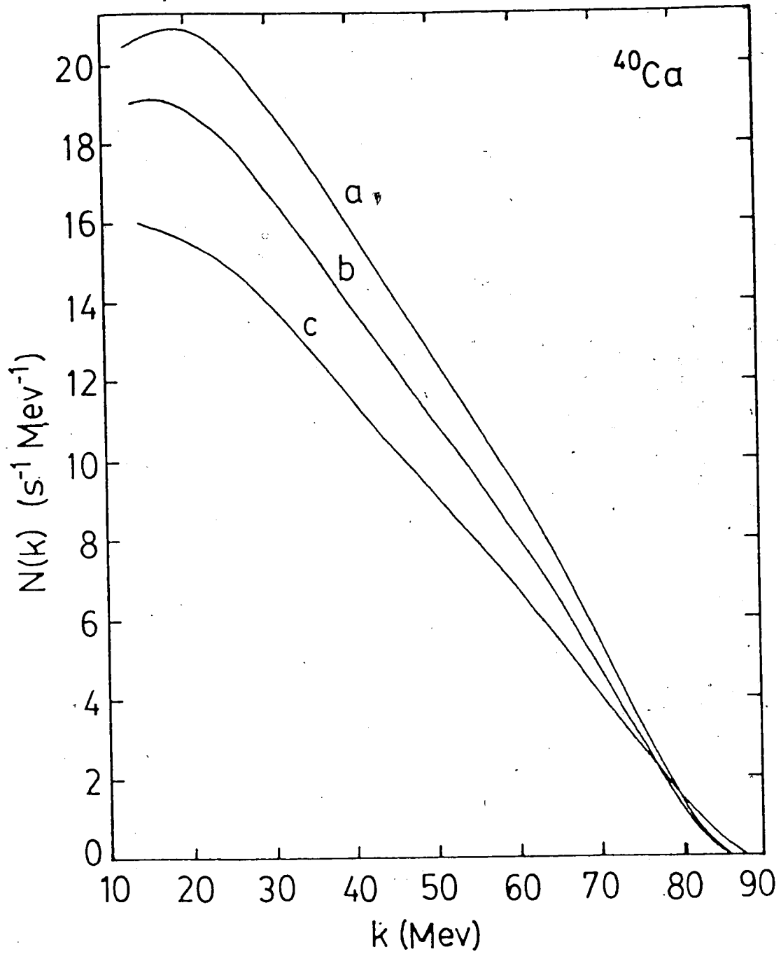
Fig. 15. Photon spectrum for ^{40}\text{Ca} calculated using SBL wave function
