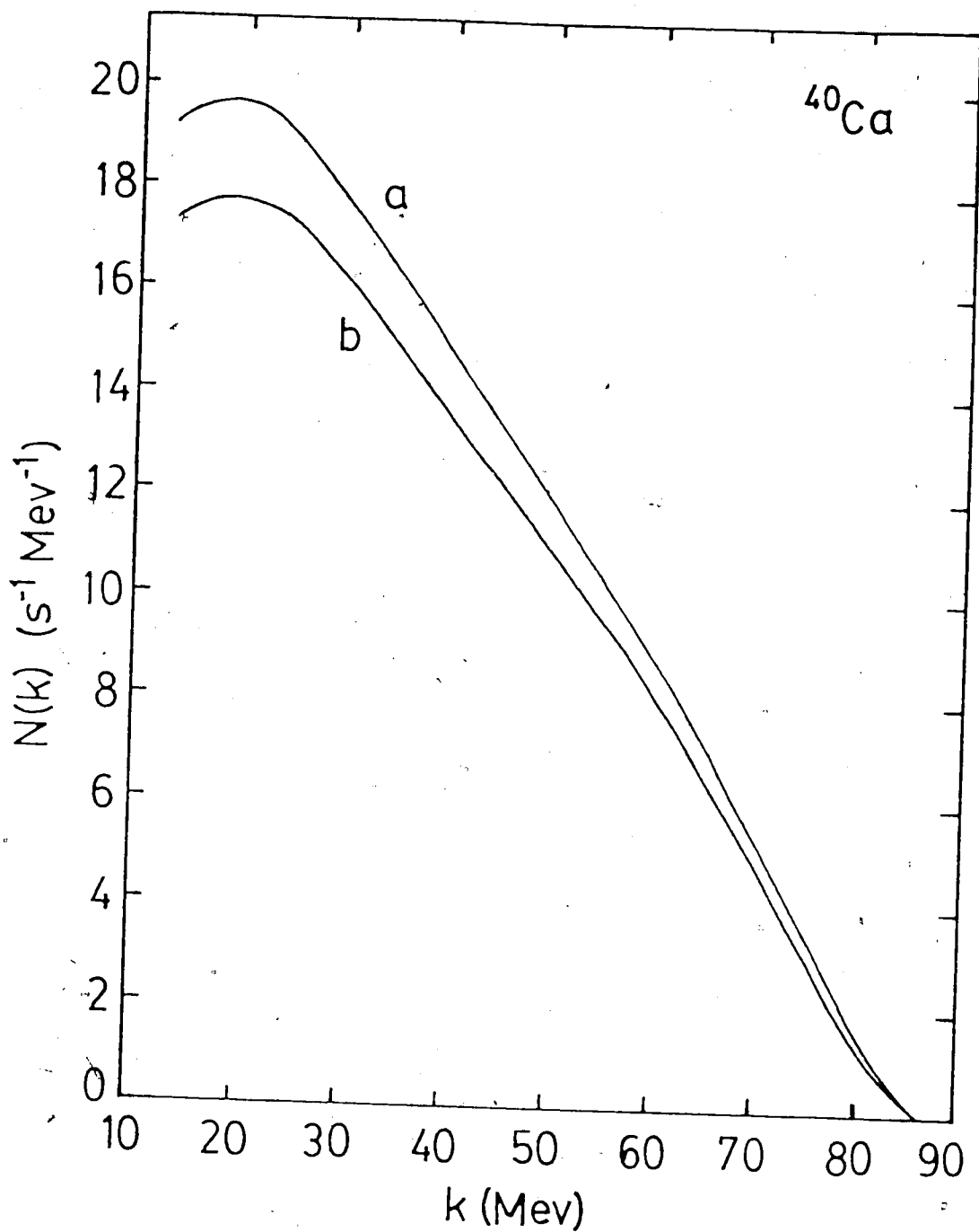
Fig. 6. Effect of neglecting the anomalous magnetic moment of the proton and neutron on the photon spectrum for ^{40}\text{Ca} , calculated in the CHO model a - complete O(1/m^2) result b - \chi_P = \chi_N = 0 .
