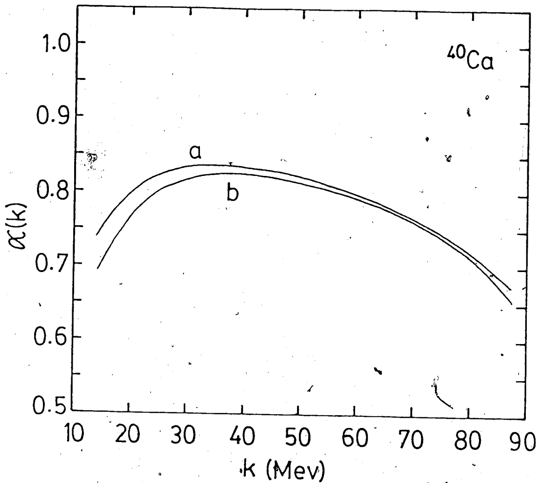
Fig. 25. Photon asymmetry for ^{40}\text{Ca} calculated in the GDR model to O(1/m^2) . a - CHO model O(1/m^2) result b - GDR model
