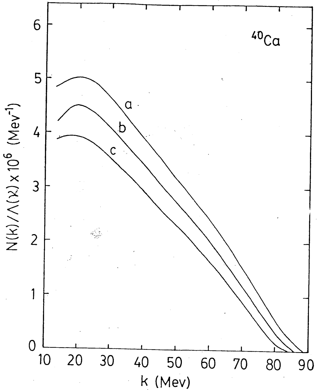
Fig. 17. Effect of varying the ratio k_m/\nu on the relative photon spectrum for ^{40}\text{Ca} . The average neutrino energy was fixed at \nu = 85 Mev. The ordinary capture rate is \Lambda = 4.36 \times 10^6/\text{s} .
