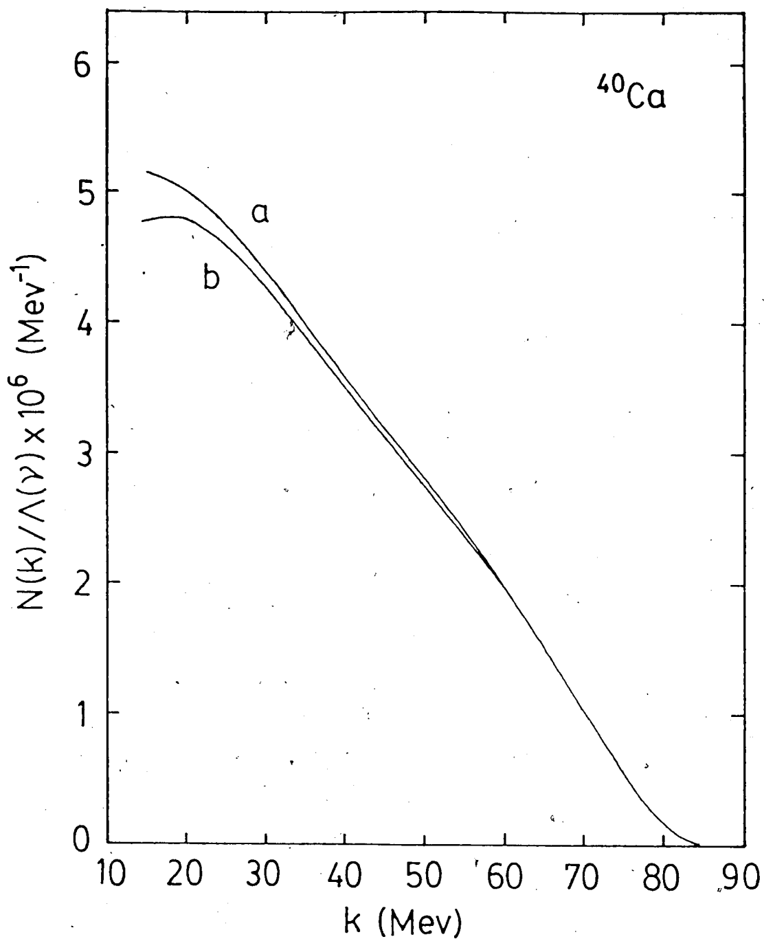
Fig. 18. ^{40}\text{Ca} relative photon spectrum for the best parameter choices \gamma=79 Mev, k_m=84 Mev, calculated in the CHC model. The ordinary capture rate \Lambda is also given. \Lambda_{exp}=(2.29\pm 0.06)\times 10^6/\text{s} . (Ha 77) a - SBL wave function; \Lambda=3.13\times 10^6/\text{s} b - simple wave function; \Lambda=3.37\times 10^6/\text{s} .
