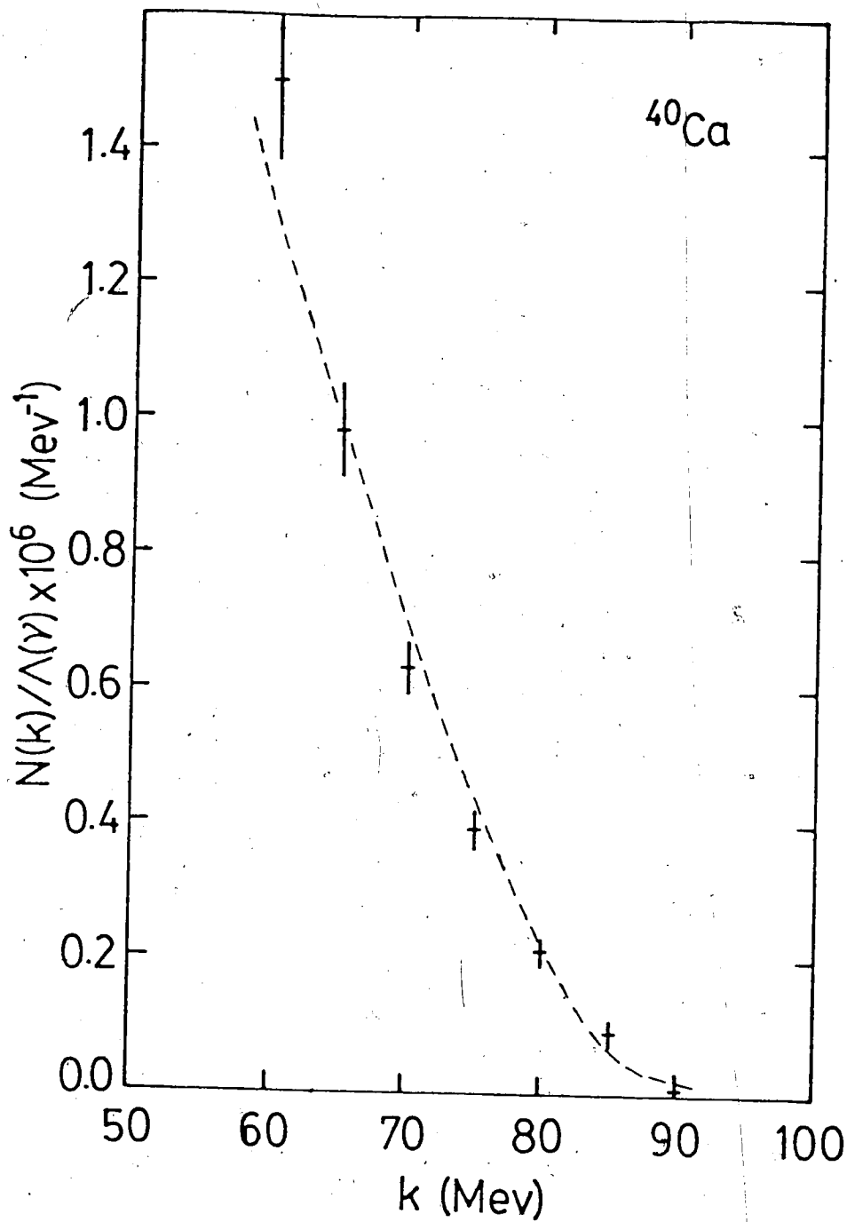
Fig. 22. Two-parameter fit to the relative photon spectrum of Hart et al (Ha 77) using the GDR model with the SHO wave function and k_m/\gamma=1.06 . Results for the fitted parameters are k_m=87.0\pm 3.0 Mev, g_p=(-0.3\pm 2.0)g_n . The ordinary capture rate is \Lambda=3.9\times 10^6/s .
