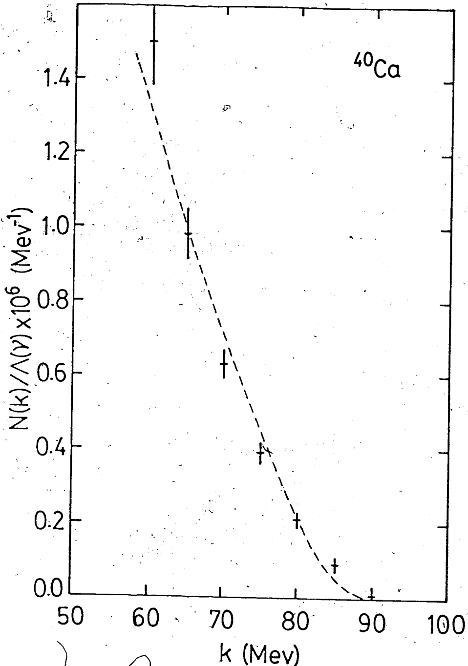
Fig. 21. Two-parameter fit to the relative photon spectrum of Hart et al (Ha 77) using the CHO model with the SHO wave function and k_m/\gamma = 1.06 . Results for the fitted parameters are k_m = 89.1 \pm 0.9 Mev, g_p = (-2.8 \pm 4.8) g_A . The ordinary capture rate is \Lambda = 5.3 \times 10^6/\text{s} .
