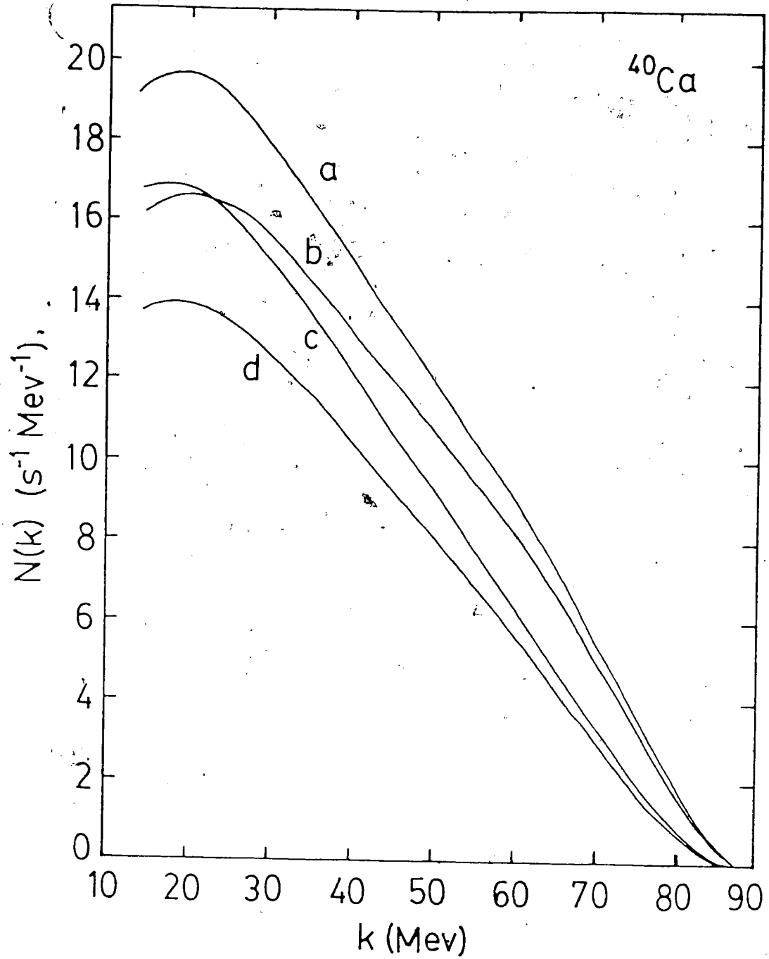
Fig. 5. Contribution to the ^{40}\text{Ca} photon spectrum from the weak magnetism and induced pseudoscalar couplings a - complete O(1/m^2) result, standard couplings b - g_M=0 c - g_P=0 d - g_M=g_P=0
