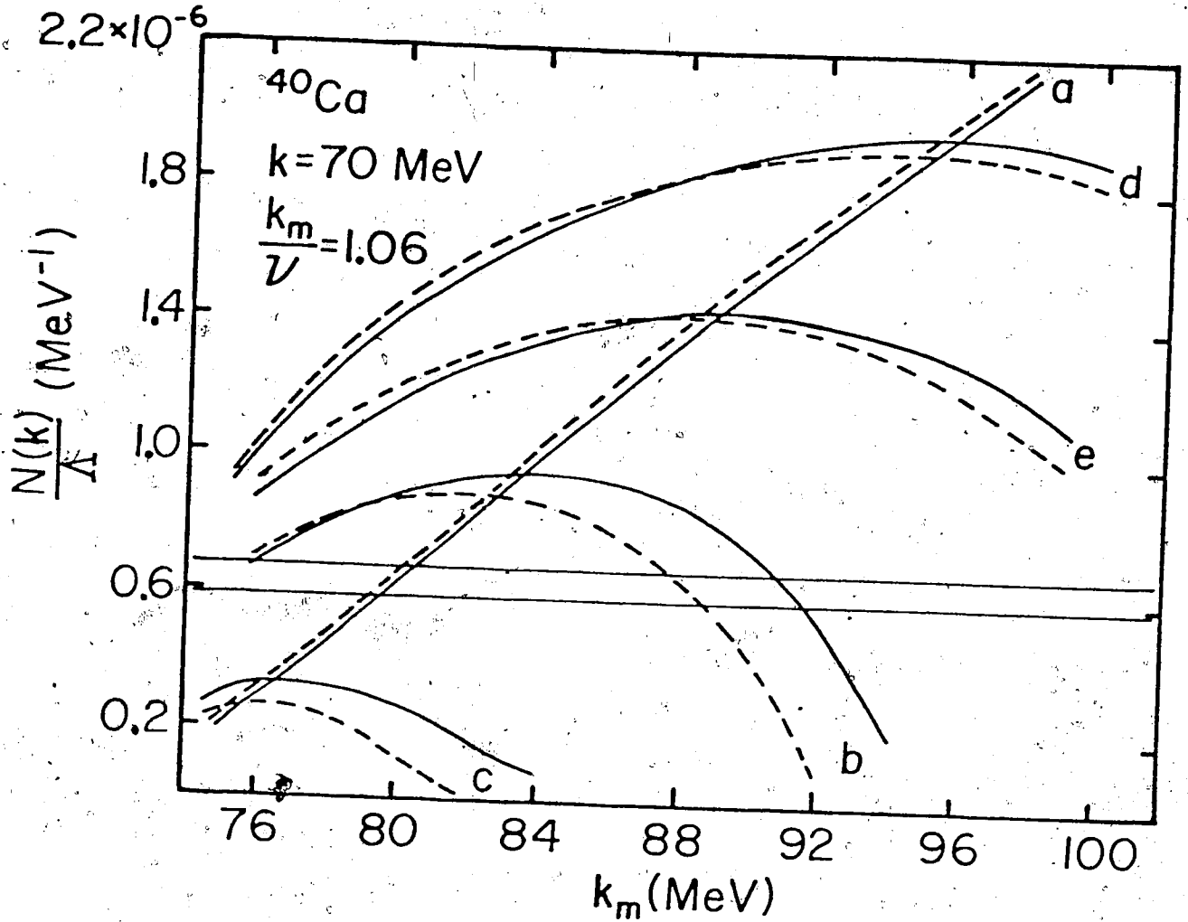
Fig. 31. Influence of the Coulomb energy shift and velocity terms on the ^{40}\text{Ca} relative capture rate for k=70 Mev and k_m/v=1.06 . Results including velocity terms (solid curves) and not including them (dashed curves) are shown for two choices of the phenomenological factor \delta and with and without the Coulomb energy shift E_c . The horizontal lines are experimental bounds on N(k)/A from (Ha 77) a - usual closure result b - \delta=1.15 , E_c=7.1 Mev c - \delta=1.15 , E_c=0 d - \delta=0 , E_c=7.1 Mev e - \delta=0 , E_c=0 .
