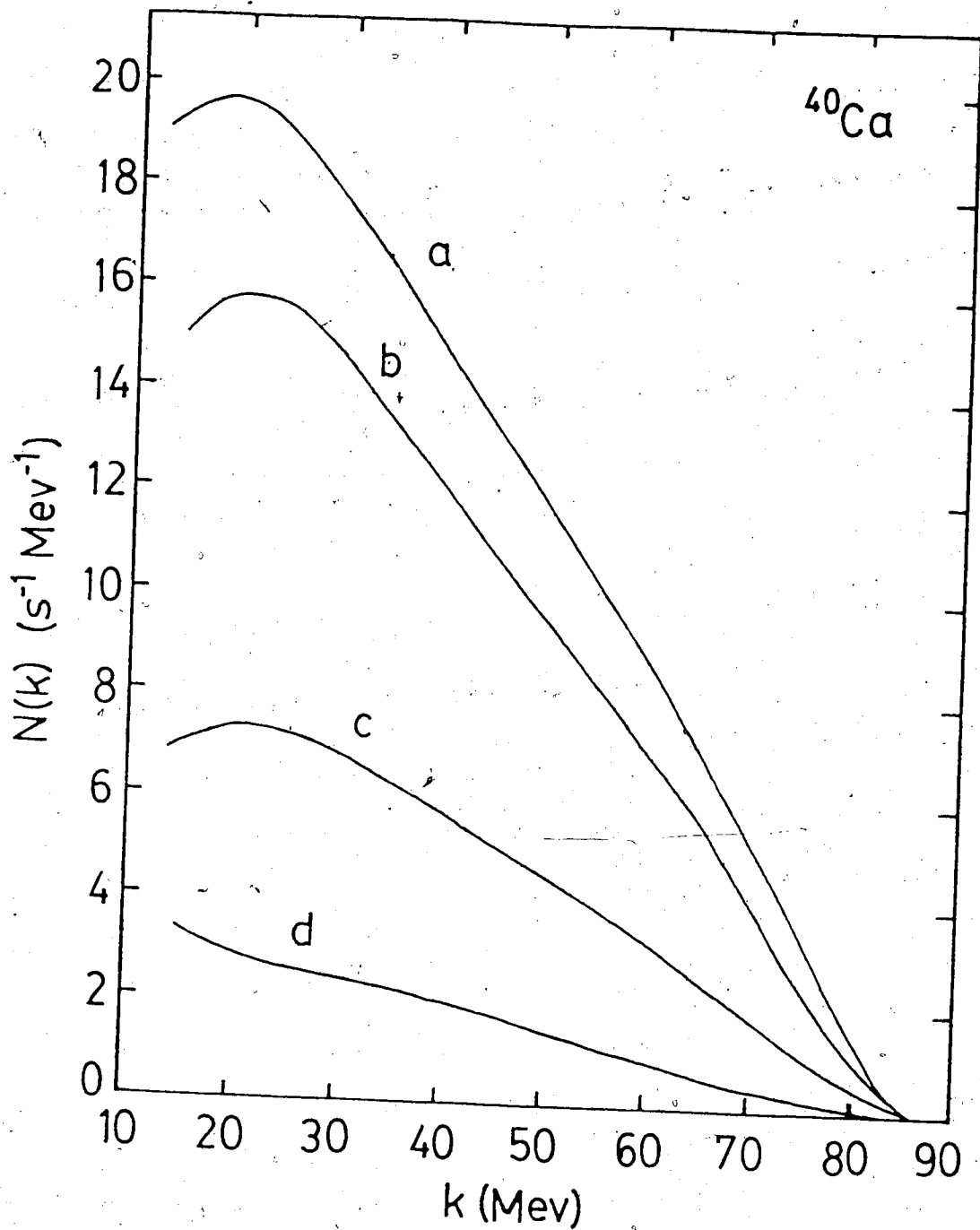
Fig. 3. Decomposition of the photon spectrum for ^{40}\text{Ca} according to powers of (1/m) appearing in the squared matrix element, and the contribution of the velocity terms, calculated in the CHO model a - through O(1/m^2) b - through O(1/m) c - through O(1) d - velocity terms through O(1/m^2) .
