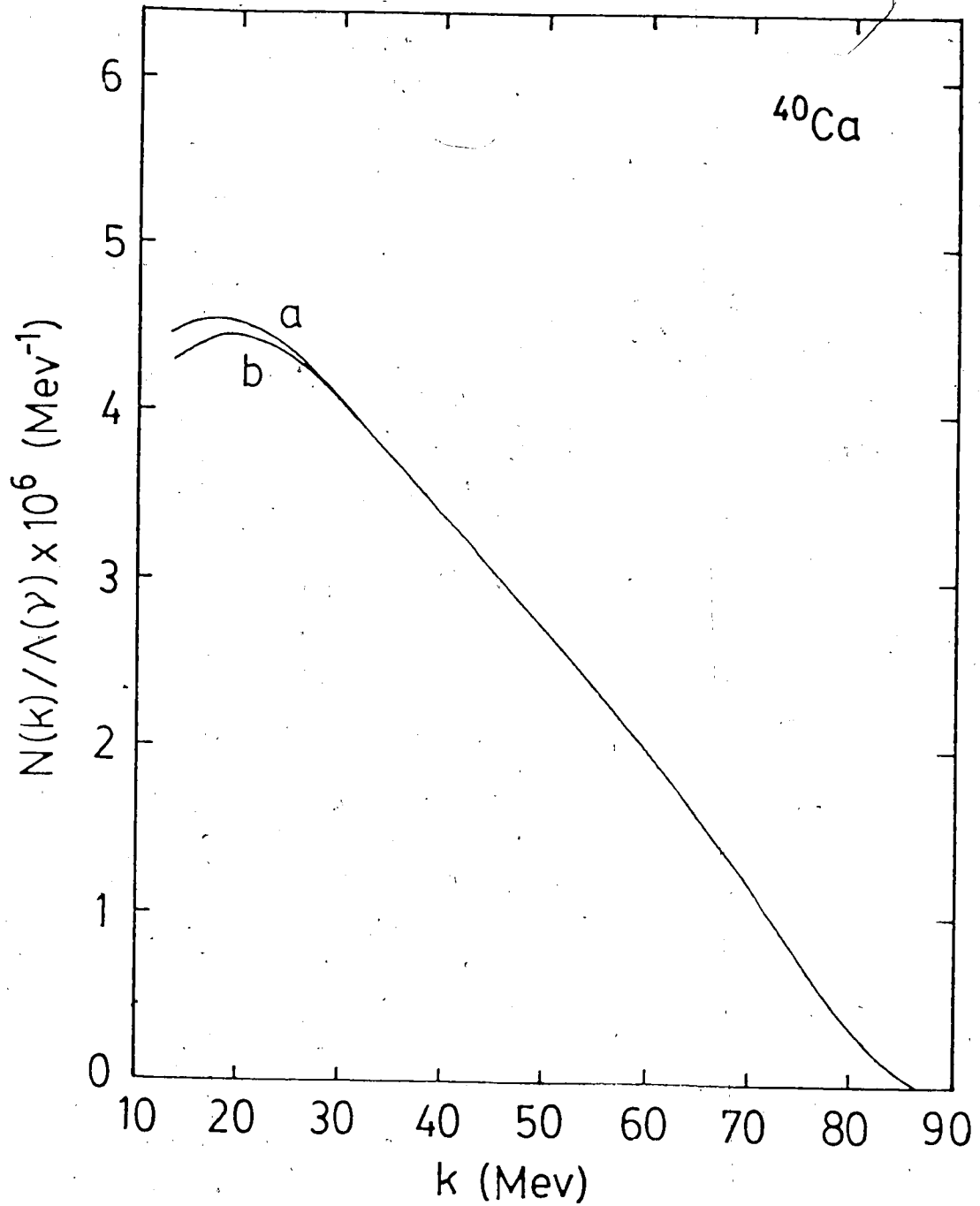
Fig. 13. Effect of varying the oscillator parameter b on the relative photon spectrum for ^{40}\text{Ca} , calculated in the CHO model. The ordinary capture rate \Lambda is also given.
