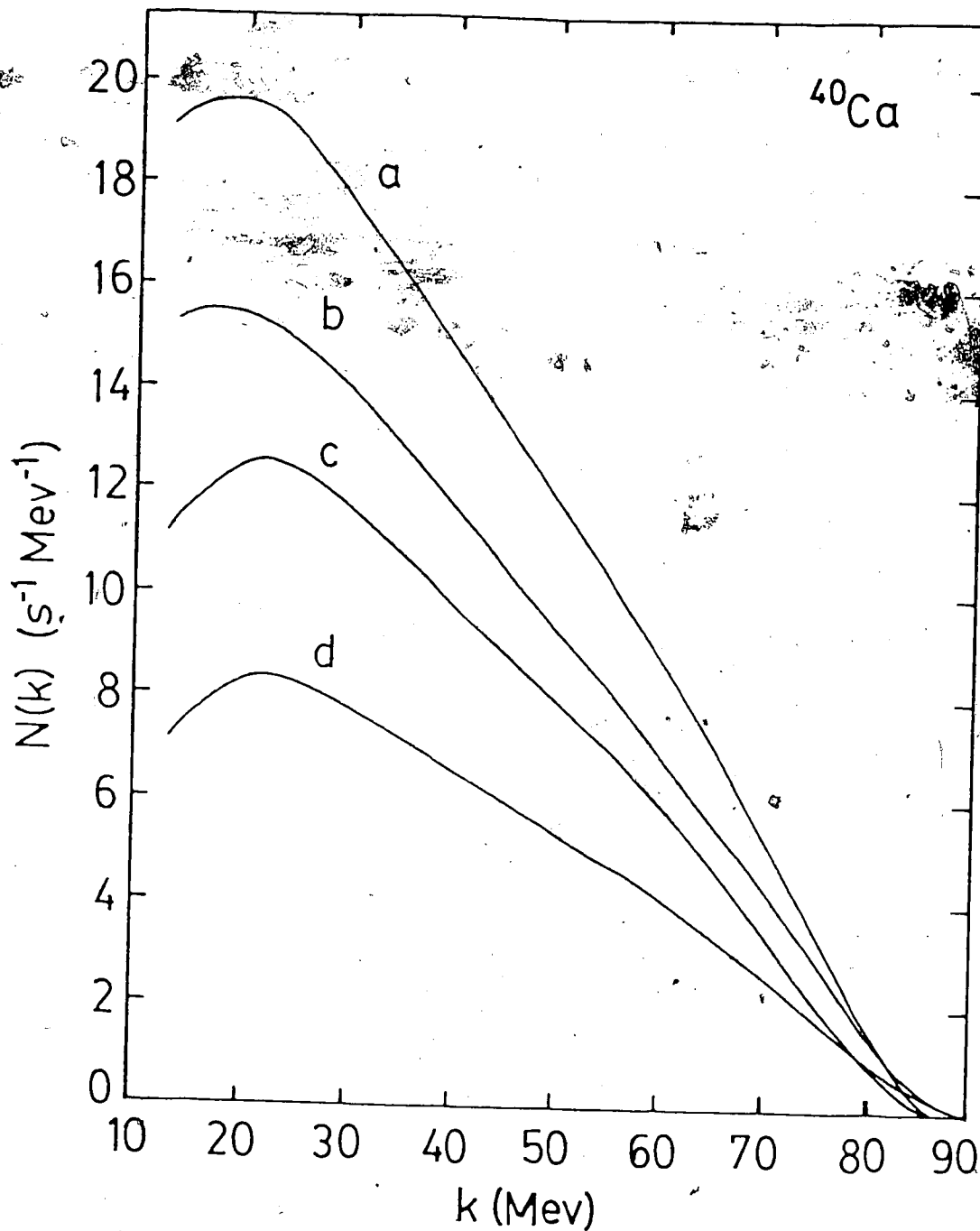
Fig. 9. Dipole contribution to the photon spectrum for ^{40}\text{Ca} a - complete spectrum, CHO model b - complete spectrum, GDR model c - dipole part, CHO model d - dipole part, GDR model.
