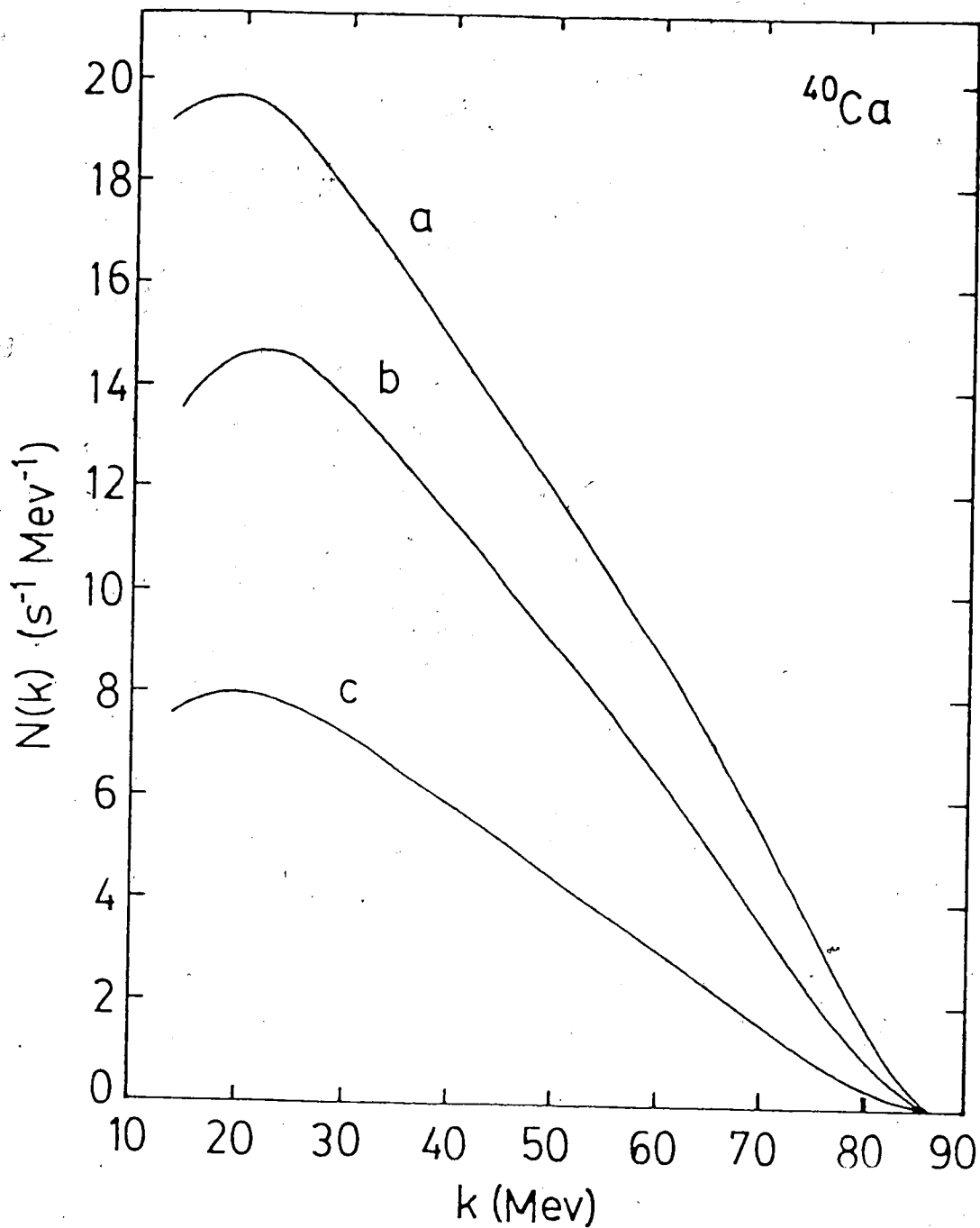
Fig. 4. Contribution of the muon radiating diagram and its interference with all other standard theory diagrams to the photon spectrum for ^{40}\text{Ca} , calculated in the CHO model a - complete O(1/m^2) result b - muon radiating diagram plus interferences c - muon radiating diagram alone.
