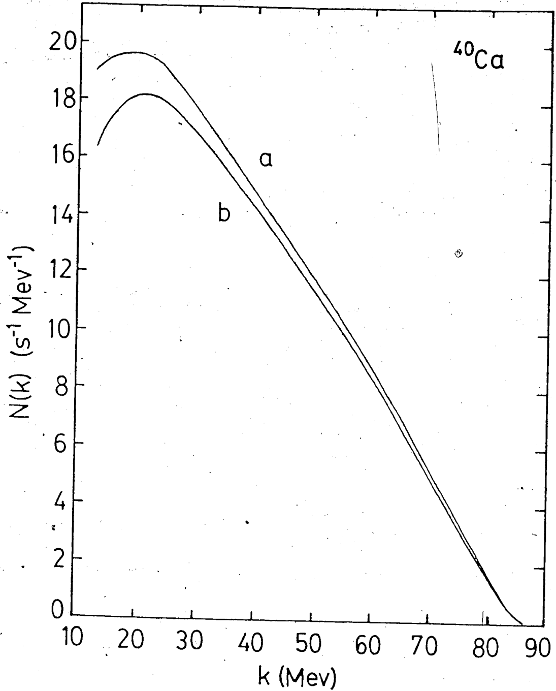
Fig. 2. Contribution of previously neglected O(1/m^2) terms in the squared matrix element to the photon spectrum for ^{40}\text{Ca} , calculated in the CHO model a - our O(1/m^2) result b - using the squared matrix element from Fearing (Fe 66).
