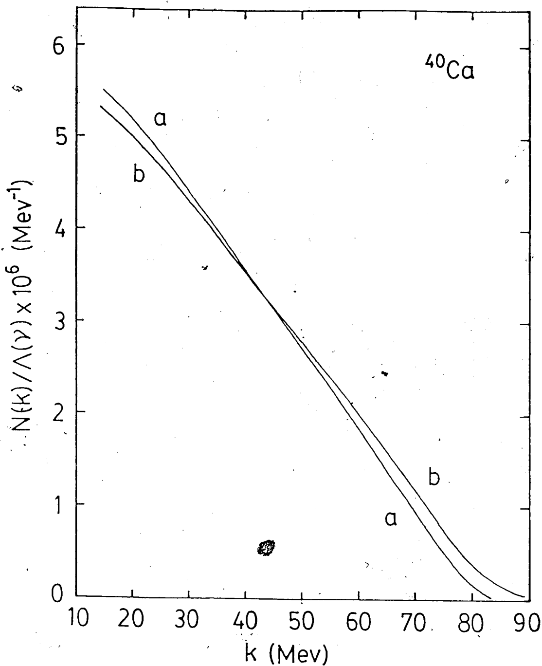
Fig. 20. ^{40}\text{Ca} relative photon spectrum for the axial vector strength quenched 25%. The SBL wave function and best parameter choices \gamma=79 Mev, k_m=84 Mev were used with g_A=-0.9 , g_p=-6.3=7xg_A . The ordinary capture rate \Lambda is also given a - CHO model; \Lambda=2.05 \times 10^6/\text{s} b - GDR model; \Lambda=1.98 \times 10^6/\text{s} .
