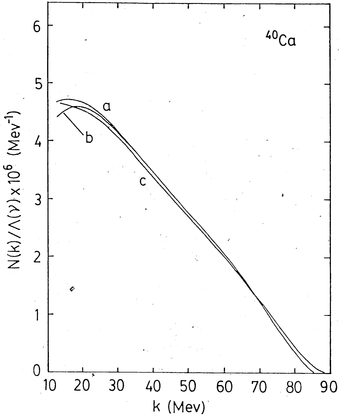
Fig. 16. Relative photon spectrum for ^{40}\text{Ca} calculated using the SBL wave function. The ordinary capture rate \Lambda is also given.
