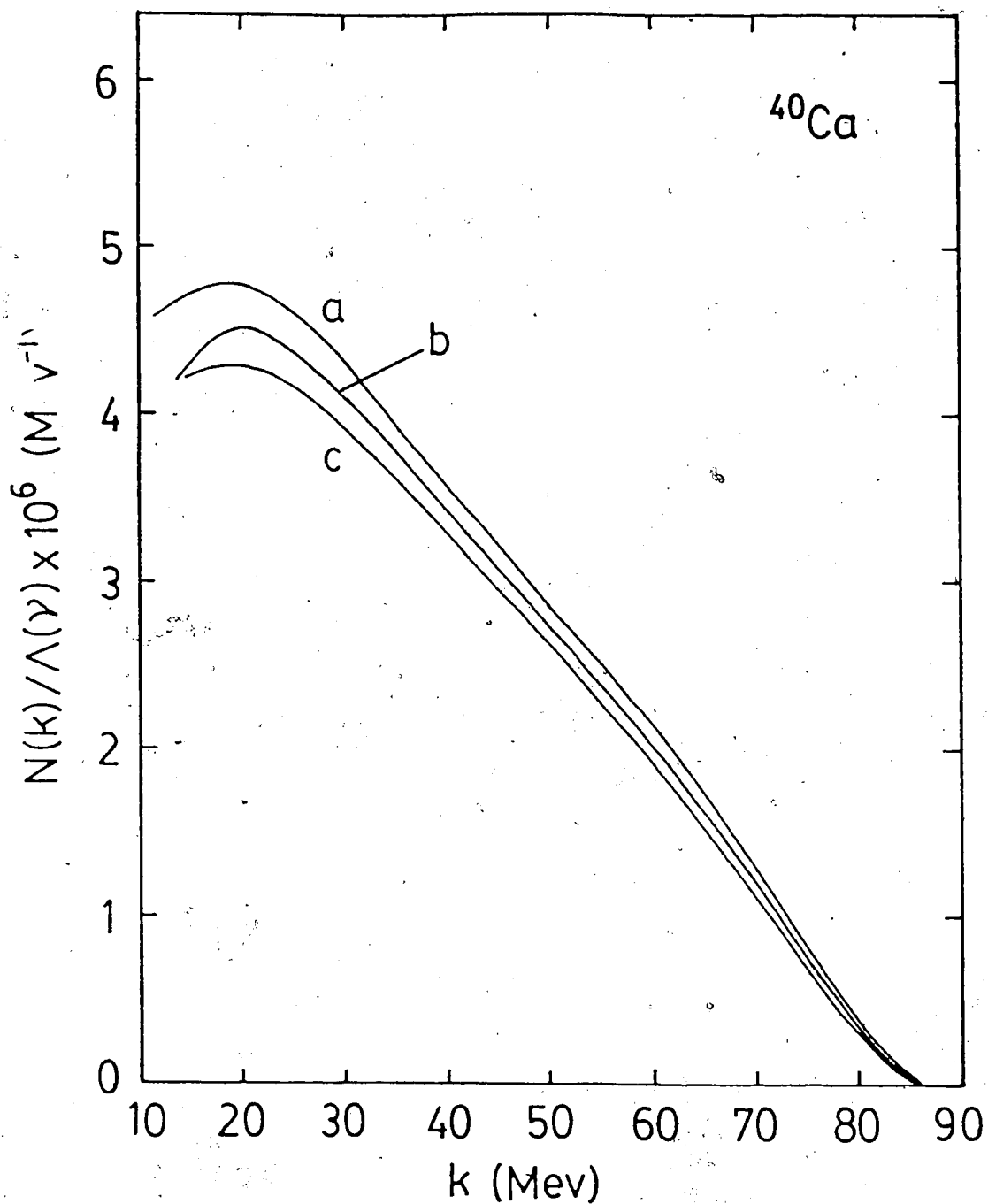
Fig. 11. Effect of varying g_T on the relative photon spectrum for ^{40}\text{Ca} , calculated in the CHO model. The ordinary capture rate \Lambda is also given.
