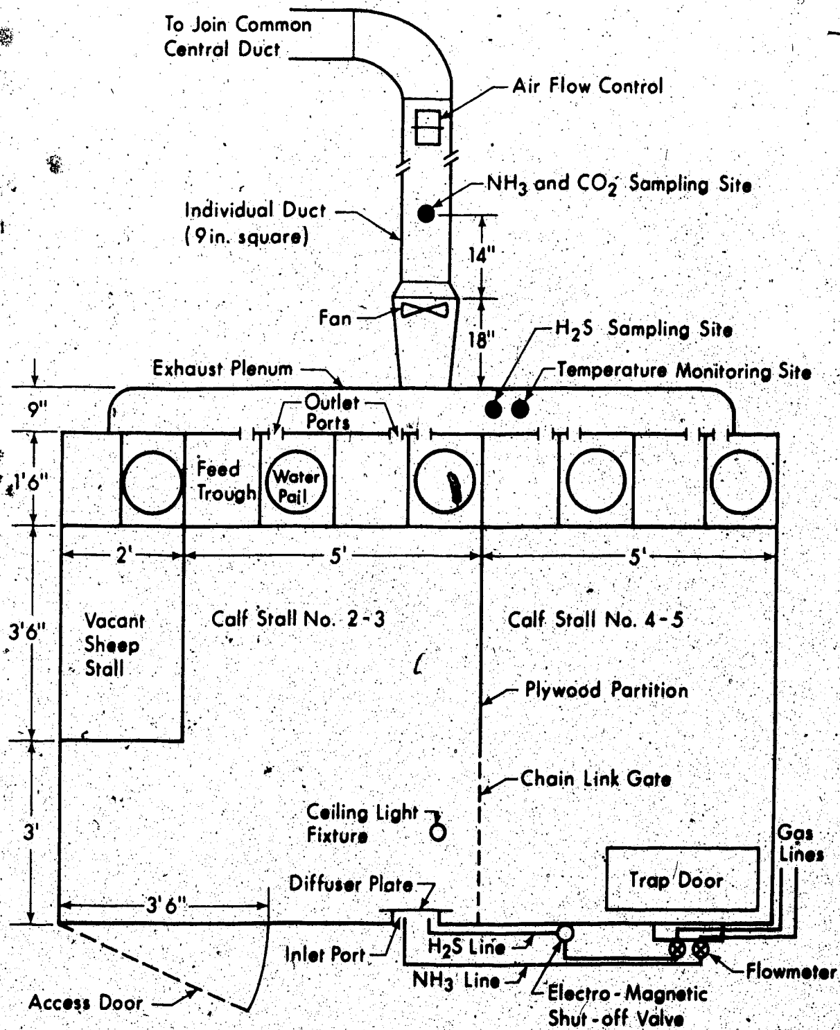
Figure 4. Plan view of an animal exposure chamber.
