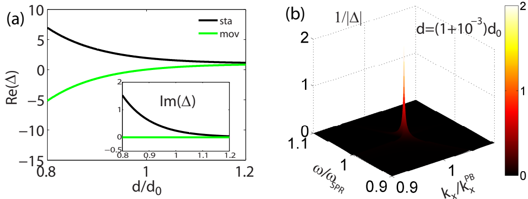
Figure 3: (a) Values of multi-reflection factor \Delta as a function of distance at the phase balance wavevector and SPR frequency. The fact that \text{Im}(\Delta) = 0 holds true for all distances in the moving plates, which is not valid for the stationary case. For moving plates at the phase balance wavevector, \Delta crosses zero at the critical distance ( d_0 ). However, for stationary plates, \Delta can never be exactly zero, which is clear from the plot. (b) The denominator in the expression of photon transfer ( 1/|\Delta| ) resolved by frequency and lateral wavevector k_x at d \rightarrow d_0^+ ( d = (1 + 10^{-3})d_0 ). Note the huge peak in the middle located at the phase balance wavevector and the SPR frequency, where the PAB condition leads to a vanishing \Delta . In both (a) and (b), we take k_y = 0 .
