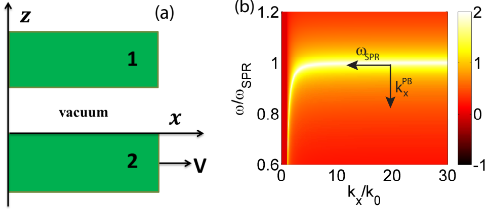
Figure 1: (a) Schematic of the work. Two half-space plates composed of the same medium are separated by a vacuum gap. One plate is moving at a constant velocity V along the its interface ( x direction). (b) Magnitude of reflection coefficient from a stationary plate of Drude metal in log scale, which depicts the enhancement in the reflection coefficient due to the surface plasmon resonance (SPR). The special phase balance wavevector is k_x^{PB} \approx 20k_0 at a velocity of V = c/10 and \omega_{SPR} = 10^{15}\text{Hz} which leads to the unique mapping of the SPR resonance frequency of the moving plate to the negative SPR resonance frequency of the stationary plate ( \omega'_{SPR} = -\omega_{SPR} ).
