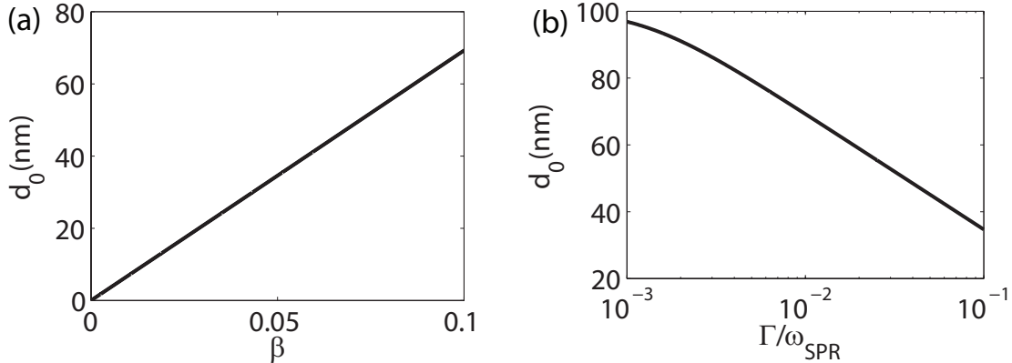
Figure 2: The opposing effects of increasing velocity and damping on the singular resonance condition. (a) Critical distance varying with moving velocity. The critical distance increases linearly versus moving velocity, in agreement with Eq. 22. (b) As the Drude damping increases, the critical distance where the resonance occurs decreases. This is expected since the amplitude balance condition is sensitive to loss in the surface plasmon resonance and occurs only if the plates are in the extreme near-field.
