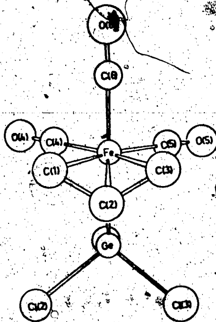
Molecular Structure of (C_3H_5)Fe(CO)_3GeCl_3
