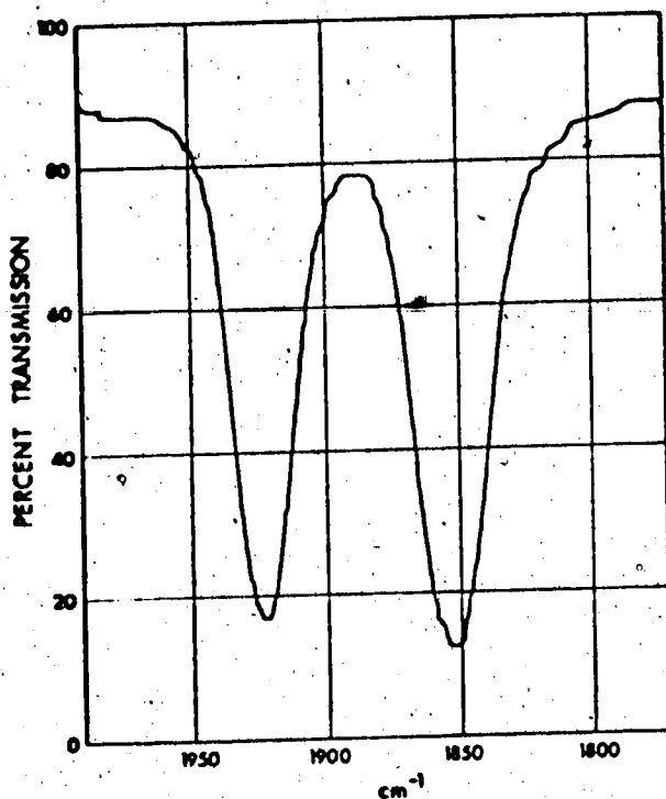
[\text{Et}_4\text{N}][\text{CpRe}(\text{CO})_2\text{GeCl}_3]
