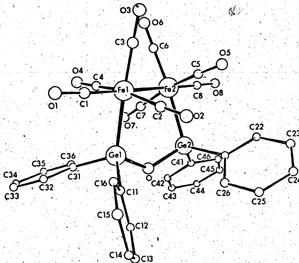
Molecular Structure of [(\text{Ph}_2\text{Ge})_2\text{O}]\text{Fe}_2(\text{CO})_8
