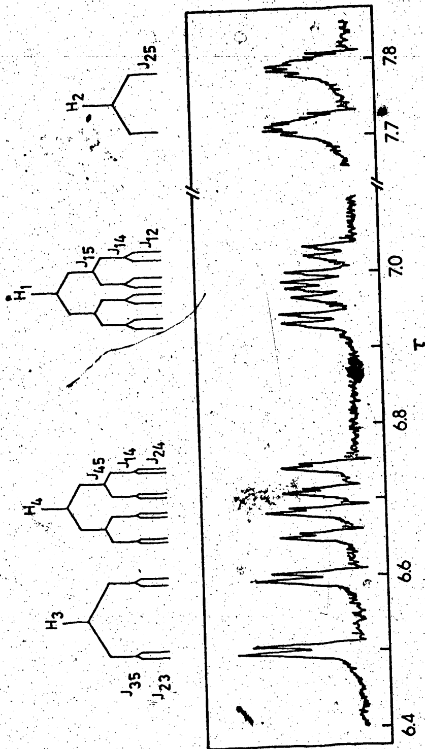
Methylene Proton Resonances in \text{Cp}(\text{C}_3\text{H}_5)\text{Re}(\text{CO})\text{Br}
