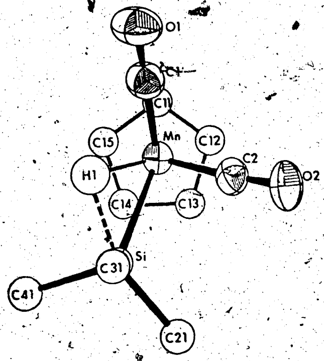
Molecular Structure of cis -CpMn(CO) 2 (SiPh 3 )H Phenyl rings omitted for clarity.
