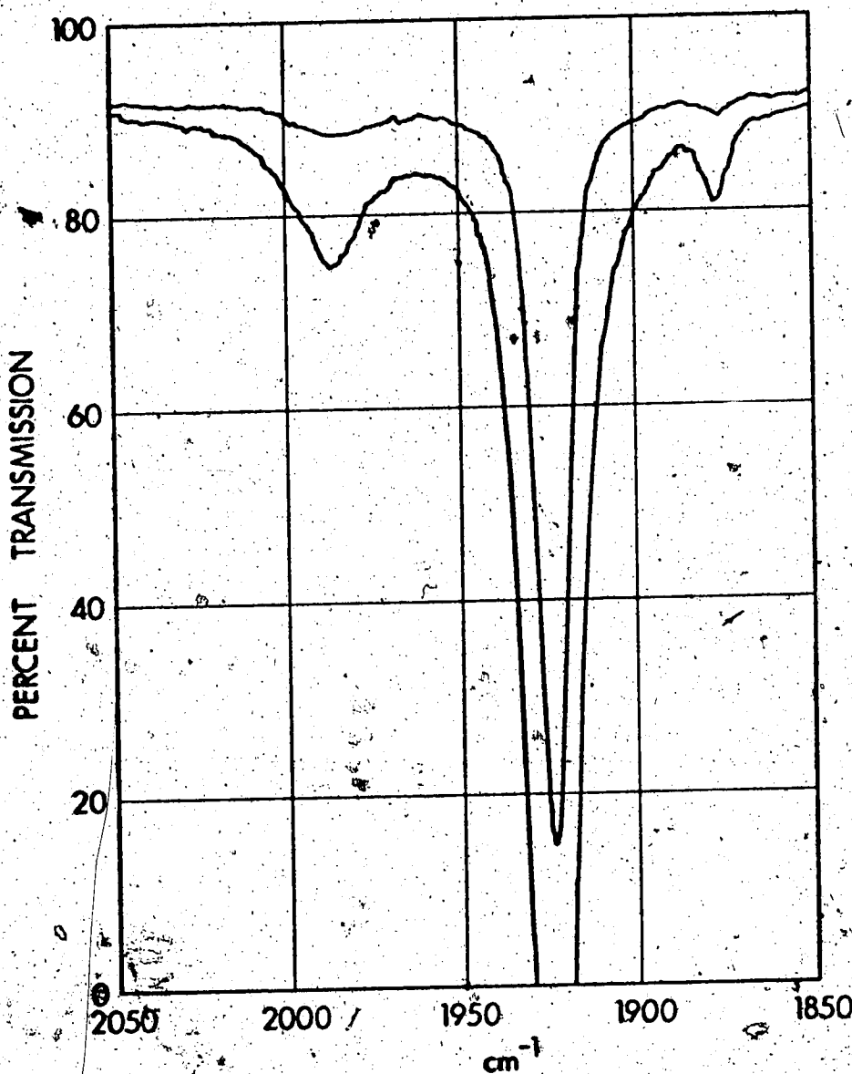
\text{Cp}(2\text{-C}_4\text{H}_7)\text{Re}(\text{CO})\text{H}
