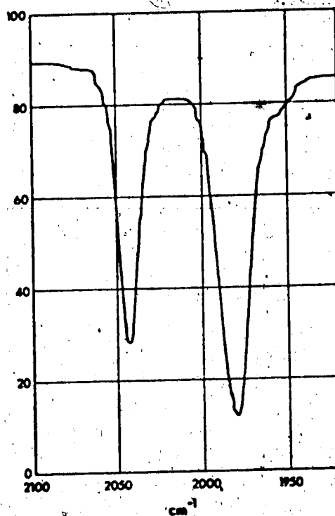
trans - \text{CpRe}(\text{CO})_2(\text{GeCl}_3)\text{H}
