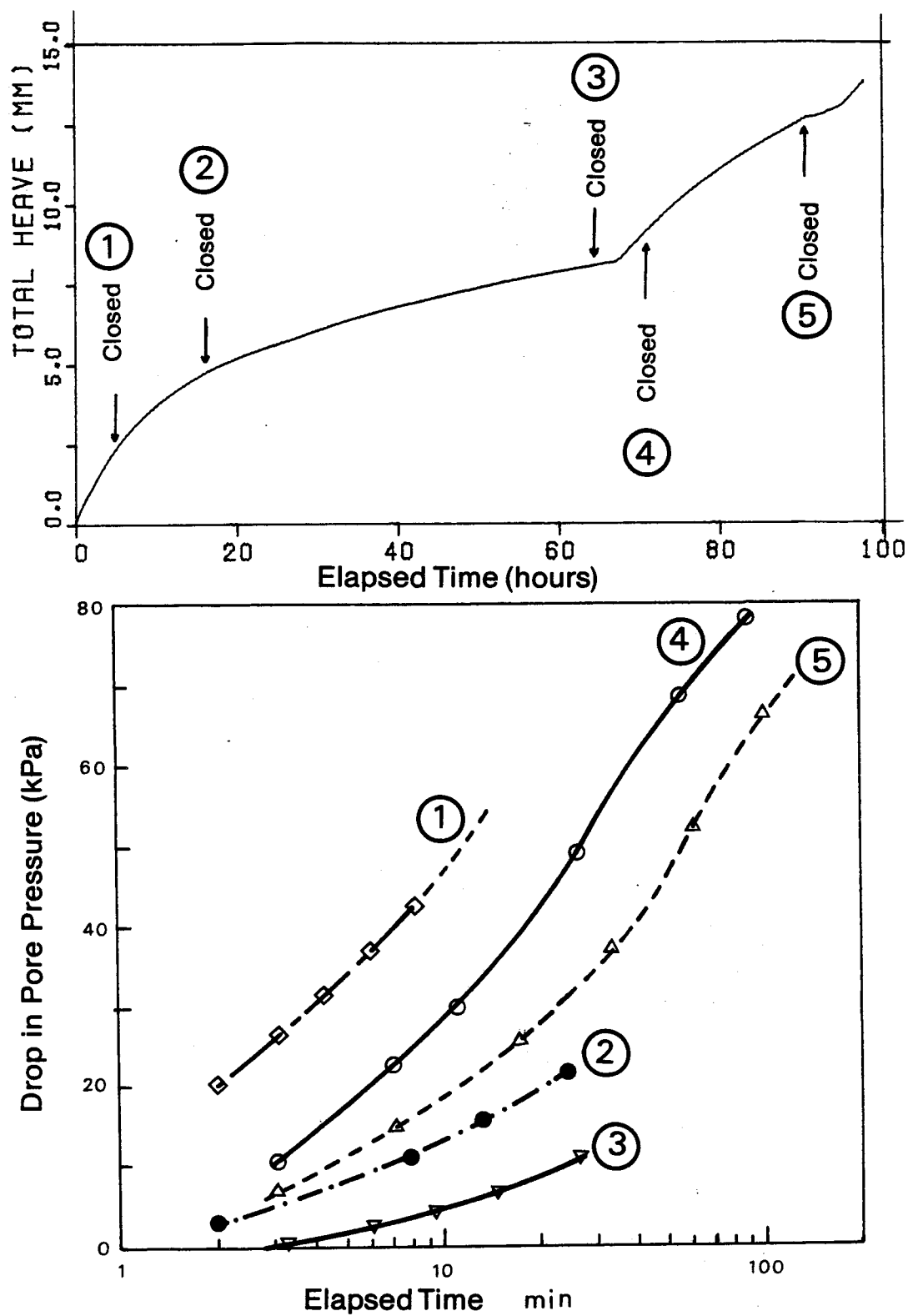
Figure 5.4 Pore Pressure Measurements in Test S1
