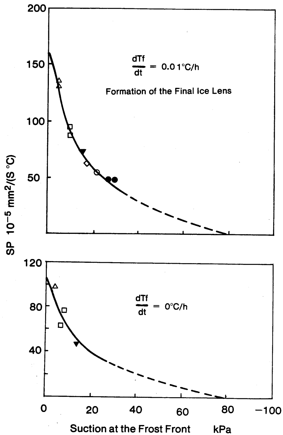
Figure 4.13 Freezing Characteristics for Devon Silt
