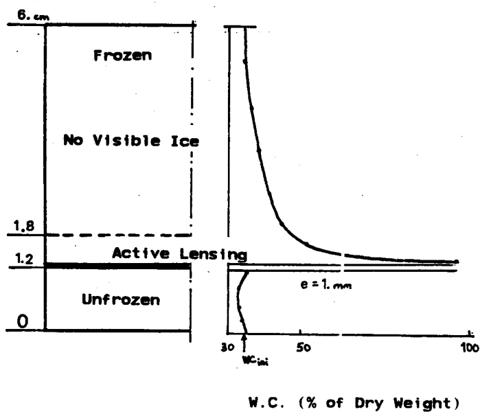
Figure E.10 Experimental Results From Test C-11. P_e=120 kPa
