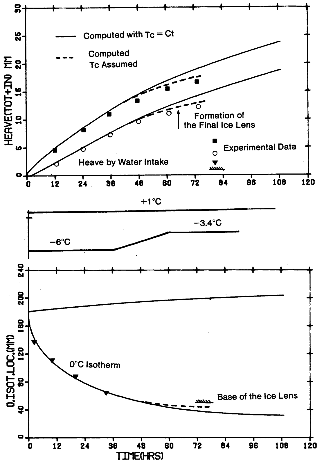
Figure 4.25 Comparison of Prediction with Actual Data for Test NS-10
