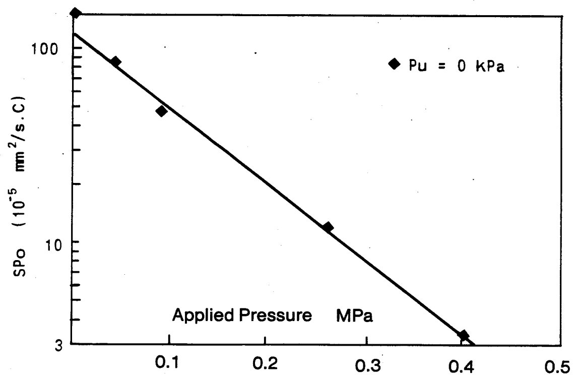
Figure 7.3 Segregation Potential for Devon Silt
