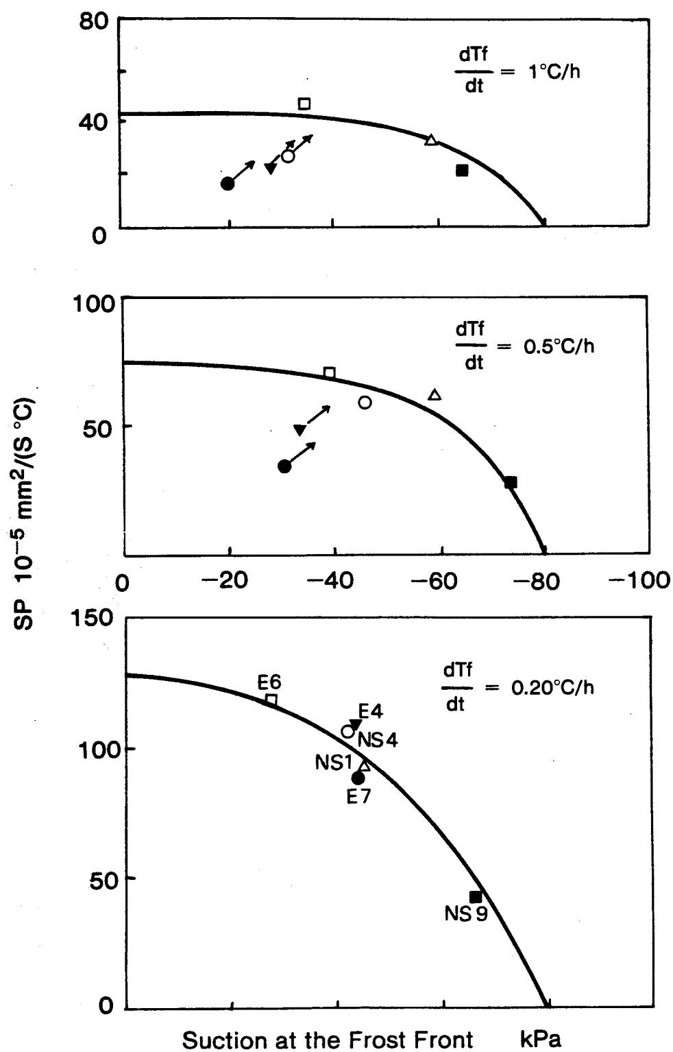
Figure 4.11 Freezing Characteristics for Devon Silt
