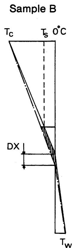
Figure 4.8 Changes in Frozen Fringe at a Given Rate of Frost Front Advance
