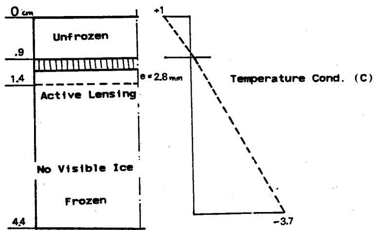
Figure E.11 Experimental Results From Test C-12. P_e = 120 \text{ kPa}
