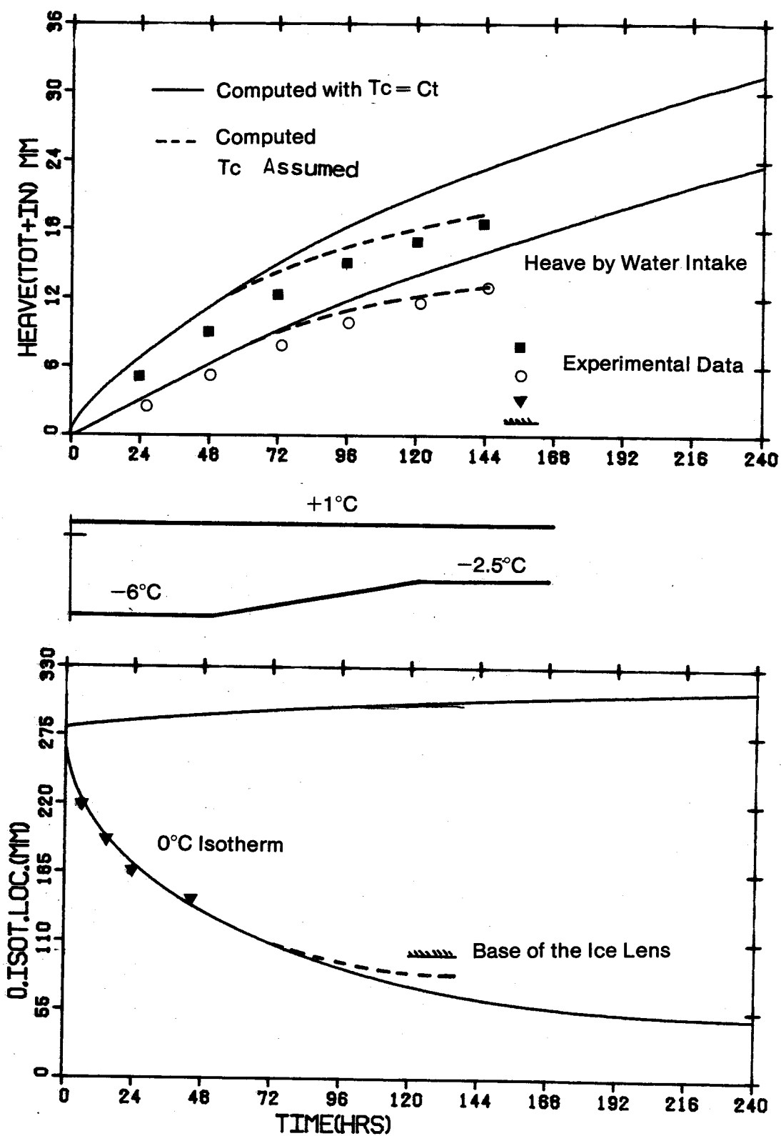
Figure 4.24 Comparison of Prediction with Actual Data for Test NS-9
