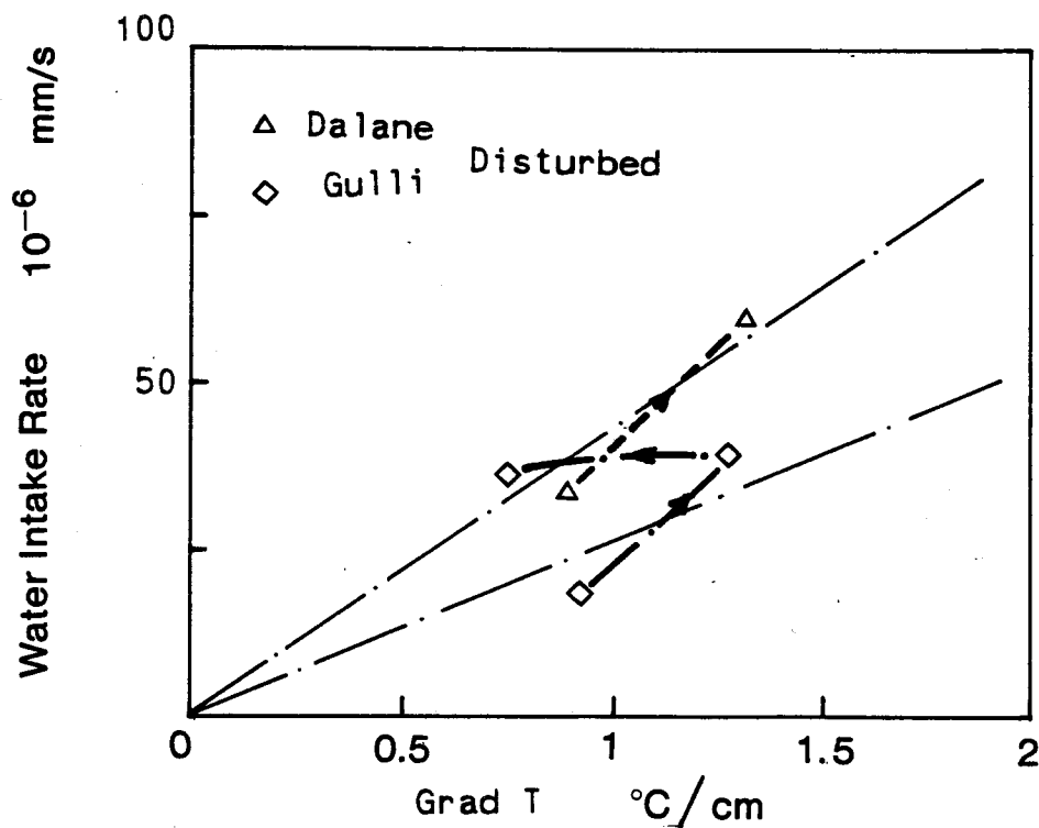
Figure 7.2 Experimental Results Obtained by Loch (1979)
