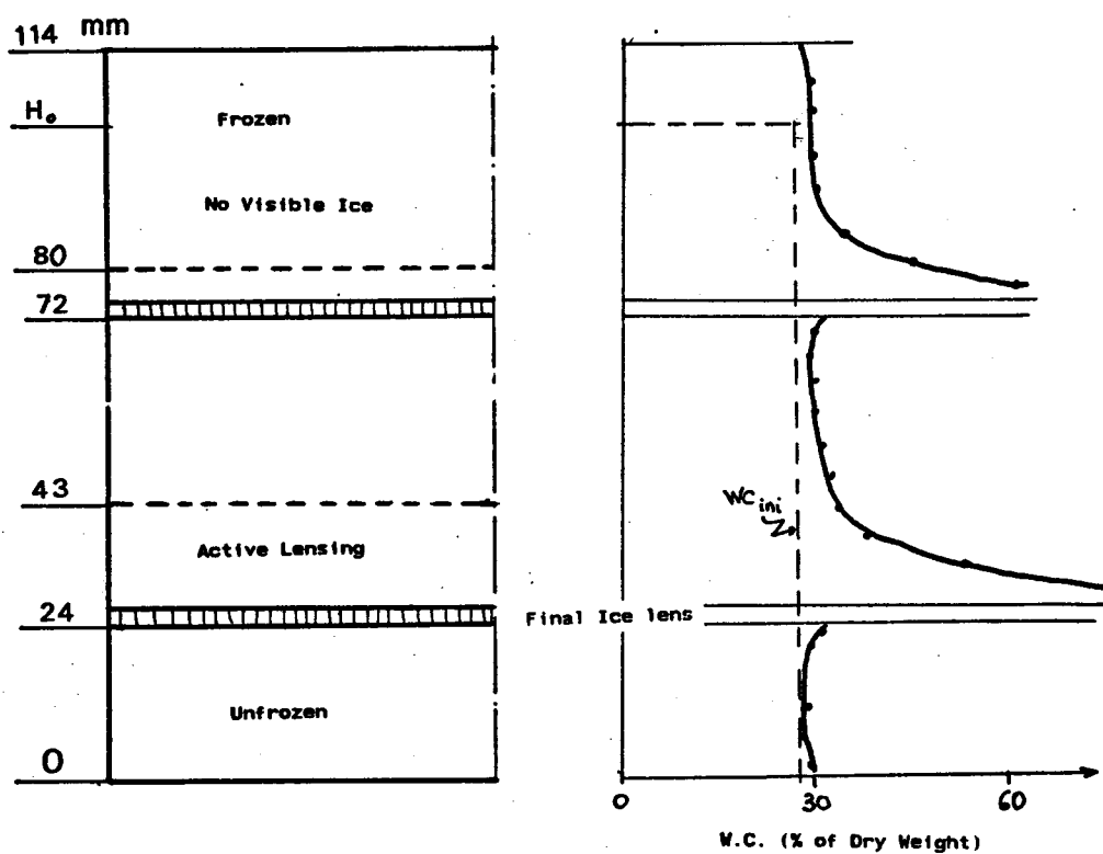
TEST S-8 (P=50.KPA;2 FREEZING FRONTS)
