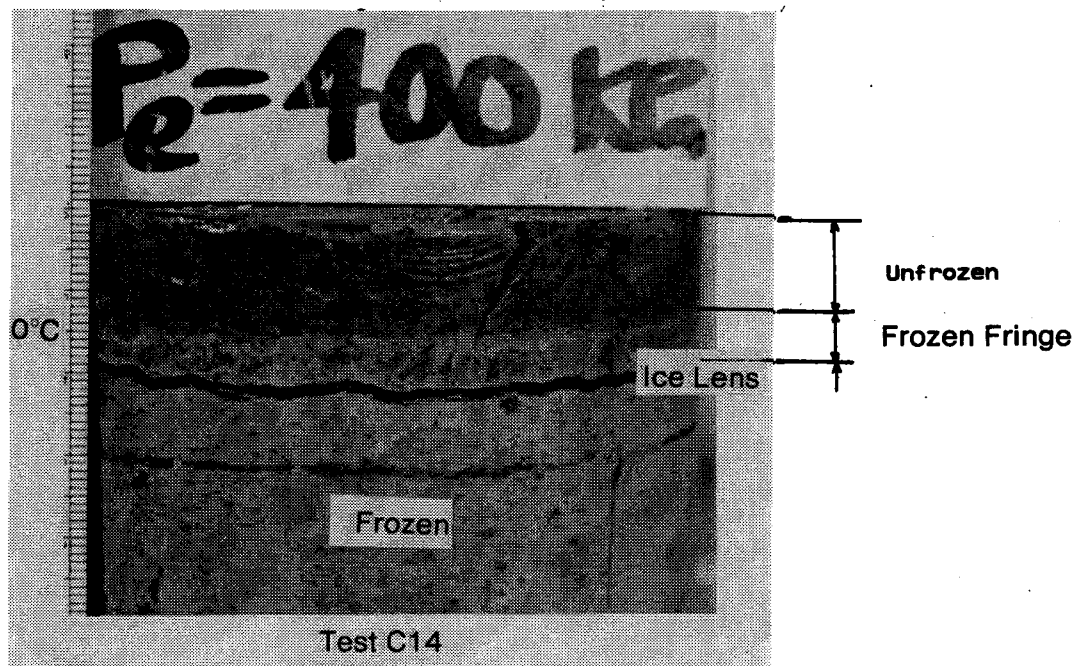
Plate 6.2 Evidence of Frozen Fringe in Devon Silt
