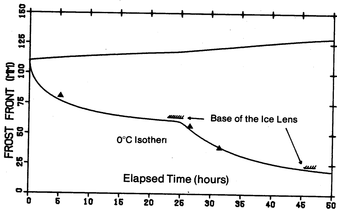
Figure 4.20 Comparison of Prediction with Actual Data for Test E-1
