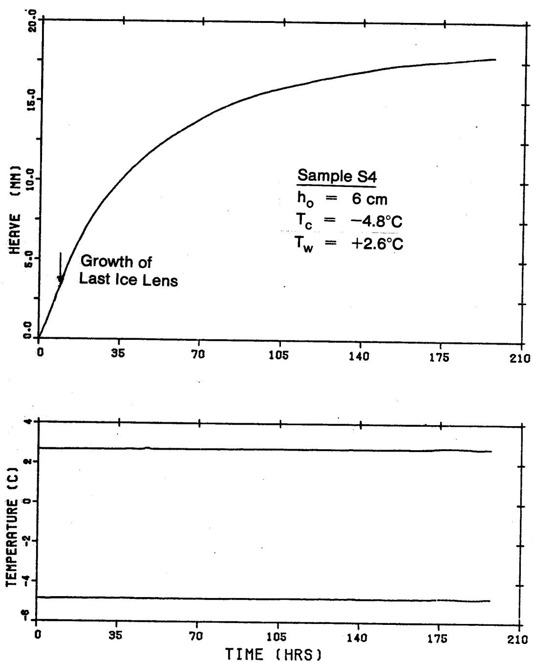
TEST S-4 (P=0.0; LONG TERM TEST)
