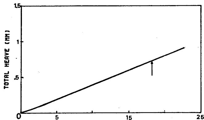
Figure E.3 Experimental Results From Test C-4. P_e=170 kPa
