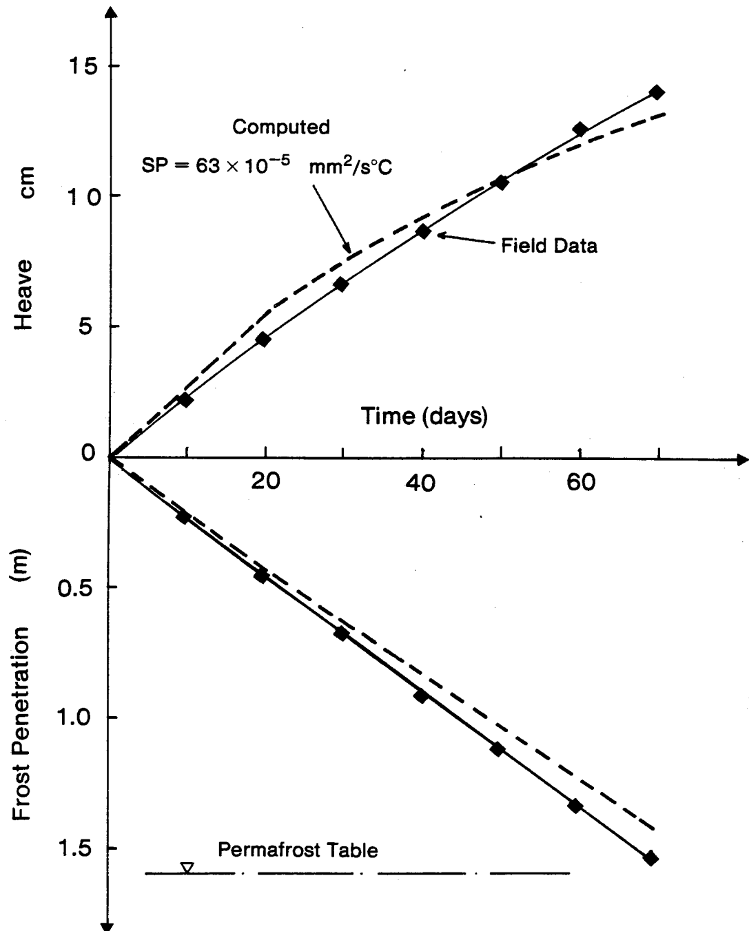
Figure 9.18 Comparison of Prediction with Actual Field Data with Zero Surcharge (Aitken, 1974) Freezing season 1960-61
