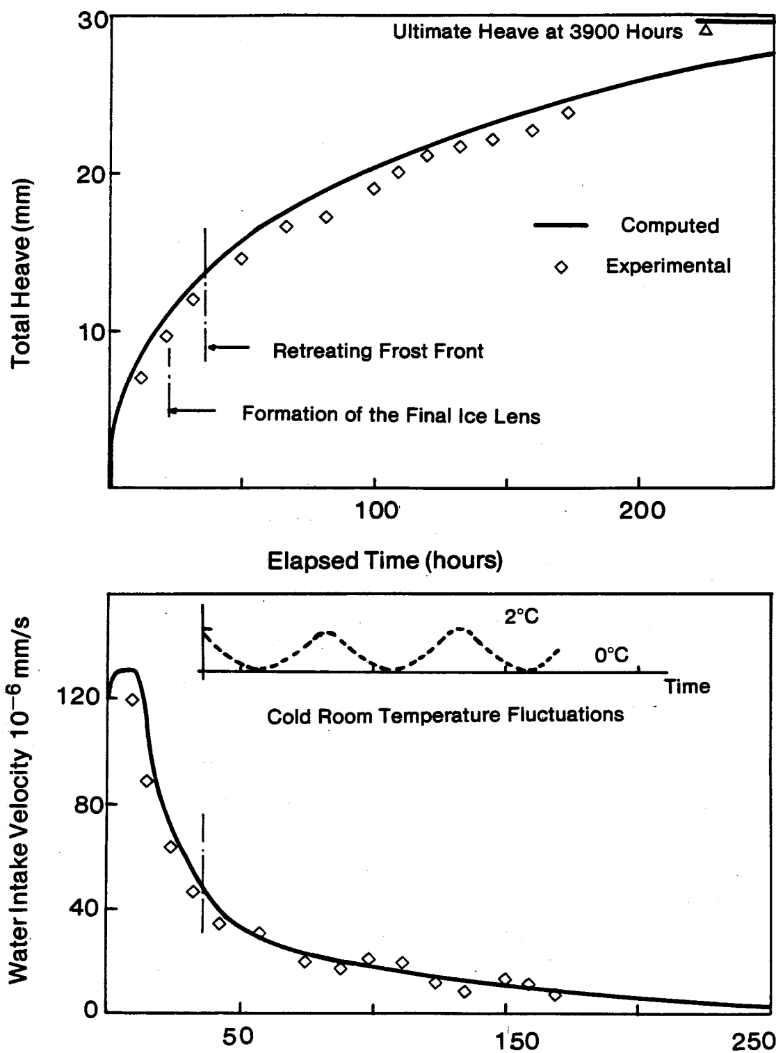
Figure 5.6 Comparison Between Predicted and Observed Data for Test NS-12
