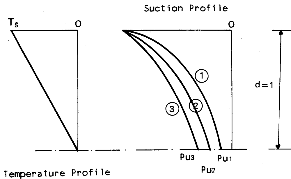
Simplified Conditions at the Initiation of the Final Ice Lens with Different Thermal Boundary Conditions
