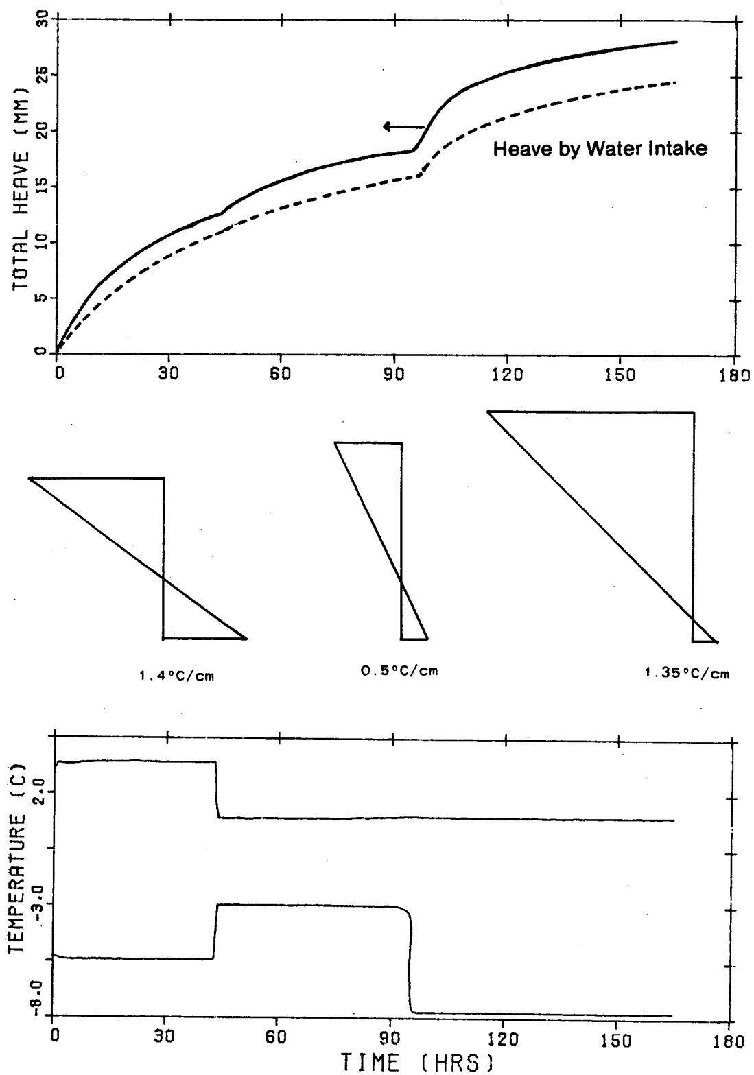
Figure 2.9 Influence of Temperature Gradient. Test S-5
