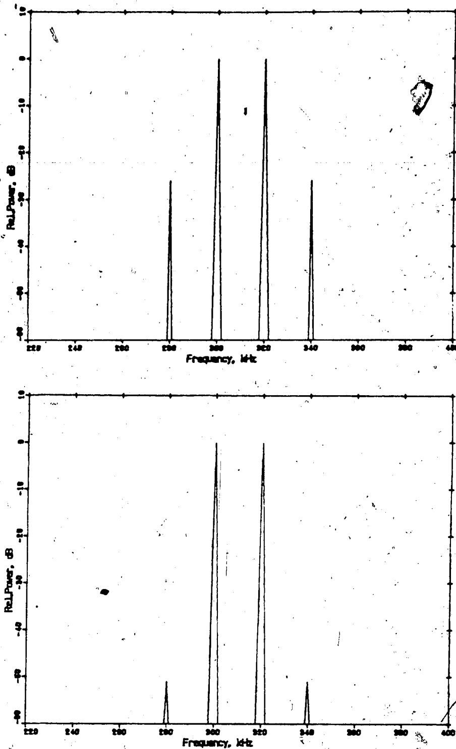
Figure 9.7 Third order IM distortion (for a LD output of 3.0 mW p-p): (a) with no linearisation, and (b) with opto-electronic feedback and adaptive predistortion.
