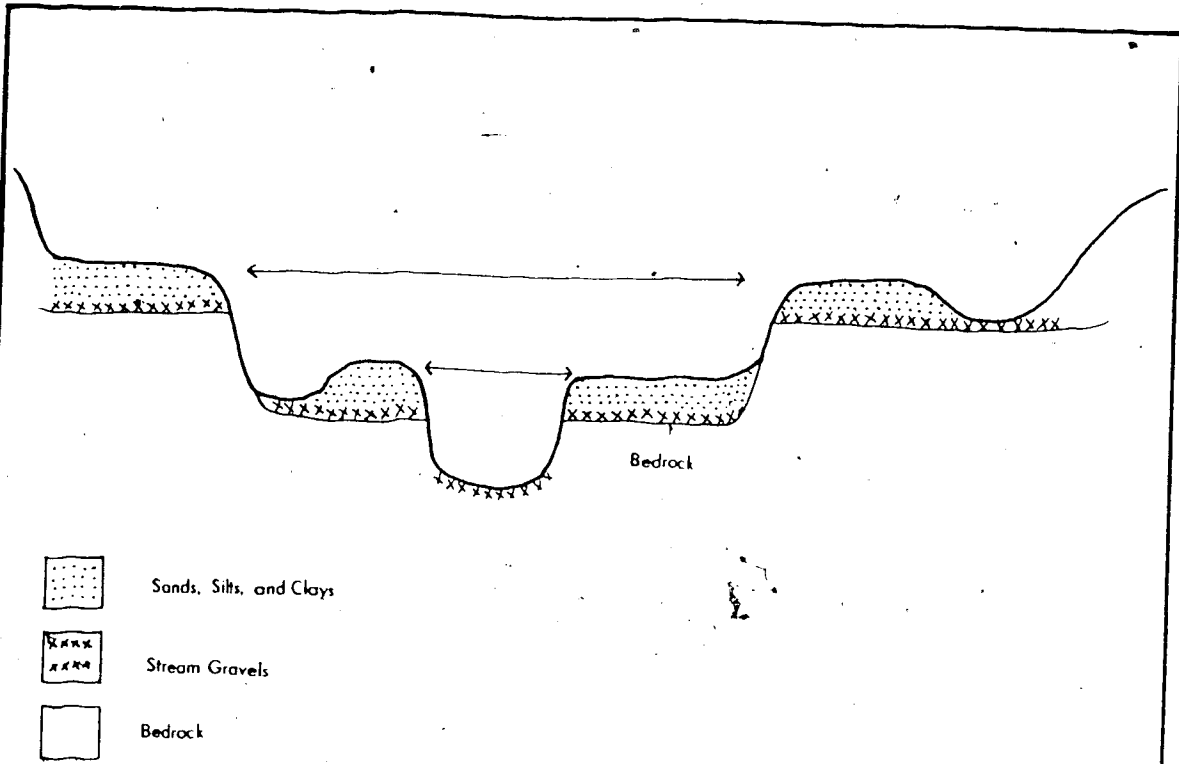
Figure 2:3 Cyclic Terraces (Depositional type)
