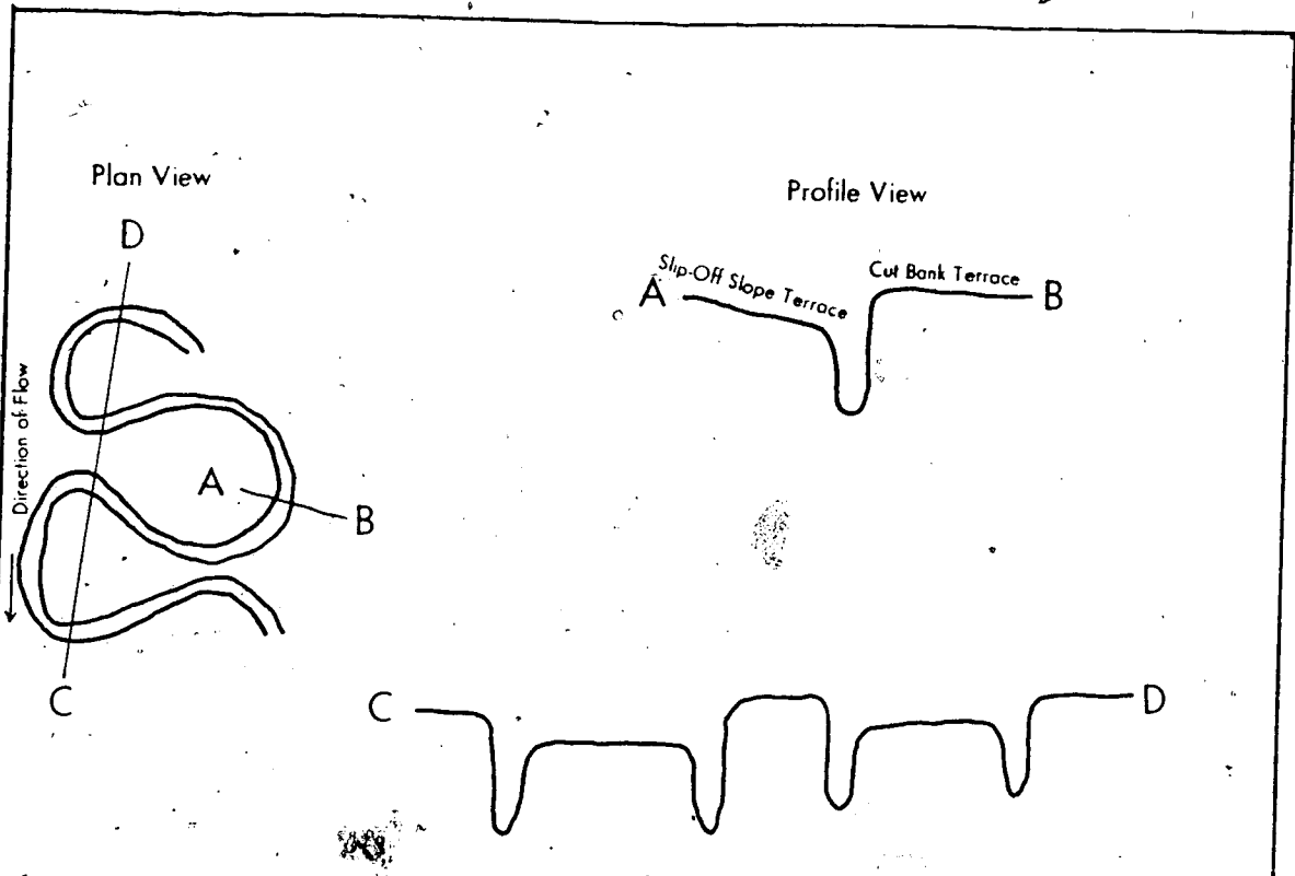
Figure 2:9 Cut Bank Slipoff Slope Terrace
