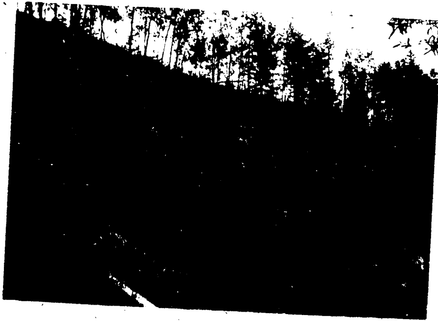
Plate 16 (See P9 on Fig. 3:8 and 3:8.7) A lower terrace just downstream from cross-valley profile number 8.
