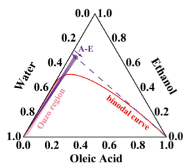
Figure 2. Ternary phase diagram of water, ethanol and oleic acid. The initial component ratio of Sample A-E in Table 1 are also marked here.
