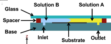
Figure 3. Sketch of the fluid cell set up for the formation of oleic acid nanodroplets on a Si wafer.
