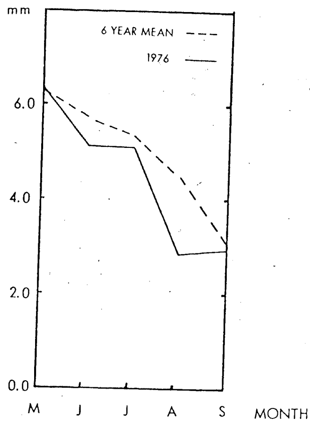
FIG.4.5: EVAPORATION CLASS 'A' PAN
