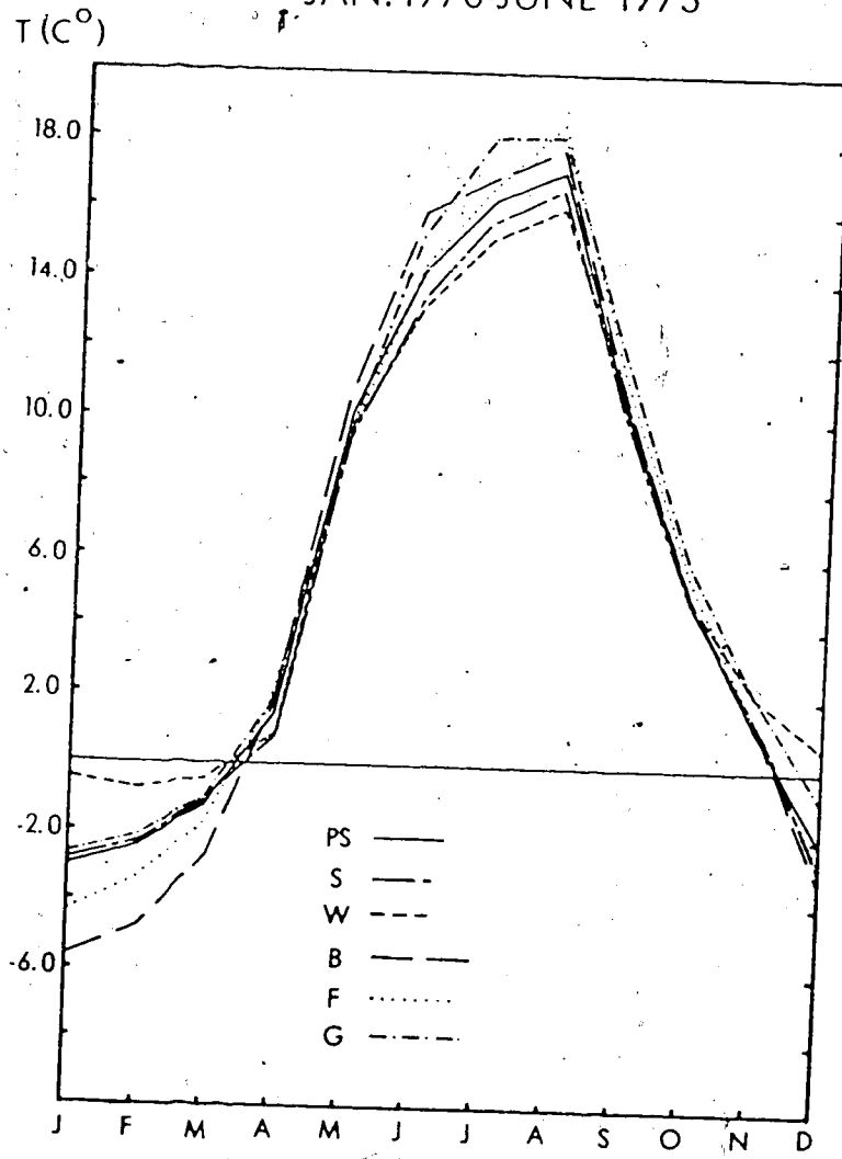
FIG. 4.3: MEAN 20 cm SOIL TEMPERATURES JAN. 1970-JUNE 1973
