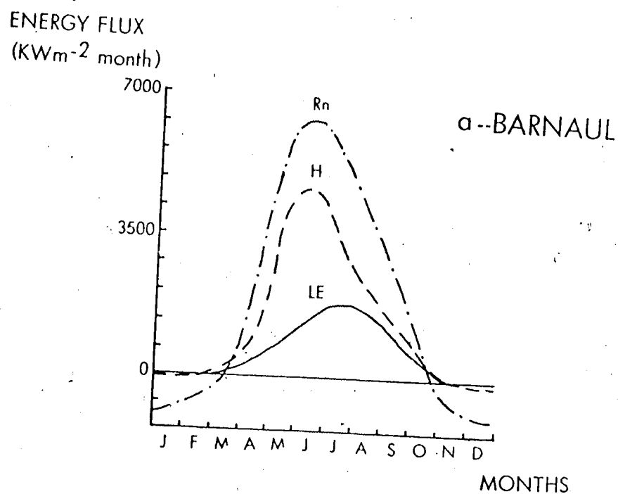
FIG. 3.3: ANNUAL MARCH OF HEAT BALANCE
