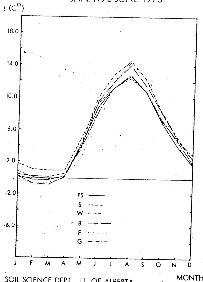
FIG. 4. 4: MEAN 100 cm. SOIL TEMPERATURES JAN. 1970-JUNE 1973
