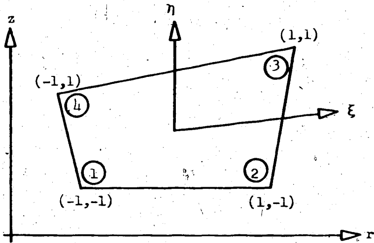
Figure 1.a Eight Degree of Freedom Quadrilateral Element Crosssection.
