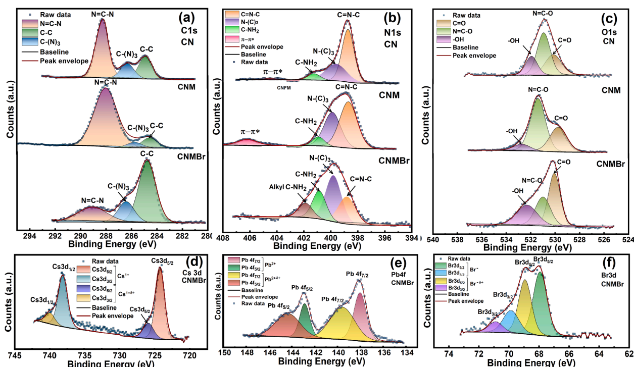
Fig. 3. Core-level HR-XPS spectra of CN, CNM, CNMBr in (a) C1s, (b) N1s, (c) O1s regions and HR-XPS spectra of CsPbBr 3 in (d) Cs3d, (e) Pb4f and (f) Br3d region.
