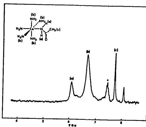
Figure 5. Pmr spectra in d_6 -dimethylsulfoxide of (\text{NH}_3)_5\text{CoNHCHO}^{2+} (at 100 MHz), (\text{NH}_3)_5\text{CoNHC(O)CH}_3^{2+} , and (\text{NH}_3)_5\text{CoNH}_2\text{C(O)CH}_3^{3+} (at 60 MHz).
