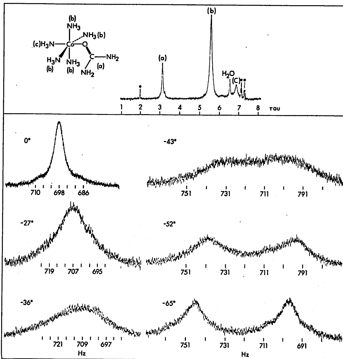
Figure 11. Temperature variation of the \text{C}(\text{NH}_2)_2 pmr, in \text{d}_7 -DMF, of (\text{NH}_3)_5\text{CoOC}(\text{NH}_2)_2^{3+} . Spectra recorded at 100 MHz.
