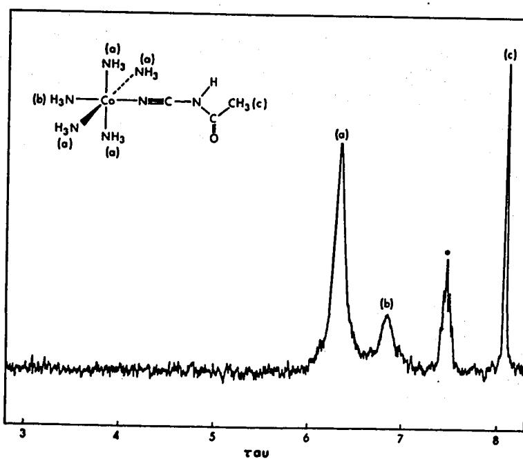
Figure 7. PMR spectra in d_6 -dimethylsulfoxide of (\text{NH}_3)_5\text{CoNCNH}_2^{3+} and (\text{NH}_3)_5\text{CoNCNHC(O)CH}_3^{3+} (both at 60 MHz).
