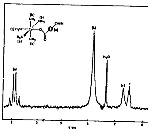
Figure 6. Pmr spectra in d_6 -dimethylsulfoxide of (\text{NH}_3)_5\text{CoNCC}_6\text{H}_4\text{CN}^{3+} (at 100 MHz), (\text{NH}_3)_5\text{NHCOC}_6\text{H}_4\text{CN}^{2+} (at 60 MHz), and (\text{NH}_3)_5\text{CoO}_2\text{CC}_6\text{H}_4\text{CN}^{2+} (at 60 MHz).
