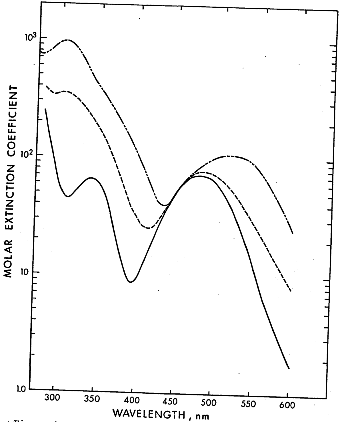
Figure 2. Visible spectra of ((\text{NH}_3)_5\text{CoNCNH}_2)(\text{ClO}_4)_3 in 1.0 M \text{HClO}_4 (—), \text{H}_2\text{O} (pH ~3.7) (----), and 1.0 M sodium acetate (pH ~8.2) (-·-·-).
