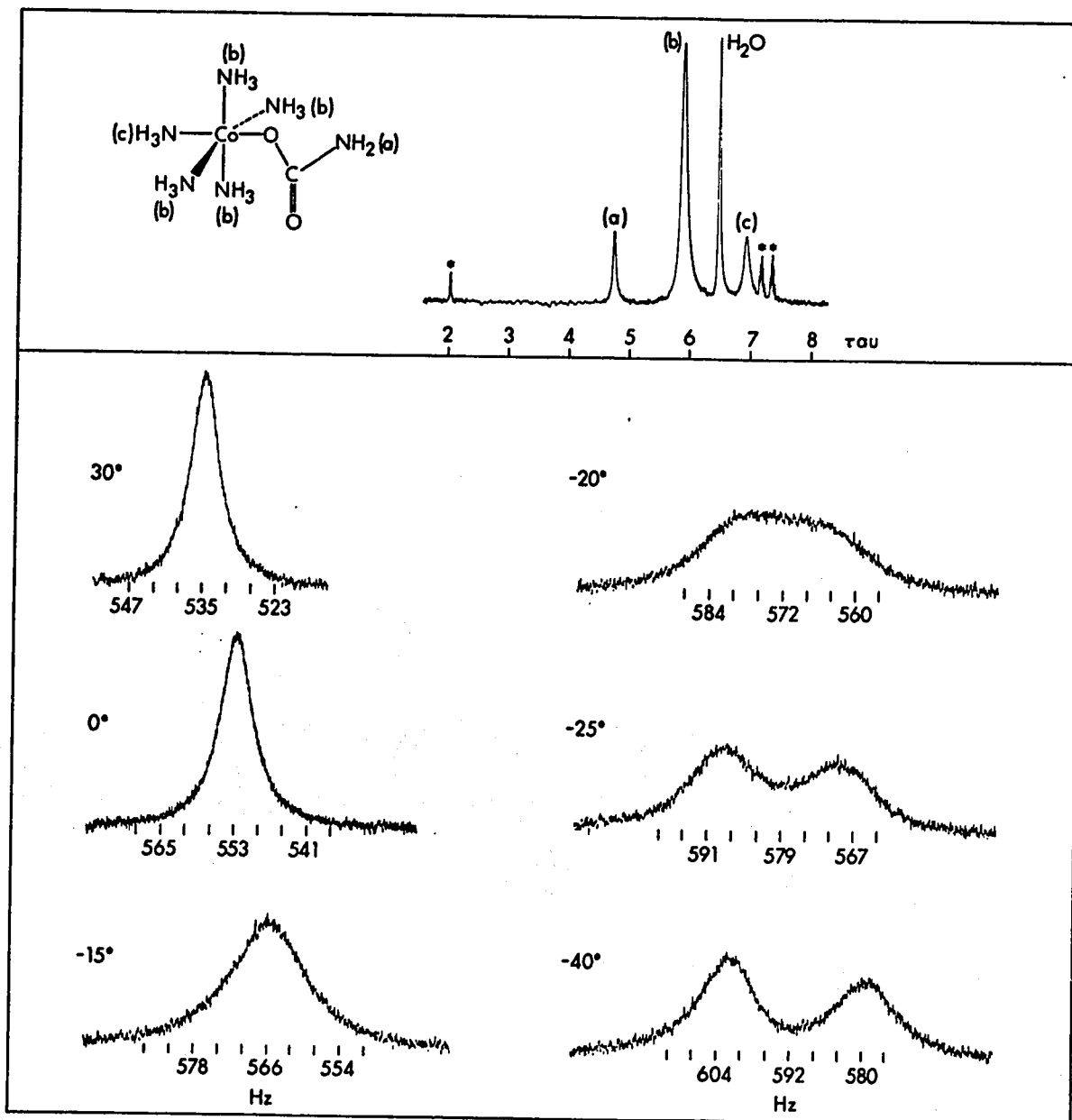
Figure 10. Temperature variation of the C-NH 2 pmr, in d 7 -DMF, of (\text{NH}_3)_5\text{CoO}_2\text{CNH}_2^{2+} . Spectra recorded at 100 MHz.
