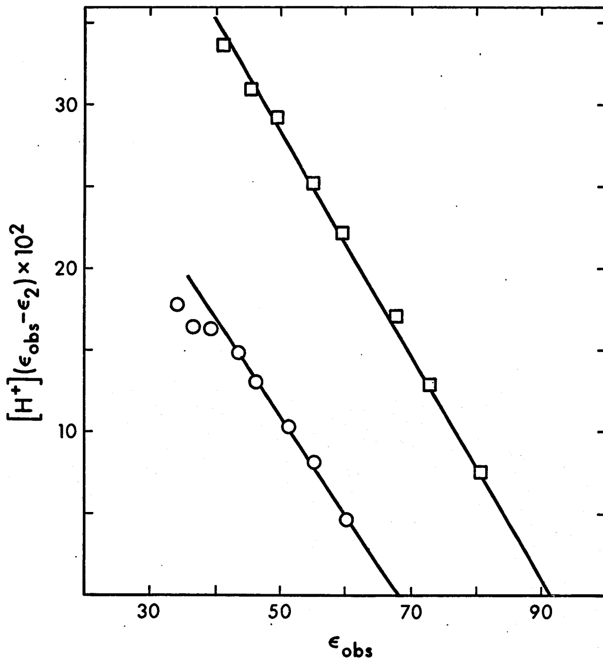
Figure 14. Determination of the acid dissociation constant ( K_a ) for (\text{NH}_3)_5\text{CoNH}_2\text{CHO}^{3+} from the change in absorbance at 318.4 nm ( \square ) and 366.4 nm ( \circ ) at 25.5°; ionic strength, 0.92 M ( \text{LiClO}_4 ). \epsilon_2 is the molar extinction coefficient of (\text{NH}_3)_5\text{CoNH}_2\text{CHO}^{3+} and \epsilon_{\text{obsd}} is the observed molar extinction coefficient.
