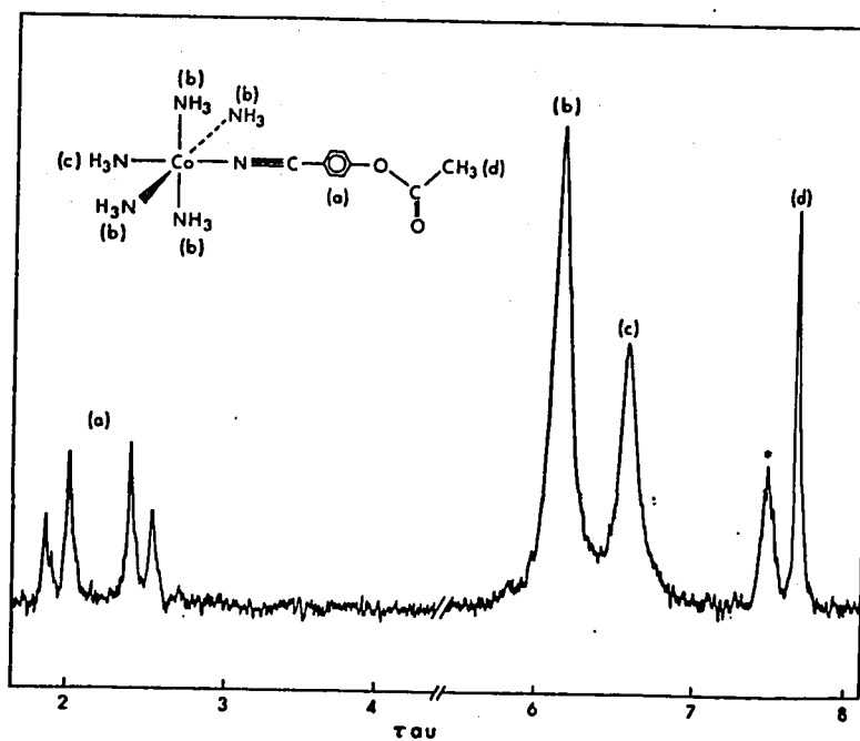
Figure 8. Pmr spectra in d_6 -dimethylsulfoxide of (\text{NH}_3)_5\text{CoNCC}_6\text{H}_4\text{OH}^{3+} and (\text{NH}_3)_5\text{CoNCC}_6\text{H}_4\text{O}_2\text{CCH}_3^{3+} (both at 60 MHz).
