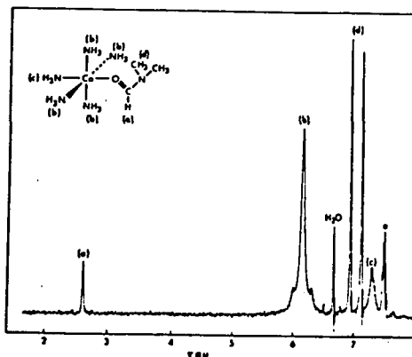
Figure 4. Pmr spectra in d_6 -dimethylsulfoxide of the oxygen bonded pentaamminecobalt(III) complexes of formamide, N-methylformamide, and dimethylformamide (all at 100 MHz.).
