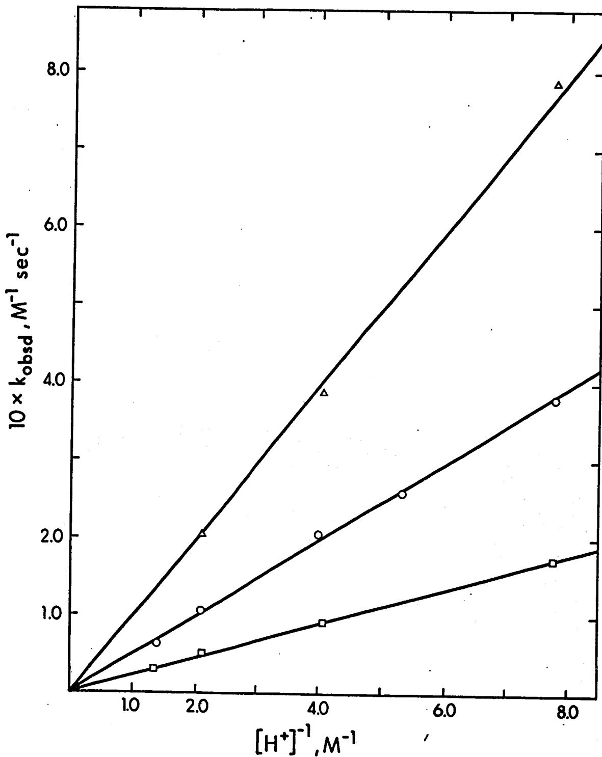
Figure 18. Dependence of the reduction rate of (\text{NH}_3)_5\text{CoNCNH}_2^{3+} by \text{Cr}^{2+} on [\text{H}^+] , ionic strength 1.0 M ( \text{LiClO}_4 ): \Delta , 43.8°; O, 34.8°; \square 24.6°.
