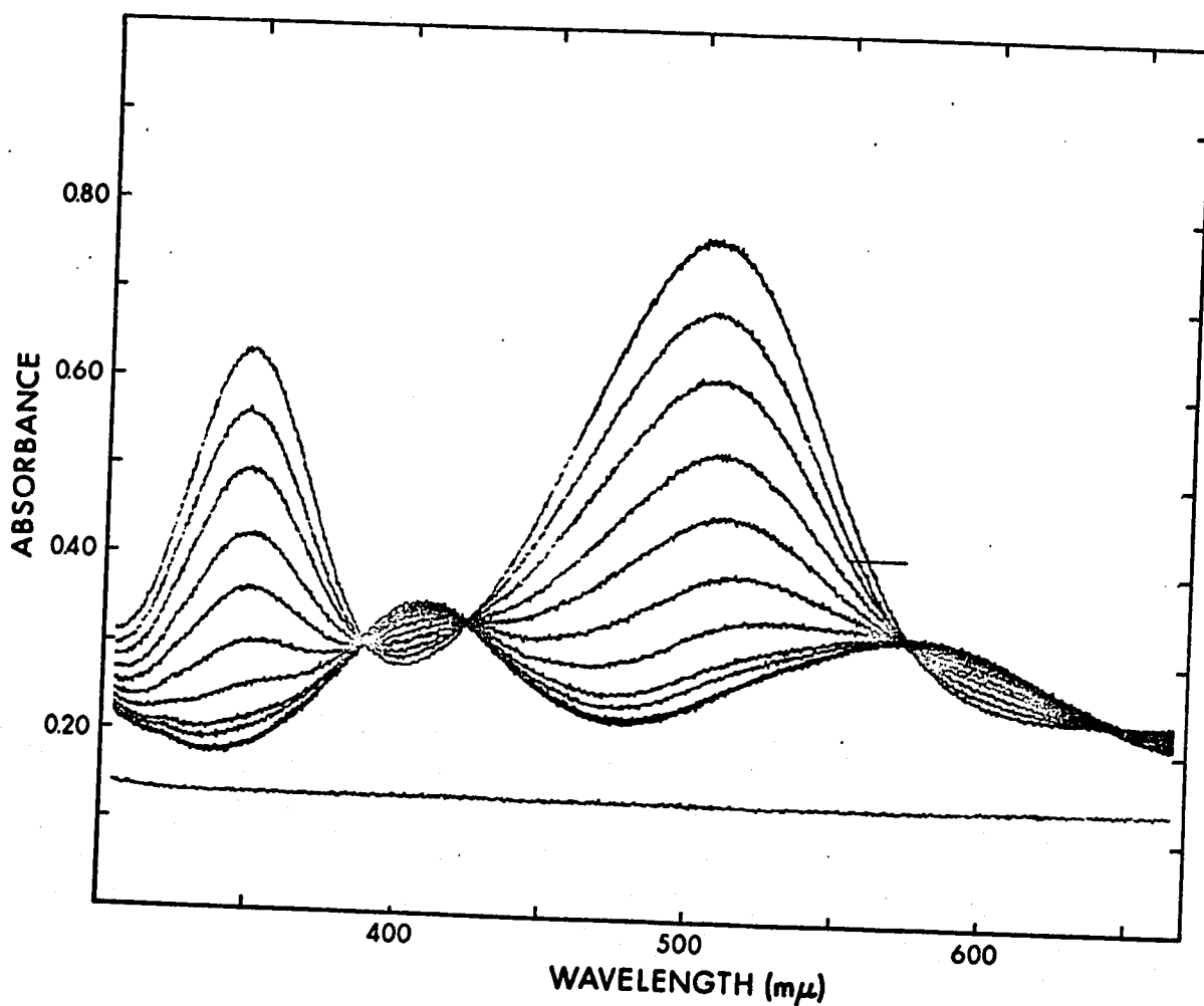
Figure 16. Change in visible spectrum during reduction of (\text{NH}_3)_5\text{CoOCHNH}_2^{3+} (0.011 M) by chromium(II) (0.019 M); [\text{H}^+] = 0.505 \text{ M} ; 28.5^\circ ; ionic strength 0.99 M ( \text{LiClO}_4 ). The absorbance is decreasing at \sim 500 \text{ nm} and \sim 350 \text{ nm} due to consumption of \text{Co}^{3+} complex, and increasing at \sim 575 \text{ nm} and \sim 410 \text{ nm} due to production of \text{Cr}(\text{OH}_2)_6^{3+} . Isosbestic points occur at 388, 432, 573, and 642 nm. The spectral scans were started at 4, 22, 45, 80, 121, 180, 262, 460, 645, 763, and 1436 min after mixing. The last three show no change.
