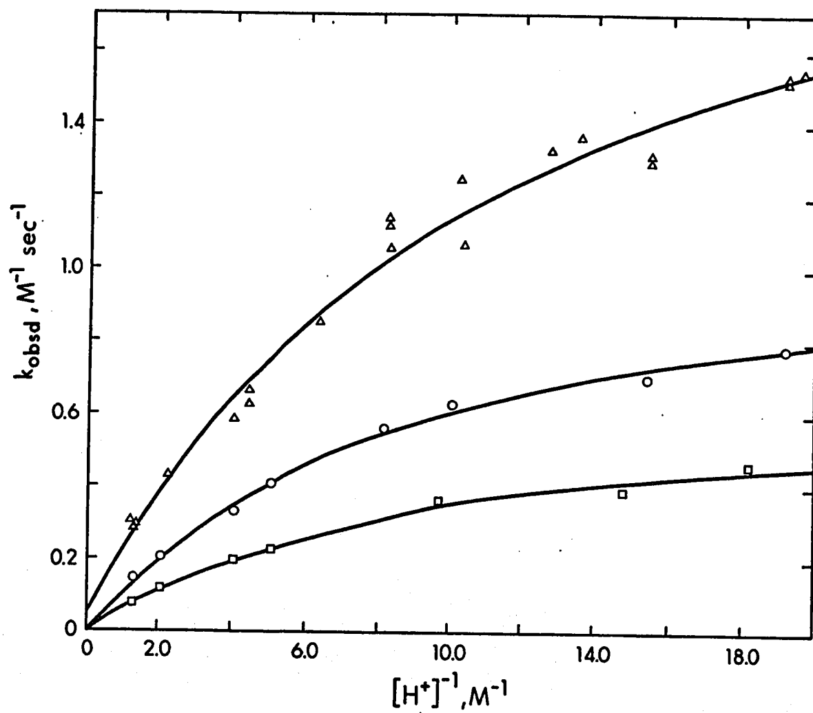
Figure 19. Dependence of the reduction rate of (\text{NH}_3)_5\text{CoO}_2\text{CNH}_2^{2+} by \text{Cr}^{2+} on [\text{H}^+] , ionic strength 1.0 M ( \text{LiClO}_4 ): \Delta , 25.8°; \circ , 15.0°; \square , 8.0°.
