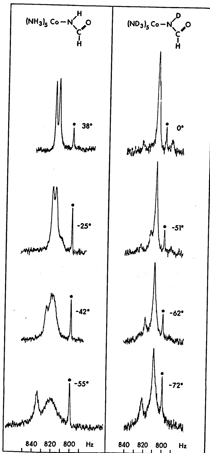
Figure 9. Temperature variation of the C-H pmr, in d_7 -DMF, of (\text{NH}_3)_5\text{CoNHCHO}^{2+} and (\text{ND}_3)_5\text{CoNDCHO}^{2+} . An asterisk denotes solvent peak due to formyl C-H in DMF. Spectra recorded at 100 MHz.
