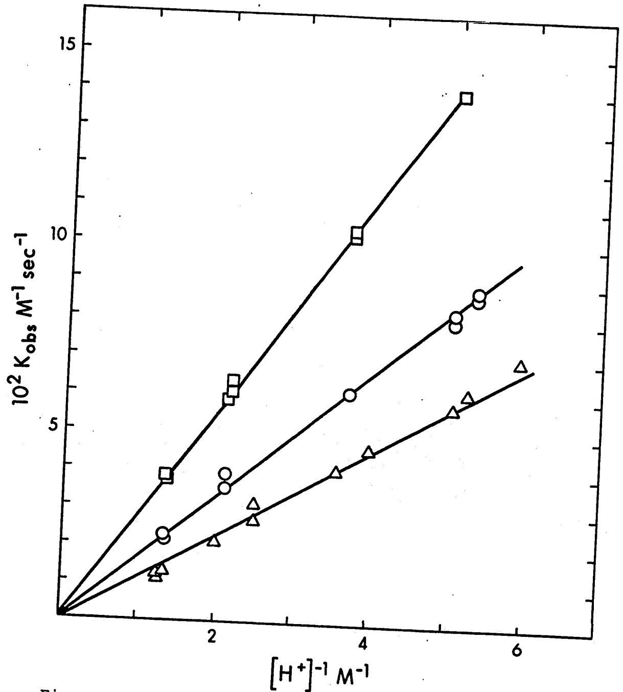
Figure 17. Dependence of reduction rate of (\text{NH}_3)_5\text{CoNH}_2\text{CHO}^{3+} by \text{Cr}^{2+} on [\text{H}^+] , ionic strength 0.92 M ( \text{LiClO}_4 ): \Delta 25.5°; \circ , 34.6°; \square 44.4°.
