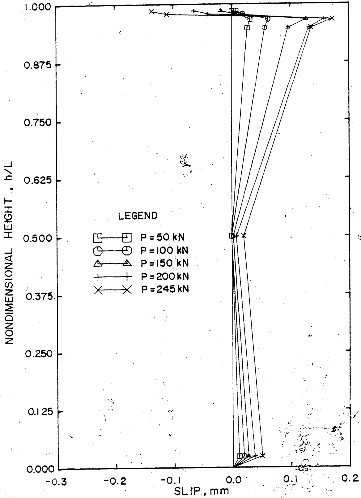
Figure 5.34 Slip on South Fac of Beam Column C1206, Method B
