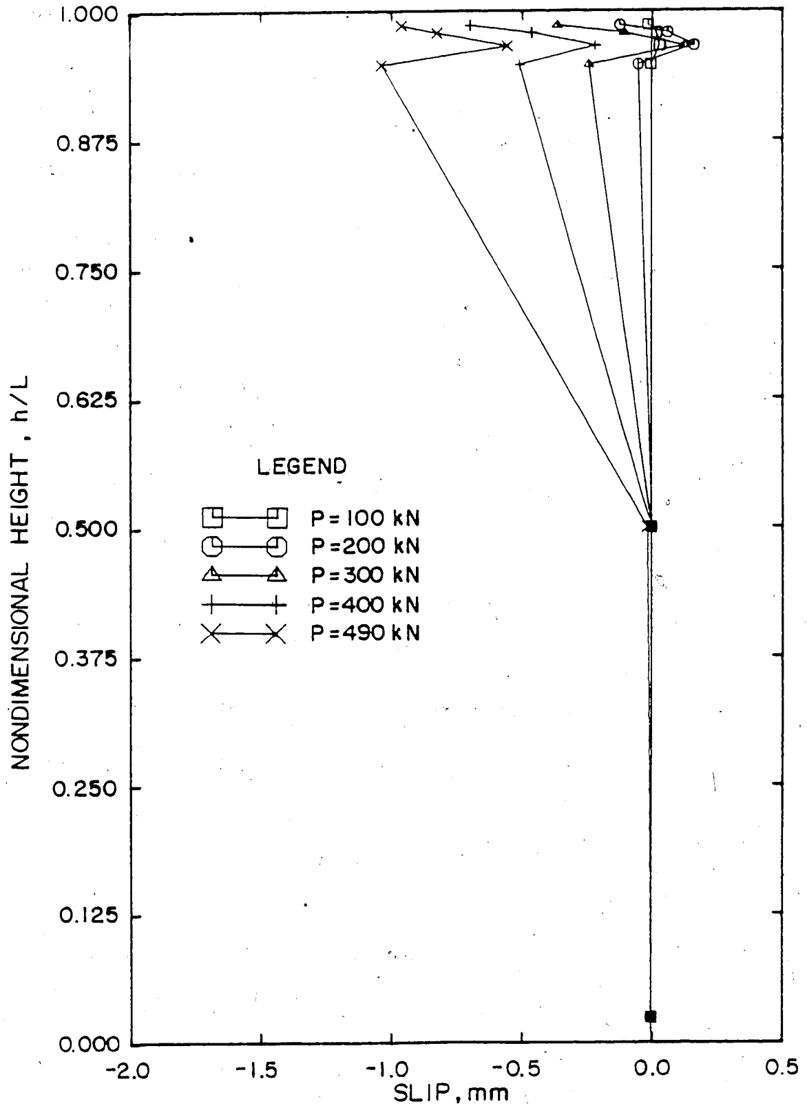
Figure 5.28 Slip on South Face of Column C1205, Method B
