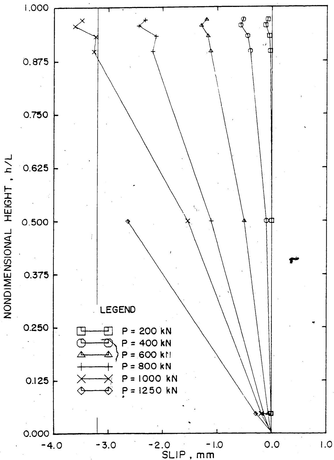
Figure 5.27 Slip on South Face of Column C605, Method B
