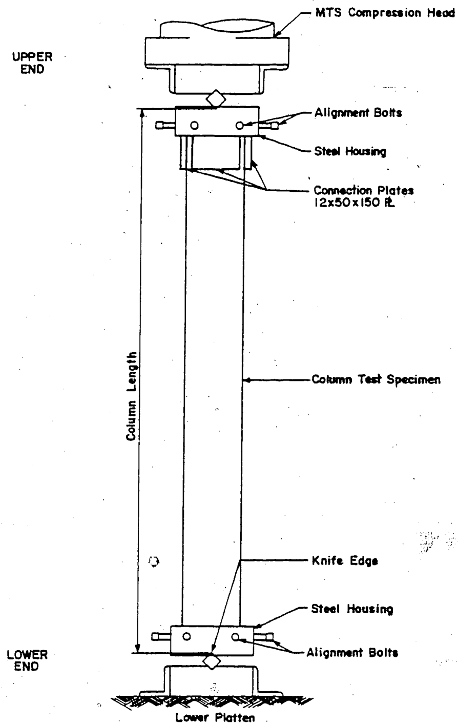
Figure 3.2 Schematic Diagram of a Column Specimen
