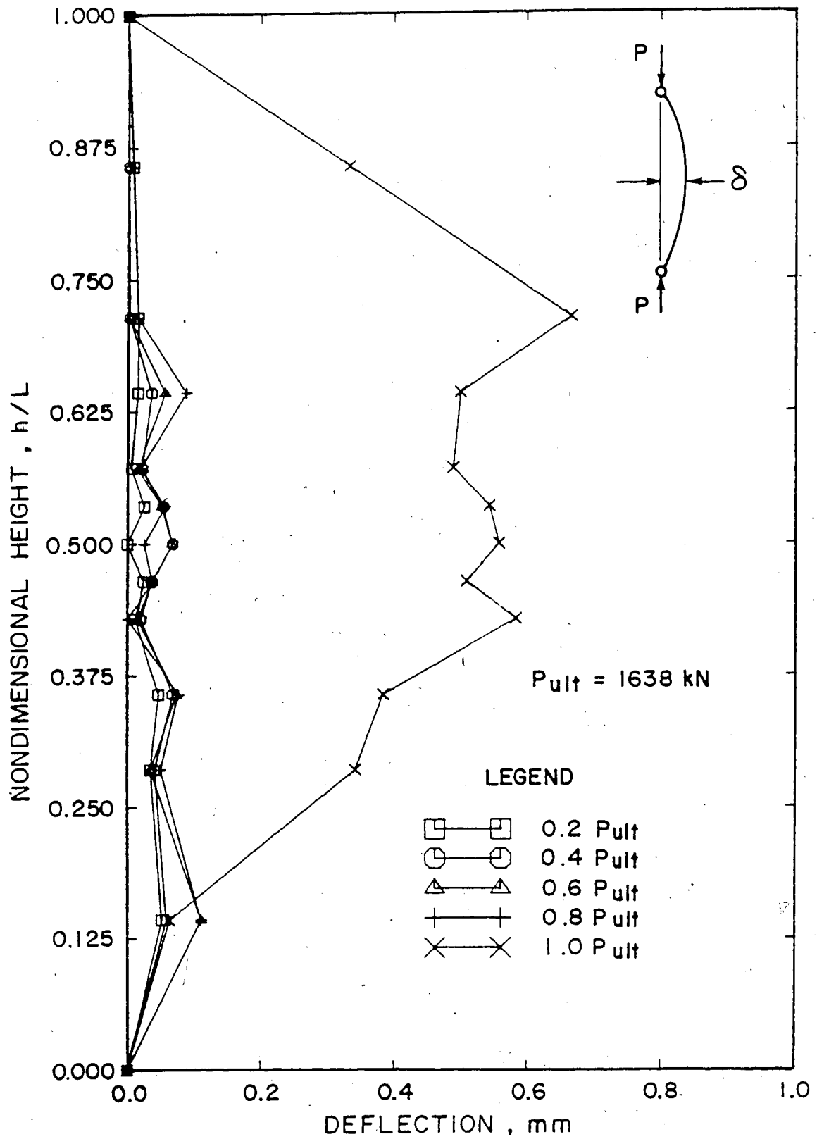
Figure 5.11 Load Deflection for Concentrically Loaded Column C203
