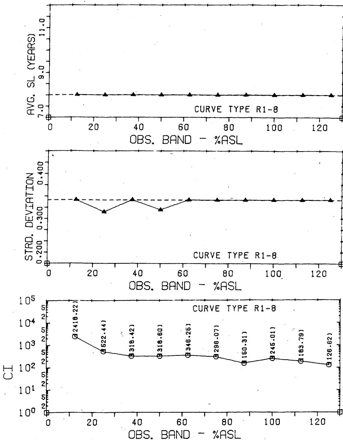
Figure 6.14 Results of the Investigation of the Observation Band Length for a R1-8 Curve With an Exponential Growth Rate of 1.03
