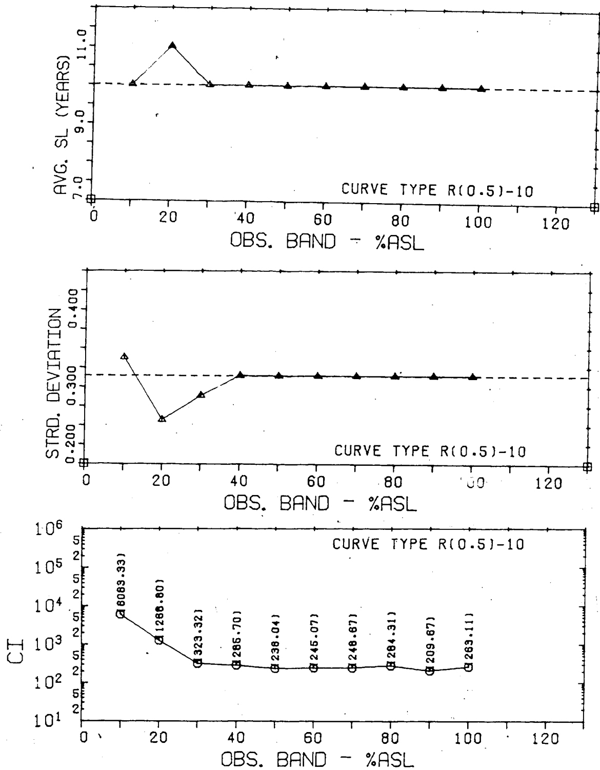
Figure 6.13 Results of the Investigation of the Observation Band Length for a R(0.5)-10 Curve With a Linear Growth Rate of 3700 Units/Yr.
