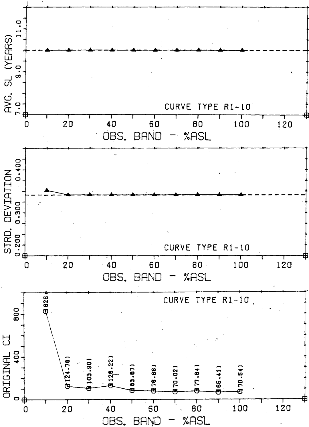
Figure 6.15 Results of the Investigation of the Observation Band Length for a R1-10 Curve With a Stationary Plant Balance
