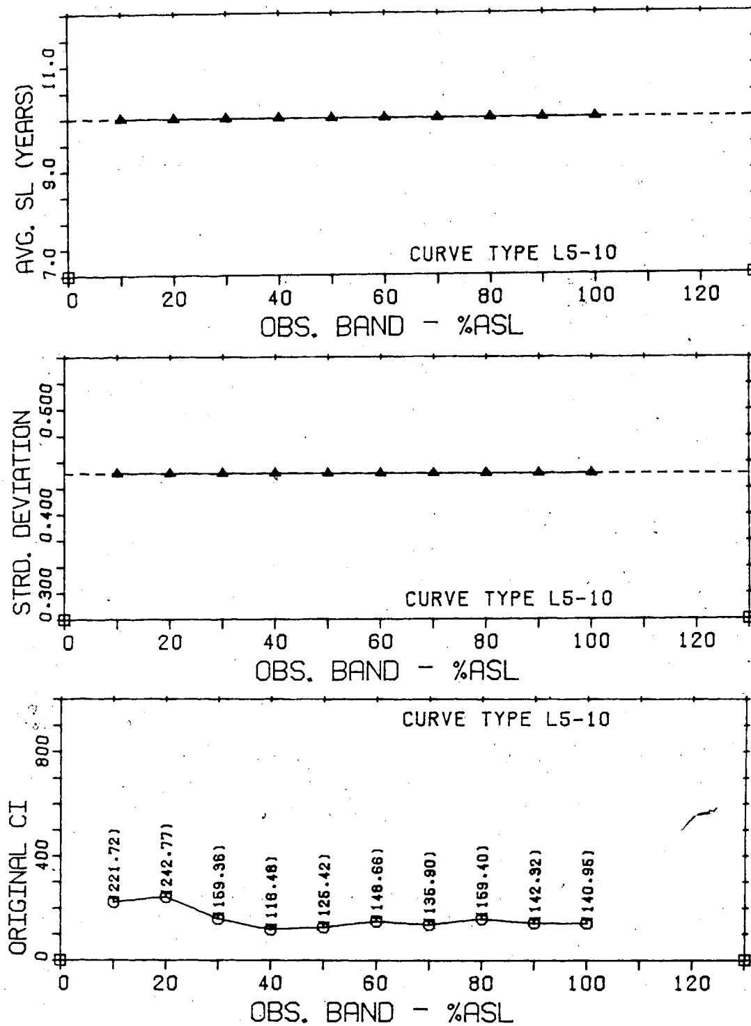
Figure 6.4 Results of the Investigation of the Observation Band Length for a L5-10 Curve With a Linear Growth Rate of 2500 Units/Yr.
