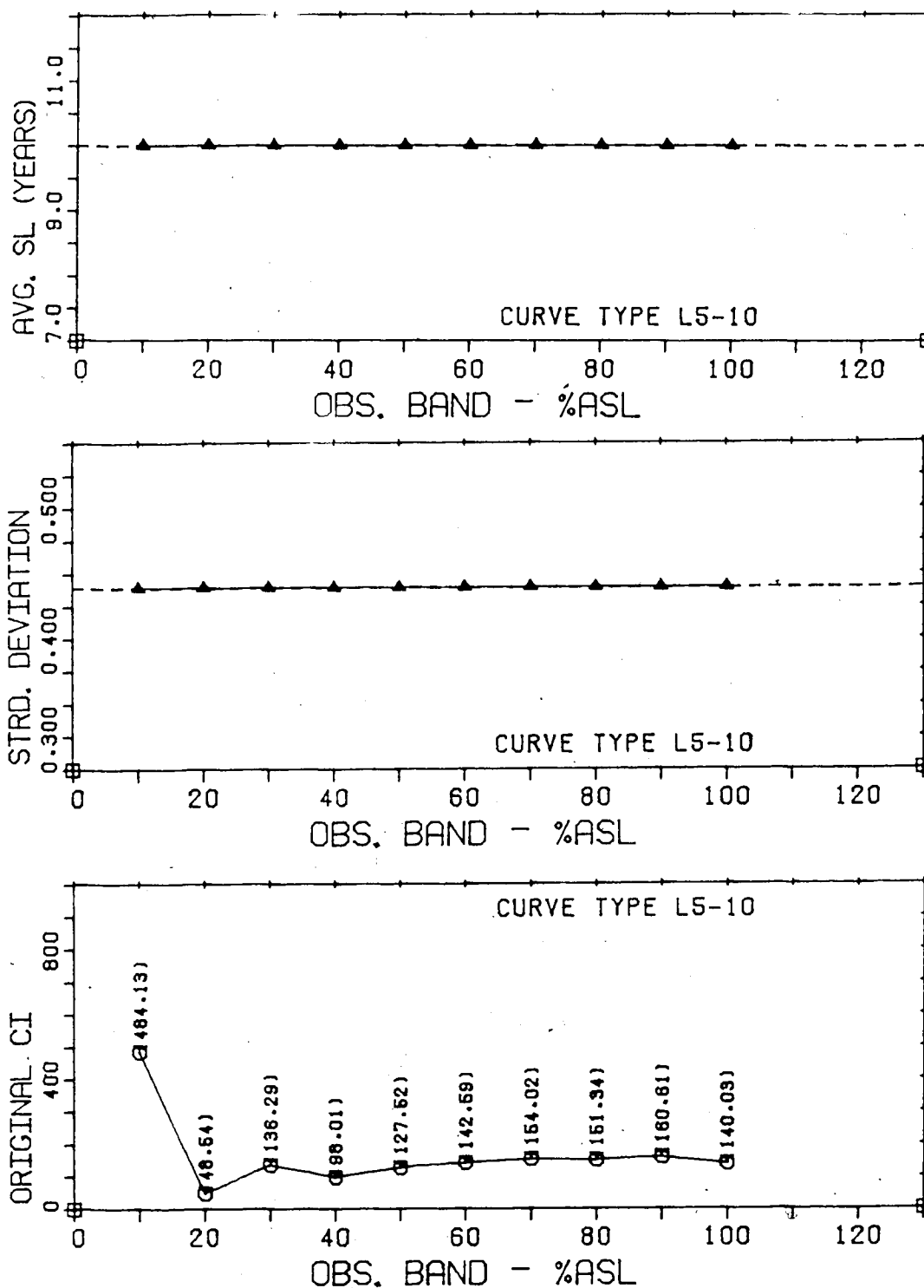
Figure 6.6 Results of the Investigation of the Observation Band Length for a L5-10 Curve With a Stationary Plant Balance
