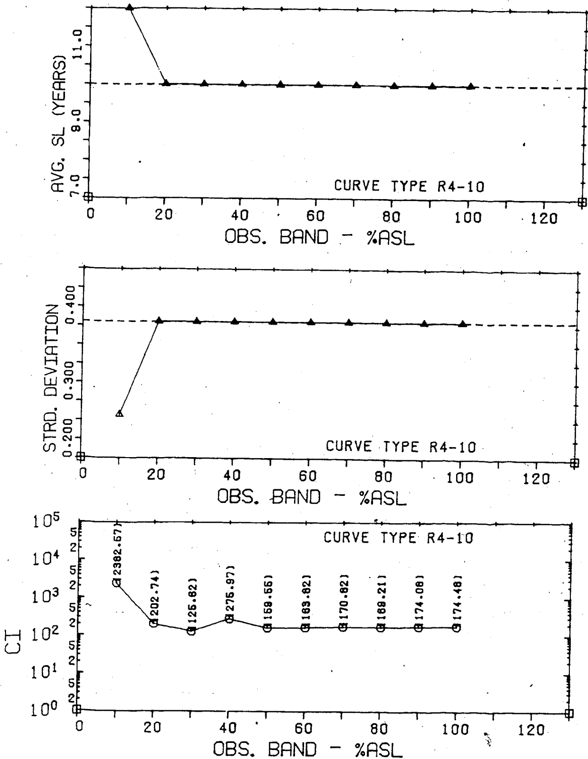
Figure 6.17 Results of the Investigation of the Observation Band Length for a R4-10 Curve With an Exponential Growth Rate of 1.03
