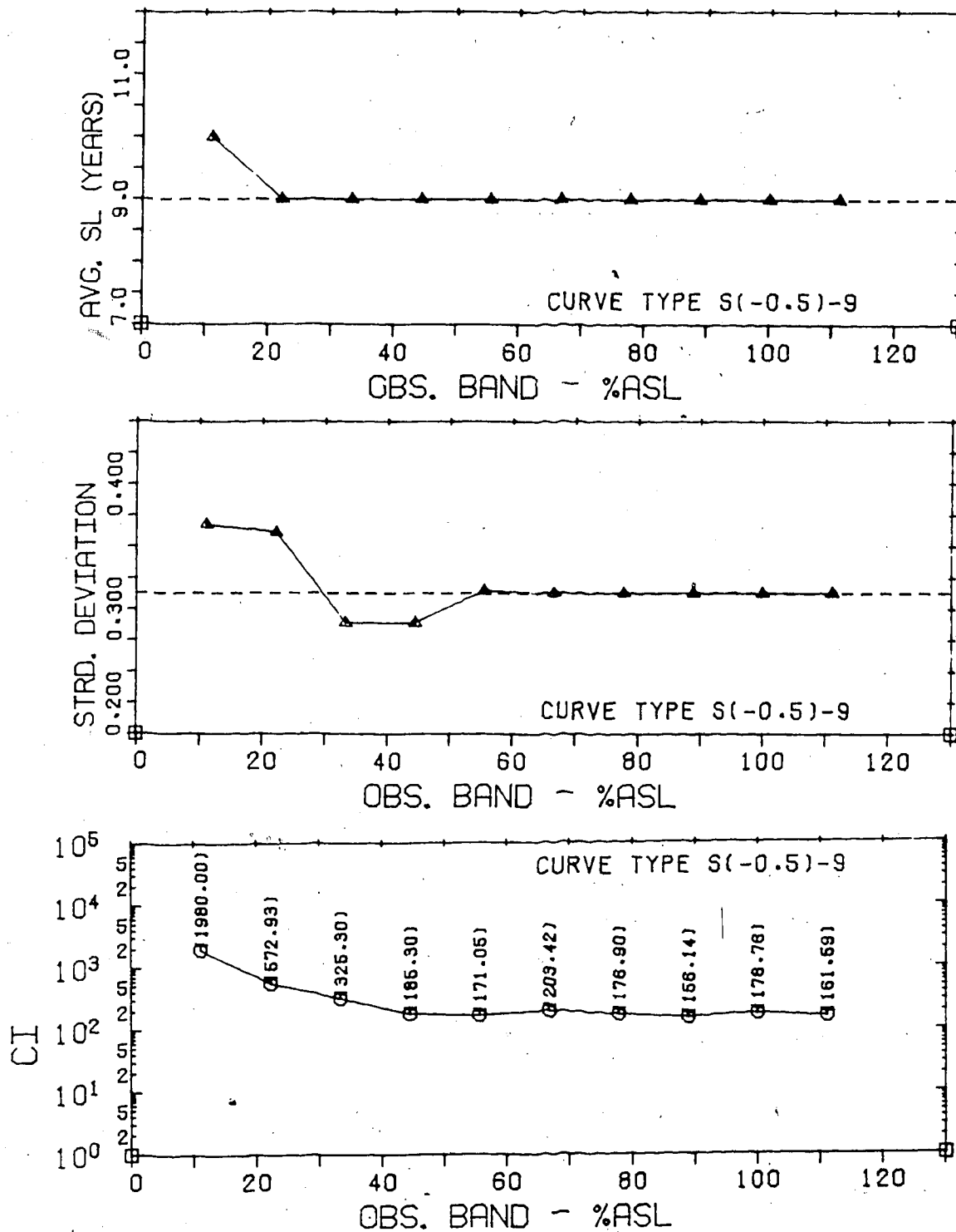
Figure 6.8 Results of the Investigation of the Observation Band Length for a S(-0.5)-9 Curve With an Exponential Growth Rate of 1.04
