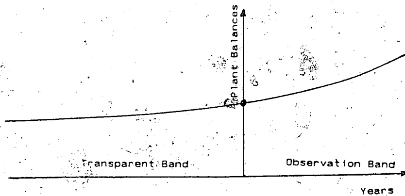
Figure 4.4 Exponential Growth Profile of the MTPBM
