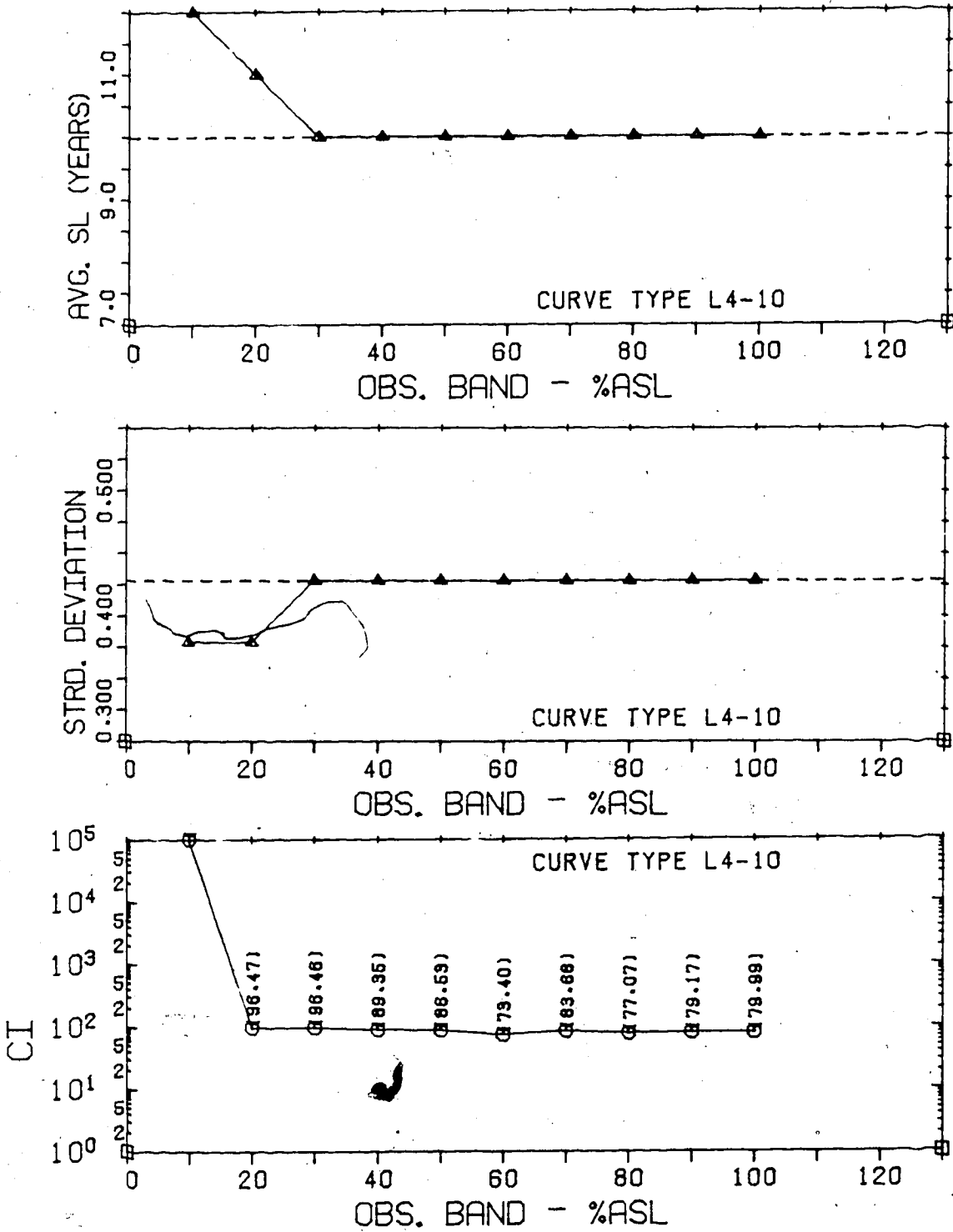
Figure 6.5 Results of the Investigation of the Observation Band Length for a L4-10 Curve With an Exponential Growth Rate of 1.02
