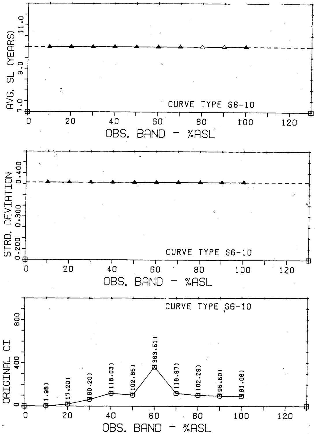
Figure 6.12 Results of the Investigation of the Observation Band Length for a S6-10 Curve With a Stationary Plant Balance
