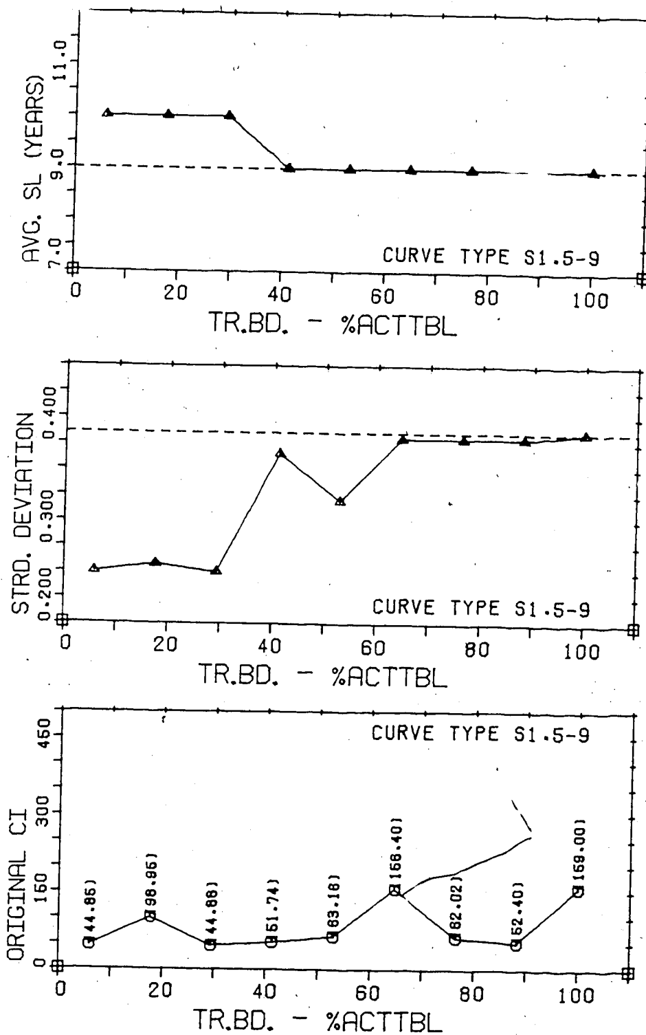
Figure 6.22 Results of the Investigation of the Transparent Band Length for a S(1.5)-9 Curve With a Linear Growth Rate of 3000 Units/Yr
