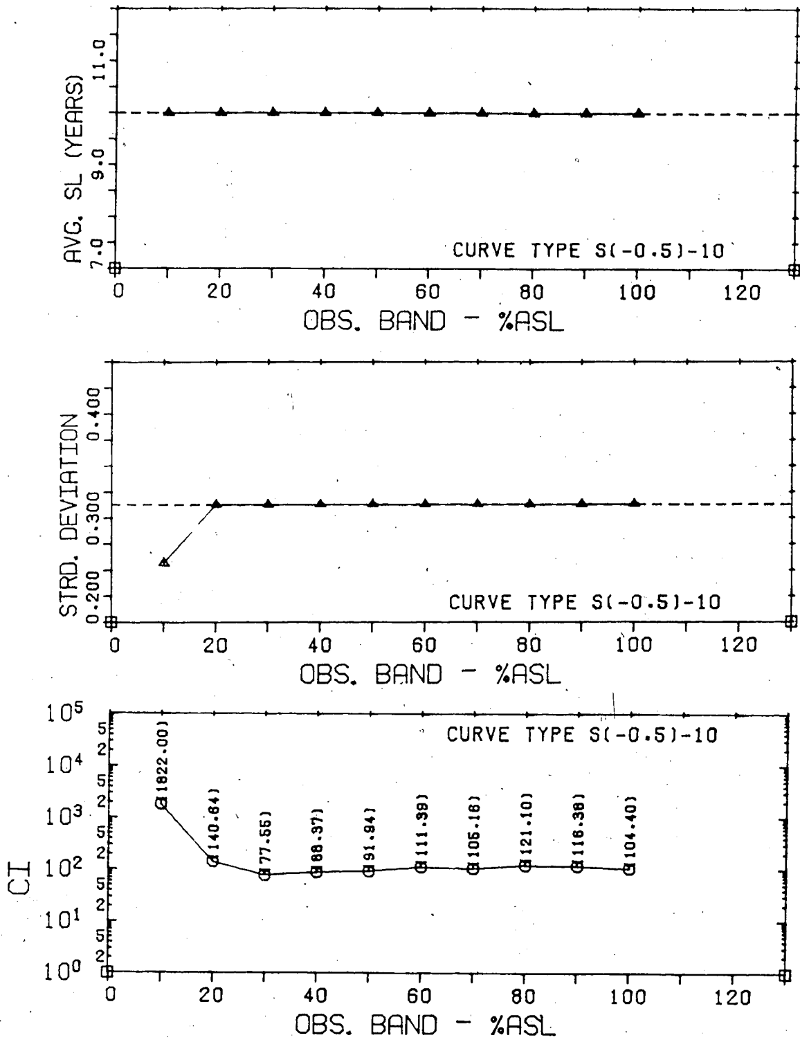
Figure 6.9 Results of the Investigation of the Observation Band Length for a S(-0.5)-10 Curve With a Stationary Plant Balance
