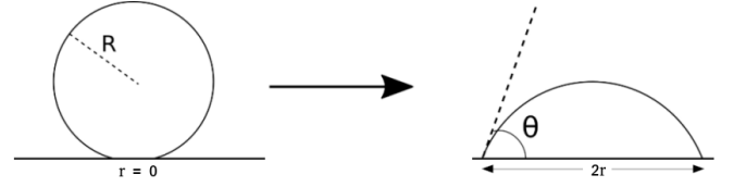
FIG. 9. Initial and steady-state configuration for the sessile droplet starting with an initial contact angle \approx 180^\circ , and evolving with a spreading displacement of r .
