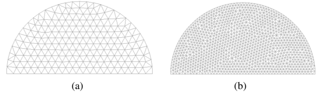
FIG. 5. Initial configuration of a sessile droplet with a starting contact angle of 90^\circ : a) coarse mesh of 1.25 \times 10^{-5} \text{ m} and b) fine mesh of 5 \times 10^{-6} \text{ m} .
