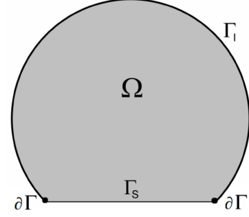
FIG. 1. Schematic representation of the considered Lagrangian domain at the continuum level.
