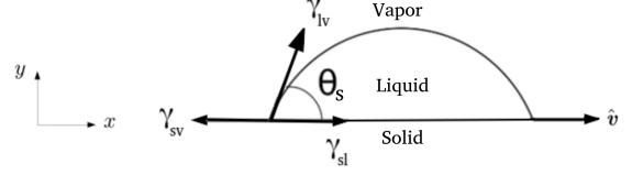
FIG. 2. Schematic representation of the forces acting on a contact line of a sessile droplet.
