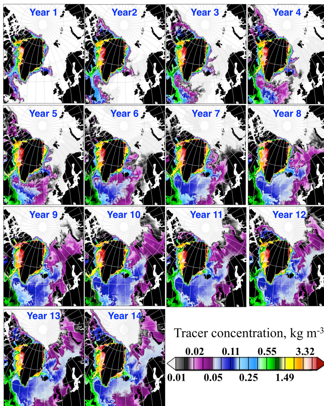
Figure 6. Five-day mean tracer concentration in the surface model layer ( \sim 1 m) for output including 17 December for every model year from NEMO-LIM2. The concentration is on the natural-log scale ( \text{kg m}^{-3} ).
