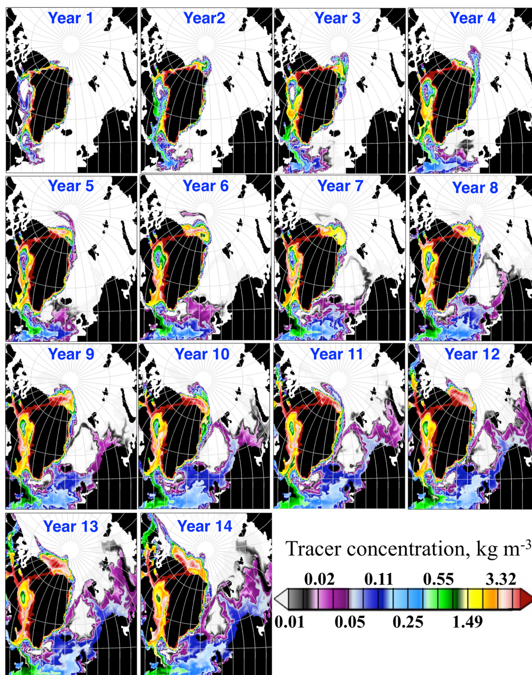
Figure 7. Daily mean tracer concentration in the surface model layer ( \sim 2 m) on 17 December for every model year from ICMMG. The concentration is on the natural-log scale ( \text{kg m}^{-3} ).
