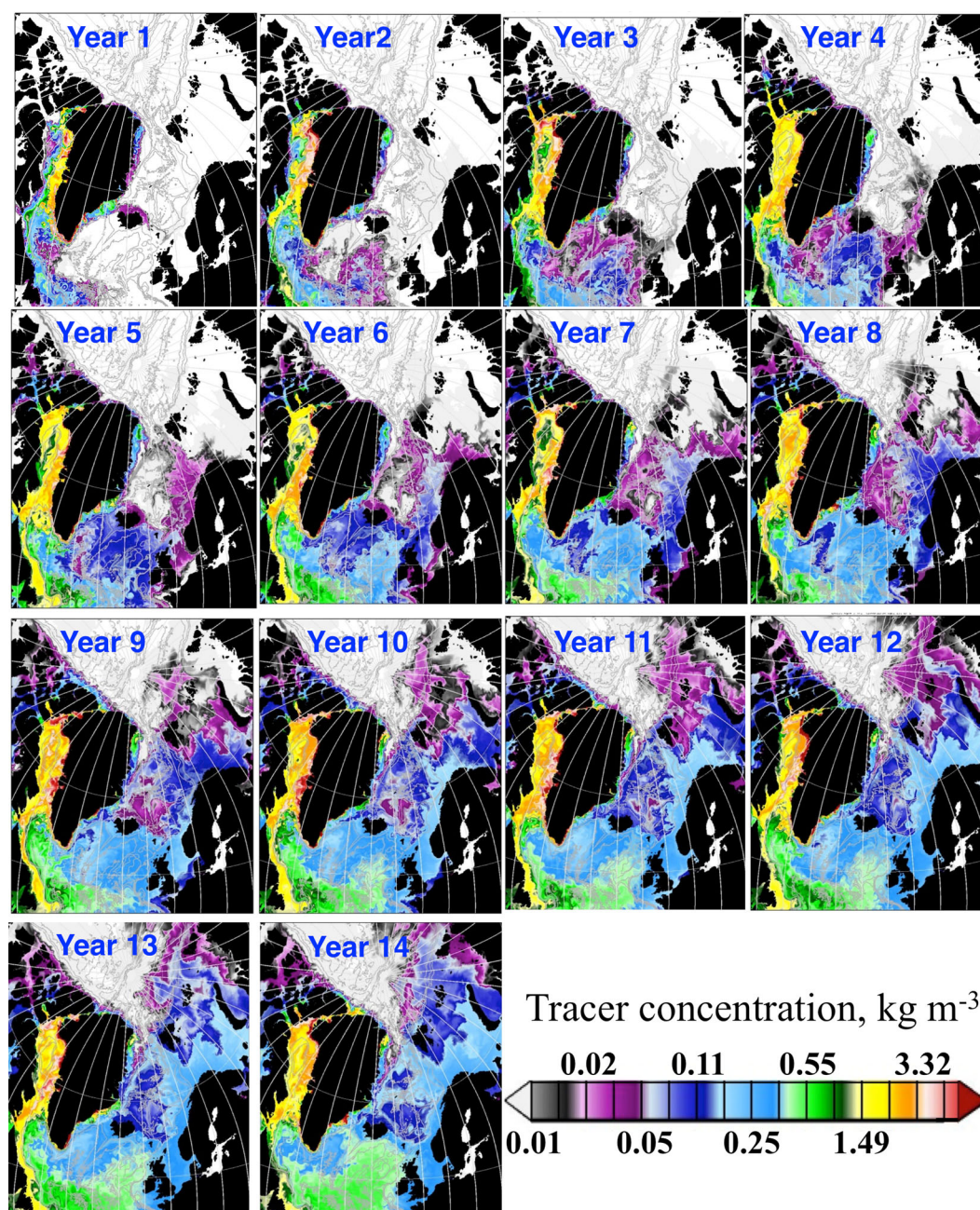
Figure 5. Daily mean tracer concentration in the first model layer ( \sim 3 m) on 17 December for every model year from AO-HYCOM. The concentration is on the natural-log scale ( \text{kg m}^{-3} ). See animated fields of daily mean tracer concentration from AO-HYCOM in Supporting information.
