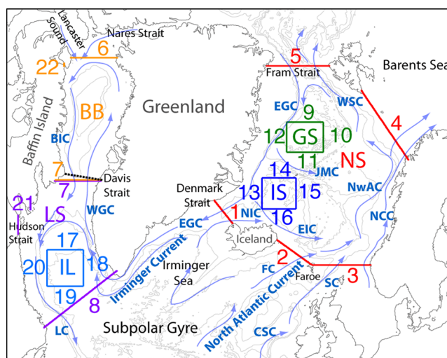
Figure 1. Map of the sub-Arctic seas with general circulation and geographic names shown, including the regions selected for tracer budget analysis (section 4). Three main basins include the Nordic Seas (NS), the Labrador Sea (LS), and Baffin Bay (BB). The boxes are interior regions in the Greenland Sea (GS), Iceland Sea (IS), and interior Labrador Sea (IL). The numbers indicate segments bounding the regions. Color coding is used for ease of identification of the segments bounding the regions. The dashed black line across Davis Strait shows the location of the 2004–present moored array. Abbreviated currents: CSC – Continental Slope Current, FC – Faroe Current, SC – Shetland Current, NCC – Norwegian Coastal Current, NWAC – Norwegian Atlantic Current, WSC – West Spitsbergen Current, EGC – East Greenland Current, JMC – Jan Mayen Current, EIC – East Icelandic Current, NIC – North Icelandic Current, WGC – West Greenland Current, BIC – Baffin Island Current, LC – Labrador Current.
