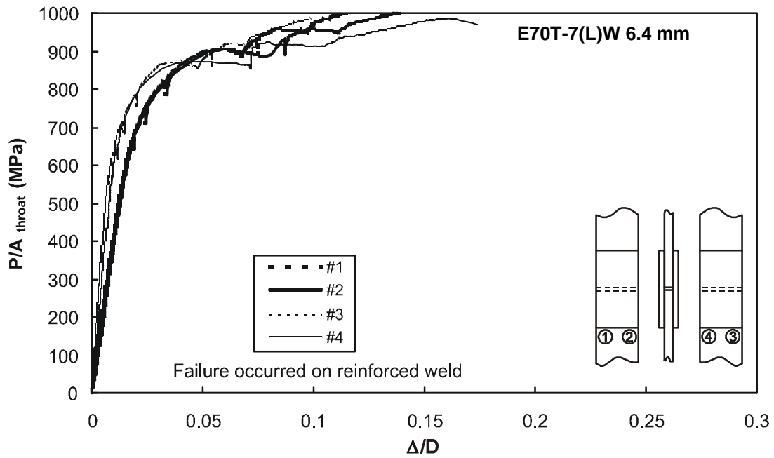
Figure F38 – Specimen 13-2 with 6.4 mm weld from E70T-7 electrode
