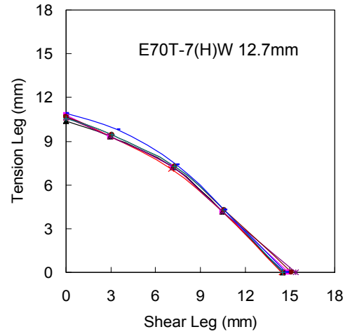
Figure C73 – Weld Profile for Specimen T25-1
