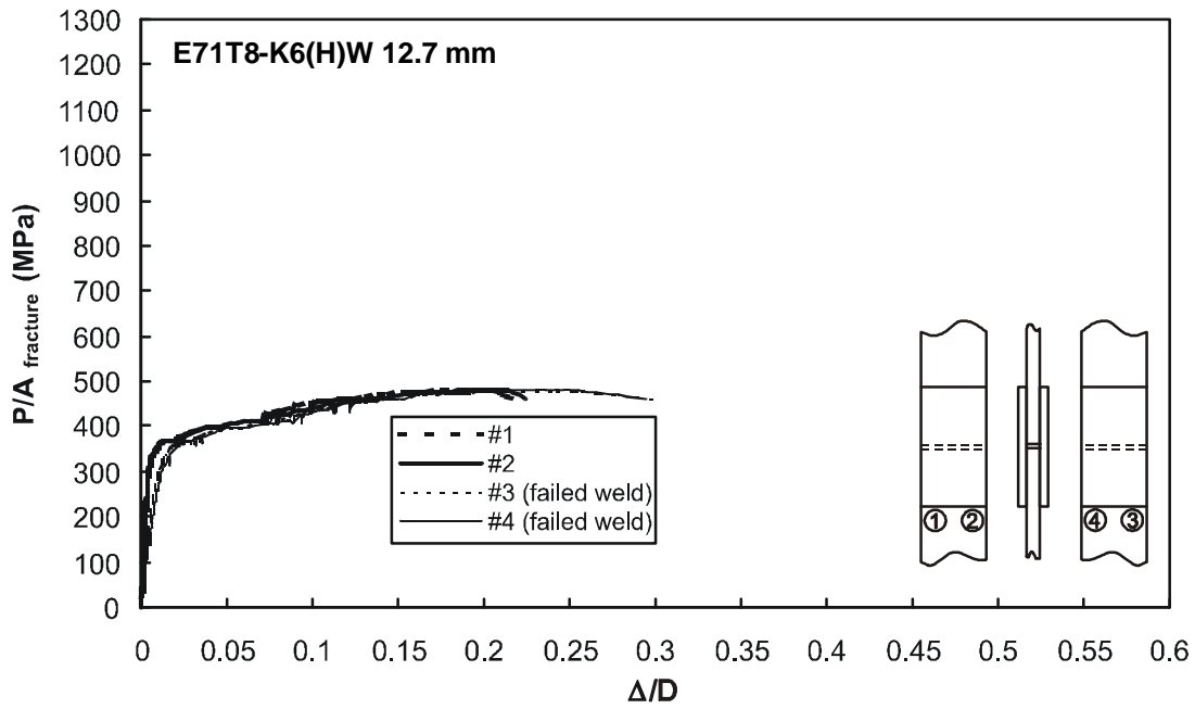
Figure F93 – Specimen T31-3 with 12.7 mm weld from E71T8-K6 electrode
