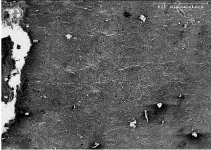
Figure H11 –Fracture Surface of Test Specimen T22-2
