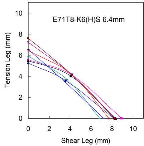
Figure C57 – Weld Profile for Specimen T19-3
