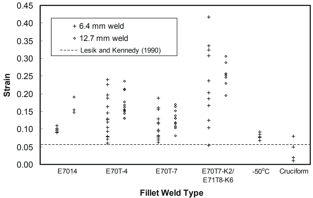
(b) Fillet Weld Ductility at Fracture
