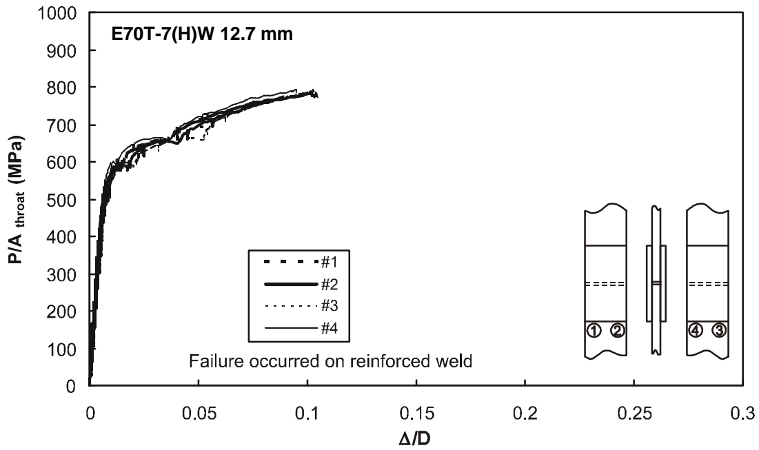
Figure F73 – Specimen T25-1 with 12.7 mm weld from E70T-7 electrode
