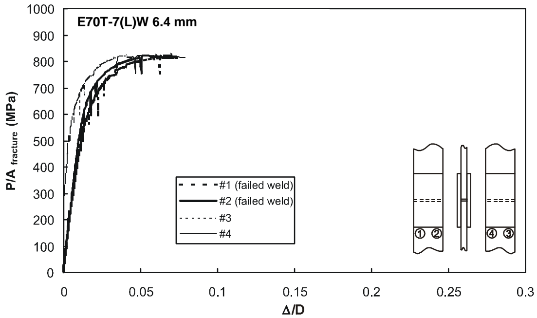
Figure F37 – Specimen 13-1 with 6.4 mm weld from E70T-7 electrode
