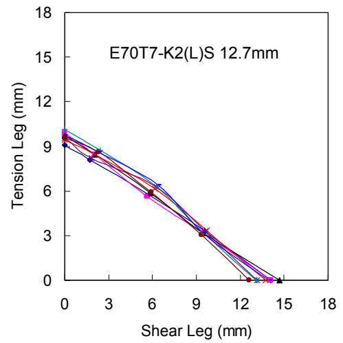
Figure C89 – Weld Profile for Specimen T30-2
