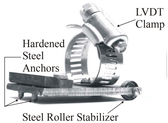
(c) LVDT Bracket
