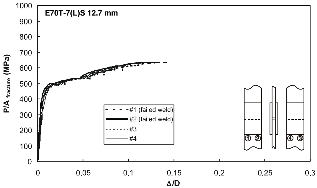
Figure F82 – Specimen T28-1 with 12.7 mm weld from E70T-7 electrode
