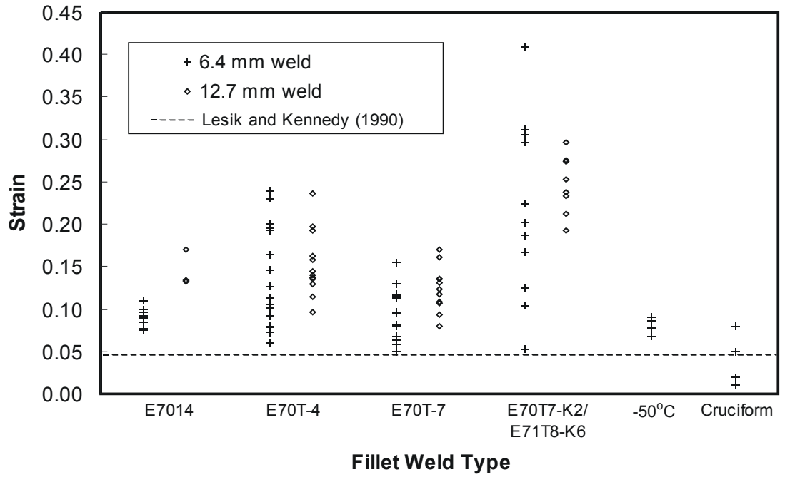
(a) Fillet Weld Ductility at Ultimate Load
