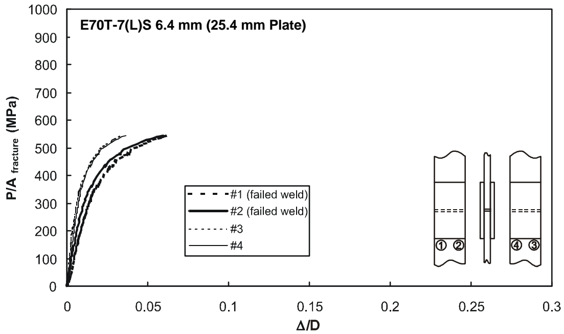
Figure F45 – Specimen T15-3 with 6.4 mm weld from E70T-7 electrode
