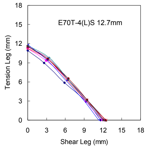
Figure C71 – Weld Profile for Specimen T24-2
