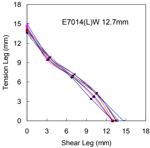
Figure C58 – Weld Profile for Specimen T20-1
