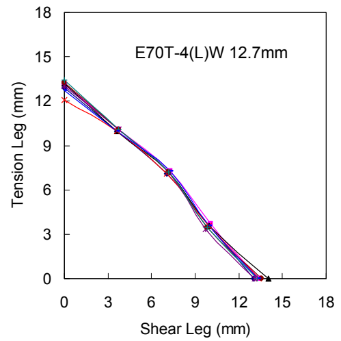
Figure C68 – Weld Profile for Specimen T23-2
