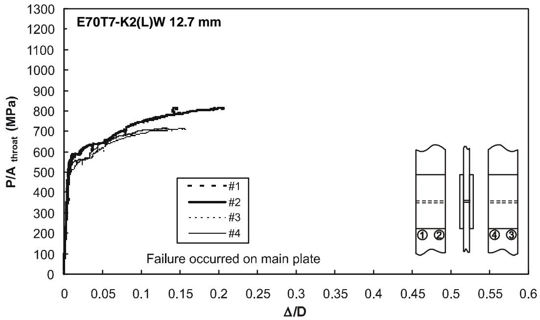
Figure F85 – Specimen T29-1 with 12.7 mm weld from E70T7-K2 electrode
