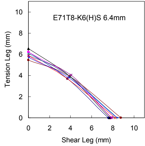
Figure C56 – Weld Profile for Specimen T19-2
