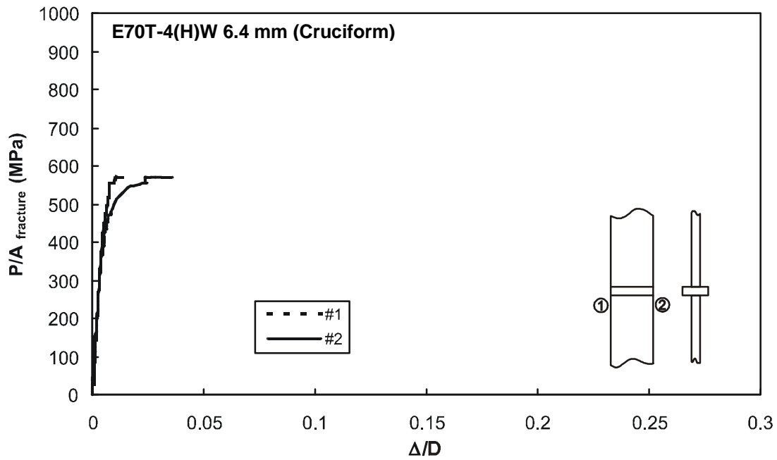
Figure F98 – Specimen C1-2 with 6.4 mm weld from E70T-4 electrode
