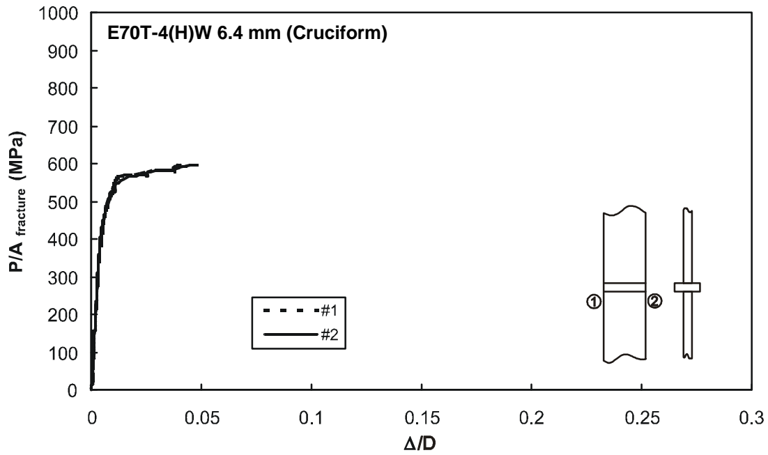
Figure F97 – Specimen C1-1 with 6.4 mm weld from E70T-4 electrode
