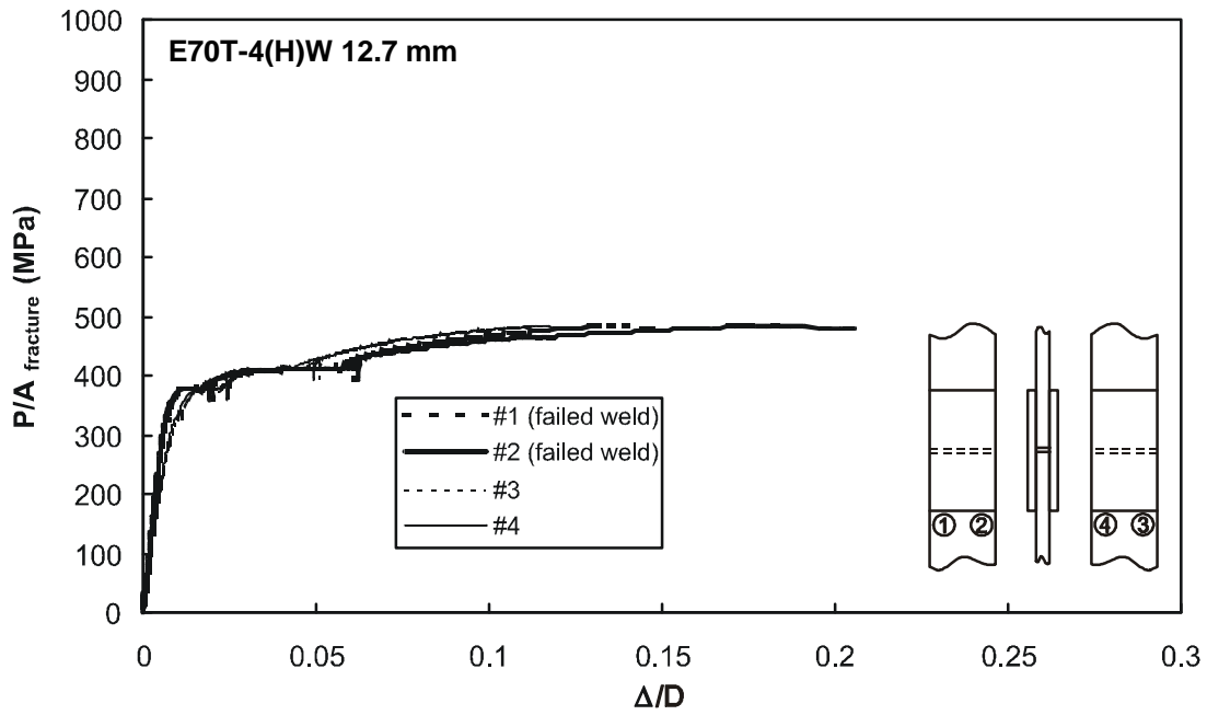
Figure F61 – Specimen T21-1 with 12.7 mm weld from E70T-4 electrode
