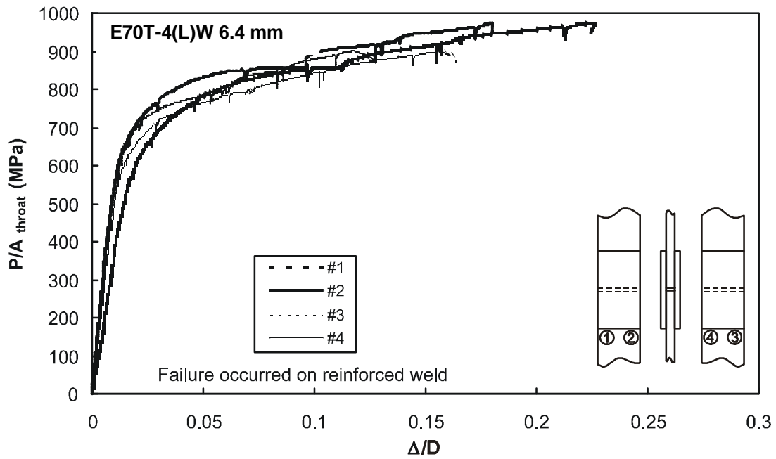
Figure F22 – Specimen T8-1 with 6.4 mm weld from E70T-4 electrode
