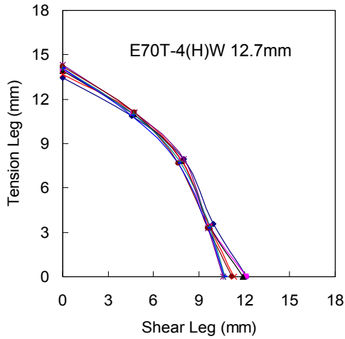
Figure C61 – Weld Profile for Specimen T21-1
