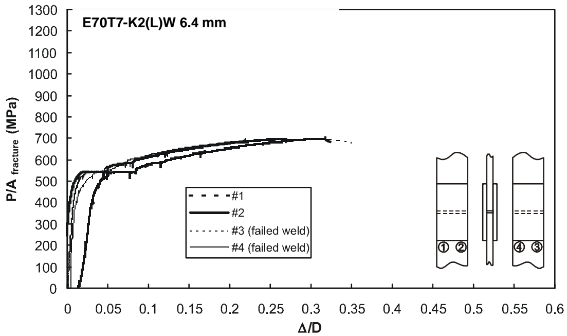
Figure F46 – Specimen T16-1 with 6.4 mm weld from E70T7-K2 electrode
