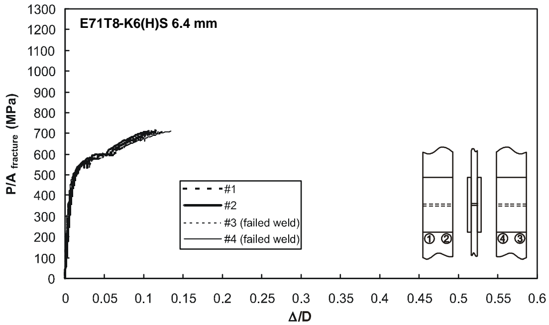
Figure F57 – Specimen T19-3 with 6.4 mm weld from E71T8-K6 electrode
