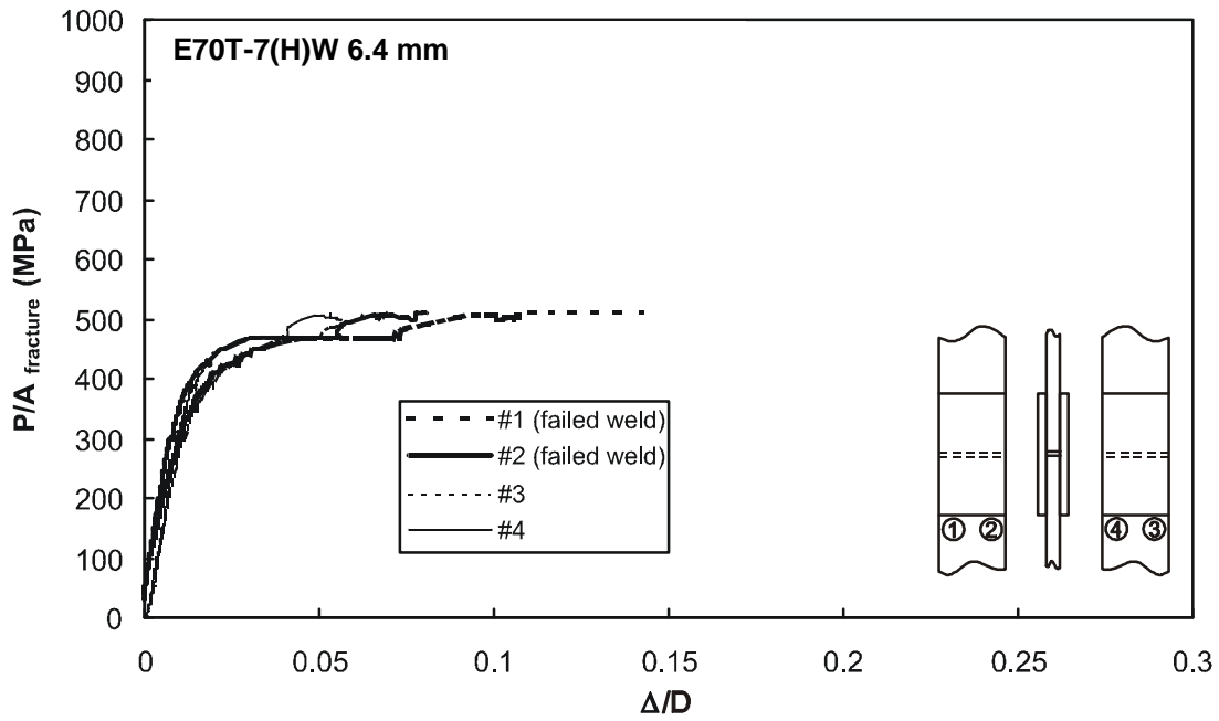
Figure F33 – Specimen T11-3 with 6.4 mm weld from E70T-7 electrode
