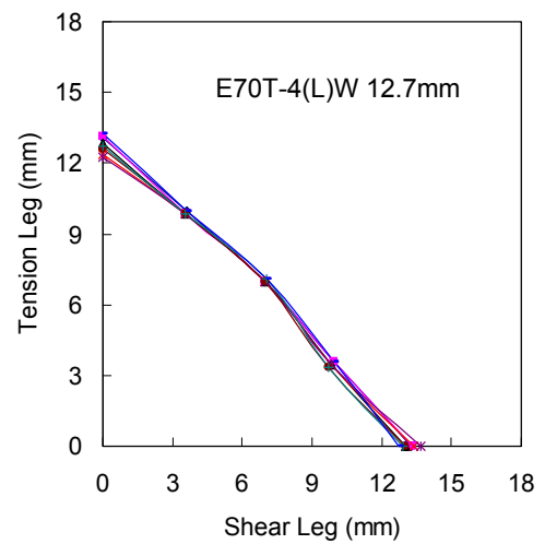
Figure C69 – Weld Profile for Specimen T23-3
