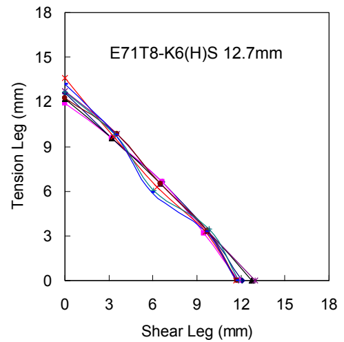
Figure C95 – Weld Profile for Specimen T32-2
