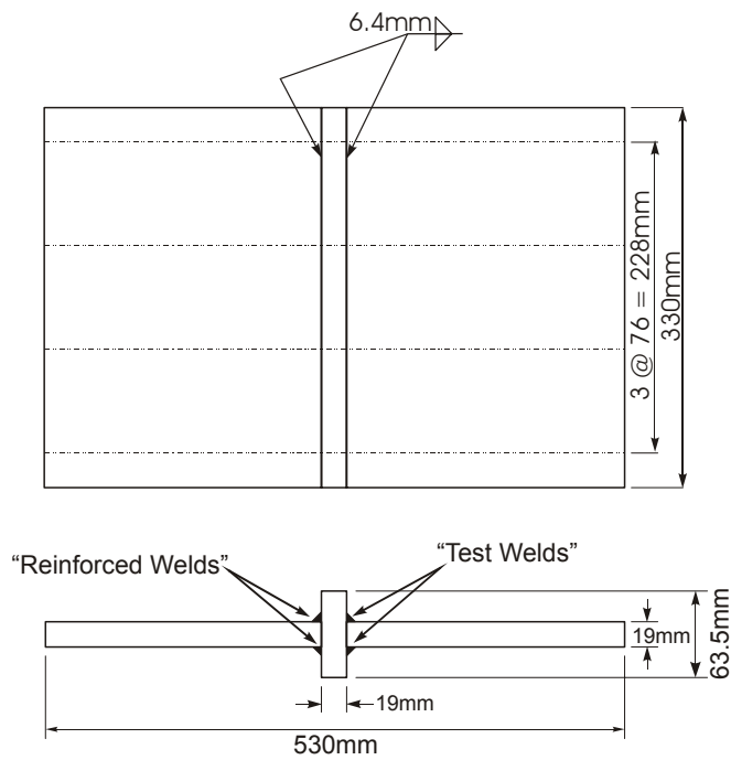
(b) Cruciform Specimens
