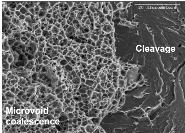
(b) Cleavage and Microvoid Coalescence on Fracture Surface of Specimen T13-1
