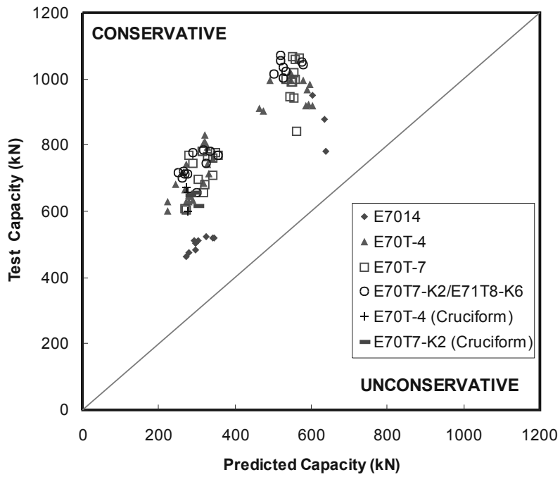
(a) Predicted Capacity Using Nominal Strength
