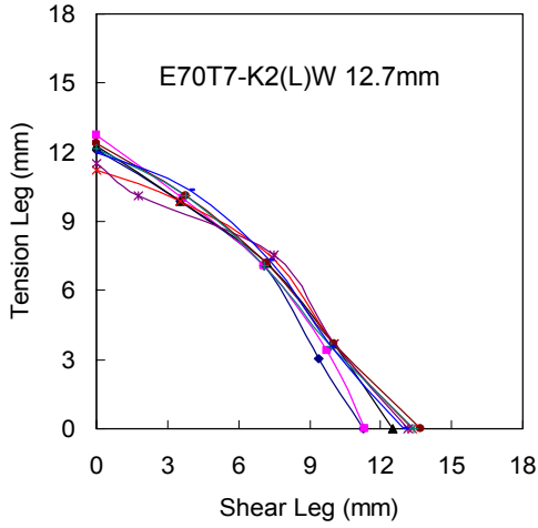
Figure C85 – Weld Profile for Specimen T29-1
