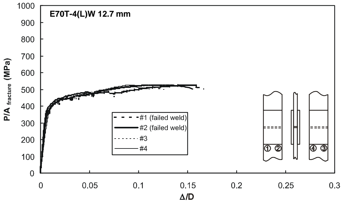
Figure F69 – Specimen T23-3 with 12.7 mm weld from E70T-4 electrode
