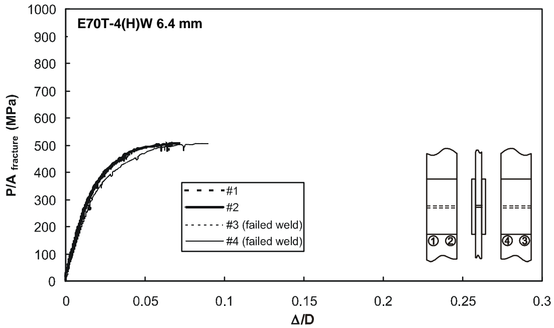
Figure F13 – Specimen T5-1 with 6.4 mm weld from E70T-4 electrode
