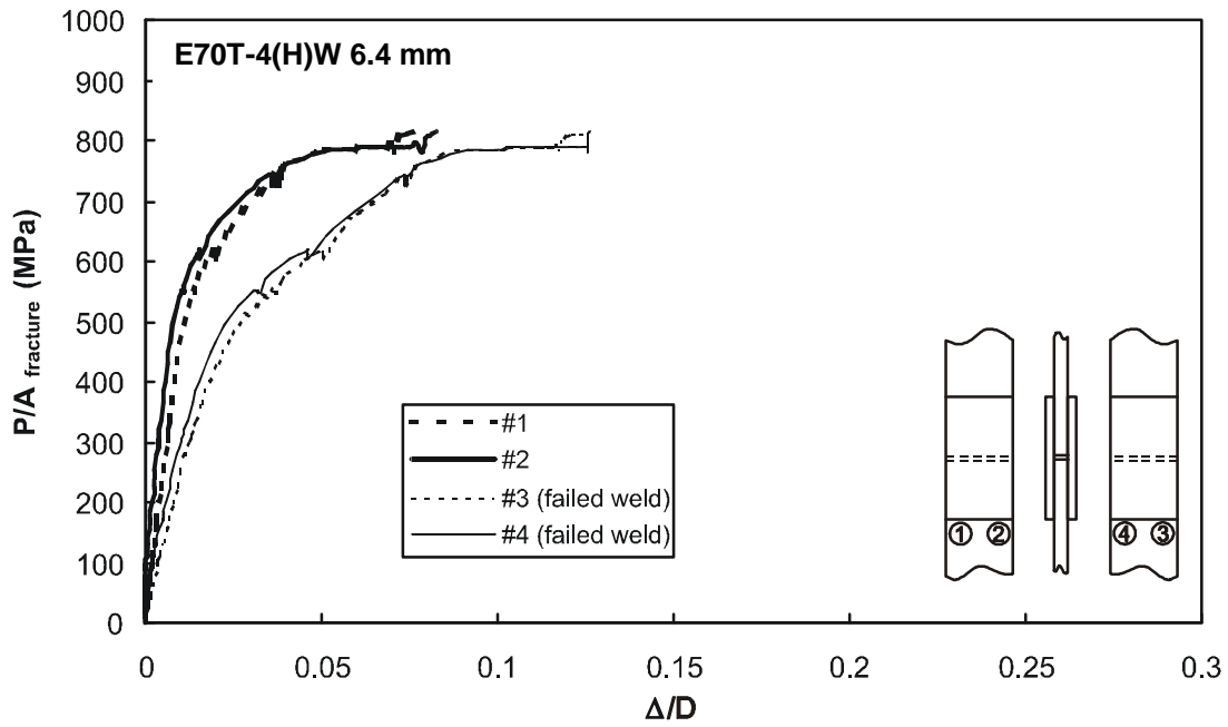
Figure F17 – Specimen T6-2 with 6.4 mm weld from E70T-4 electrode
