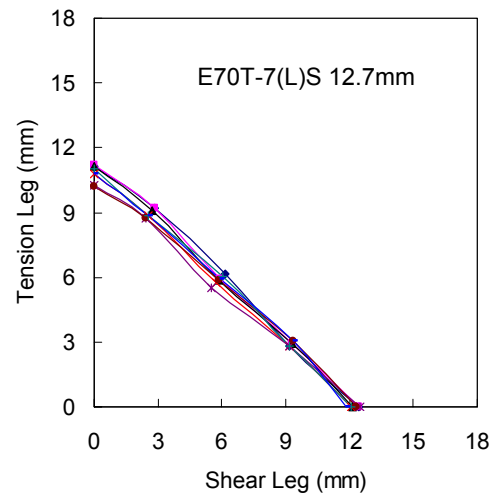
Figure C83 – Weld Profile for Specimen T28-2
