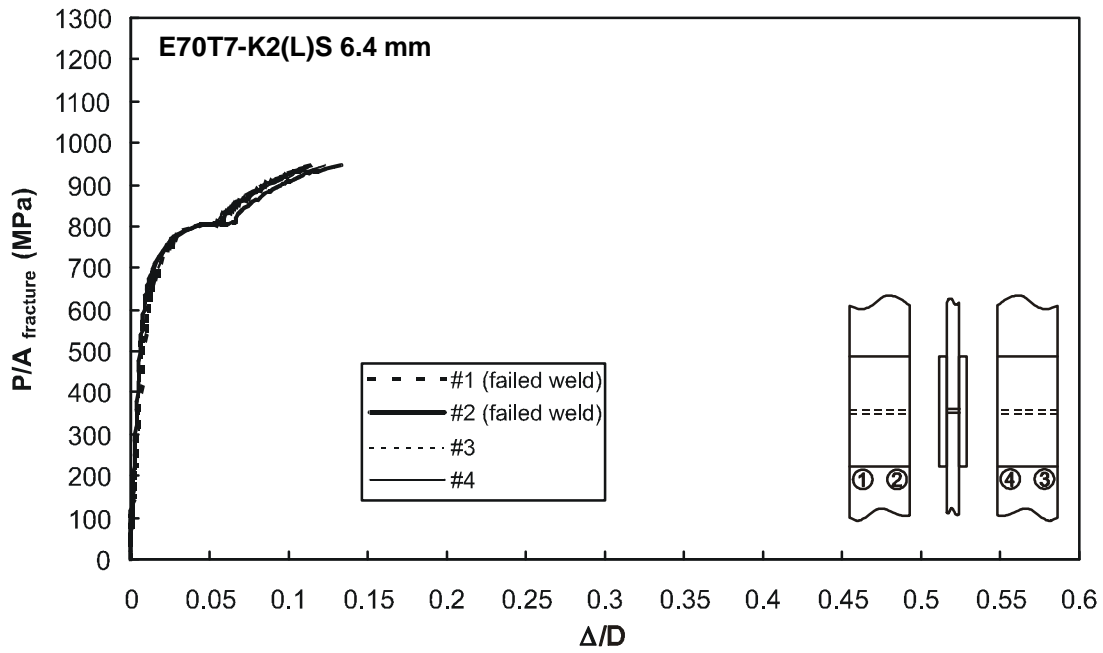
Figure F49 – Specimen T17-1 with 6.4 mm weld from E70T7-K2 electrode
