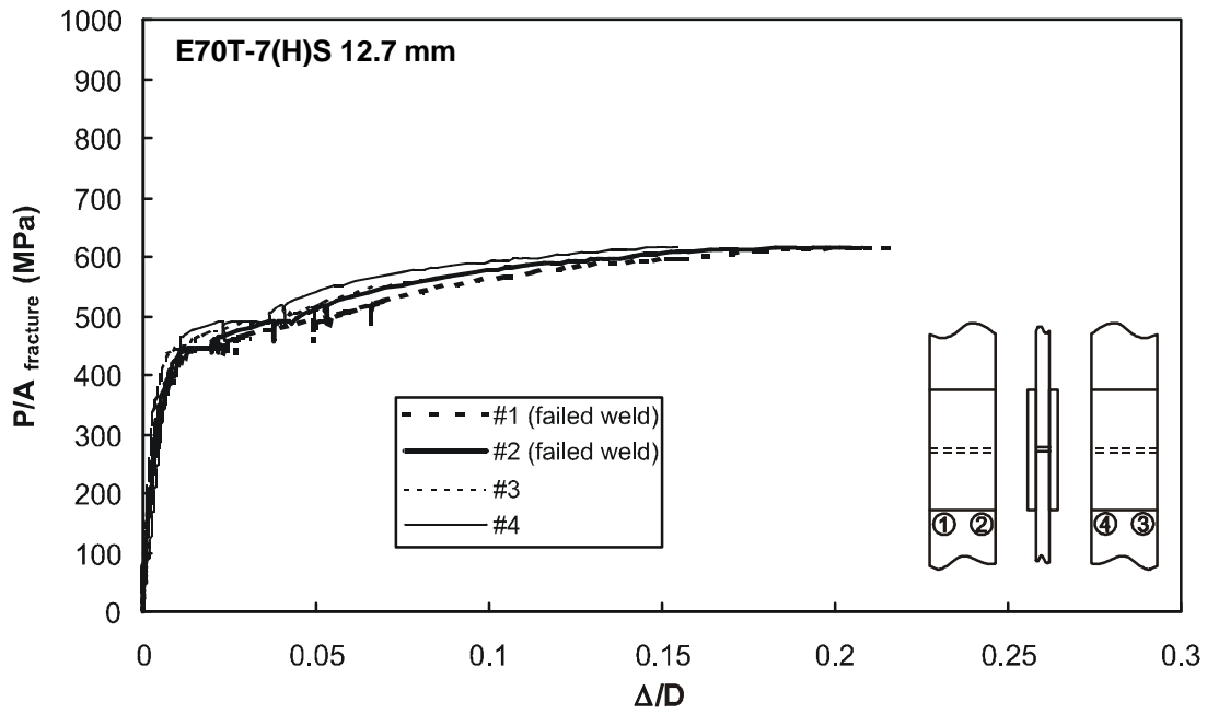
Figure F77 – Specimen T26-2 with 12.7 mm weld from E70T-7 electrode
