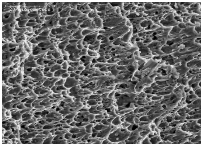
(c) Elongated Microvoids on Fracture Surface of Specimen T32-2
