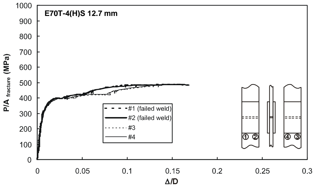
Figure F66 – Specimen T22-3 with 12.7 mm weld from E70T-4 electrode
