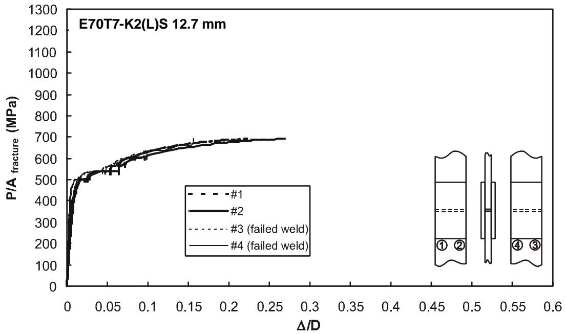
Figure F89 – Specimen T30-2 with 12.7 mm weld from E70T7-K2 electrode
