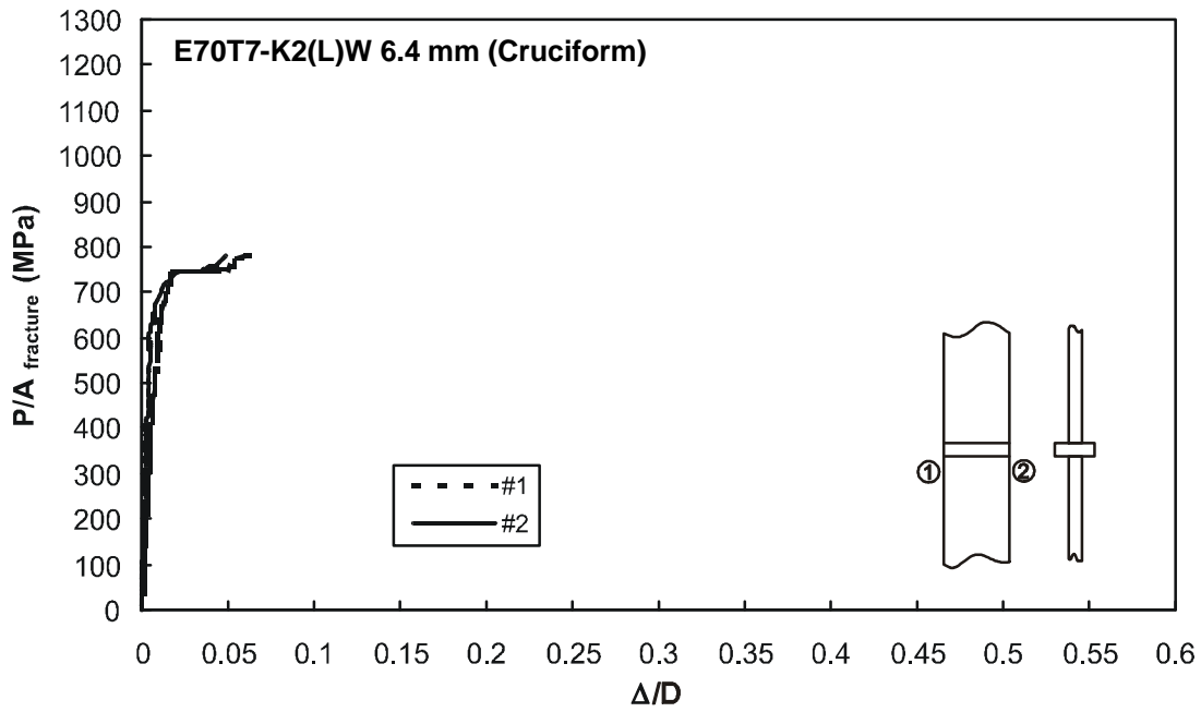
Figure F101 – Specimen C2-2 with 6.4 mm weld from E70T7-K2 electrode
