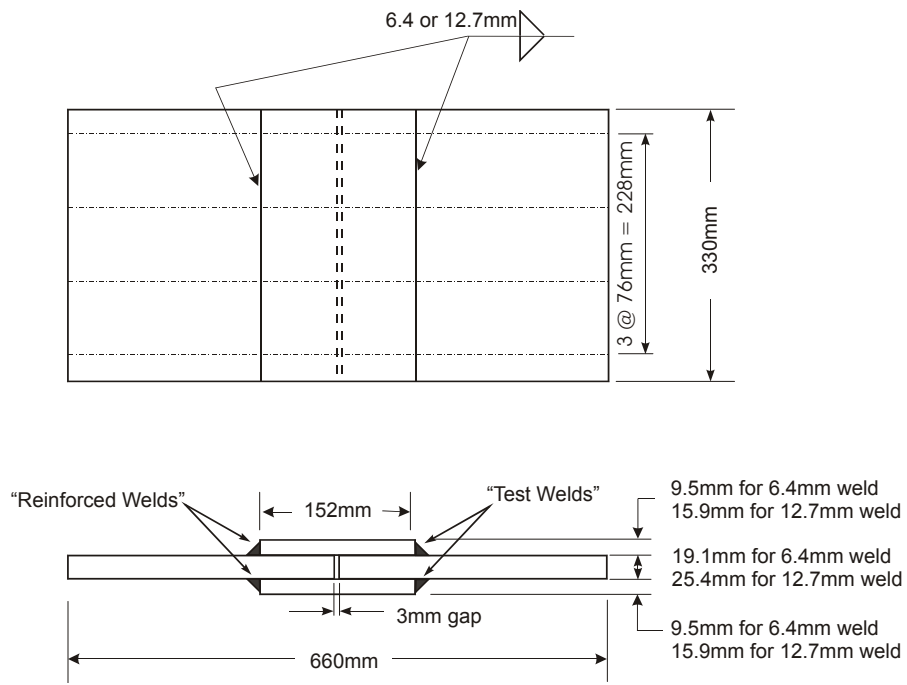
(a) Lapped Splice Specimens
