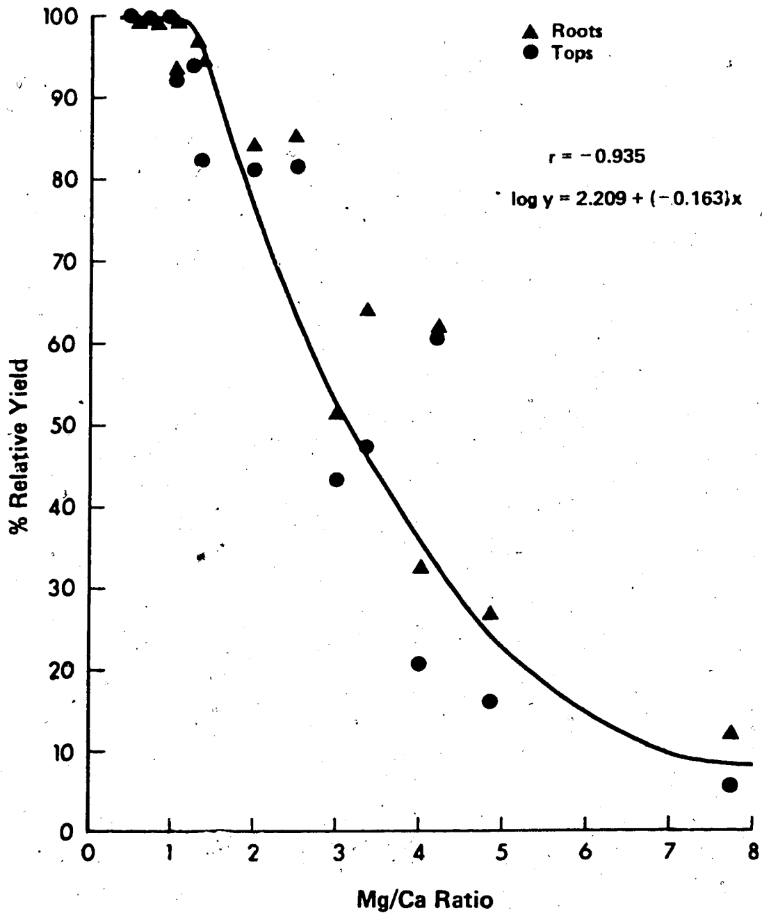
Figure 4. Correlation between Mg/Ca ratios in solution and relative yield of tops and roots of barley in experiments I, II and III
