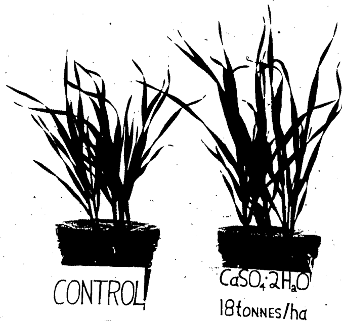
10. Effect of added gypsum on barley growth on a Duagh Ap (Chipman) horizon
