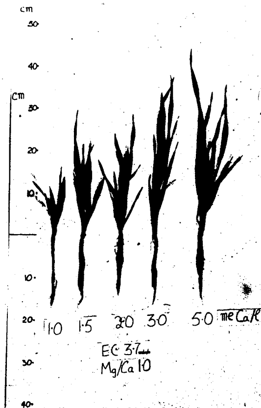
5. Effect of an increasing Ca/TC ratio on growth of barley in experiment IV
