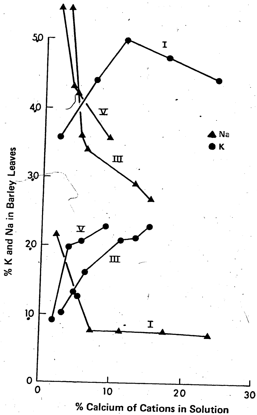
Figure 8. Uptake of potassium and sodium at different levels of calcium in solution from experiments I, III and V.
