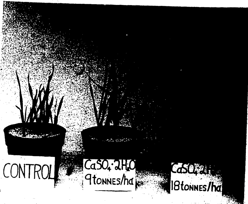
9. Effect of added gypsum on barley growth on a Killam Bnt horizon
