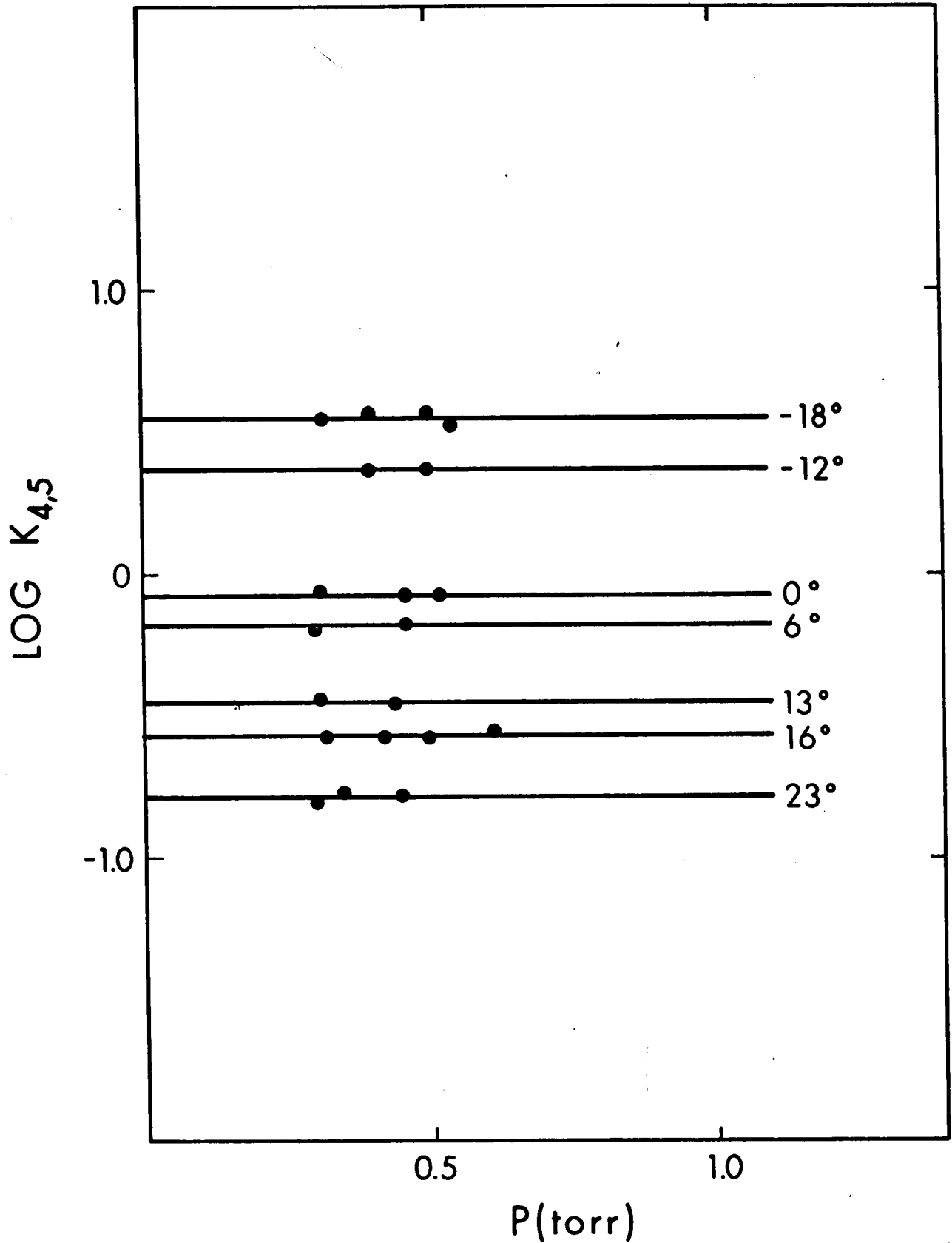
FIGURE 3.17 Plots of Log K_{4,5} for the Gas Phase Hydration of Rb^+ , at Various Temperatures, Versus Pressure of H_2O
