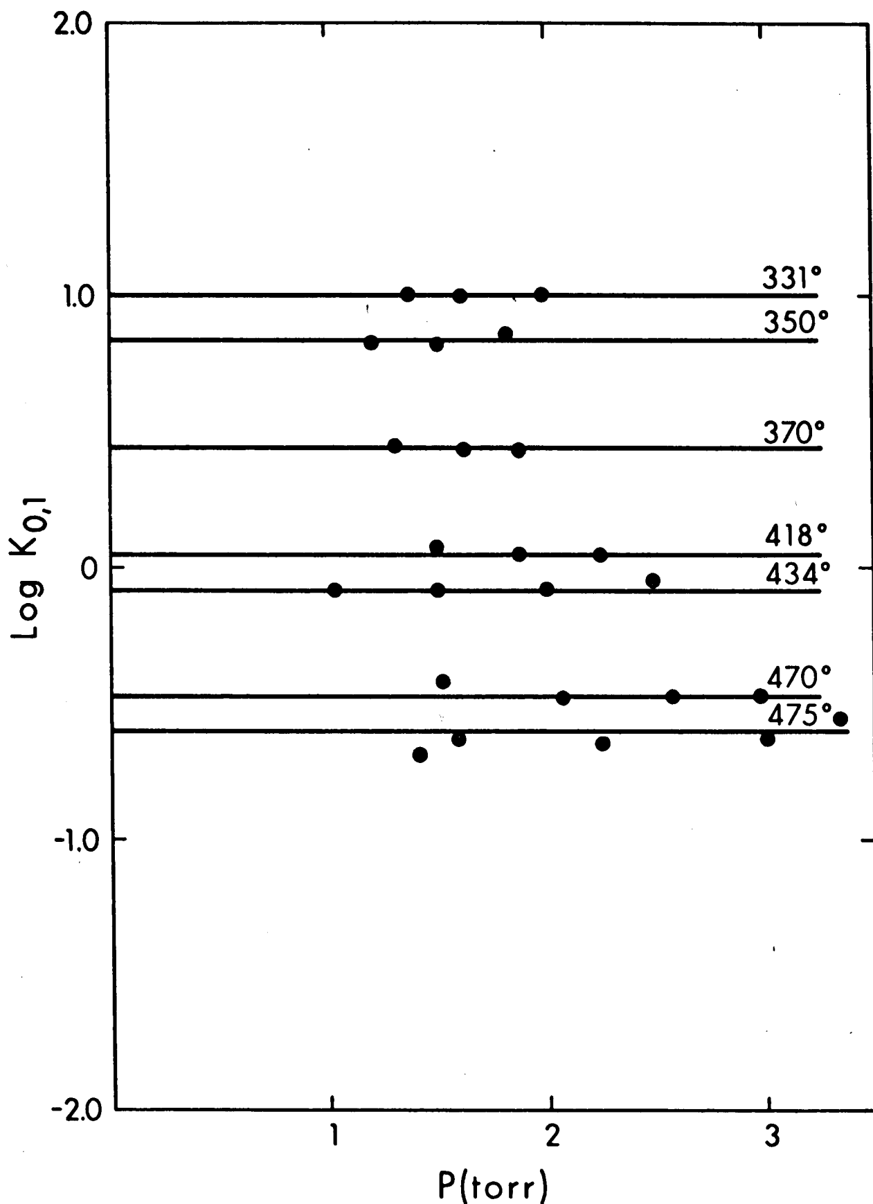
FIGURE 3.6 Plots of \text{Log } K_{0,1} for the Gas Phase Hydration of \text{Na}^+ , at Various Temperatures, Versus Pressure of \text{H}_2\text{O} .
