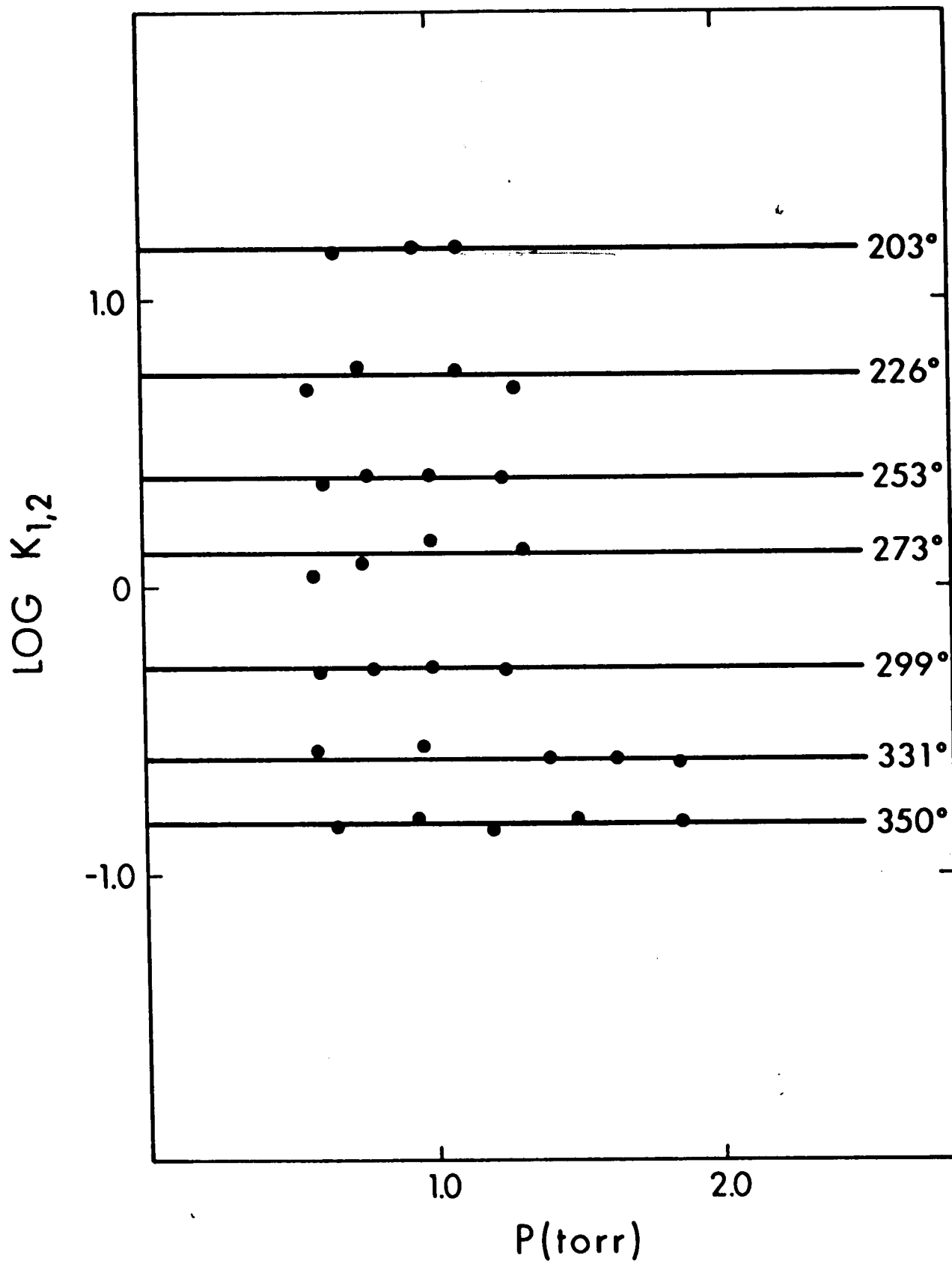
FIGURE 3.7 Plots of \text{Log } K_{1,2} for the Gas Phase Hydration of \text{Na}^+ , at Various Temperatures, Versus Pressure of \text{H}_2\text{O} .
