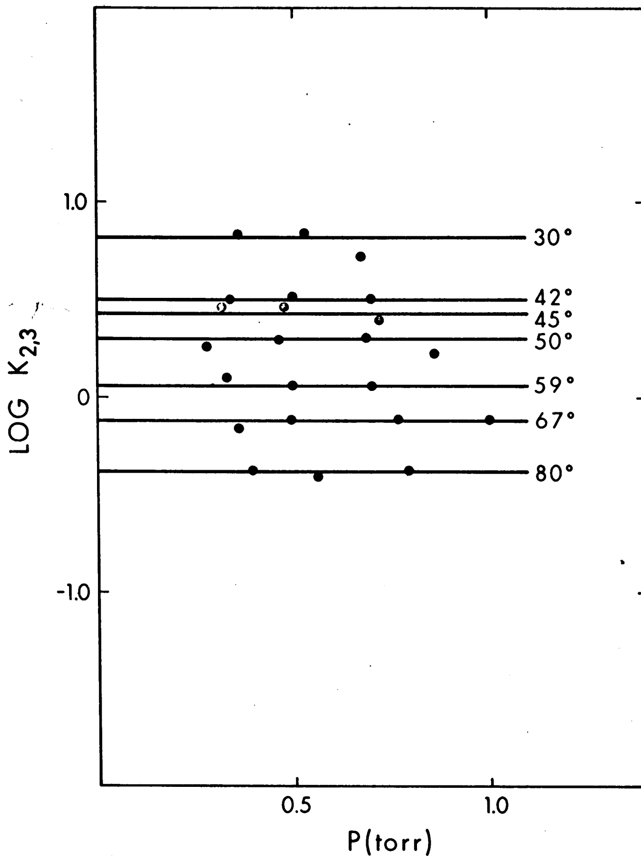
FIGURE 3.15 Plots of Log K_{2,3} for the Gas Phase Hydration of Rb^+ , at Various Temperatures, Versus Pressure of H_2O
