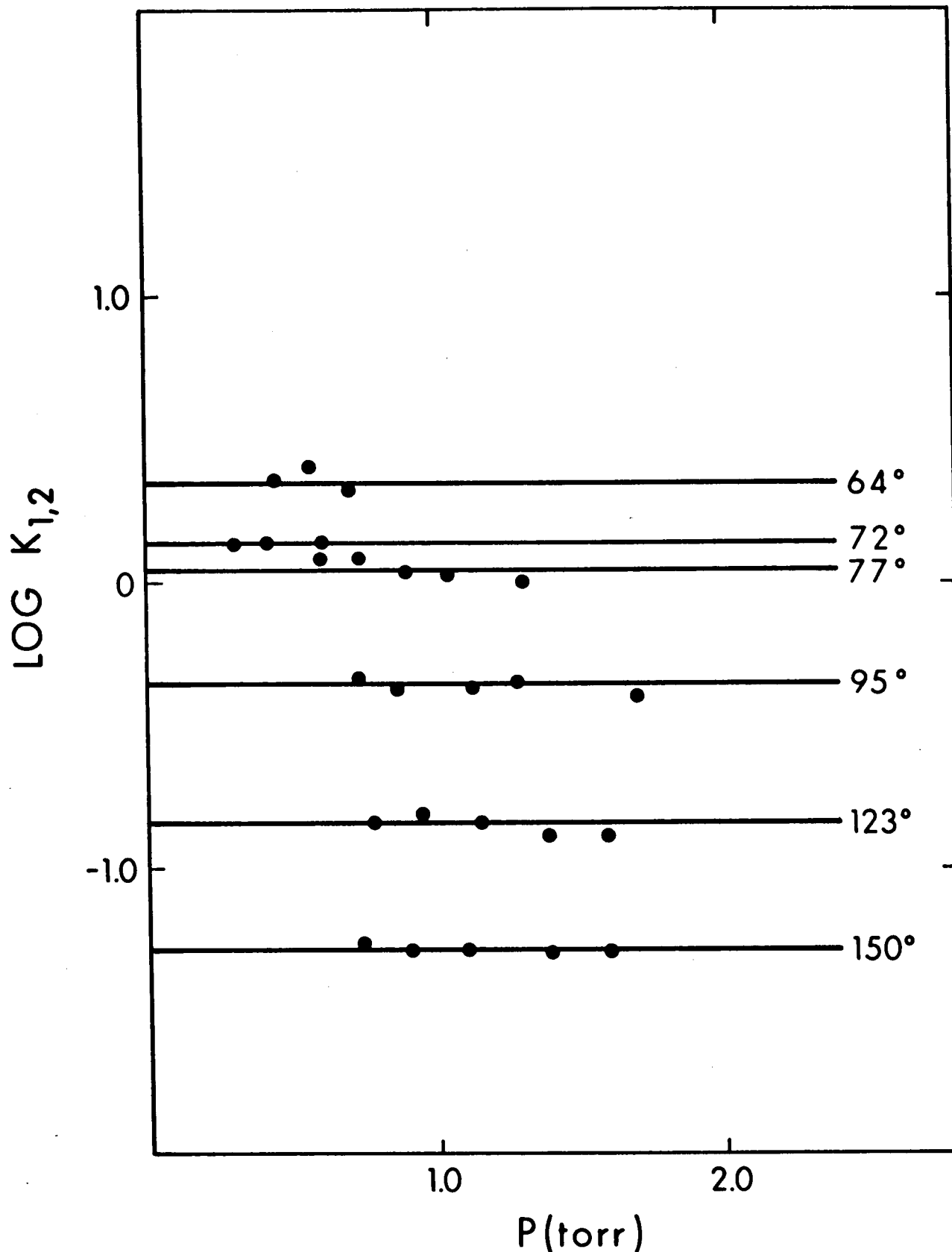
FIGURE 3.19 Plots of Log K_{1,2} for the Gas Phase Hydration of \text{Cs}^+ , at Various Temperatures, Versus Pressure of \text{H}_2\text{O}
