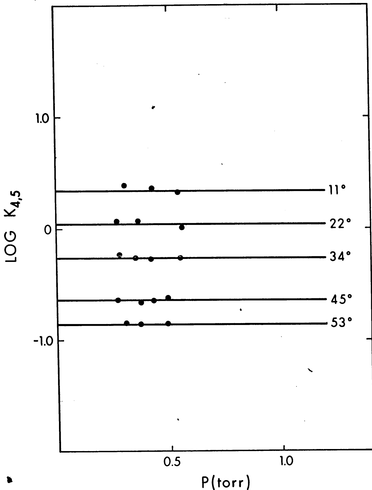
FIGURE 3.11 Plots of \text{Log } K_{4,5} for the Gas Phase Hydration of \text{Na}^+ , at Various Temperatures, Versus Pressure of \text{H}_2\text{O}
