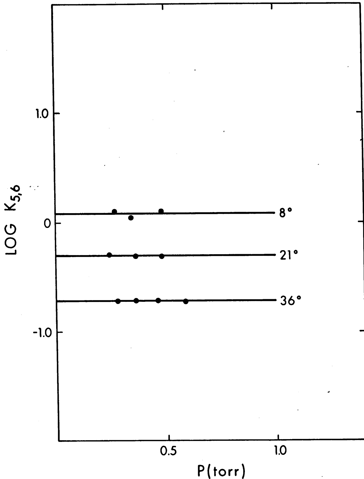
FIGURE 3.5 Plots of Log K_{5,6} for the Gas Phase Hydration of \text{Li}^+ , at Various Temperatures, Versus Pressure of \text{H}_2\text{O} .
