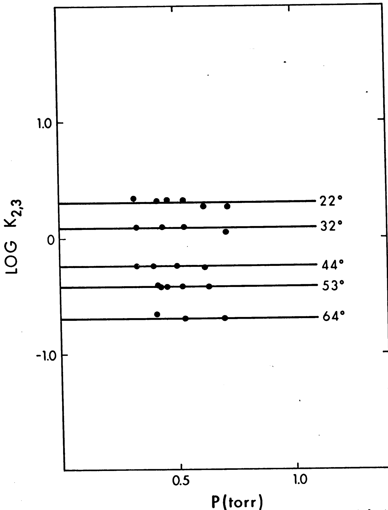
FIGURE 3.20 Plots of Log K_{2,3} for the Gas Phase Hydration of Cs^+ , at Various Temperatures, versus Pressure of H_2O
