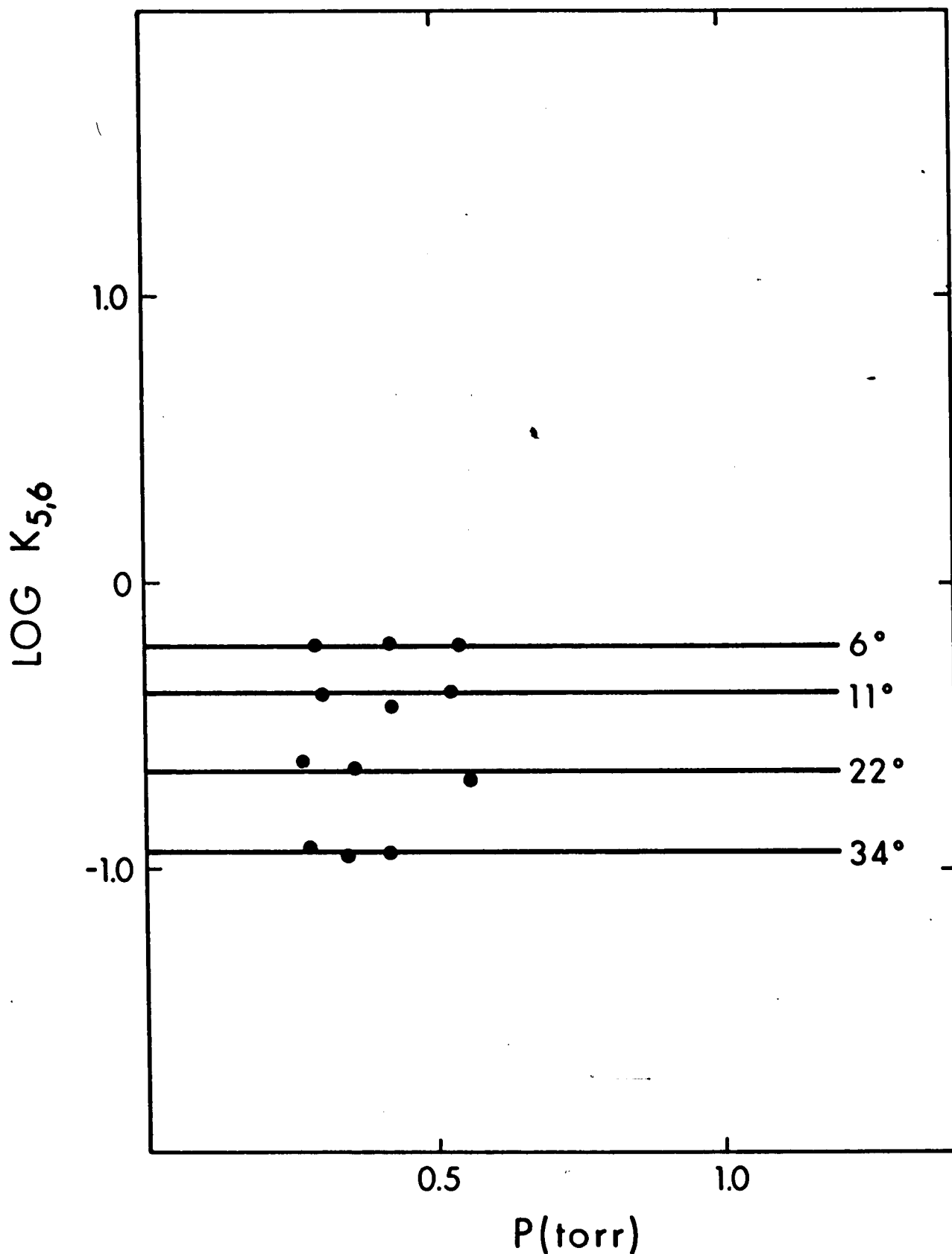
FIGURE 3.12 Plots of \text{Log } K_{5,6} for the Gas Phase Hydration of \text{Na}^+ , at Various Temperatures, Versus Pressure of \text{H}_2\text{O}
