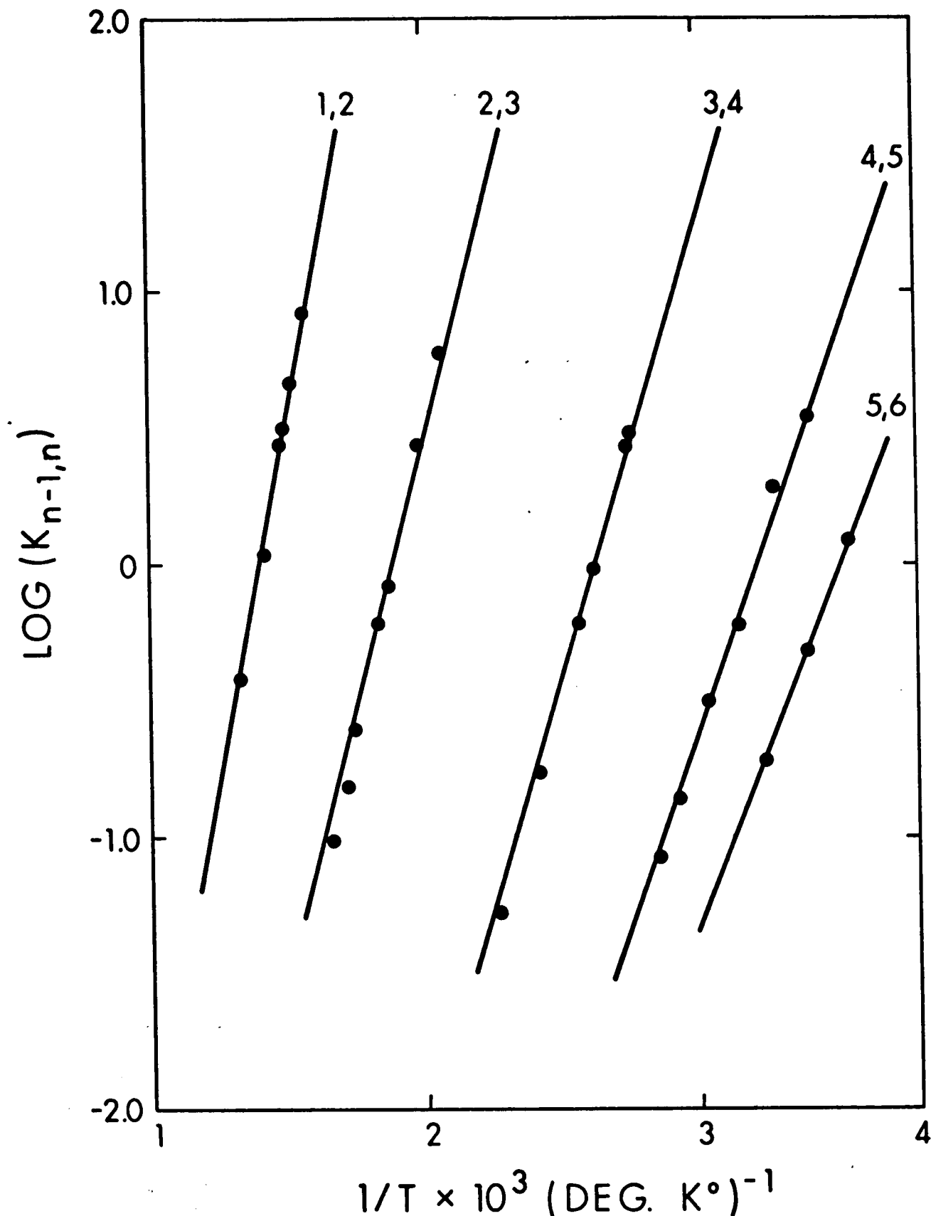
FIGURE 3.22 Van't Hoff Type Plots of the Equilibrium Constants for the Gas Phase Hydration of \text{Li}^+
