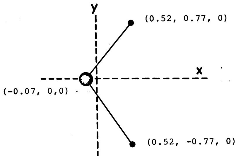
Principal axes of H_2O
