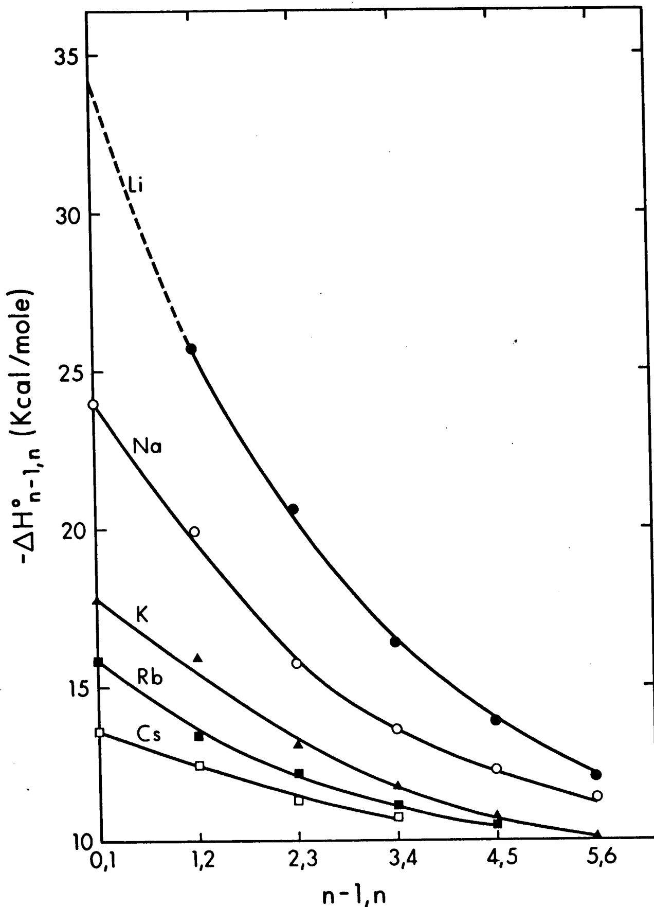
FIGURE 3.26 Enthalpies for Clustering Reactions
