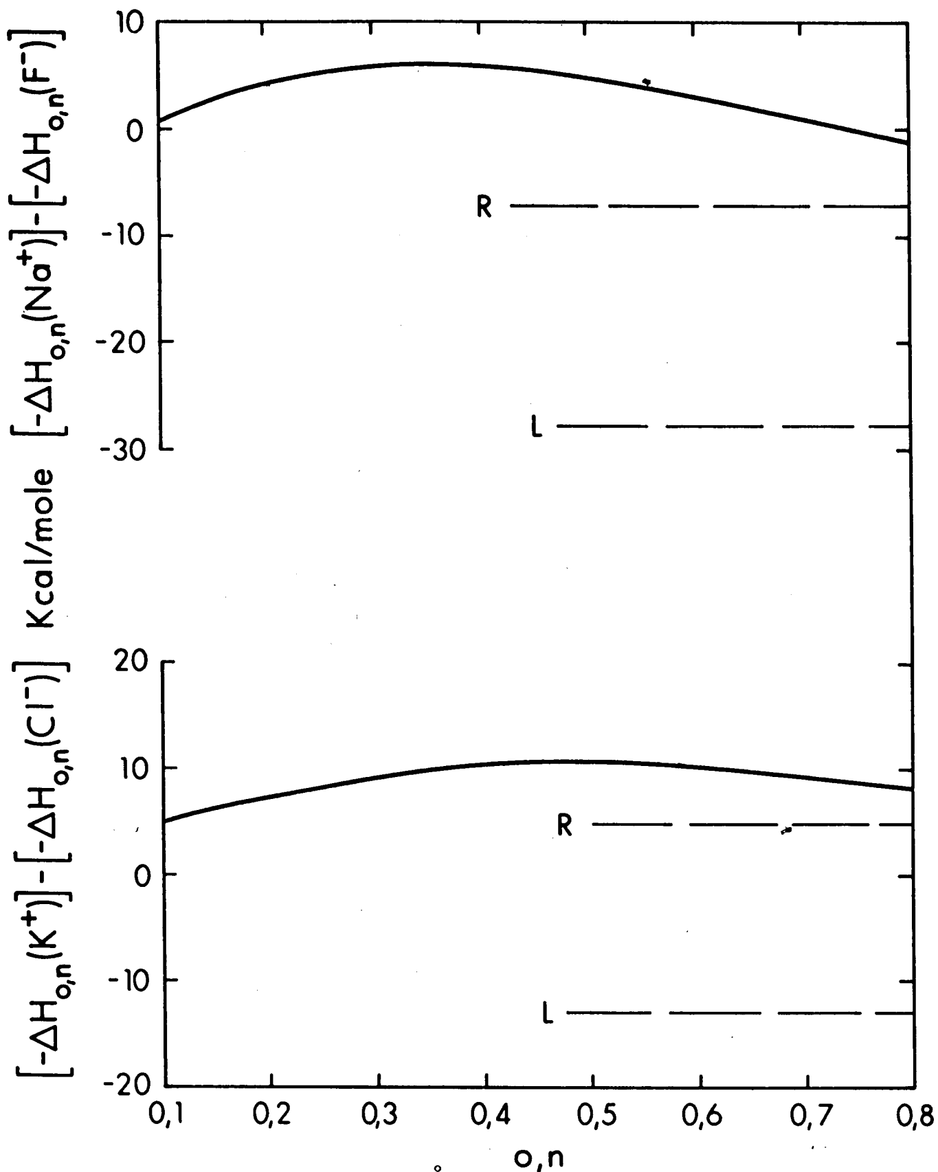
FIGURE 5a Comparison of \Delta H_{o,n}^{\circ} hydration of alkali and halide ions with total enthalpies of hydration of Latimer, Pitzer and Slansky (L) and Randles (R).
