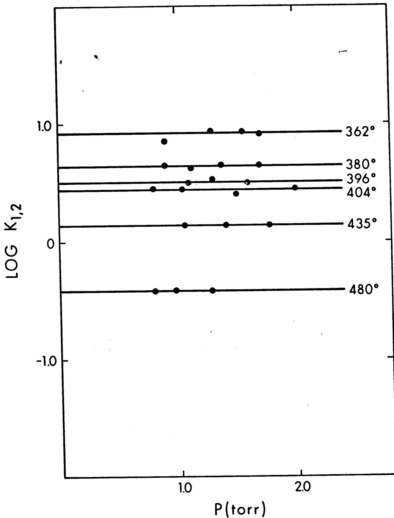
FIGURE 3.1 Plots of Log K_{1,2} for the Gas Phase Hydration of \text{Li}^+ , at Various Temperatures, Versus Pressure of \text{H}_2\text{O} .
