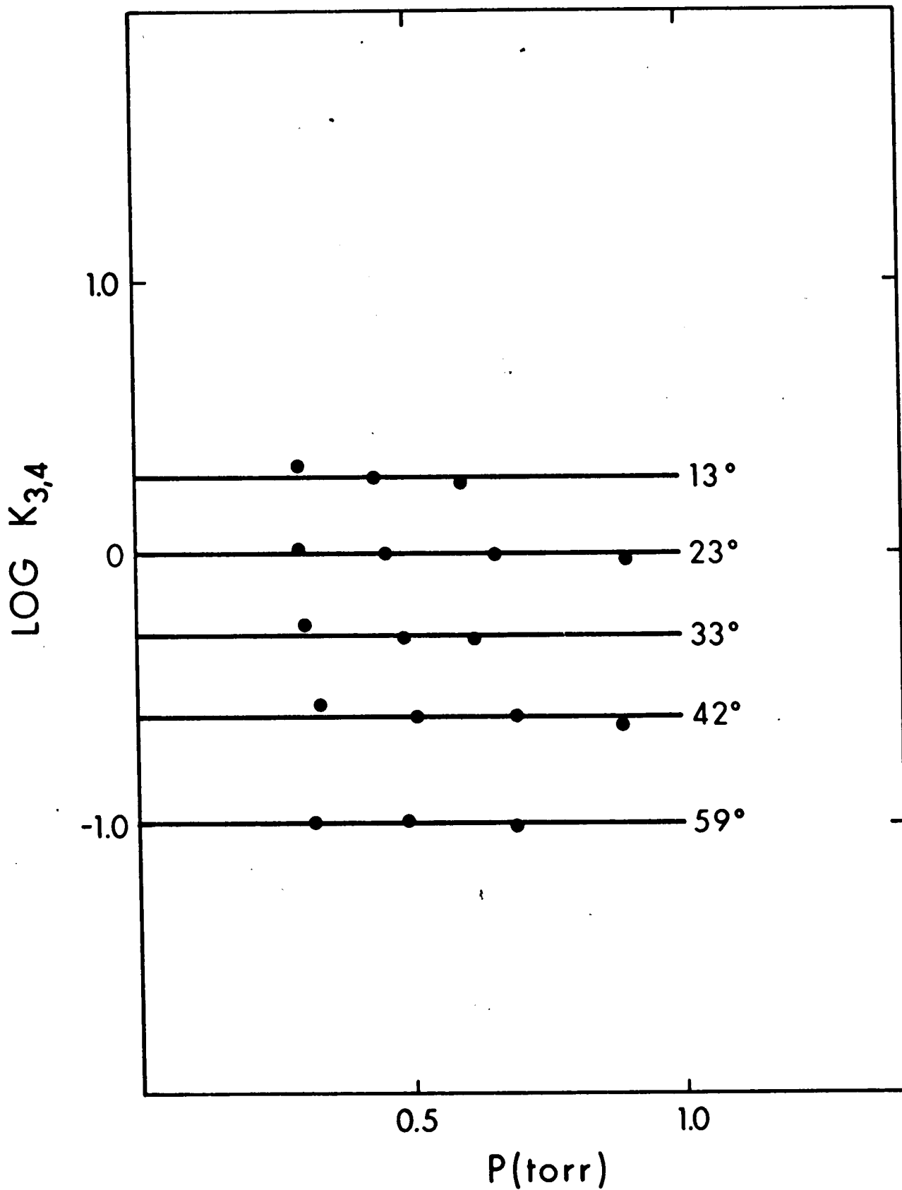
FIGURE 3.16 Plots of \text{Log } K_{3,4} for the Gas Phase Hydration of \text{Rb}^+ , at Various Temperatures, Versus Pressure of \text{H}_2\text{O}
