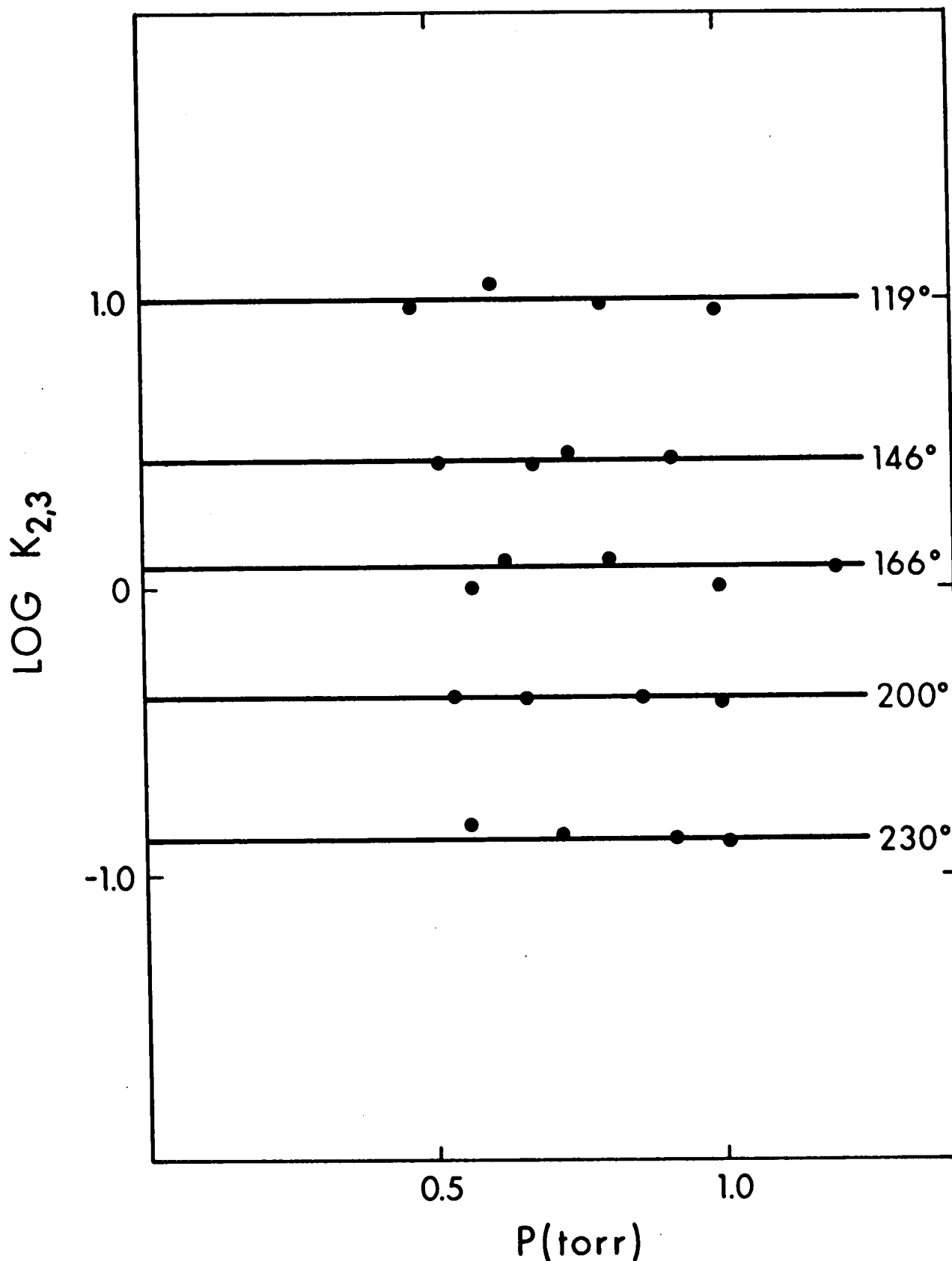
FIGURE 3.8 Plots of \text{Log } K_{2,3} for the Gas Phase Hydration of \text{Na}^+ , at Various Temperatures, Versus Pressure of \text{H}_2\text{O} .
