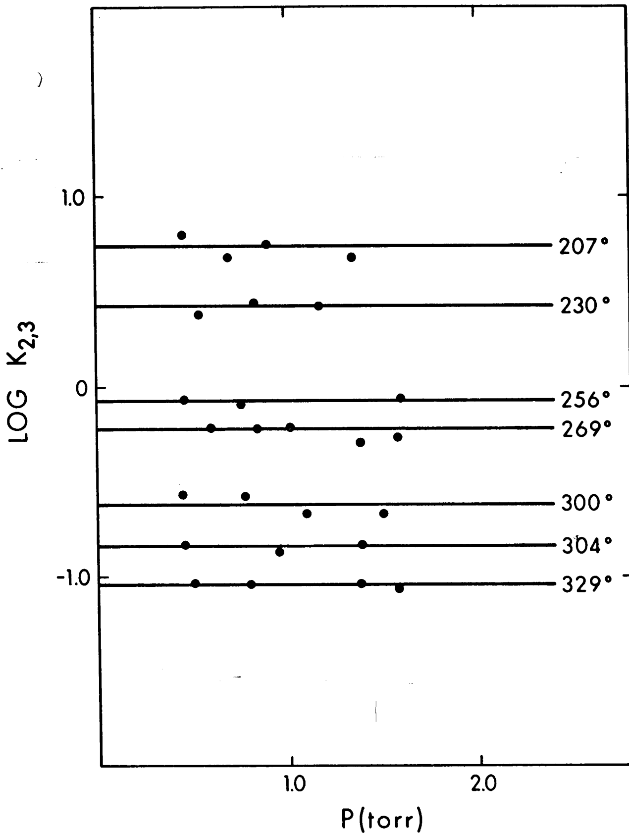
FIGURE 3.2 Plots of \text{Log } K_{2,3} for the Gas Phase Hydration of \text{Li}^+ , at Various Temperatures, Versus Pressure of \text{H}_2\text{O} .
