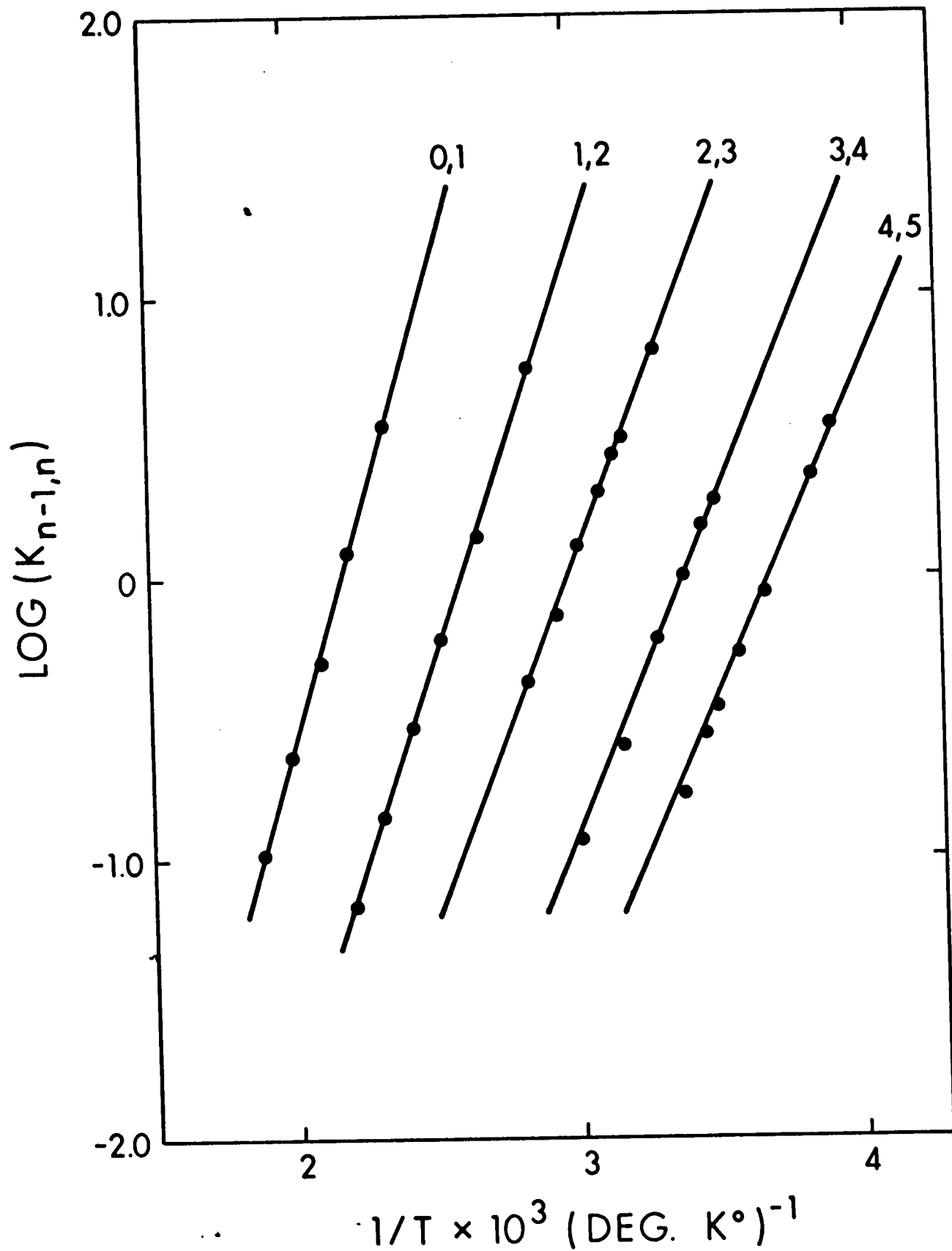
FIGURE 3.24 Van't Hoff Type Plots of the Equilibrium Constants for the Gas Phase Hydration of \text{Rb}^+
