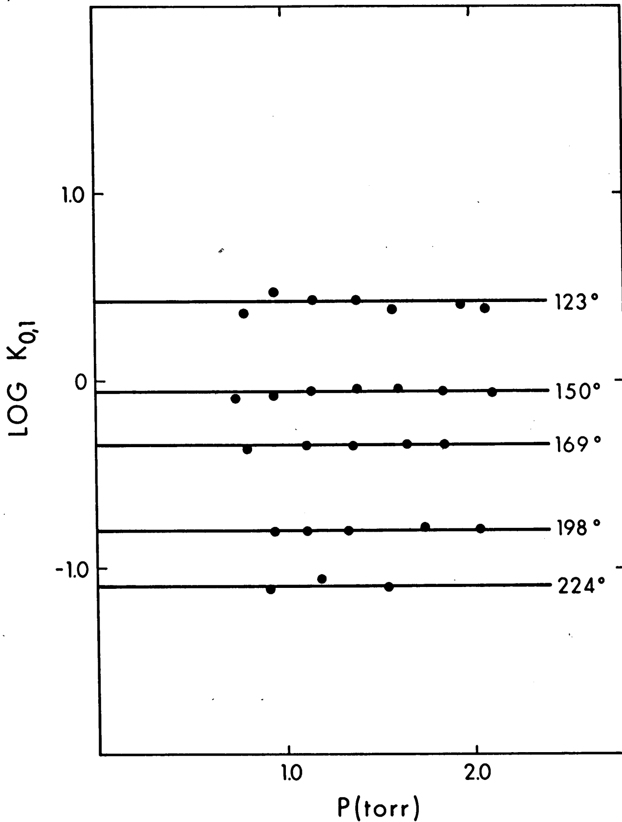
FIGURE 3.18 Plots Of Log K_{0,1} for the Gas Phase Hydration of \text{Cs}^+ , at Various Temperatures, Versus Pressure of \text{H}_2\text{O}
