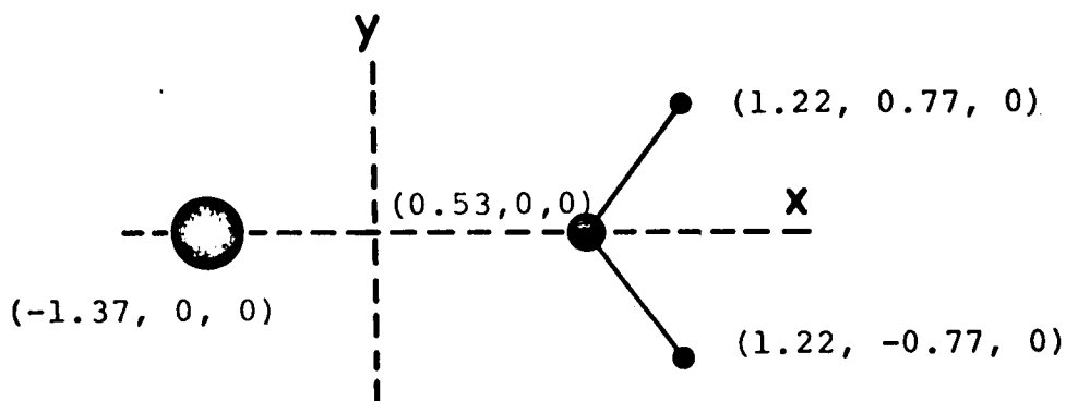
Principal axes of Li^+(H_2O)
