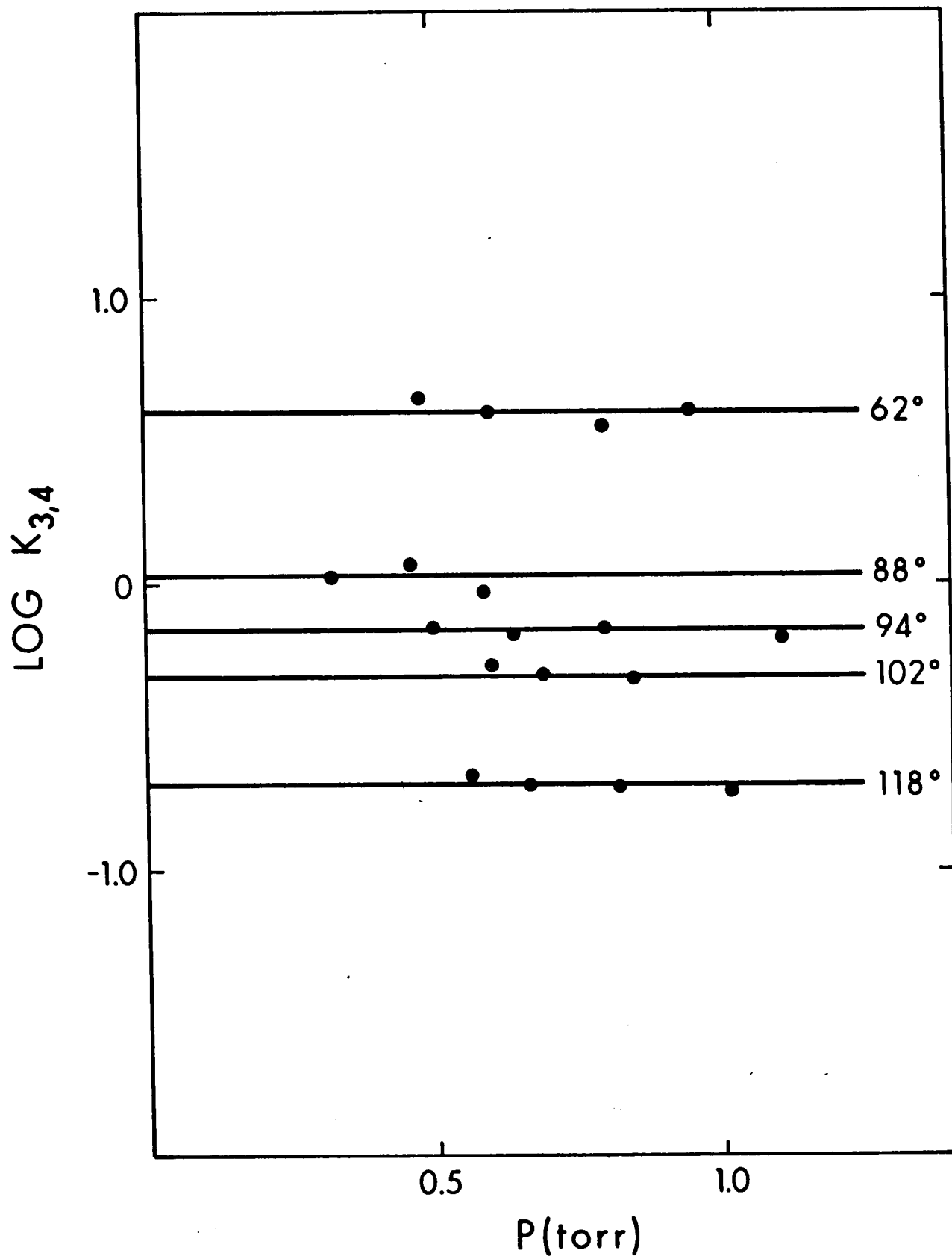
FIGURE 3.10 Plots of \text{Log } K_{3,4} for the Gas Phase Hydration of \text{Na}^+ , at Various Temperatures, Versus Pressure of \text{H}_2\text{O}
