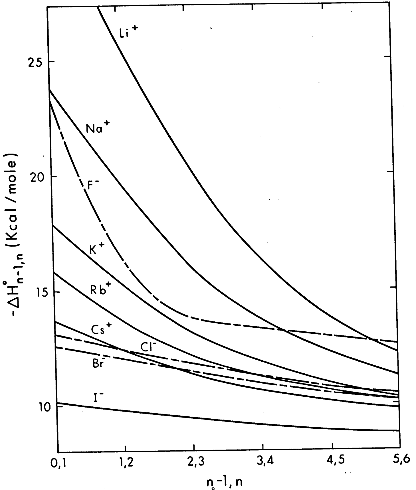
FIGURE 5.1 Comparison of \Delta H_{n-1,n}^{\circ} for hydration of alkali positive and halide negative ions.
