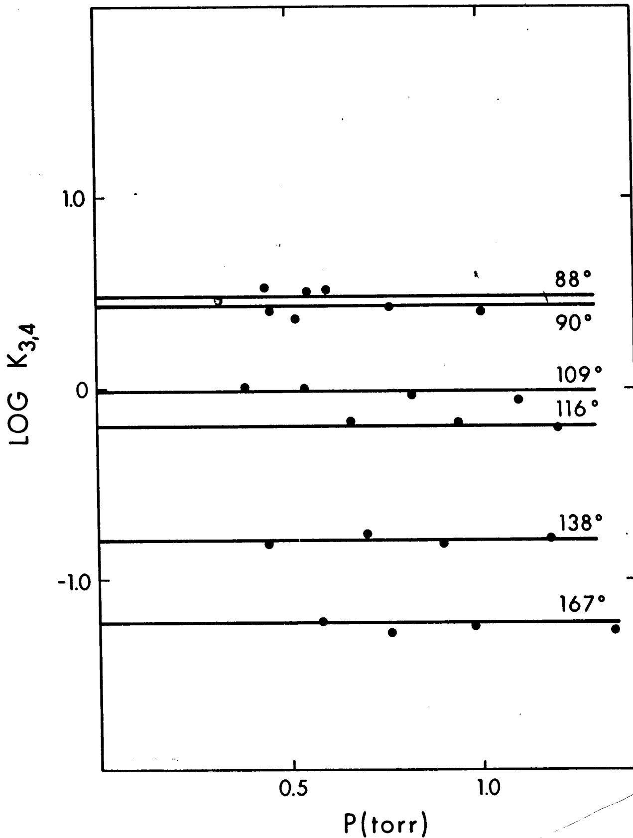
FIGURE 3.3 Plots of Log K_{3,4} for the Gas Phase Hydration of \text{Li}^+ , at Various Temperatures, Versus Pressure of \text{H}_2\text{O} .
