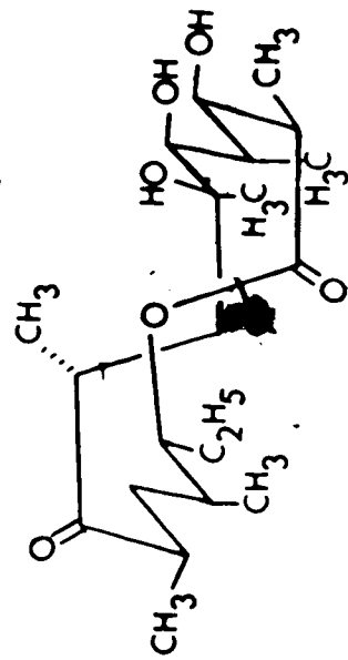
Celmer Conformation
