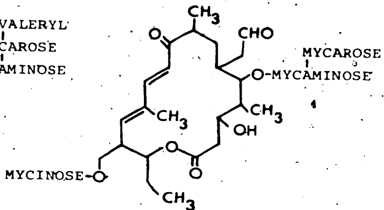
Tylochin
