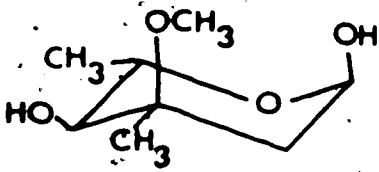
L-Cladinose
