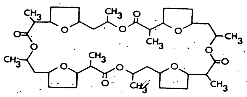
Nonactin
