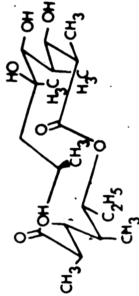
Perun Conformation
