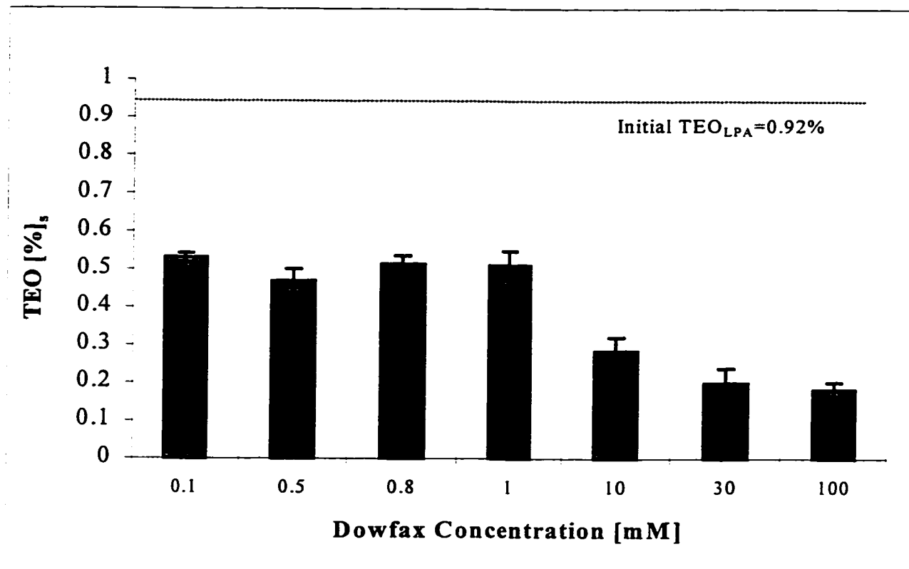
Figure 4.23. TEO_{MC} [% (s) dry soil] reductions following sequential Dowfax washing of LPA soil
