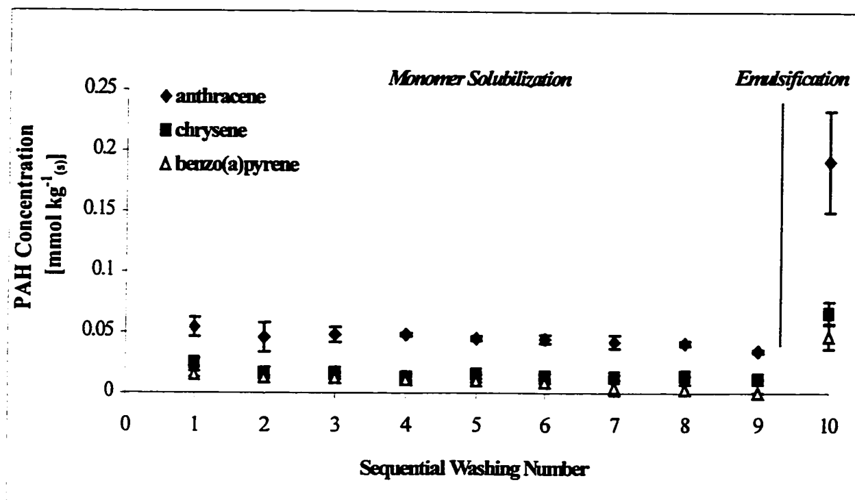
Figure 5. PAH concentrations [mmol kg -1 (s) dry soil] during sequential 1.0mM Dowfax washing of MPA soil
