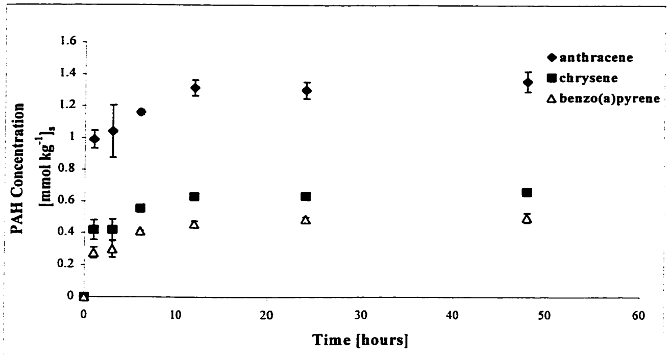
Figure 4.14. Apparent PAH concentrations [mmol kg -1 (s) dry soil] over time during 30mM Dowfax washing of MPA soil using a 10:1 solution to soil ratio
