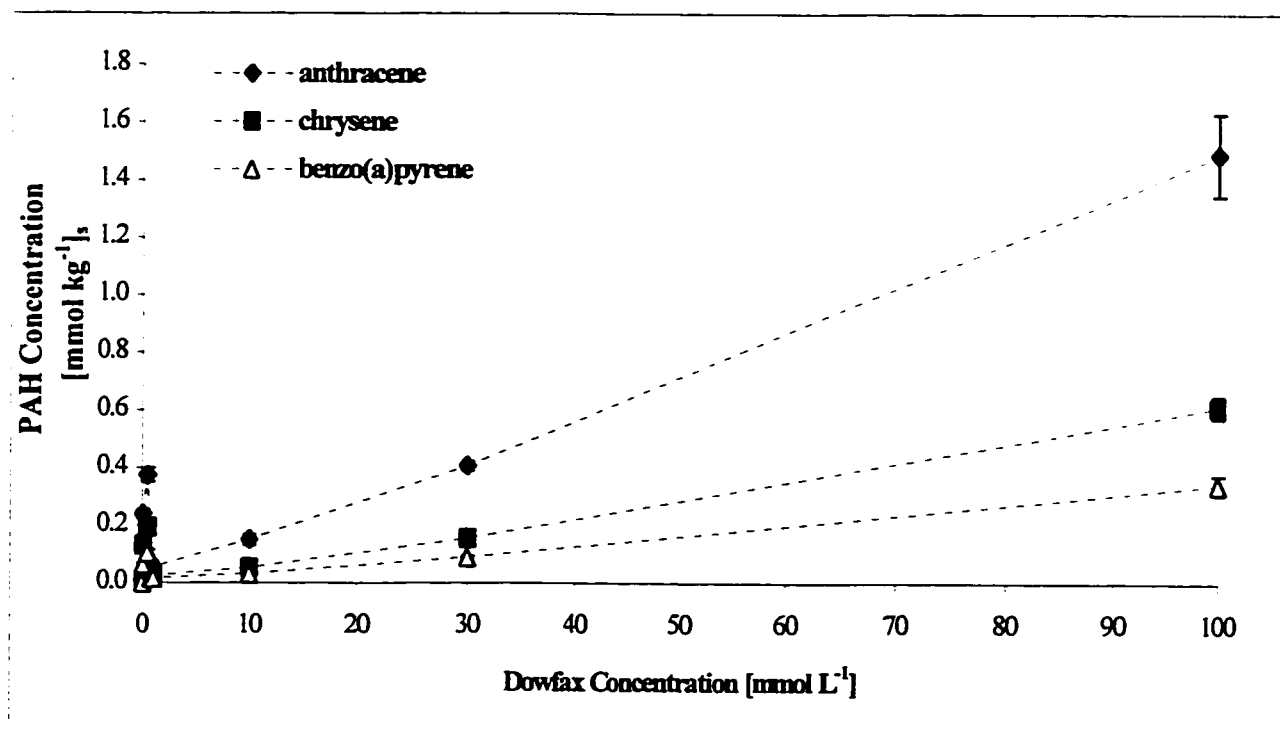
Figure 4.31. Micellar solubilization of target PAHs [mmol kg -1 (s) dry soil] following 24 hour Dowfax washing of MPA soil
