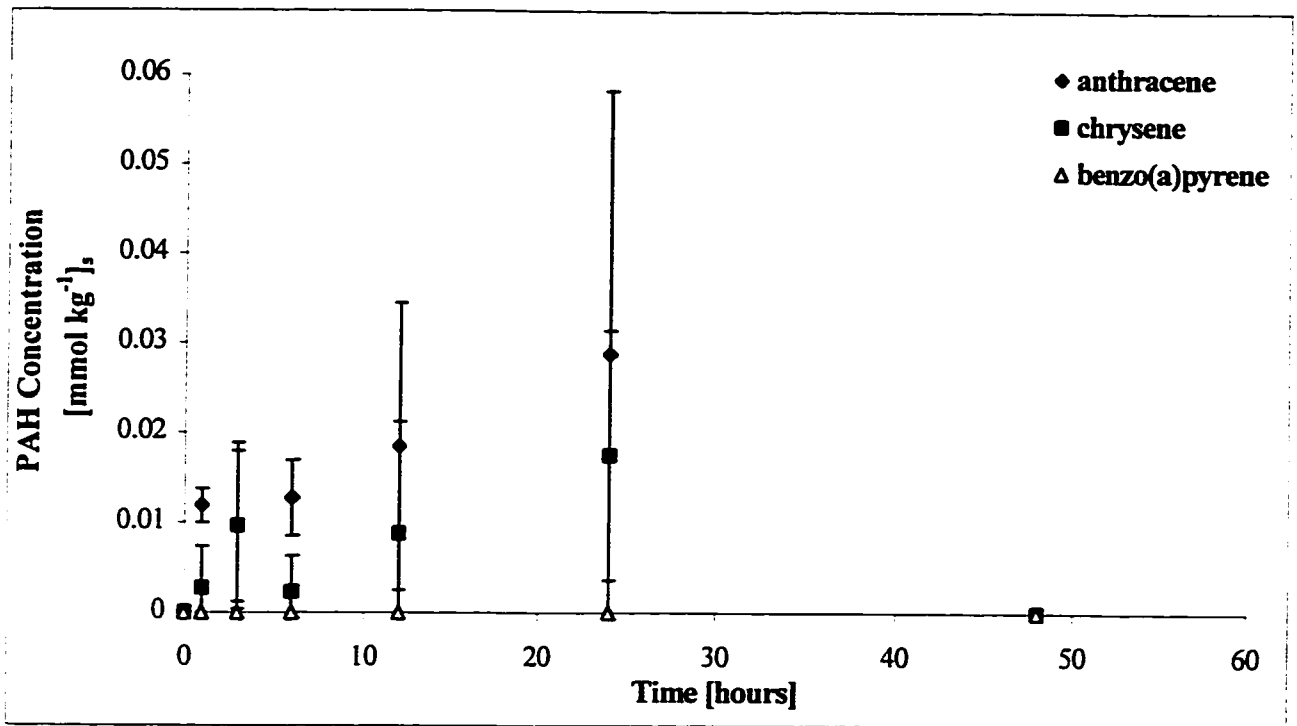
Figure 4.15. Apparent PAH concentrations [mmol kg -1 (s) dry soil] over time during 0.1mM Dowfax washing of MPA soil using a 20:1 solution to soil ratio
