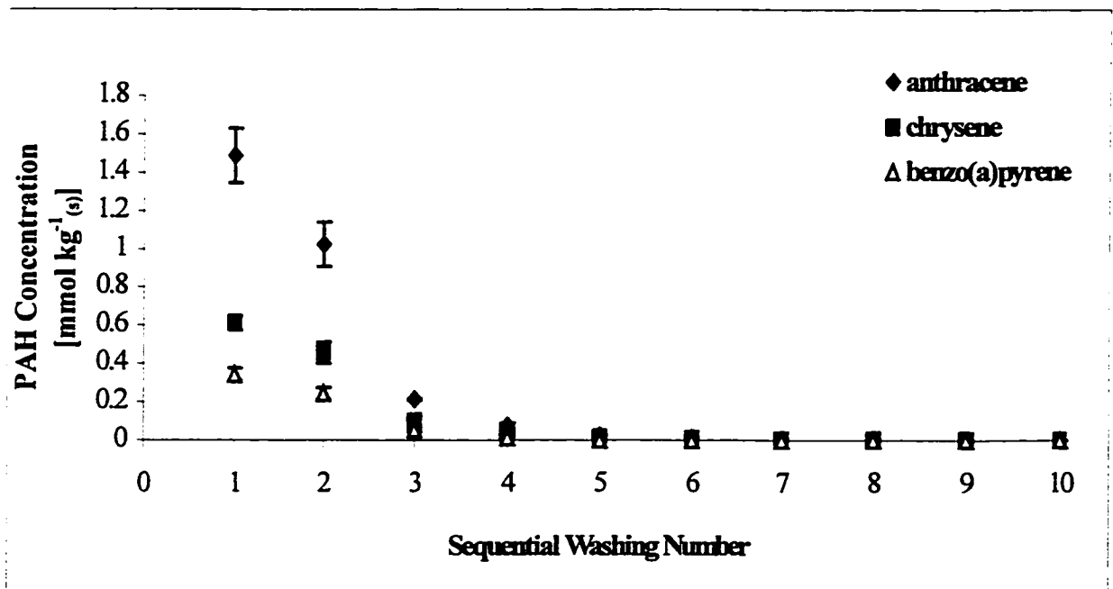
Figure 8. PAH concentrations [mmol kg -1 (s) dry soil] during sequential 100mM Dowfax washing of MPA soil.
