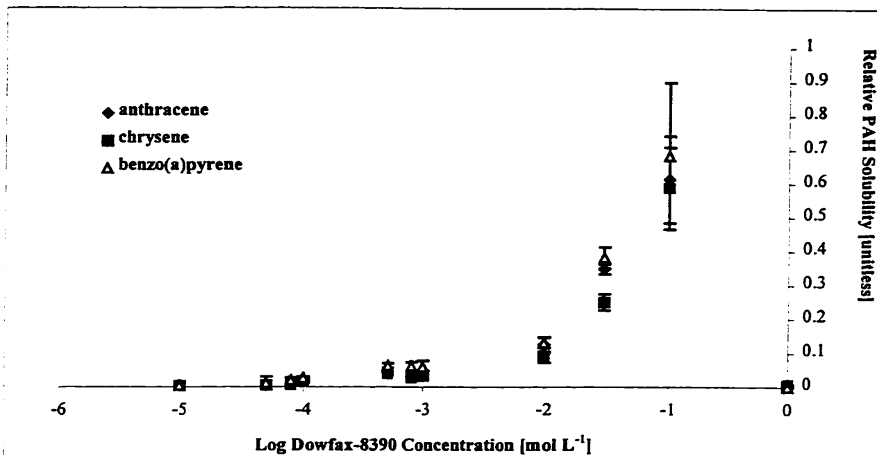
Figure 1. Normalized PAH solubility enhancement following 24 hr Dowfax washing of LPA soil
