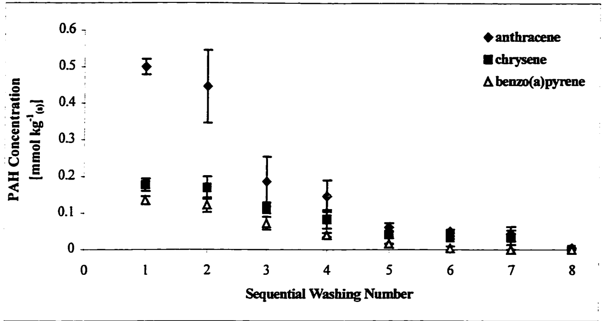
Figure 7. PAH concentrations [mmol kg -1 (s) dry soil] during sequential 30mM Dowfax washing of LPA soil
