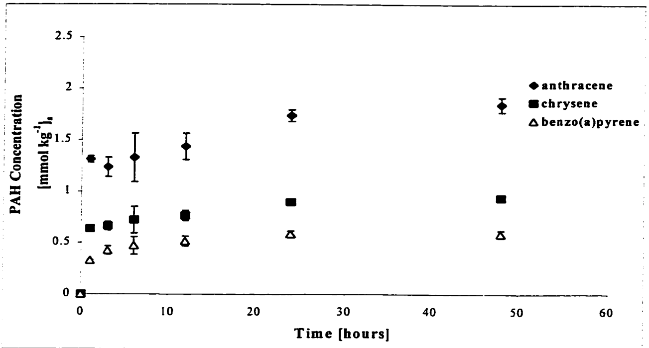
Figure 4.17. Apparent PAH concentrations [ \text{mmol kg}^{-1}_{(s)} dry soil] over time during 30mM Dowfax washing of MPA soil using a 20:1 solution to soil ratio
