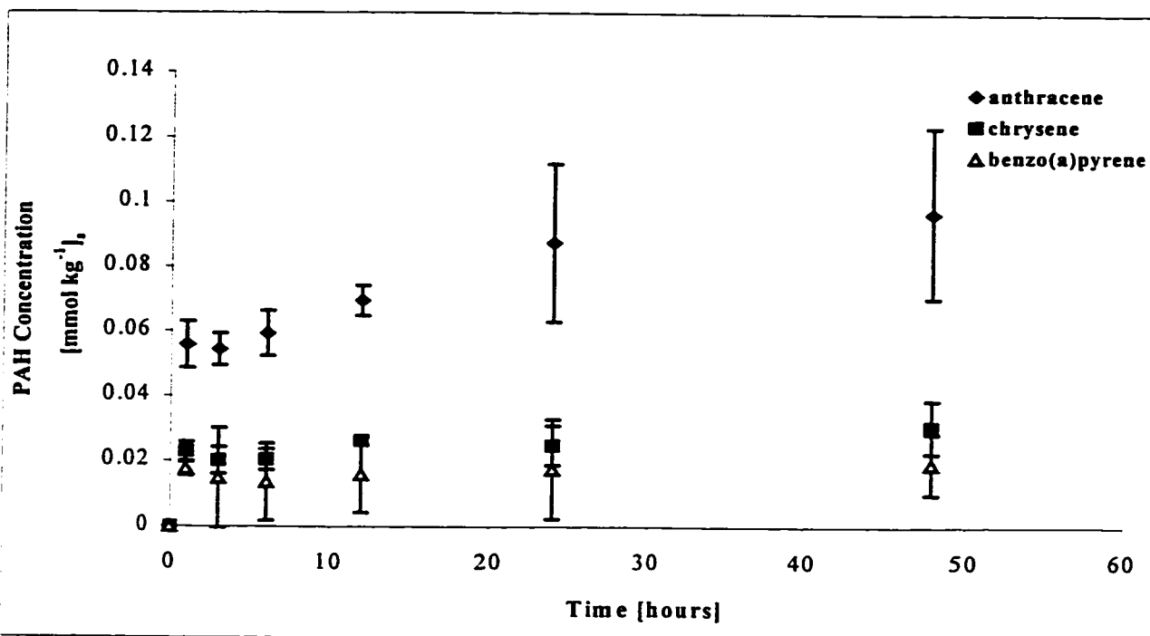
Figure 4.16. Apparent PAH concentrations [ \text{mmol kg}^{-1}_{(s)} dry soil] over time during 1.0mM Dowfax washing of MPA soil using a 20:1 solution to soil ratio
