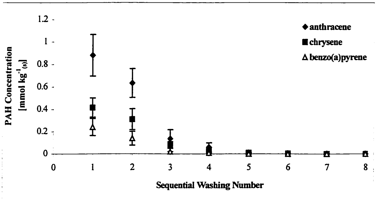
Figure 8. PAH concentrations [mmol kg -1 (s) dry soil] during sequential 100mM Dowfax washing of LPA soil
