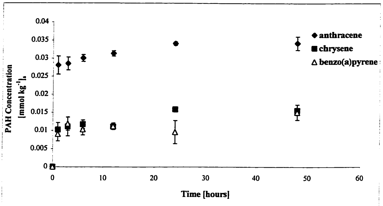
Figure 4.13. Apparent PAH concentrations [ \text{mmol kg}^{-1}_{(\text{s})} dry soil] over time during 1.0mM Dowfax washing of MPA soil using a 10:1 solution to soil ratio
