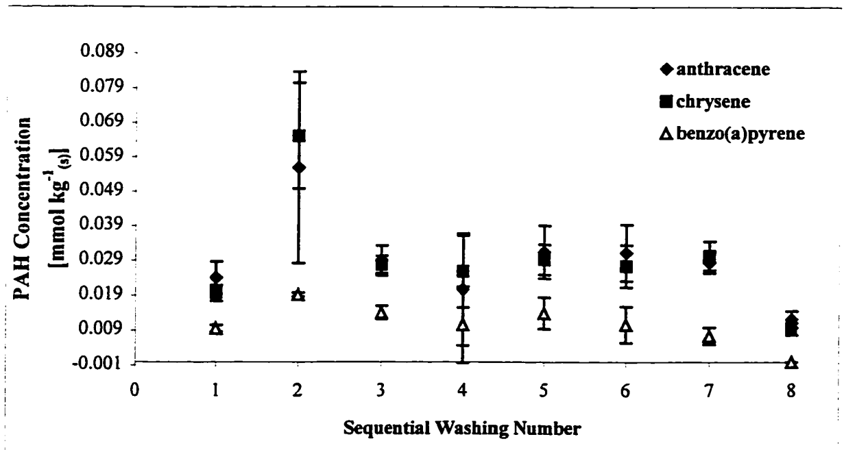
Figure 2. PAH Concentrations [ \text{mmol kg}^{-1} \text{ (s) dry soil} ] during sequential 0.1mM Dowfax washing of LPA soil
