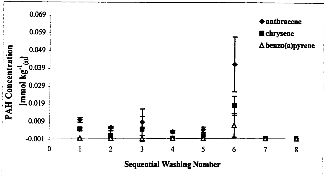
Figure 1. PAH concentrations [ \text{mmol kg}^{-1} \text{ (s) dry soil} ] during sequential \text{ddH}_2\text{O} washing of LPA soil
