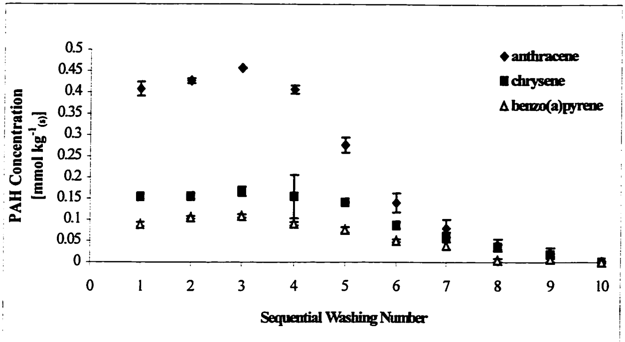
Figure 7. PAH concentrations [mmol kg -1 (s) dry soil] during sequential 30mM Dowfax washing of MPA soil
