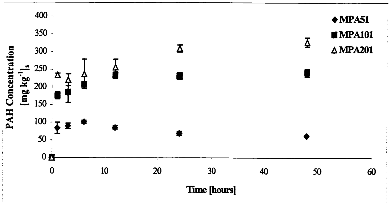
Figure 4.18. Apparent anthracene concentration [ \text{mg kg}^{-1}_{(s)} dry soil] over time during 30mM Dowfax washing of MPA soil using various solution to soil ratios
