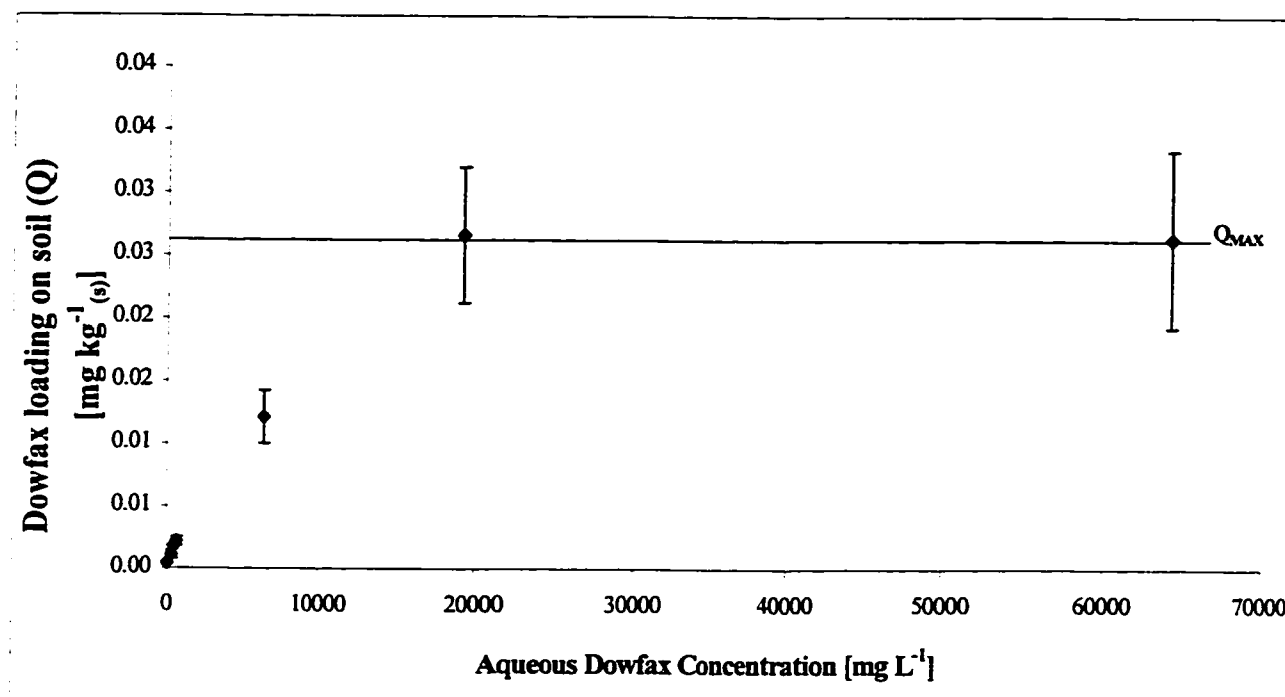
Figure 4.33. Sorption of Dowfax [ \text{mg kg}^{-1}(\text{s}) dry soil] on MPA soil
