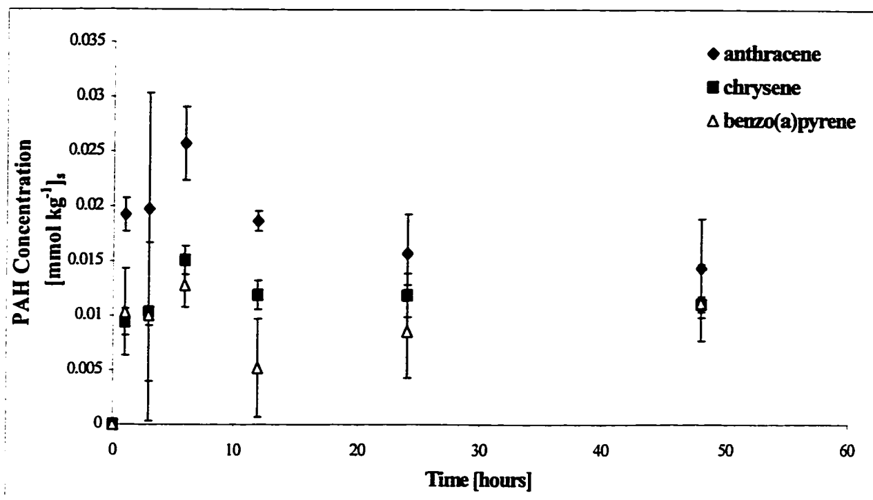
Figure 4.12. Apparent PAH concentrations [ \text{mmol kg}^{-1}_s ] dry soil over time during 0.1mM Dowfax washing of MPA soil using a 10:1 solution to soil ratio
