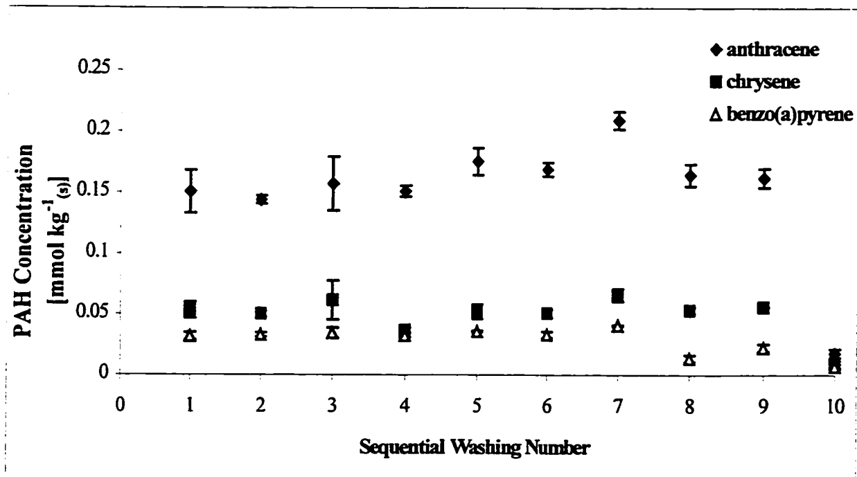
Figure 6. PAH concentrations [mmol kg -1 (s) dry soil] during sequential 10mM Dowfax washing of MPA soil
