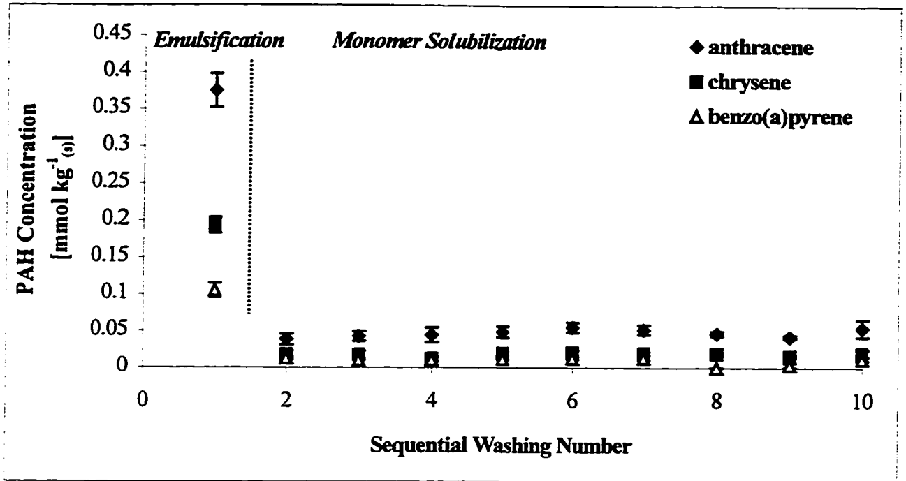
Figure 3. PAH concentrations [ \text{mmol kg}^{-1}(\text{s}) dry soil] during sequential 0.5mM Dowfax washing of MPA soil
