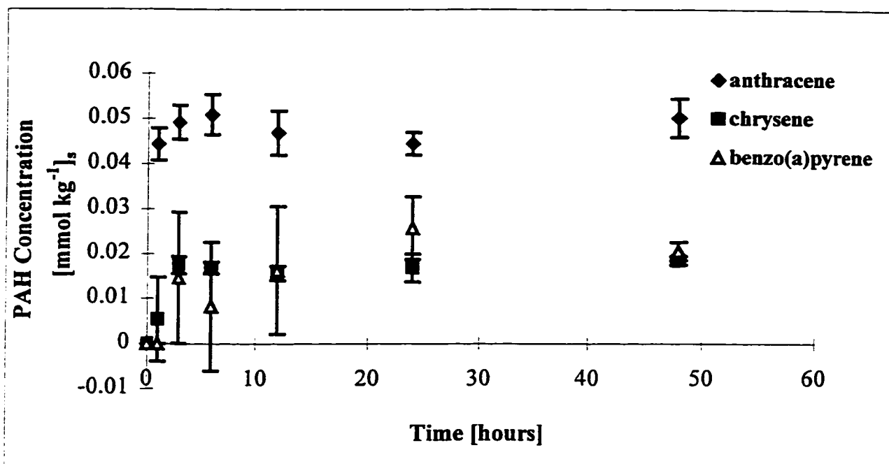
Figure 4.6. Apparent PAH concentrations [mmol kg -1 (s) dry weight] over time during 1.0mM Dowfax washing of LPA soil using a 20 : 1 solution to soil ratio
