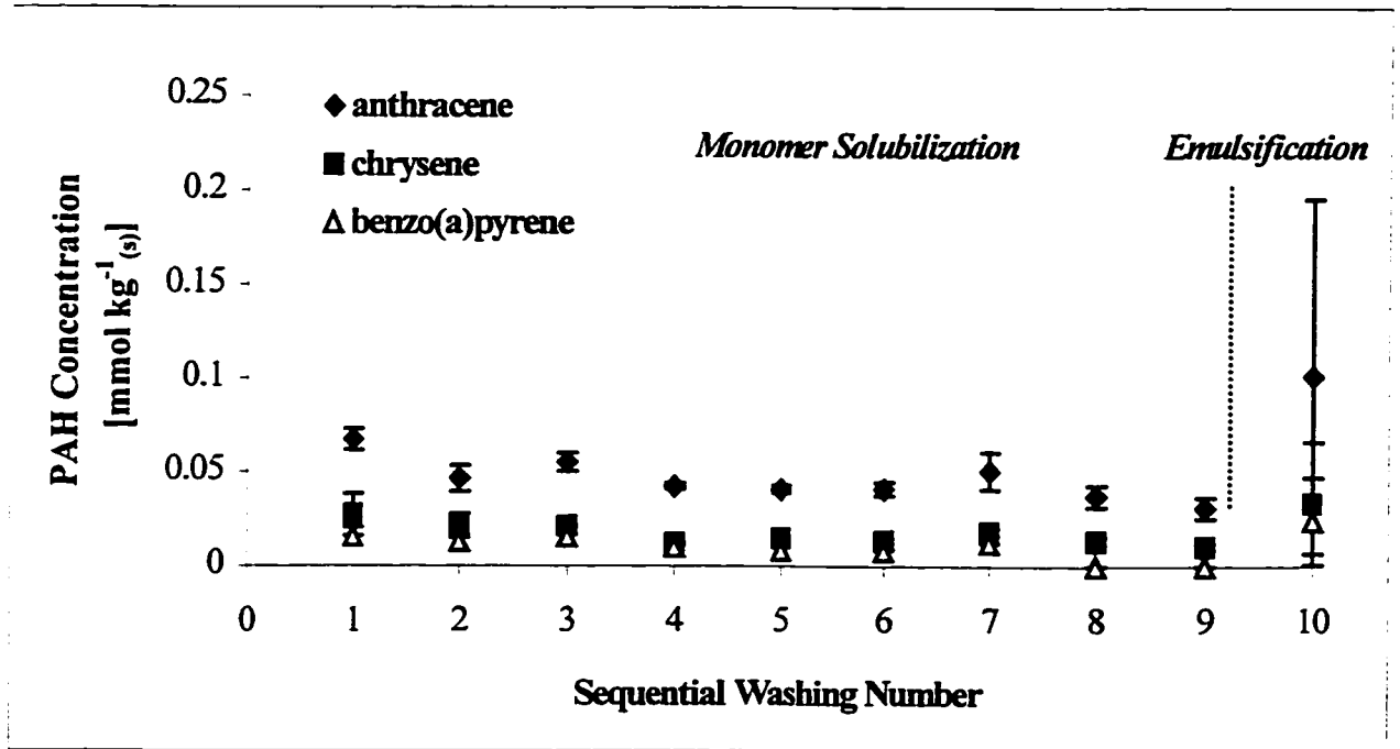
Figure 4. PAH concentrations [ \text{mmol kg}^{-1}(\text{s}) dry soil] during sequential 0.8mM Dowfax washing of MPA soil
