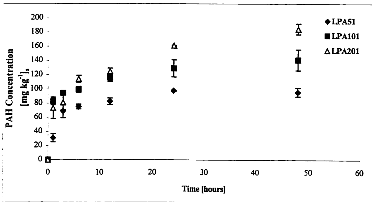
Figure 4.8. Apparent anthracene concentration [ \text{mg kg}^{-1}_{(s)} dry weight] over time during 30mM Dowfax washing of LPA soil using various solution to soil ratios
