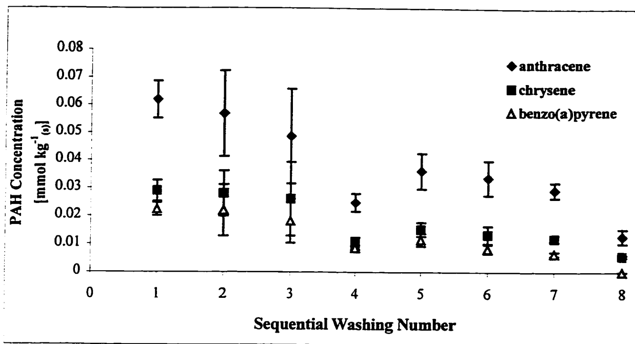
Figure 3. PAH concentrations [mmol kg -1 (s) dry soil] during sequential 0.5mM Dowfax washing of LPA soil
